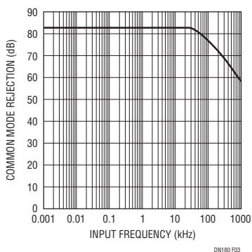
Figure 3. Input Common Mode Rejection vs Input Frequency
