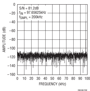
Figure 2. LTC1418 FFT
