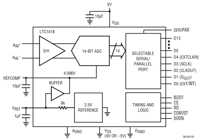
Figure 1. LTC1418 Block Diagram
