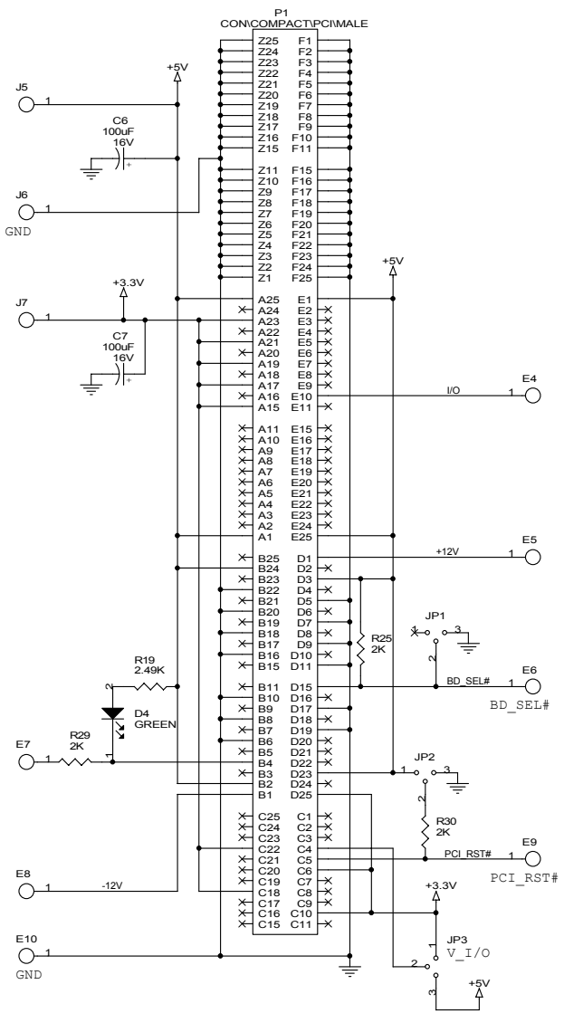
SYSTEM BACKPLANE
