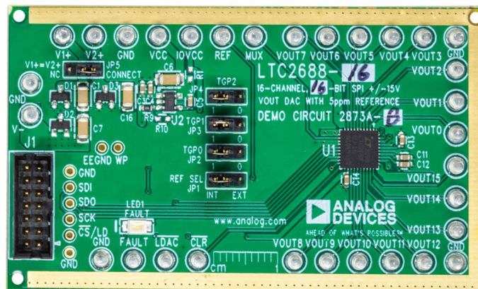
Figure 1. DC2873A-B Evaluation Board
