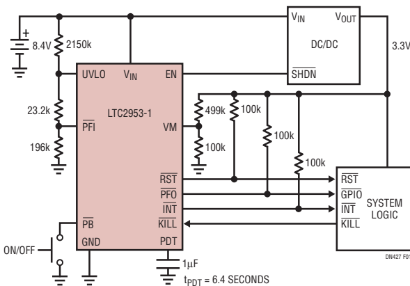
Figure 1. Typical Application
