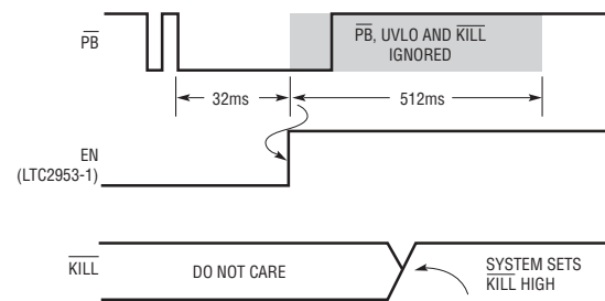
Figure 2. Orderly Power On
