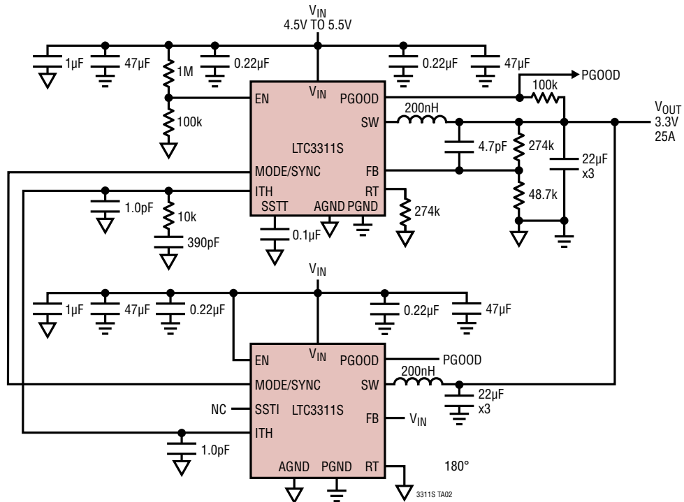
Dual Phase 5V to 3.3V, 25A, Forced Continuous Mode
