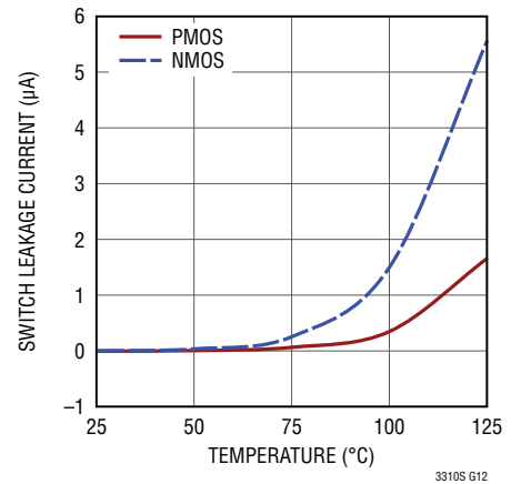
Switch Leakage
