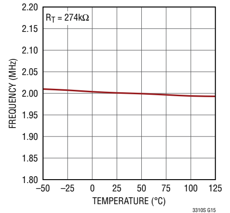
Switching Frequency
