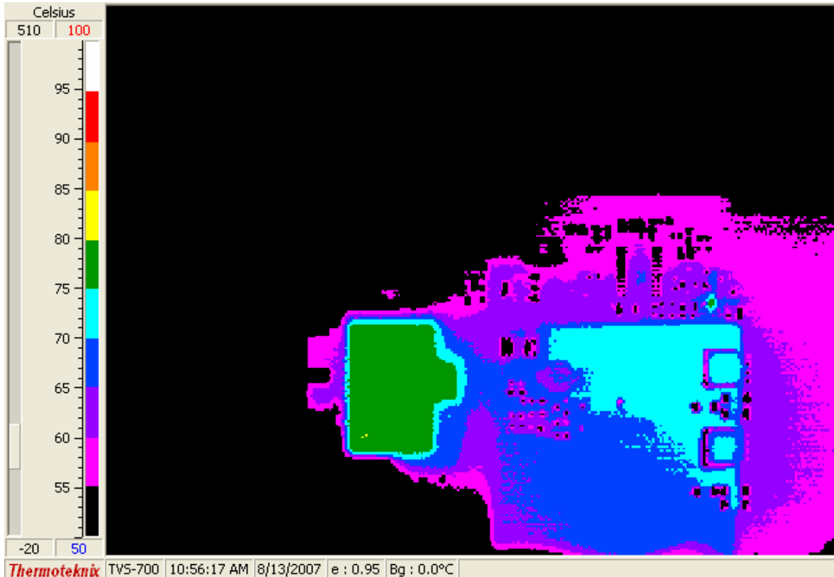
Figure 12. Temp Data (48Vin, 40A, 200LFM airflow – bottom)
