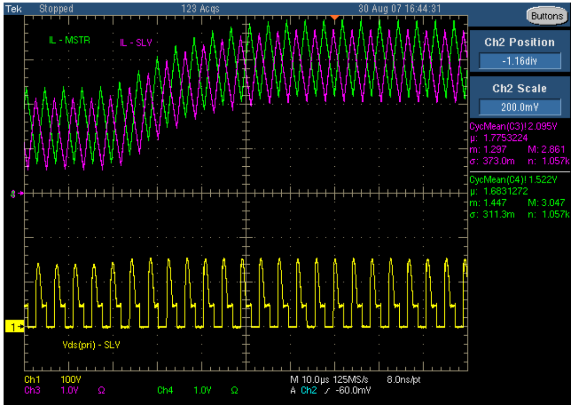
Figure 9. Transient Sharing of Inductor Current (48Vin, 30A to 60A, PolyPhase)
