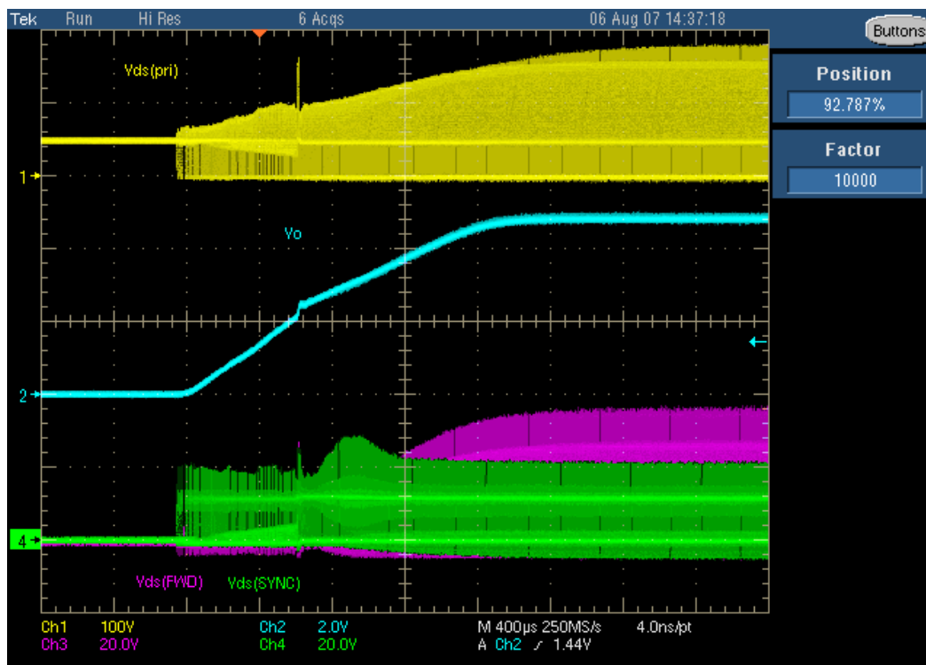
Figure 7. Turn-on (48Vin, 40A, Single Phase)
