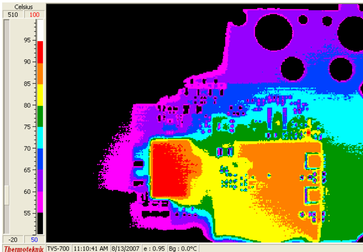
Figure 14. Temp Data (48Vin, 36A, 0LFM airflow – bottom)
