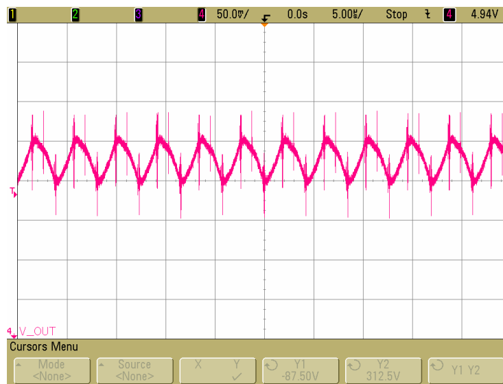
Figure 4. Output Voltage Ripple (48V in , 40A, Single Phase)
