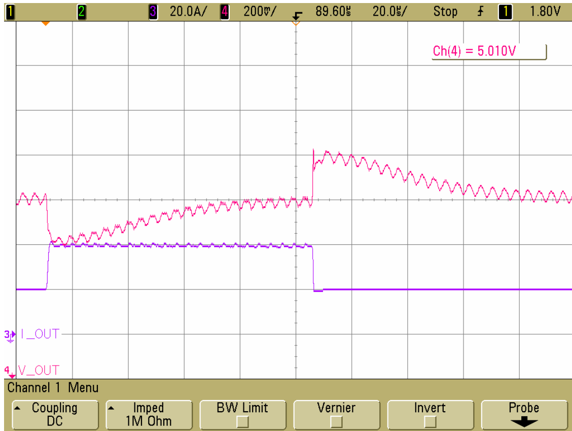
Figure 5. Load Transient Response (48Vin, 20A to 40A to 20A at 10A/us, Single Phase)
