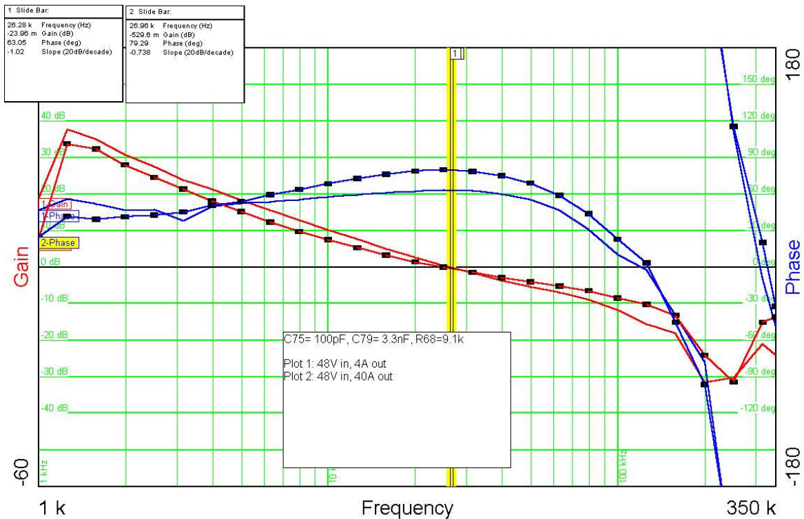
Figure 6. Loop Response (48Vin, 4A & 40A, Single Phase)
