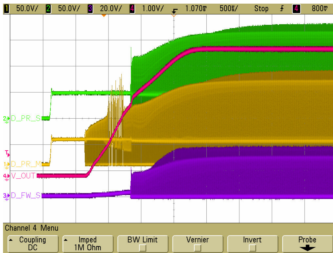
Figure 8. Turn-on (48Vin, 80A, PolyPhase)
