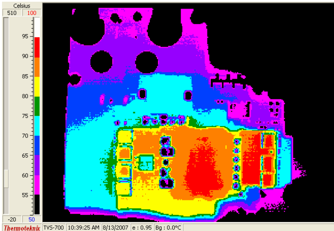
Figure 13. Temp Data (48Vin, 36A, 0LFM airflow – top)
