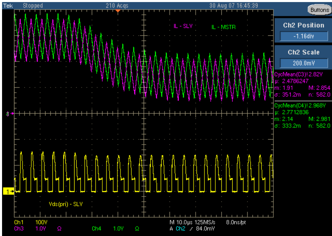
Figure 10. Transient Sharing of Inductor Current (48Vin, 60A to 30A, PolyPhase)
