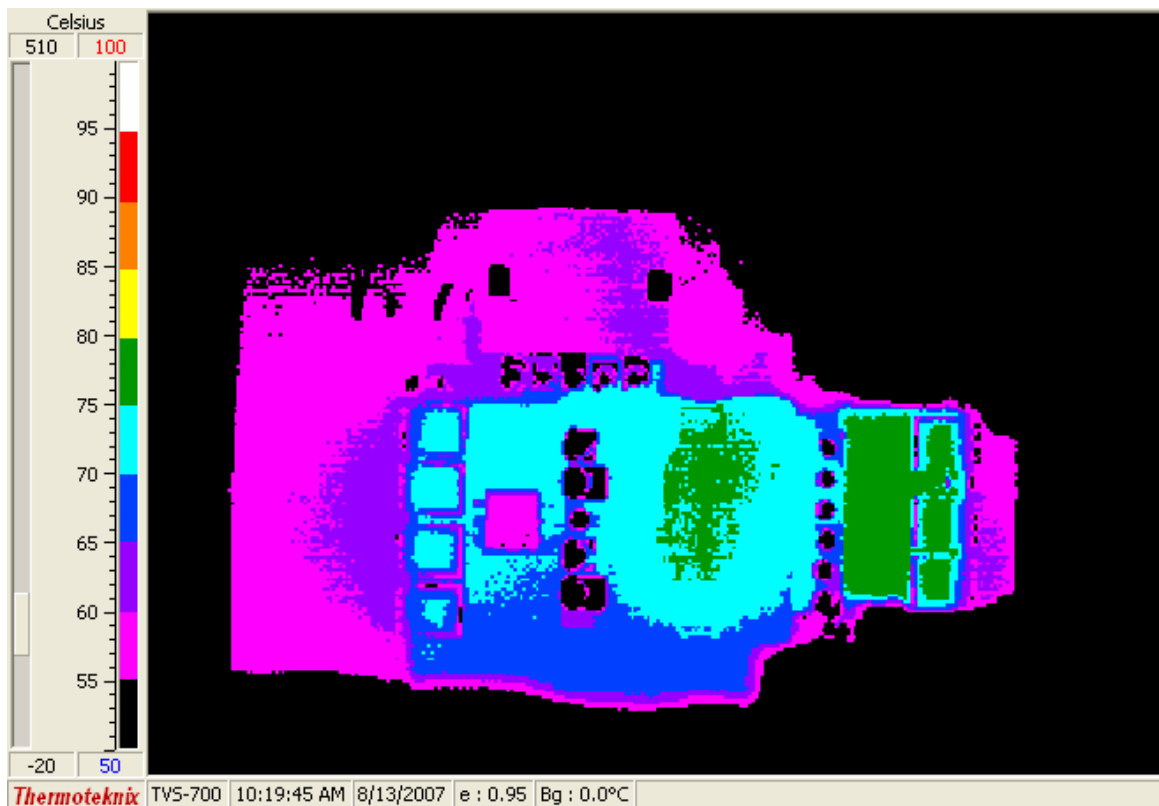
Figure 11. Temp Data (48Vin, 40A, 200LFM airflow – top)
