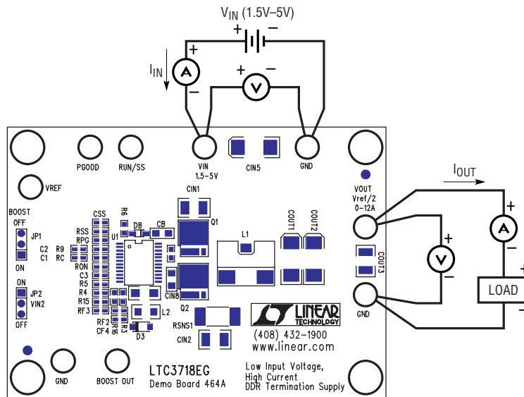
Figure 1. Proper Measurement Equipment Setup for Output Sourcing Current
