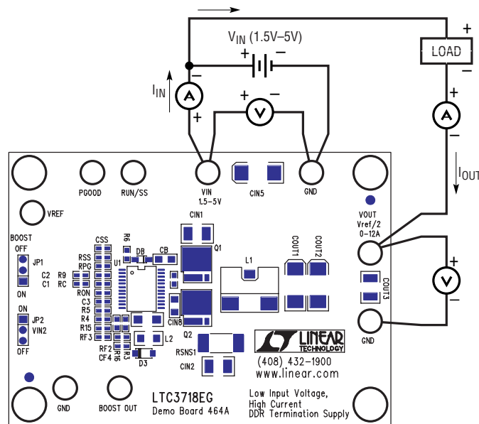
Figure 2. Proper Measurement Equipment Setup for Output Sinking Current
