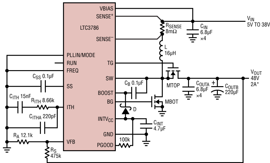
High Efficiency 48V Boost Converter
