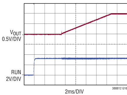
Soft-Start Ramp
