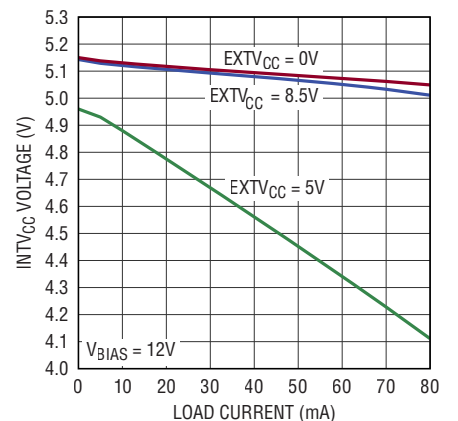
INTV CC and EXT CC vs Load Current
