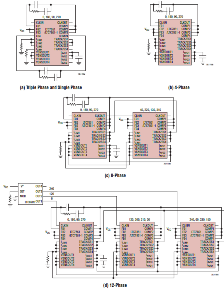
Figure 5. LTC7851 Multiple Phase Configurations
