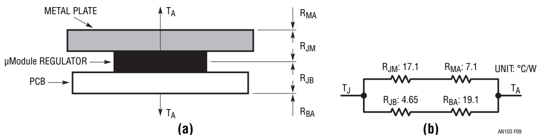
Figure 9. Thermal Model for Case 3
