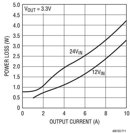
Figure 11. Power Loss vs Load Current
