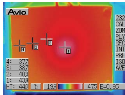
CONDITIONS: 24V TO 3.3V AT 10A, 25°C, NO AIR FLOW. A BERGQUIST “GAP PAD 1000” IS USED BETWEEN THE \mu Module PACKAGE AND THE METAL PLATE. 0.04 THICKNESS 2°C/W. (METAL PLATE = 100mm \times 75mm \times 1.5mm)
