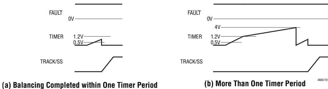
Figure 1. Charge Balancing During Power-Up
