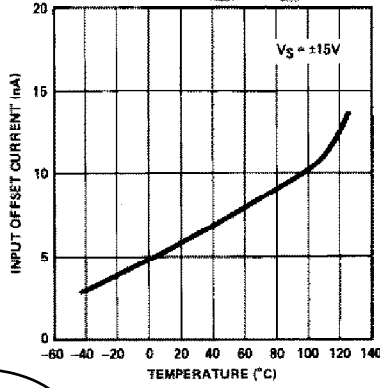
OFFSET CURRENT vs TEMPERATURE
