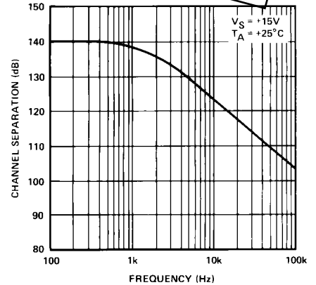
MATCHING CHARACTERISTICS CHANNEL SEPARATION vs FREQUENCY
