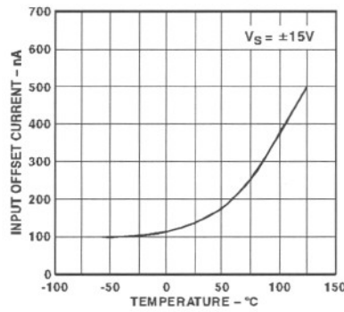
TPC 2. Input Offset Current vs. Temperature
