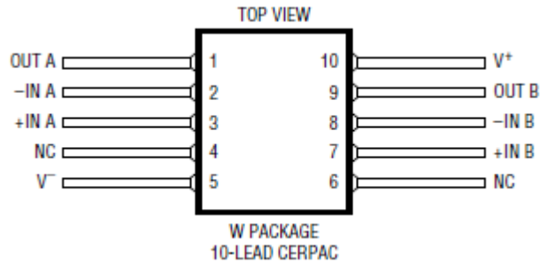
Figure B.2. W package drawing (for reference only). This figure was extracted from Linear Technology RH1013M Datasheet I.D No. 66-11-1013 Revision E.
