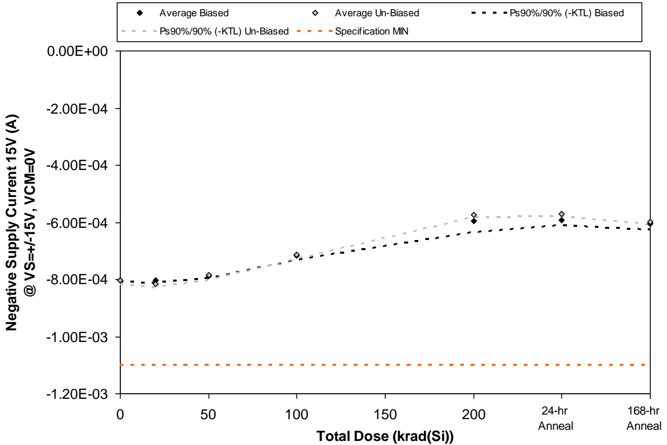
Figure 5.2. Plot of Negative Supply Current 15V (A) @ VS= \pm 15V, VCM=0V versus total dose. The solid diamonds are the average of the measured data points for the samples irradiated under electrical bias while the shaded diamonds are the average of the measured data points for the samples irradiated with all pins tied to ground. The black lines (solid and/or dashed) are the upper and/or lower confidence limits, as determined by KTL statistics, on the samples irradiated under electrical bias while the gray lines (solid and/or dashed) are the upper and/or lower confidence limits, as determined by KTL statistics, on the samples irradiated in the unbiased condition. The red dotted line(s) are the pre- and/or post-irradiation minimum and/or maximum specification value as defined in the datasheet and/or test plan.
