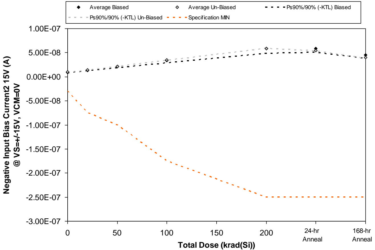
Figure 5.10. Plot of Negative Input Bias Current2 15V (A) @ VS=+/-15V, VCM=0V versus total dose. The solid diamonds are the average of the measured data points for the samples irradiated under electrical bias while the shaded diamonds are the average of the measured data points for the samples irradiated with all pins tied to ground. The black lines (solid and/or dashed) are the upper and/or lower confidence limits, as determined by KTL statistics, on the samples irradiated under electrical bias while the gray lines (solid and/or dashed) are the upper and/or lower confidence limits, as determined by KTL statistics, on the samples irradiated in the unbiased condition. The red dotted line(s) are the pre- and/or post-irradiation minimum and/or maximum specification value as defined in the datasheet and/or test plan.
