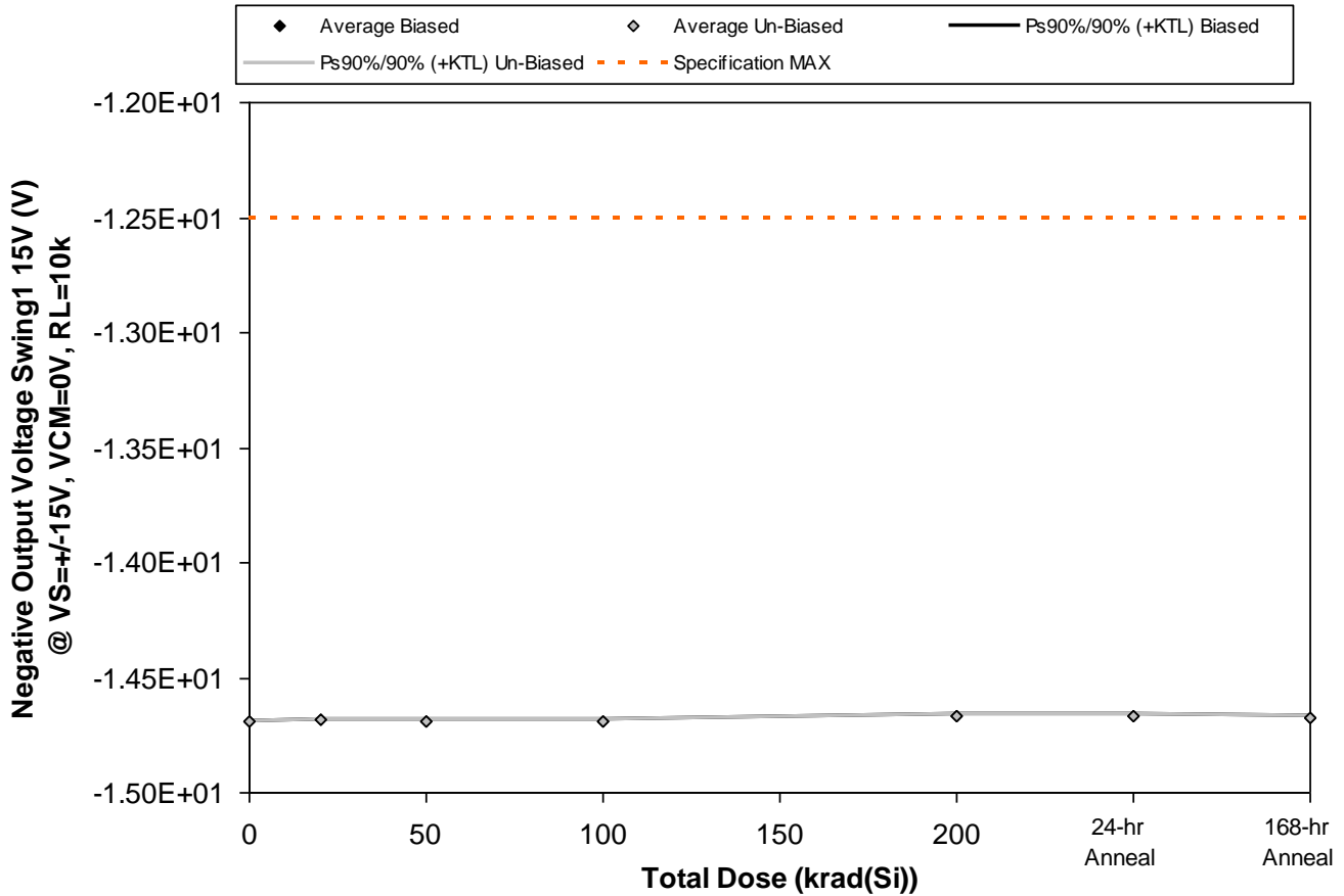
Figure 5.19. Plot of Negative Output Voltage Swing1 15V (V) @ VS= \pm 15V, VCM=0V, RL=10k versus total dose. The solid diamonds are the average of the measured data points for the samples irradiated under electrical bias while the shaded diamonds are the average of the measured data points for the samples irradiated with all pins tied to ground. The black lines (solid and/or dashed) are the upper and/or lower confidence limits, as determined by KTL statistics, on the samples irradiated under electrical bias while the gray lines (solid and/or dashed) are the upper and/or lower confidence limits, as determined by KTL statistics, on the samples irradiated in the unbiased condition. The red dotted line(s) are the pre- and/or post-irradiation minimum and/or maximum specification value as defined in the datasheet and/or test plan.
