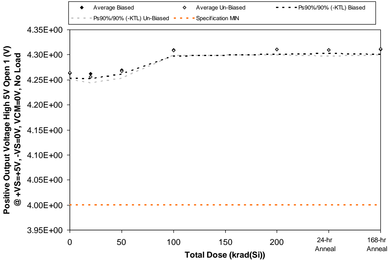
Figure 5.35. Plot of Positive Output Voltage High 5V Open 1 (V) @ +VS=+5V, -VS=0V, VCM=0V, No Load versus total dose. The solid diamonds are the average of the measured data points for the samples irradiated under electrical bias while the shaded diamonds are the average of the measured data points for the samples irradiated with all pins tied to ground. The black lines (solid and/or dashed) are the upper and/or lower confidence limits, as determined by KTL statistics, on the samples irradiated under electrical bias while the gray lines (solid and/or dashed) are the upper and/or lower confidence limits, as determined by KTL statistics, on the samples irradiated in the unbiased condition. The red dotted line(s) are the pre- and/or post-irradiation minimum and/or maximum specification value as defined in the datasheet and/or test plan.
