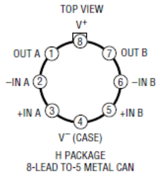
Figure B.2. H package drawing (for reference only). This figure was extracted from Linear Technology RH1013M Datasheet Revision E.
