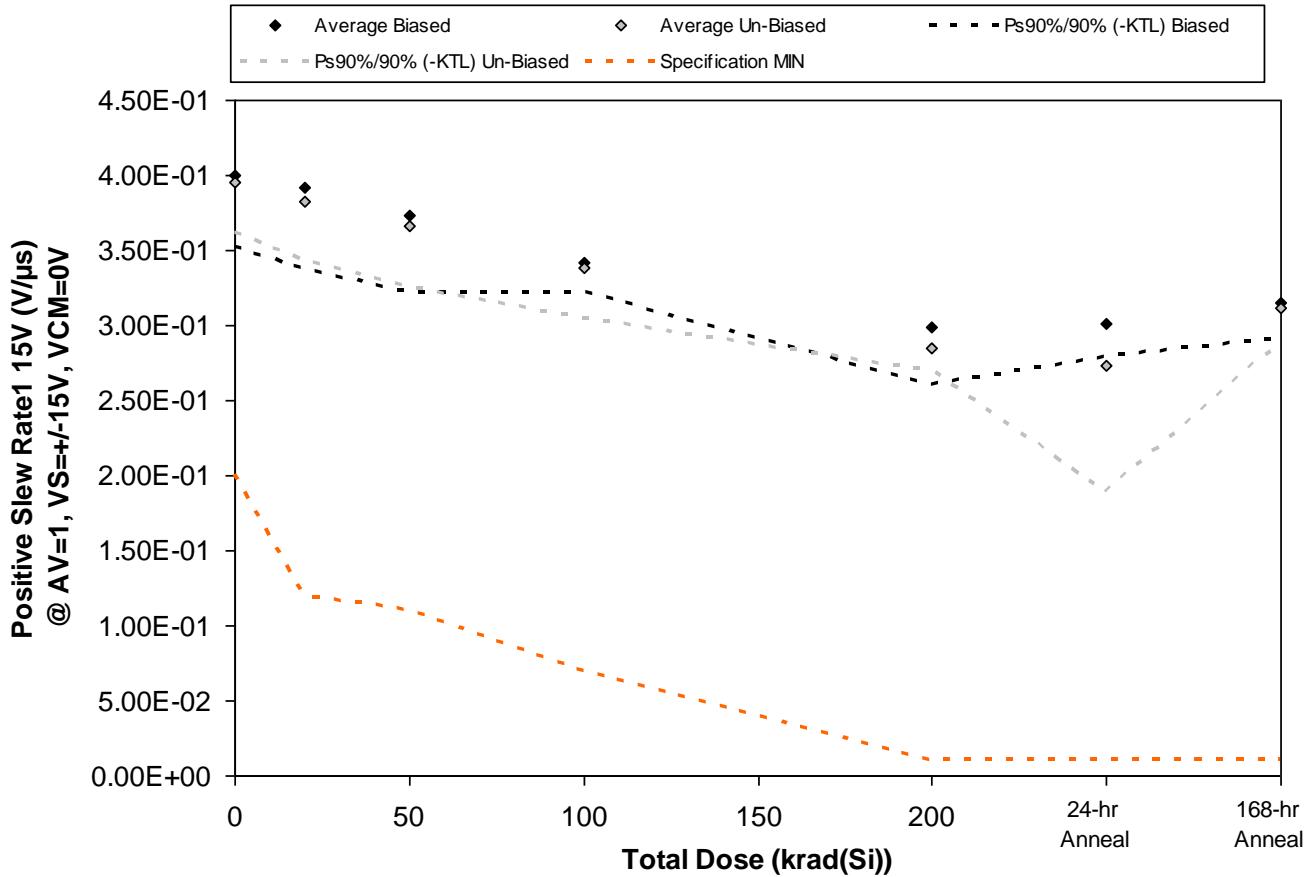
Figure 5.21. Plot of Positive Slew Rate 15V (V/μs) @ AV=1, VS=+/-15V, VCM=0V versus total dose. The solid diamonds are the average of the measured data points for the samples irradiated under electrical bias while the shaded diamonds are the average of the measured data points for the samples irradiated with all pins tied to ground. The black lines (solid and/or dashed) are the upper and/or lower confidence limits, as determined by KTL statistics, on the samples irradiated under electrical bias while the gray lines (solid and/or dashed) are the upper and/or lower confidence limits, as determined by KTL statistics, on the samples irradiated in the unbiased condition. The red dotted line(s) are the pre- and/or post-irradiation minimum and/or maximum specification value as defined in the datasheet and/or test plan.
