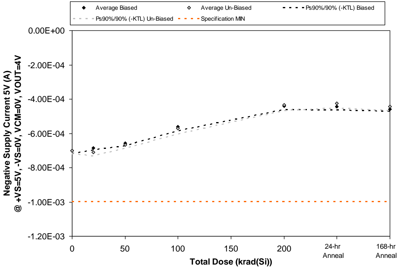
Figure 5.26. Plot of Negative Supply Current 5V (A) @ +VS=5V, -VS=0V, VCM=0V, VOUT=4V versus total dose. The solid diamonds are the average of the measured data points for the samples irradiated under electrical bias while the shaded diamonds are the average of the measured data points for the samples irradiated with all pins tied to ground. The black lines (solid and/or dashed) are the upper and/or lower confidence limits, as determined by KTL statistics, on the samples irradiated under electrical bias while the gray lines (solid and/or dashed) are the upper and/or lower confidence limits, as determined by KTL statistics, on the samples irradiated in the unbiased condition. The red dotted line(s) are the pre- and/or post-irradiation minimum and/or maximum specification value as defined in the datasheet and/or test plan.
