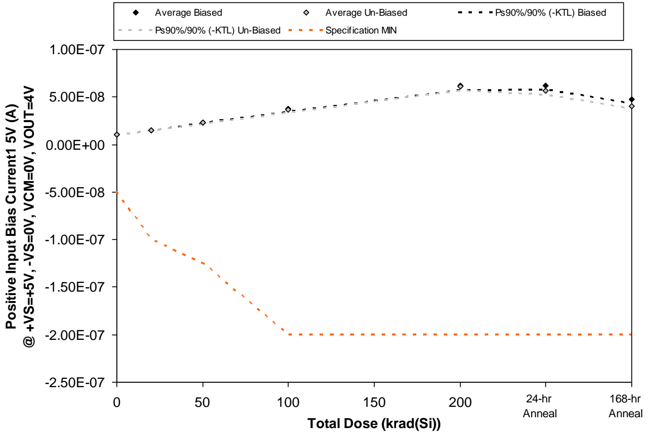
Figure 5.31. Plot of Positive Input Bias Current1 5V (A) @ +VS=+5V, -VS=0V, VCM=0V, VOUT=4V versus total dose. The solid diamonds are the average of the measured data points for the samples irradiated under electrical bias while the shaded diamonds are the average of the measured data points for the samples irradiated with all pins tied to ground. The black lines (solid and/or dashed) are the upper and/or lower confidence limits, as determined by KTL statistics, on the samples irradiated under electrical bias while the gray lines (solid and/or dashed) are the upper and/or lower confidence limits, as determined by KTL statistics, on the samples irradiated in the unbiased condition. The red dotted line(s) are the pre- and/or post-irradiation minimum and/or maximum specification value as defined in the datasheet and/or test plan.
