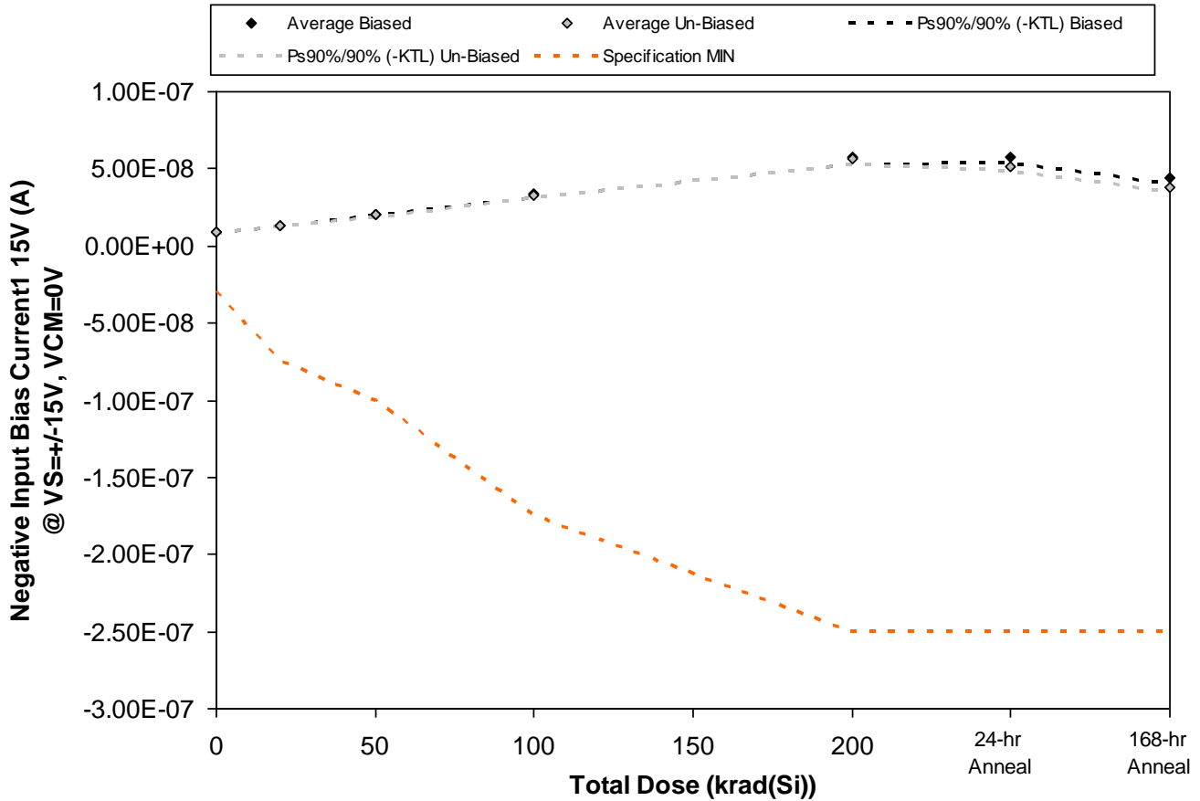
Figure 5.9. Plot of Negative Input Bias Current1 15V (A) @ VS=+-15V, VCM=0V versus total dose. The solid diamonds are the average of the measured data points for the samples irradiated under electrical bias while the shaded diamonds are the average of the measured data points for the samples irradiated with all pins tied to ground. The black lines (solid and/or dashed) are the upper and/or lower confidence limits, as determined by KTL statistics, on the samples irradiated under electrical bias while the gray lines (solid and/or dashed) are the upper and/or lower confidence limits, as determined by KTL statistics, on the samples irradiated in the unbiased condition. The red dotted line(s) are the pre- and/or post-irradiation minimum and/or maximum specification value as defined in the datasheet and/or test plan.
