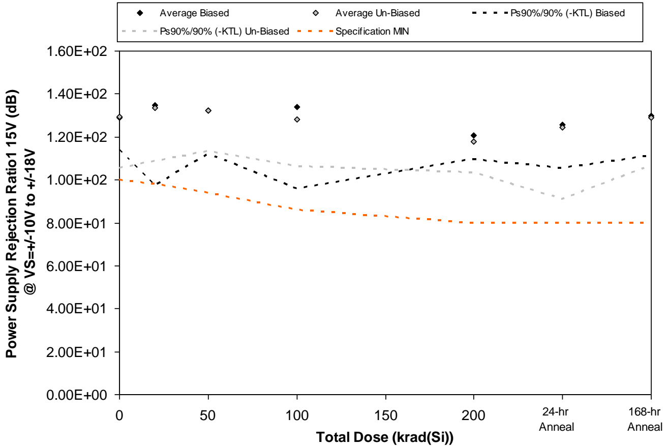
Figure 5.13. Plot of Power Supply Rejection Ratio 15V (dB) @ VS=+-10V to +/-18V versus total dose. The solid diamonds are the average of the measured data points for the samples irradiated under electrical bias while the shaded diamonds are the average of the measured data points for the samples irradiated with all pins tied to ground. The black lines (solid and/or dashed) are the upper and/or lower confidence limits, as determined by KTL statistics, on the samples irradiated under electrical bias while the gray lines (solid and/or dashed) are the upper and/or lower confidence limits, as determined by KTL statistics, on the samples irradiated in the unbiased condition. The red dotted line(s) are the pre- and/or post-irradiation minimum and/or maximum specification value as defined in the datasheet and/or test plan.
