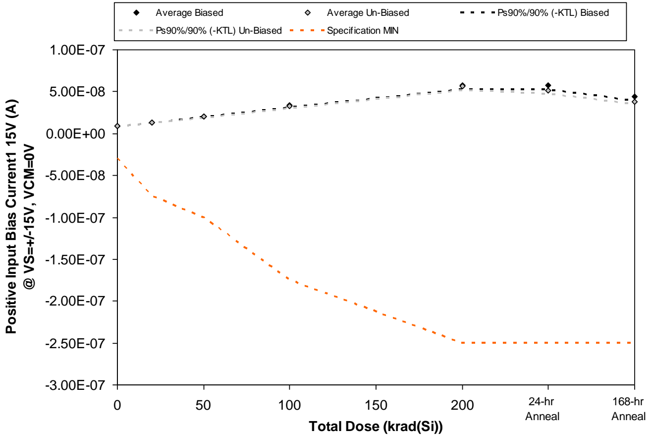
Figure 5.7. Plot of Positive Input Bias Current1 15V (A) @ VS=+-15V, VCM=0V versus total dose. The solid diamonds are the average of the measured data points for the samples irradiated under electrical bias while the shaded diamonds are the average of the measured data points for the samples irradiated with all pins tied to ground. The black lines (solid and/or dashed) are the upper and/or lower confidence limits, as determined by KTL statistics, on the samples irradiated under electrical bias while the gray lines (solid and/or dashed) are the upper and/or lower confidence limits, as determined by KTL statistics, on the samples irradiated in the unbiased condition. The red dotted line(s) are the pre- and/or post-irradiation minimum and/or maximum specification value as defined in the datasheet and/or test plan.
