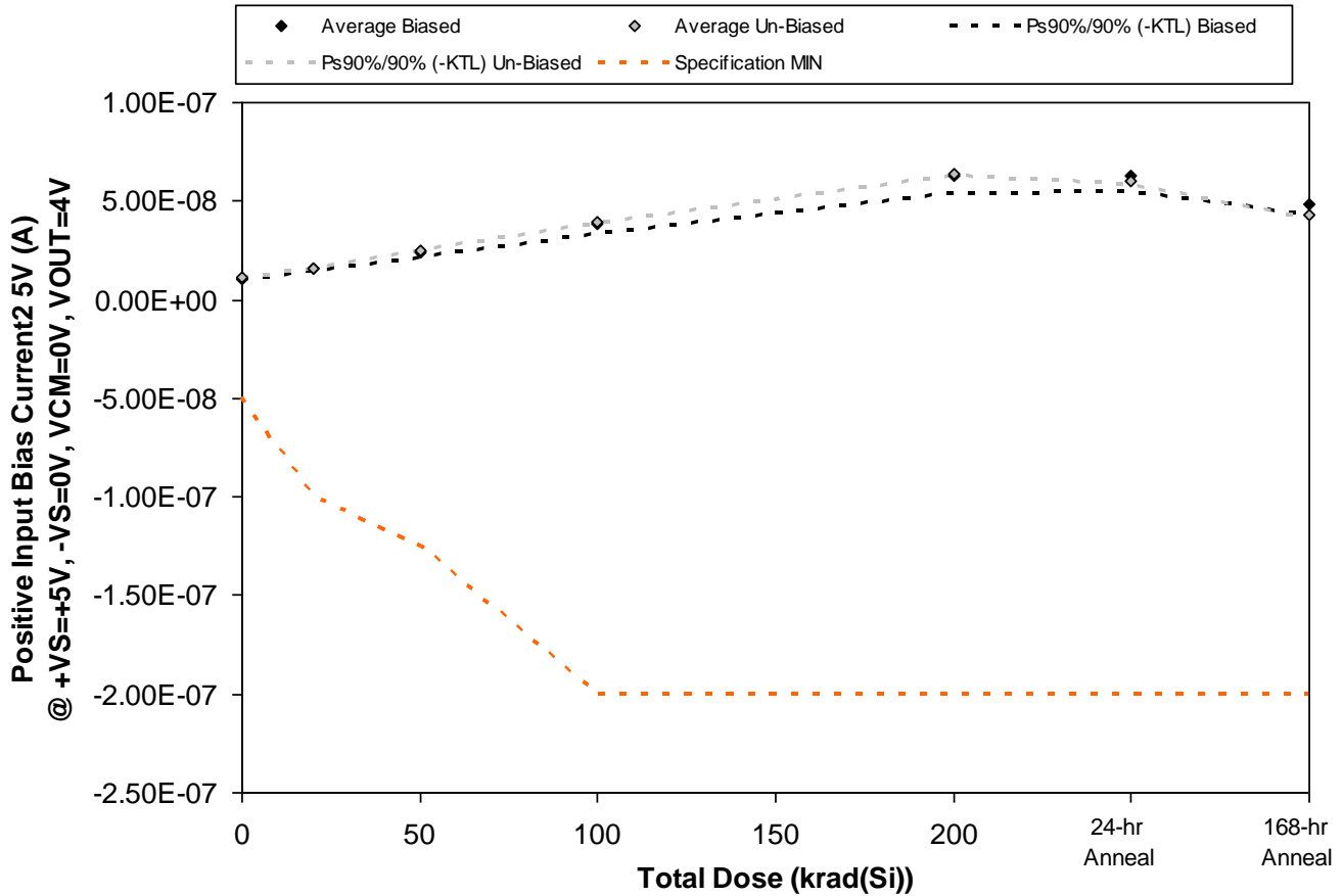
Figure 5.32. Plot of Positive Input Bias Current 2.5V (A) @ +VS=+5V, -VS=0V, VCM=0V, VOUT=4V versus total dose. The solid diamonds are the average of the measured data points for the samples irradiated under electrical bias while the shaded diamonds are the average of the measured data points for the samples irradiated with all pins tied to ground. The black lines (solid and/or dashed) are the upper and/or lower confidence limits, as determined by KTL statistics, on the samples irradiated under electrical bias while the gray lines (solid and/or dashed) are the upper and/or lower confidence limits, as determined by KTL statistics, on the samples irradiated in the unbiased condition. The red dotted line(s) are the pre- and/or post-irradiation minimum and/or maximum specification value as defined in the datasheet and/or test plan.
