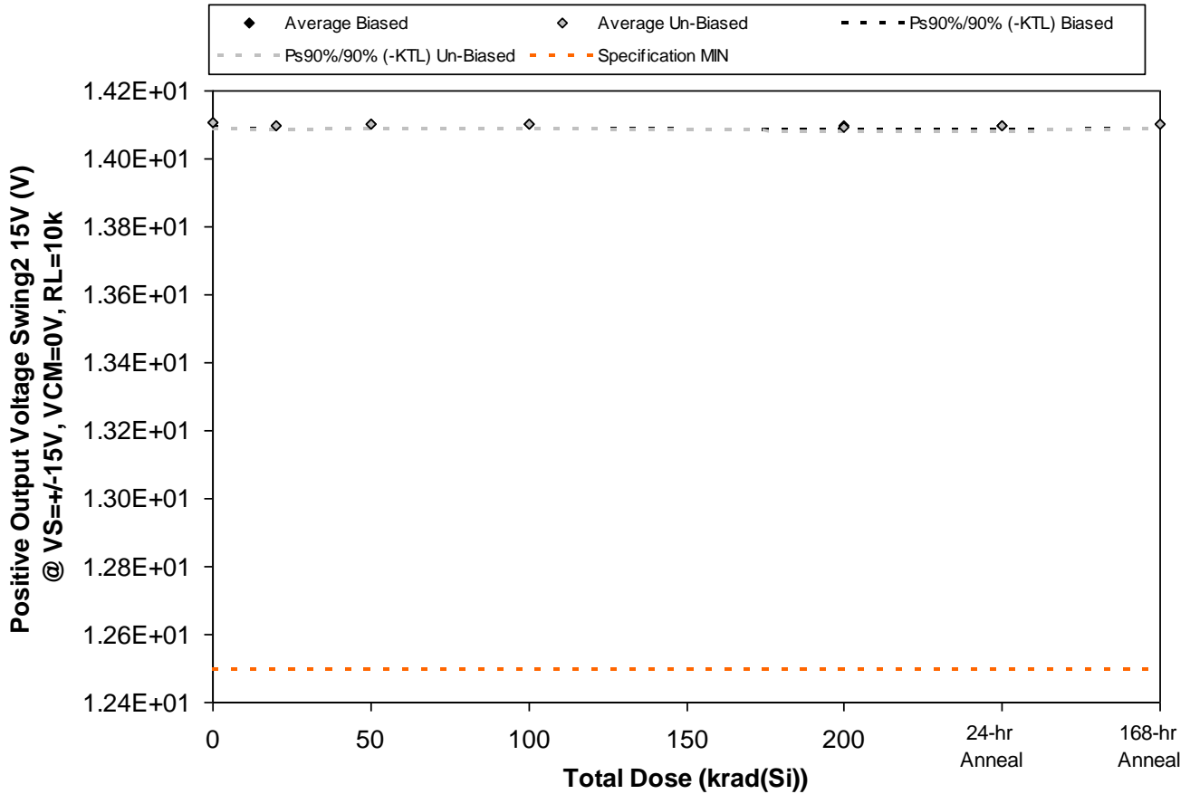
Figure 5.18. Plot of Positive Output Voltage Swing2 15V (V) @ VS= \pm 15V, VCM=0V, RL=10k versus total dose. The solid diamonds are the average of the measured data points for the samples irradiated under electrical bias while the shaded diamonds are the average of the measured data points for the samples irradiated with all pins tied to ground. The black lines (solid and/or dashed) are the upper and/or lower confidence limits, as determined by KTL statistics, on the samples irradiated under electrical bias while the gray lines (solid and/or dashed) are the upper and/or lower confidence limits, as determined by KTL statistics, on the samples irradiated in the unbiased condition. The red dotted line(s) are the pre- and/or post-irradiation minimum and/or maximum specification value as defined in the datasheet and/or test plan.
