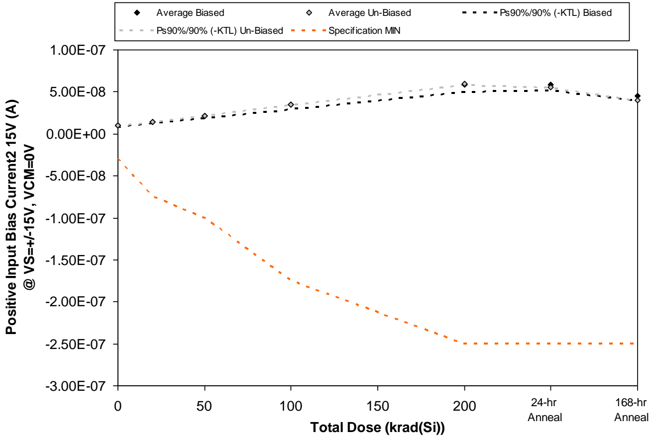
Figure 5.8. Plot of Positive Input Bias Current2 15V (A) @ VS=+-15V, VCM=0V versus total dose. The solid diamonds are the average of the measured data points for the samples irradiated under electrical bias while the shaded diamonds are the average of the measured data points for the samples irradiated with all pins tied to ground. The black lines (solid and/or dashed) are the upper and/or lower confidence limits, as determined by KTL statistics, on the samples irradiated under electrical bias while the gray lines (solid and/or dashed) are the upper and/or lower confidence limits, as determined by KTL statistics, on the samples irradiated in the unbiased condition. The red dotted line(s) are the pre- and/or post-irradiation minimum and/or maximum specification value as defined in the datasheet and/or test plan.
