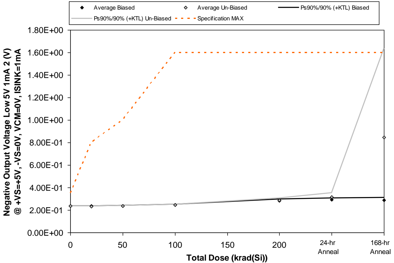
Figure 5.44. Plot of Negative Output Voltage Low 5V 1mA 2 (V) @ +VS=+5V, -VS=0V, VCM=0V, ISINK=1mA versus total dose. The solid diamonds are the average of the measured data points for the samples irradiated under electrical bias while the shaded diamonds are the average of the measured data points for the samples irradiated with all pins tied to ground. The black lines (solid and/or dashed) are the upper and/or lower confidence limits, as determined by KTL statistics, on the samples irradiated under electrical bias while the gray lines (solid and/or dashed) are the upper and/or lower confidence limits, as determined by KTL statistics, on the samples irradiated in the unbiased condition. The red dotted line(s) are the pre- and/or post-irradiation minimum and/or maximum specification value as defined in the datasheet and/or test plan.
