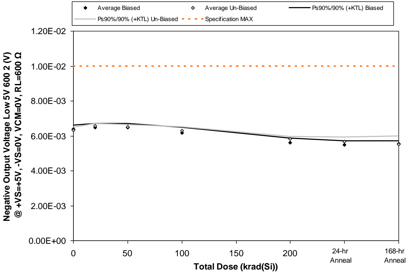
Figure 5.42. Plot of Negative Output Voltage Low 5V 600 2 (V) @ +VS=+5V, -VS=0V, VCM=0V, RL=600Ω versus total dose. The solid diamonds are the average of the measured data points for the samples irradiated under electrical bias while the shaded diamonds are the average of the measured data points for the samples irradiated with all pins tied to ground. The black lines (solid and/or dashed) are the upper and/or lower confidence limits, as determined by KTL statistics, on the samples irradiated under electrical bias while the gray lines (solid and/or dashed) are the upper and/or lower confidence limits, as determined by KTL statistics, on the samples irradiated in the unbiased condition. The red dotted line(s) are the pre- and/or post-irradiation minimum and/or maximum specification value as defined in the datasheet and/or test plan.
