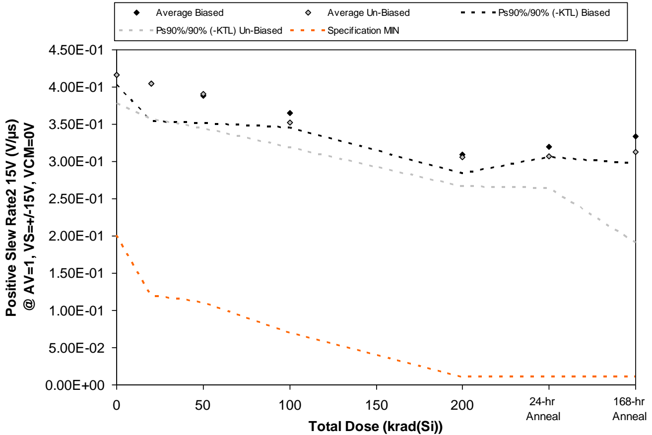
Figure 5.22. Plot of Positive Slew Rate2 15V (V/μs) @ AV=1, VS=+/-15V, VCM=0V versus total dose. The solid diamonds are the average of the measured data points for the samples irradiated under electrical bias while the shaded diamonds are the average of the measured data points for the samples irradiated with all pins tied to ground. The black lines (solid and/or dashed) are the upper and/or lower confidence limits, as determined by KTL statistics, on the samples irradiated under electrical bias while the gray lines (solid and/or dashed) are the upper and/or lower confidence limits, as determined by KTL statistics, on the samples irradiated in the unbiased condition. The red dotted line(s) are the pre- and/or post-irradiation minimum and/or maximum specification value as defined in the datasheet and/or test plan.
