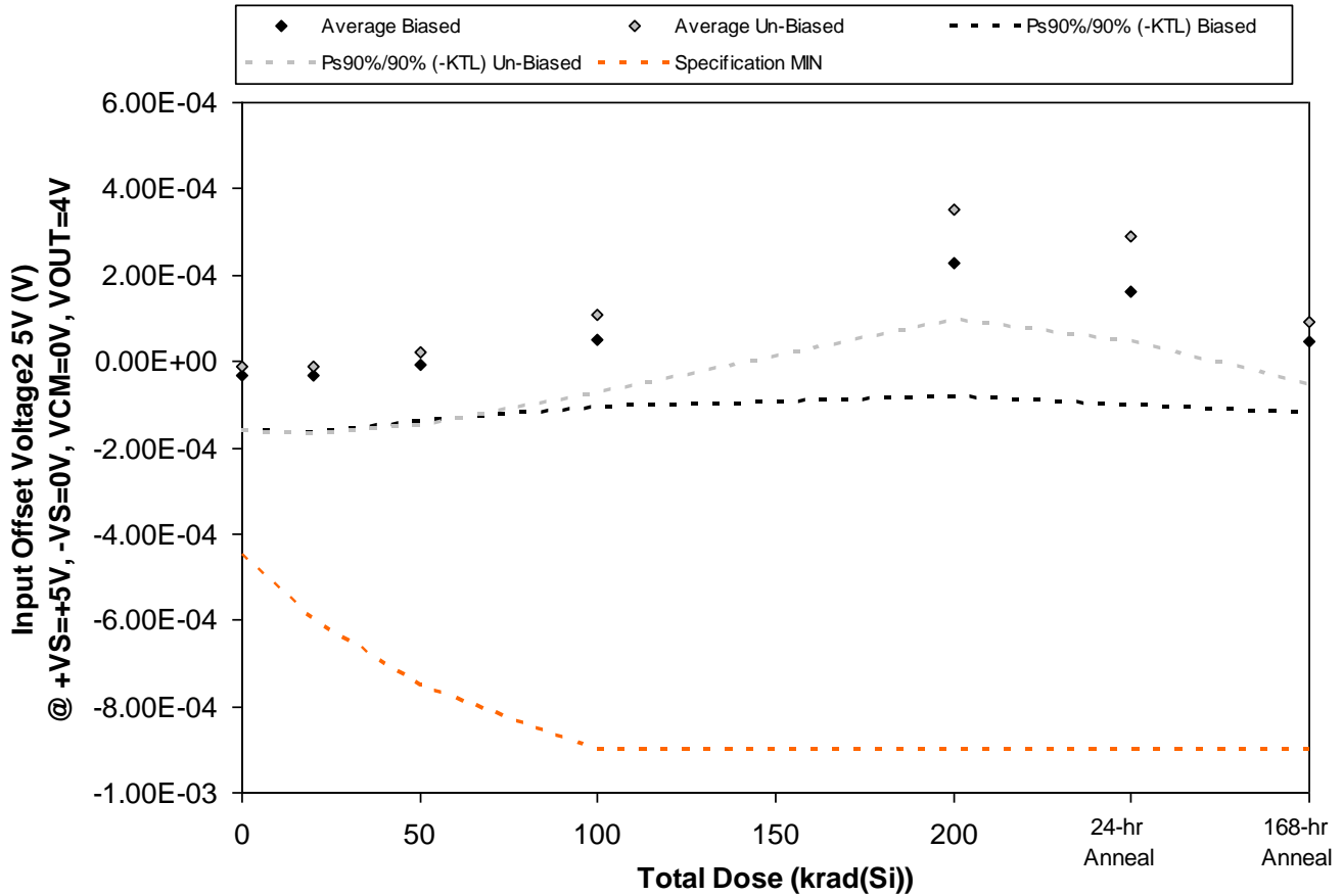
Figure 5.28. Plot of Input Offset Voltage2 5V (V) @ +VS=+5V, -VS=0V, VCM=0V, VOUT=4V versus total dose. The solid diamonds are the average of the measured data points for the samples irradiated under electrical bias while the shaded diamonds are the average of the measured data points for the samples irradiated with all pins tied to ground. The black lines (solid and/or dashed) are the upper and/or lower confidence limits, as determined by KTL statistics, on the samples irradiated under electrical bias while the gray lines (solid and/or dashed) are the upper and/or lower confidence limits, as determined by KTL statistics, on the samples irradiated in the unbiased condition. The red dotted line(s) are the pre- and/or post-irradiation minimum and/or maximum specification value as defined in the datasheet and/or test plan.
