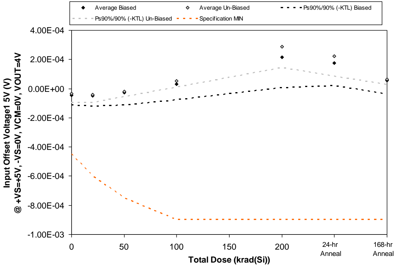
Figure 5.27. Plot of Input Offset Voltage1 5V (V) @ +VS=+5V, -VS=0V, VCM=0V, VOUT=4V versus total dose. The solid diamonds are the average of the measured data points for the samples irradiated under electrical bias while the shaded diamonds are the average of the measured data points for the samples irradiated with all pins tied to ground. The black lines (solid and/or dashed) are the upper and/or lower confidence limits, as determined by KTL statistics, on the samples irradiated under electrical bias while the gray lines (solid and/or dashed) are the upper and/or lower confidence limits, as determined by KTL statistics, on the samples irradiated in the unbiased condition. The red dotted line(s) are the pre- and/or post-irradiation minimum and/or maximum specification value as defined in the datasheet and/or test plan.
