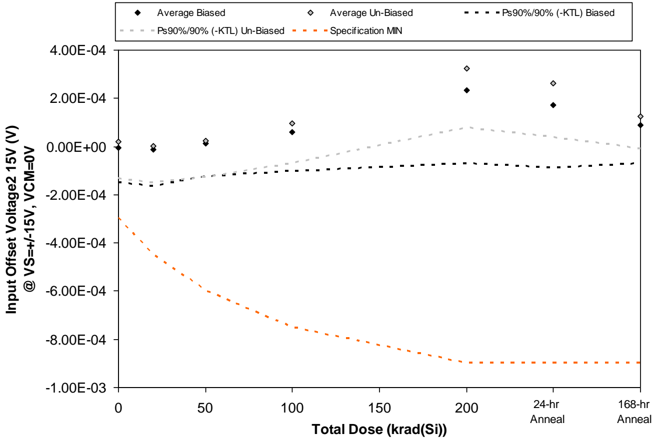
Figure 5.4. Plot of Input Offset Voltage2 15V (V) @ VS=+-15V, VCM=0V versus total dose. The solid diamonds are the average of the measured data points for the samples irradiated under electrical bias while the shaded diamonds are the average of the measured data points for the samples irradiated with all pins tied to ground. The black lines (solid and/or dashed) are the upper and/or lower confidence limits, as determined by KTL statistics, on the samples irradiated under electrical bias while the gray lines (solid and/or dashed) are the upper and/or lower confidence limits, as determined by KTL statistics, on the samples irradiated in the unbiased condition. The red dotted line(s) are the pre- and/or post-irradiation minimum and/or maximum specification value as defined in the datasheet and/or test plan.
