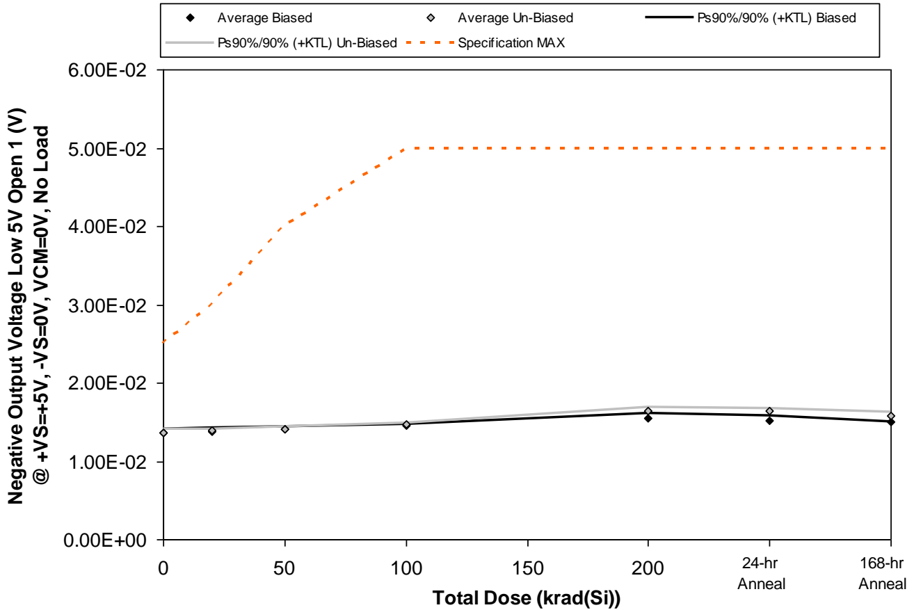
Figure 5.39. Plot of Negative Output Voltage Low 5V Open 1 (V) @ +VS=+5V, -VS=0V, VCM=0V, No Load versus total dose. The solid diamonds are the average of the measured data points for the samples irradiated under electrical bias while the shaded diamonds are the average of the measured data points for the samples irradiated with all pins tied to ground. The black lines (solid and/or dashed) are the upper and/or lower confidence limits, as determined by KTL statistics, on the samples irradiated under electrical bias while the gray lines (solid and/or dashed) are the upper and/or lower confidence limits, as determined by KTL statistics, on the samples irradiated in the unbiased condition. The red dotted line(s) are the pre- and/or post-irradiation minimum and/or maximum specification value as defined in the datasheet and/or test plan.
