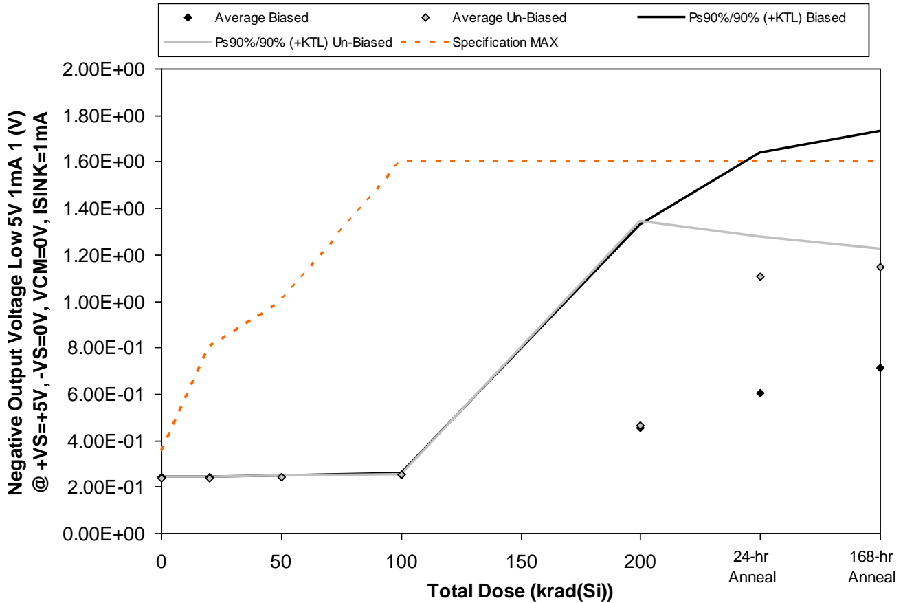
Figure 5.43. Plot of Negative Output Voltage Low 5V 1mA 1 (V) @ +VS=+5V, -VS=0V, VCM=0V, ISINK=1mA versus total dose. The solid diamonds are the average of the measured data points for the samples irradiated under electrical bias while the shaded diamonds are the average of the measured data points for the samples irradiated with all pins tied to ground. The black lines (solid and/or dashed) are the upper and/or lower confidence limits, as determined by KTL statistics, on the samples irradiated under electrical bias while the gray lines (solid and/or dashed) are the upper and/or lower confidence limits, as determined by KTL statistics, on the samples irradiated in the unbiased condition. The red dotted line(s) are the pre- and/or post-irradiation minimum and/or maximum specification value as defined in the datasheet and/or test plan.
