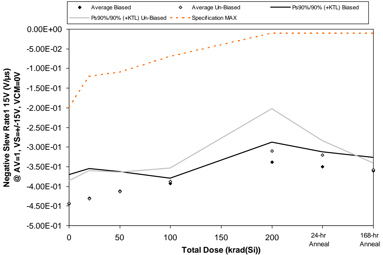
Figure 5.23. Plot of Negative Slew Rate 15V (V/μs) @ AV=1, VS=+-15V, VCM=0V versus total dose. The solid diamonds are the average of the measured data points for the samples irradiated under electrical bias while the shaded diamonds are the average of the measured data points for the samples irradiated with all pins tied to ground. The black lines (solid and/or dashed) are the upper and/or lower confidence limits, as determined by KTL statistics, on the samples irradiated under electrical bias while the gray lines (solid and/or dashed) are the upper and/or lower confidence limits, as determined by KTL statistics, on the samples irradiated in the unbiased condition. The red dotted line(s) are the pre- and/or post-irradiation minimum and/or maximum specification value as defined in the datasheet and/or test plan.
