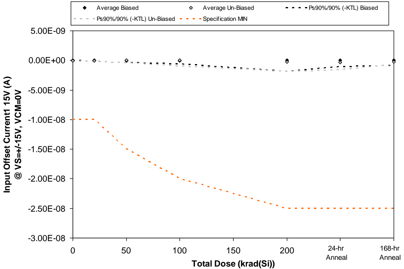
Figure 5.5. Plot of Input Offset Current1 15V (A) @ VS=+-15V, VCM=0V versus total dose. The solid diamonds are the average of the measured data points for the samples irradiated under electrical bias while the shaded diamonds are the average of the measured data points for the samples irradiated with all pins tied to ground. The black lines (solid and/or dashed) are the upper and/or lower confidence limits, as determined by KTL statistics, on the samples irradiated under electrical bias while the gray lines (solid and/or dashed) are the upper and/or lower confidence limits, as determined by KTL statistics, on the samples irradiated in the unbiased condition. The red dotted line(s) are the pre- and/or post-irradiation minimum and/or maximum specification value as defined in the datasheet and/or test plan.
