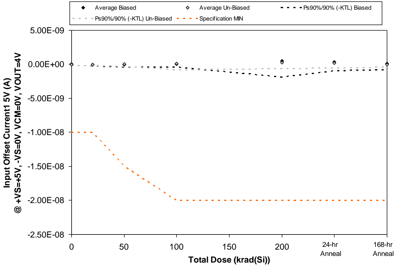
Figure 5.29. Plot of Input Offset Current1 5V (A) @ +VS=+5V, -VS=0V, VCM=0V, VOUT=4V versus total dose. The solid diamonds are the average of the measured data points for the samples irradiated under electrical bias while the shaded diamonds are the average of the measured data points for the samples irradiated with all pins tied to ground. The black lines (solid and/or dashed) are the upper and/or lower confidence limits, as determined by KTL statistics, on the samples irradiated under electrical bias while the gray lines (solid and/or dashed) are the upper and/or lower confidence limits, as determined by KTL statistics, on the samples irradiated in the unbiased condition. The red dotted line(s) are the pre- and/or post-irradiation minimum and/or maximum specification value as defined in the datasheet and/or test plan.
