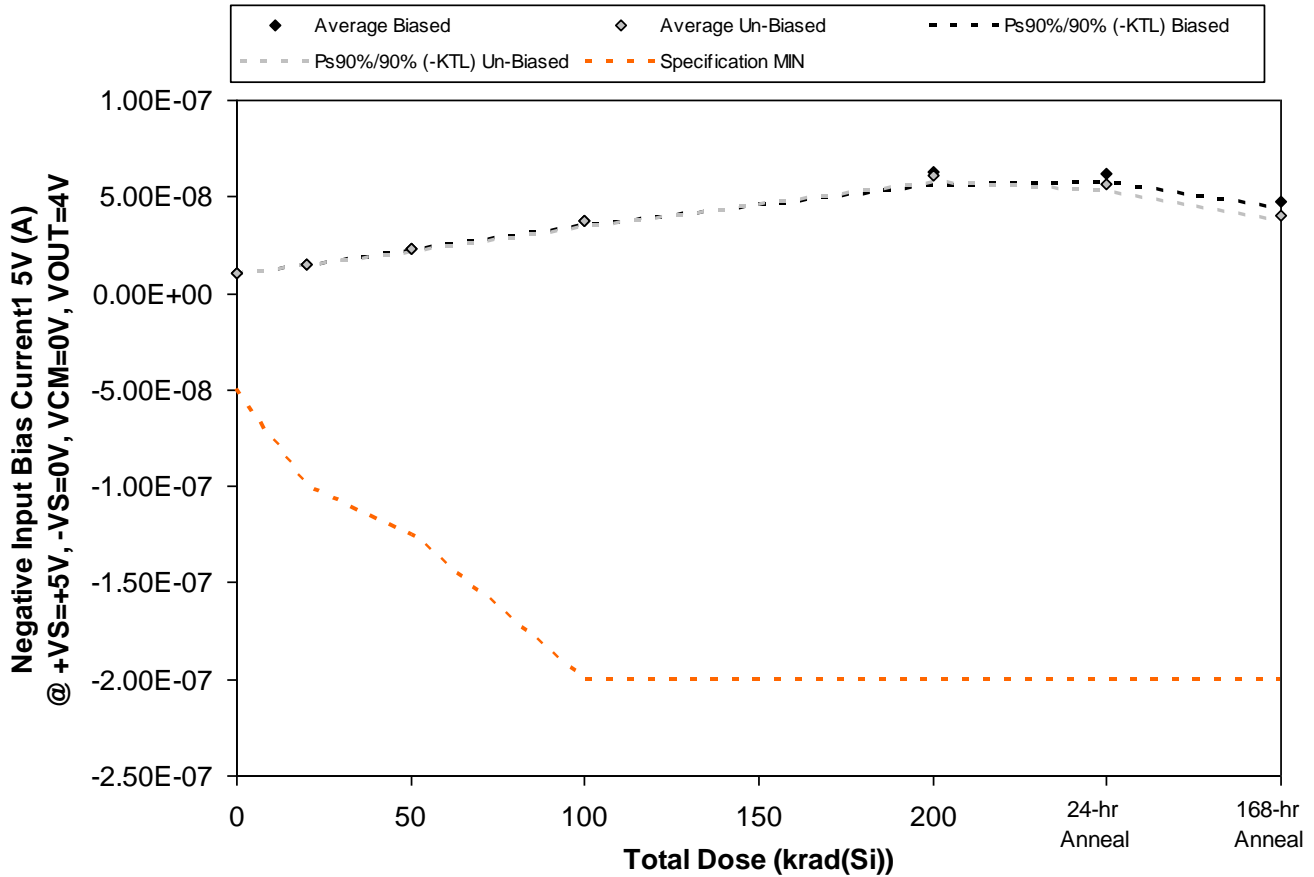
Figure 5.33. Plot of Negative Input Bias Current1 5V (A) @ +VS=+5V, -VS=0V, VCM=0V, VOUT=4V versus total dose. The solid diamonds are the average of the measured data points for the samples irradiated under electrical bias while the shaded diamonds are the average of the measured data points for the samples irradiated with all pins tied to ground. The black lines (solid and/or dashed) are the upper and/or lower confidence limits, as determined by KTL statistics, on the samples irradiated under electrical bias while the gray lines (solid and/or dashed) are the upper and/or lower confidence limits, as determined by KTL statistics, on the samples irradiated in the unbiased condition. The red dotted line(s) are the pre- and/or post-irradiation minimum and/or maximum specification value as defined in the datasheet and/or test plan.
