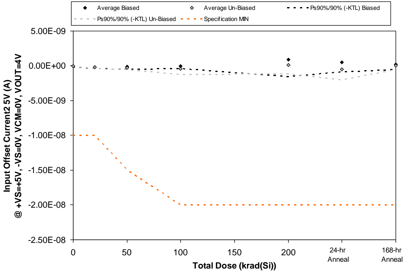
Figure 5.30. Plot of Input Offset Current2 5V (A) @ +VS=+5V, -VS=0V, VCM=0V, VOUT=4V versus total dose. The solid diamonds are the average of the measured data points for the samples irradiated under electrical bias while the shaded diamonds are the average of the measured data points for the samples irradiated with all pins tied to ground. The black lines (solid and/or dashed) are the upper and/or lower confidence limits, as determined by KTL statistics, on the samples irradiated under electrical bias while the gray lines (solid and/or dashed) are the upper and/or lower confidence limits, as determined by KTL statistics, on the samples irradiated in the unbiased condition. The red dotted line(s) are the pre- and/or post-irradiation minimum and/or maximum specification value as defined in the datasheet and/or test plan.
