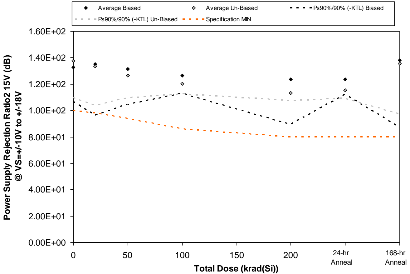
Figure 5.14. Plot of Power Supply Rejection Ratio 15V (dB) @ VS=+-10V to +/-18V versus total dose. The solid diamonds are the average of the measured data points for the samples irradiated under electrical bias while the shaded diamonds are the average of the measured data points for the samples irradiated with all pins tied to ground. The black lines (solid and/or dashed) are the upper and/or lower confidence limits, as determined by KTL statistics, on the samples irradiated under electrical bias while the gray lines (solid and/or dashed) are the upper and/or lower confidence limits, as determined by KTL statistics, on the samples irradiated in the unbiased condition. The red dotted line(s) are the pre- and/or post-irradiation minimum and/or maximum specification value as defined in the datasheet and/or test plan.
