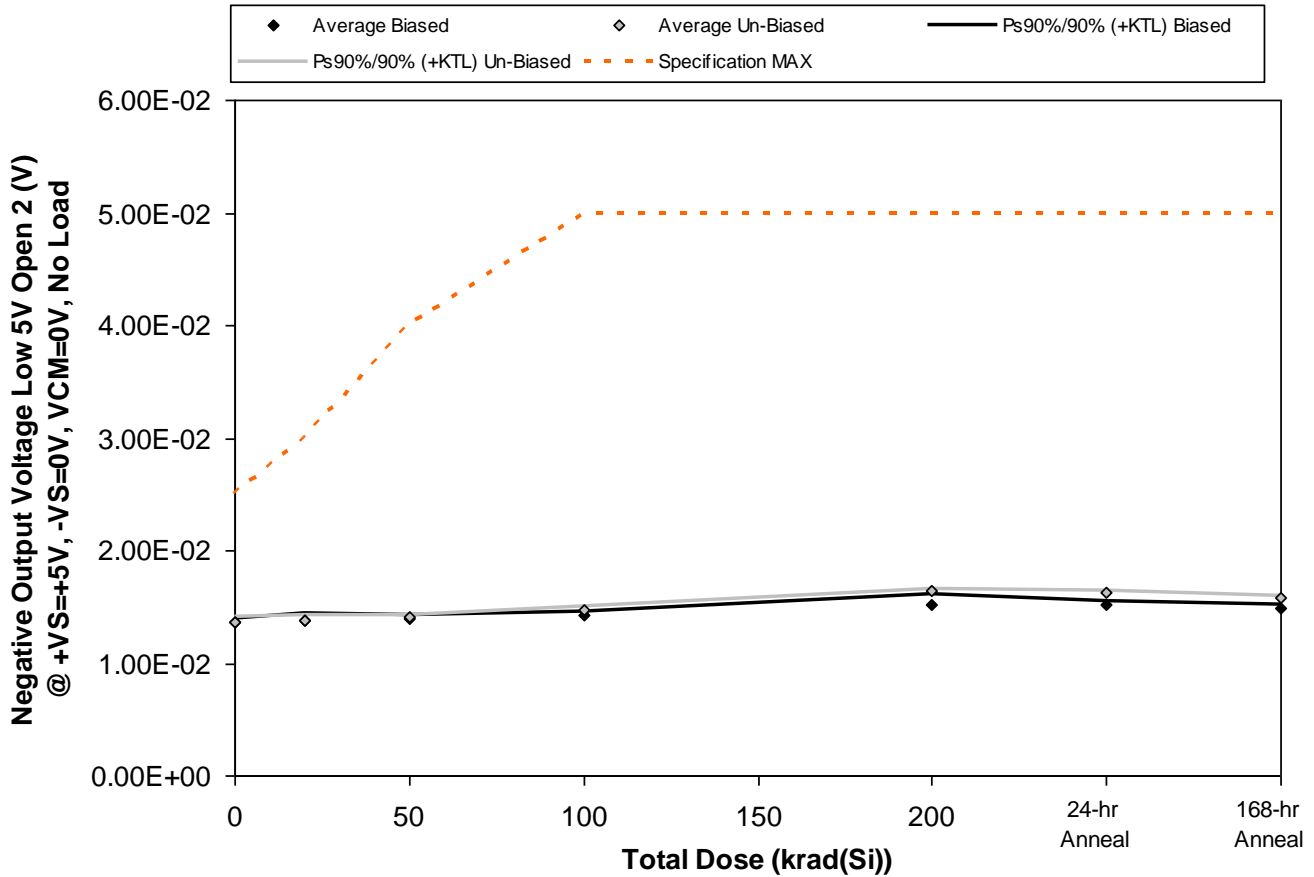
Figure 5.40. Plot of Negative Output Voltage Low 5V Open 2 (V) @ +VS=+5V, -VS=0V, VCM=0V, No Load versus total dose. The solid diamonds are the average of the measured data points for the samples irradiated under electrical bias while the shaded diamonds are the average of the measured data points for the samples irradiated with all pins tied to ground. The black lines (solid and/or dashed) are the upper and/or lower confidence limits, as determined by KTL statistics, on the samples irradiated under electrical bias while the gray lines (solid and/or dashed) are the upper and/or lower confidence limits, as determined by KTL statistics, on the samples irradiated in the unbiased condition. The red dotted line(s) are the pre- and/or post-irradiation minimum and/or maximum specification value as defined in the datasheet and/or test plan.
