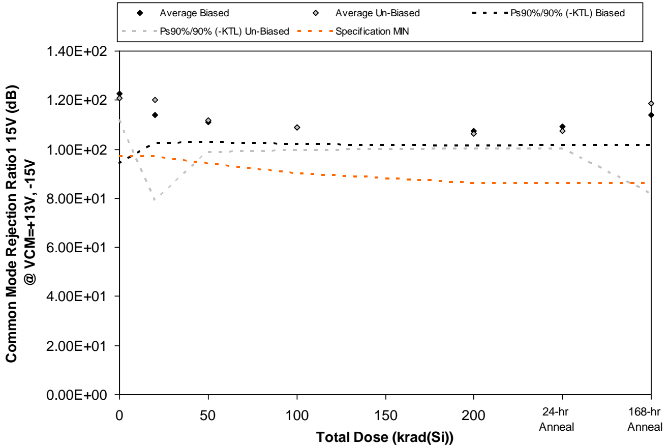
Figure 5.11. Plot of Common Mode Rejection Ratio 15V (dB) @ VCM=+13V, -15V versus total dose. The solid diamonds are the average of the measured data points for the samples irradiated under electrical bias while the shaded diamonds are the average of the measured data points for the samples irradiated with all pins tied to ground. The black lines (solid and/or dashed) are the upper and/or lower confidence limits, as determined by KTL statistics, on the samples irradiated under electrical bias while the gray lines (solid and/or dashed) are the upper and/or lower confidence limits, as determined by KTL statistics, on the samples irradiated in the unbiased condition. The red dotted line(s) are the pre- and/or post-irradiation minimum and/or maximum specification value as defined in the datasheet and/or test plan.
