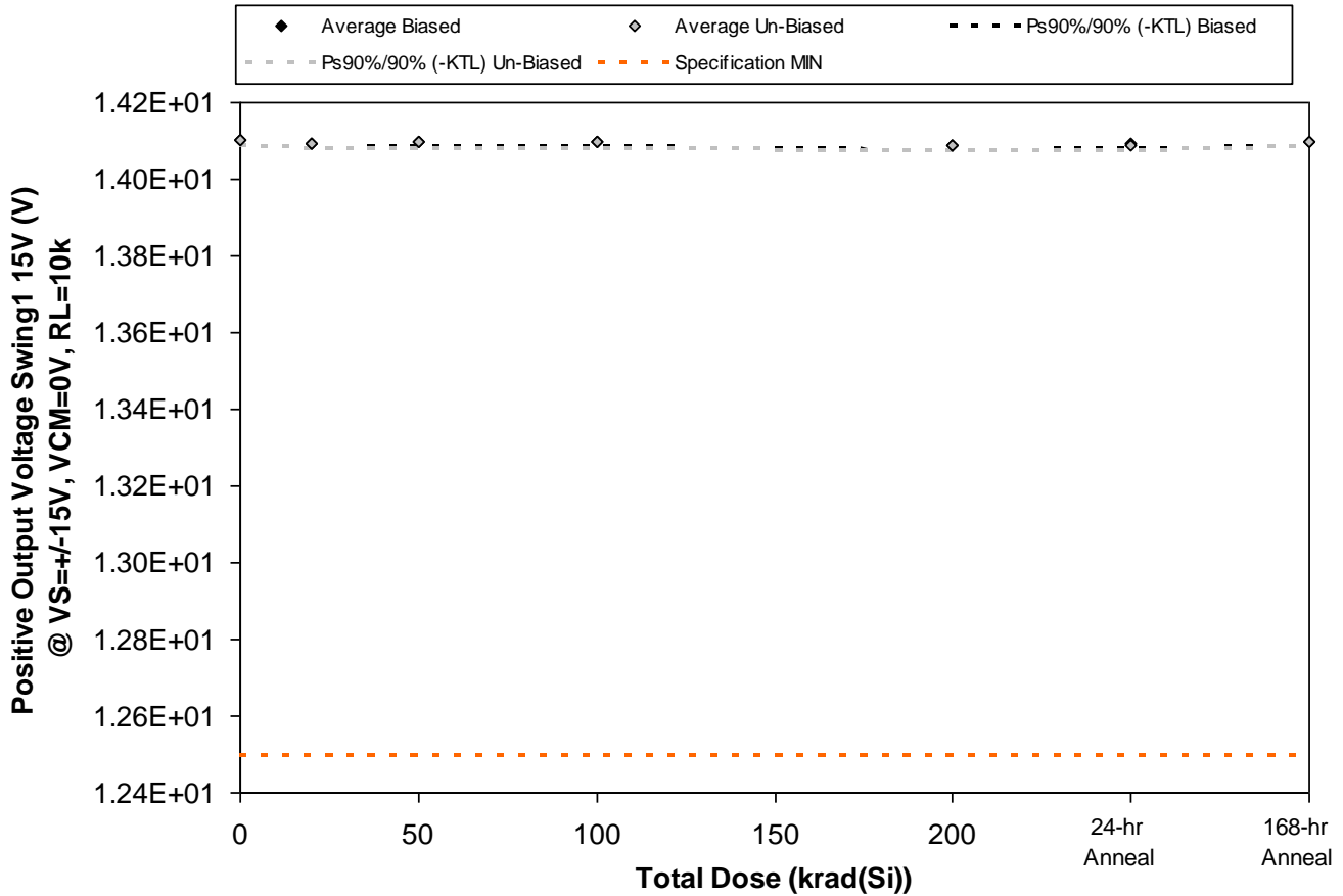
Figure 5.17. Plot of Positive Output Voltage Swing1 15V (V) @ VS= \pm 15V, VCM=0V, RL=10k versus total dose. The solid diamonds are the average of the measured data points for the samples irradiated under electrical bias while the shaded diamonds are the average of the measured data points for the samples irradiated with all pins tied to ground. The black lines (solid and/or dashed) are the upper and/or lower confidence limits, as determined by KTL statistics, on the samples irradiated under electrical bias while the gray lines (solid and/or dashed) are the upper and/or lower confidence limits, as determined by KTL statistics, on the samples irradiated in the unbiased condition. The red dotted line(s) are the pre- and/or post-irradiation minimum and/or maximum specification value as defined in the datasheet and/or test plan.
