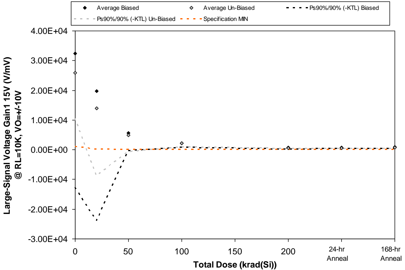
Figure 5.15. Plot of Large-Signal Voltage Gain1 15V (V/mV) @ RL=10K, VO=+-10V versus total dose. The solid diamonds are the average of the measured data points for the samples irradiated under electrical bias while the shaded diamonds are the average of the measured data points for the samples irradiated with all pins tied to ground. The black lines (solid and/or dashed) are the upper and/or lower confidence limits, as determined by KTL statistics, on the samples irradiated under electrical bias while the gray lines (solid and/or dashed) are the upper and/or lower confidence limits, as determined by KTL statistics, on the samples irradiated in the unbiased condition. The red dotted line(s) are the pre- and/or post-irradiation minimum and/or maximum specification value as defined in the datasheet and/or test plan.
