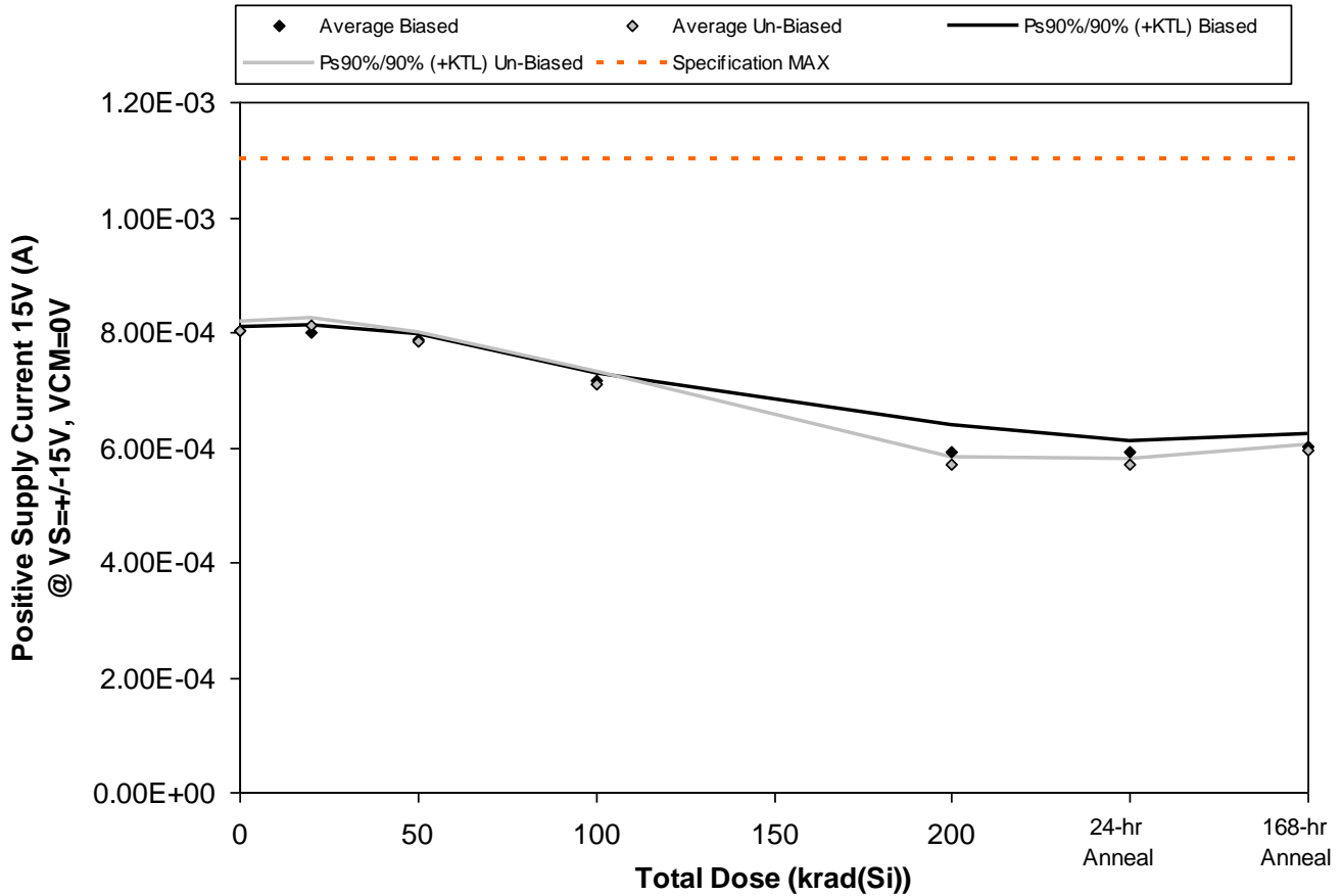
Figure 5.1. Plot of Positive Supply Current 15V (A) @ VS= \pm 15V, VCM=0V versus total dose. The solid diamonds are the average of the measured data points for the samples irradiated under electrical bias while the shaded diamonds are the average of the measured data points for the samples irradiated with all pins tied to ground. The black lines (solid and/or dashed) are the upper and/or lower confidence limits, as determined by KTL statistics, on the samples irradiated under electrical bias while the gray lines (solid and/or dashed) are the upper and/or lower confidence limits, as determined by KTL statistics, on the samples irradiated in the unbiased condition. The red dotted line(s) are the pre- and/or post-irradiation minimum and/or maximum specification value as defined in the datasheet and/or test plan.
