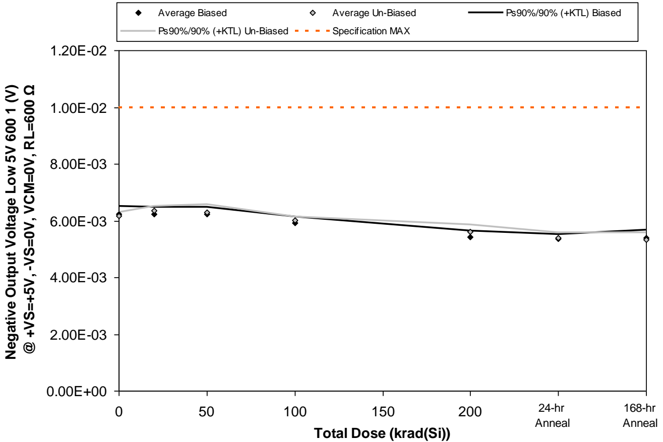
Figure 5.41. Plot of Negative Output Voltage Low 5V 600 1 (V) @ +VS=+5V, -VS=0V, VCM=0V, RL=600Ω versus total dose. The solid diamonds are the average of the measured data points for the samples irradiated under electrical bias while the shaded diamonds are the average of the measured data points for the samples irradiated with all pins tied to ground. The black lines (solid and/or dashed) are the upper and/or lower confidence limits, as determined by KTL statistics, on the samples irradiated under electrical bias while the gray lines (solid and/or dashed) are the upper and/or lower confidence limits, as determined by KTL statistics, on the samples irradiated in the unbiased condition. The red dotted line(s) are the pre- and/or post-irradiation minimum and/or maximum specification value as defined in the datasheet and/or test plan.
