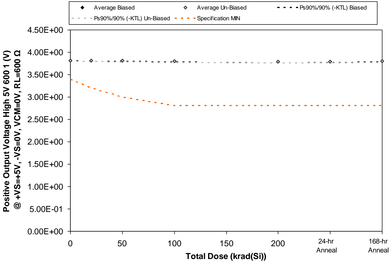
Figure 5.37. Plot of Positive Output Voltage High 5V 600 1 (V) @ +VS=+5V, -VS=0V, VCM=0V, RL=600Ω versus total dose. The solid diamonds are the average of the measured data points for the samples irradiated under electrical bias while the shaded diamonds are the average of the measured data points for the samples irradiated with all pins tied to ground. The black lines (solid and/or dashed) are the upper and/or lower confidence limits, as determined by KTL statistics, on the samples irradiated under electrical bias while the gray lines (solid and/or dashed) are the upper and/or lower confidence limits, as determined by KTL statistics, on the samples irradiated in the unbiased condition. The red dotted line(s) are the pre- and/or post-irradiation minimum and/or maximum specification value as defined in the datasheet and/or test plan.
