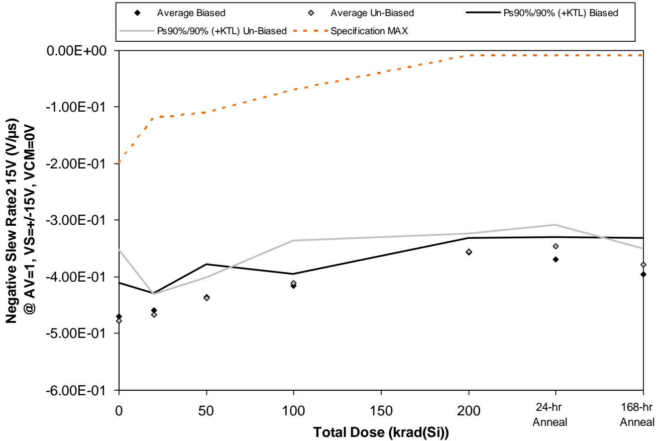
Figure 5.24. Plot of Negative Slew Rate2 15V (V/μs) @ AV=1, VS=+/-15V, VCM=0V versus total dose. The solid diamonds are the average of the measured data points for the samples irradiated under electrical bias while the shaded diamonds are the average of the measured data points for the samples irradiated with all pins tied to ground. The black lines (solid and/or dashed) are the upper and/or lower confidence limits, as determined by KTL statistics, on the samples irradiated under electrical bias while the gray lines (solid and/or dashed) are the upper and/or lower confidence limits, as determined by KTL statistics, on the samples irradiated in the unbiased condition. The red dotted line(s) are the pre- and/or post-irradiation minimum and/or maximum specification value as defined in the datasheet and/or test plan.
