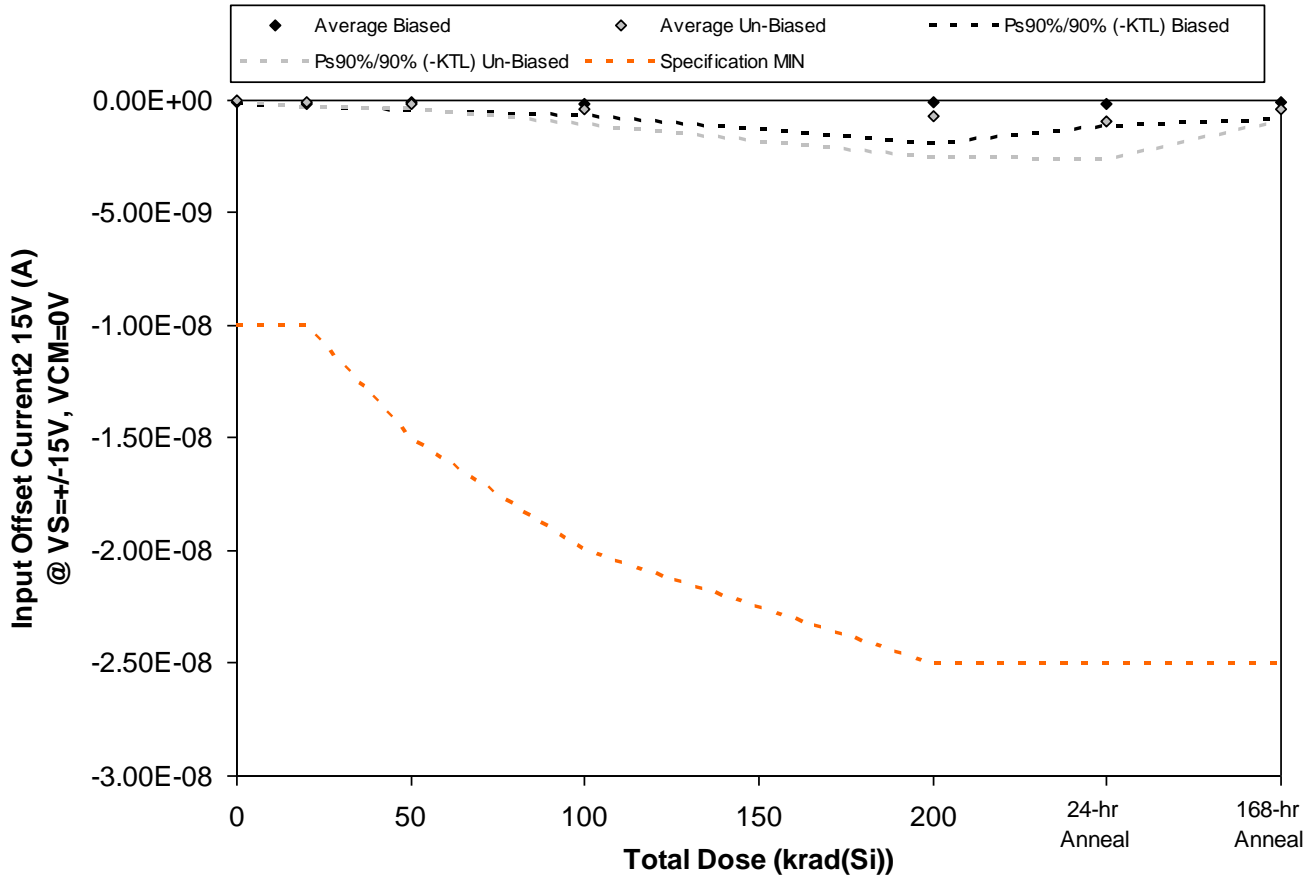
Figure 5.6. Plot of Input Offset Current2 15V (A) @ VS=+-15V, VCM=0V versus total dose. The solid diamonds are the average of the measured data points for the samples irradiated under electrical bias while the shaded diamonds are the average of the measured data points for the samples irradiated with all pins tied to ground. The black lines (solid and/or dashed) are the upper and/or lower confidence limits, as determined by KTL statistics, on the samples irradiated under electrical bias while the gray lines (solid and/or dashed) are the upper and/or lower confidence limits, as determined by KTL statistics, on the samples irradiated in the unbiased condition. The red dotted line(s) are the pre- and/or post-irradiation minimum and/or maximum specification value as defined in the datasheet and/or test plan.
