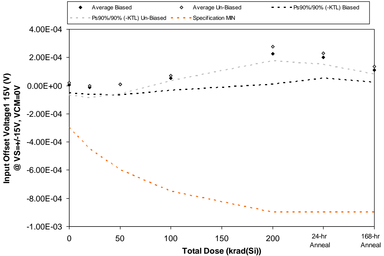
Figure 5.3. Plot of Input Offset Voltage1 15V (V) @ VS=+-15V, VCM=0V versus total dose. The solid diamonds are the average of the measured data points for the samples irradiated under electrical bias while the shaded diamonds are the average of the measured data points for the samples irradiated with all pins tied to ground. The black lines (solid and/or dashed) are the upper and/or lower confidence limits, as determined by KTL statistics, on the samples irradiated under electrical bias while the gray lines (solid and/or dashed) are the upper and/or lower confidence limits, as determined by KTL statistics, on the samples irradiated in the unbiased condition. The red dotted line(s) are the pre- and/or post-irradiation minimum and/or maximum specification value as defined in the datasheet and/or test plan.
