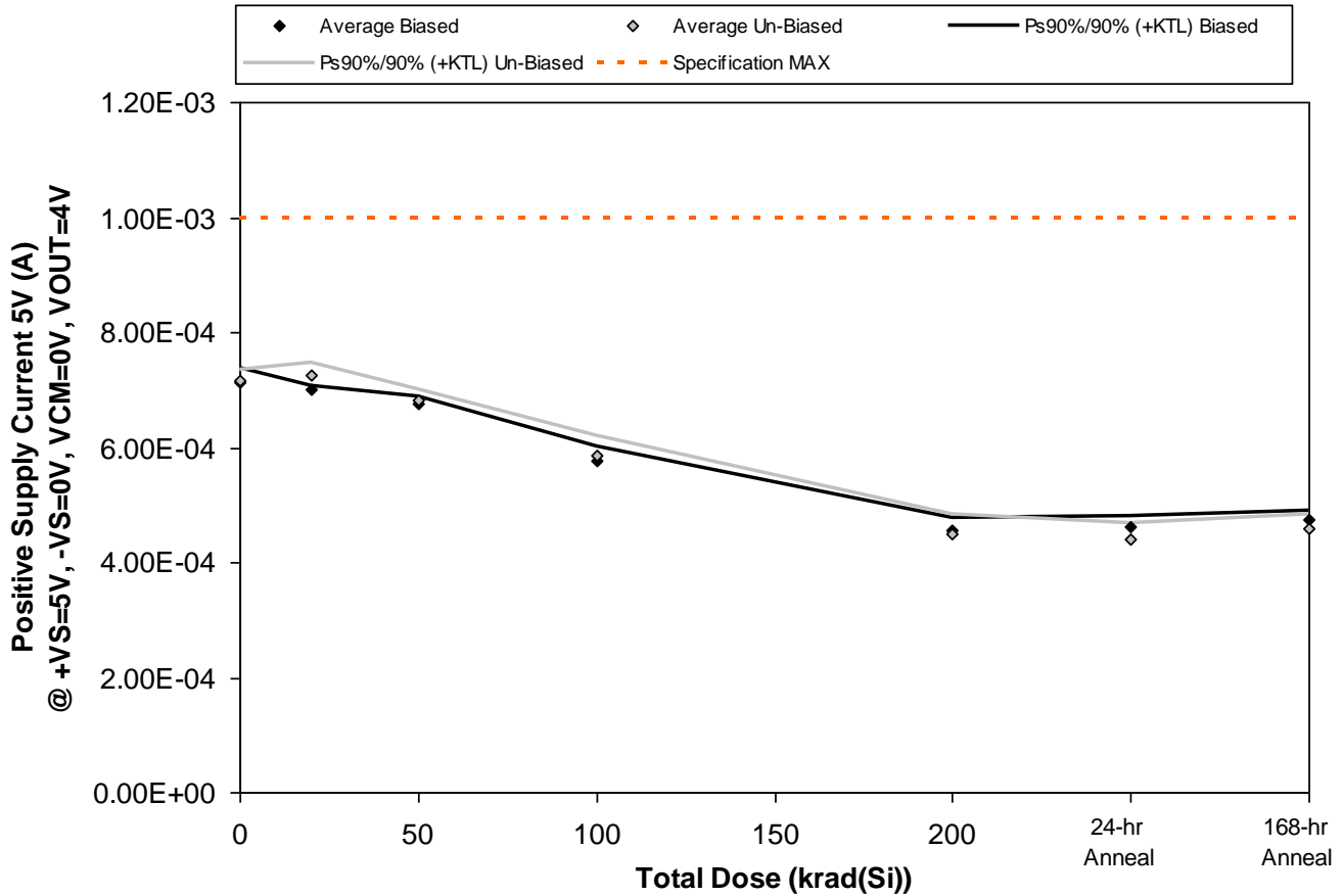
Figure 5.25. Plot of Positive Supply Current 5V (A) @ +VS=5V, -VS=0V, VCM=0V, VOUT=4V versus total dose. The solid diamonds are the average of the measured data points for the samples irradiated under electrical bias while the shaded diamonds are the average of the measured data points for the samples irradiated with all pins tied to ground. The black lines (solid and/or dashed) are the upper and/or lower confidence limits, as determined by KTL statistics, on the samples irradiated under electrical bias while the gray lines (solid and/or dashed) are the upper and/or lower confidence limits, as determined by KTL statistics, on the samples irradiated in the unbiased condition. The red dotted line(s) are the pre- and/or post-irradiation minimum and/or maximum specification value as defined in the datasheet and/or test plan.
