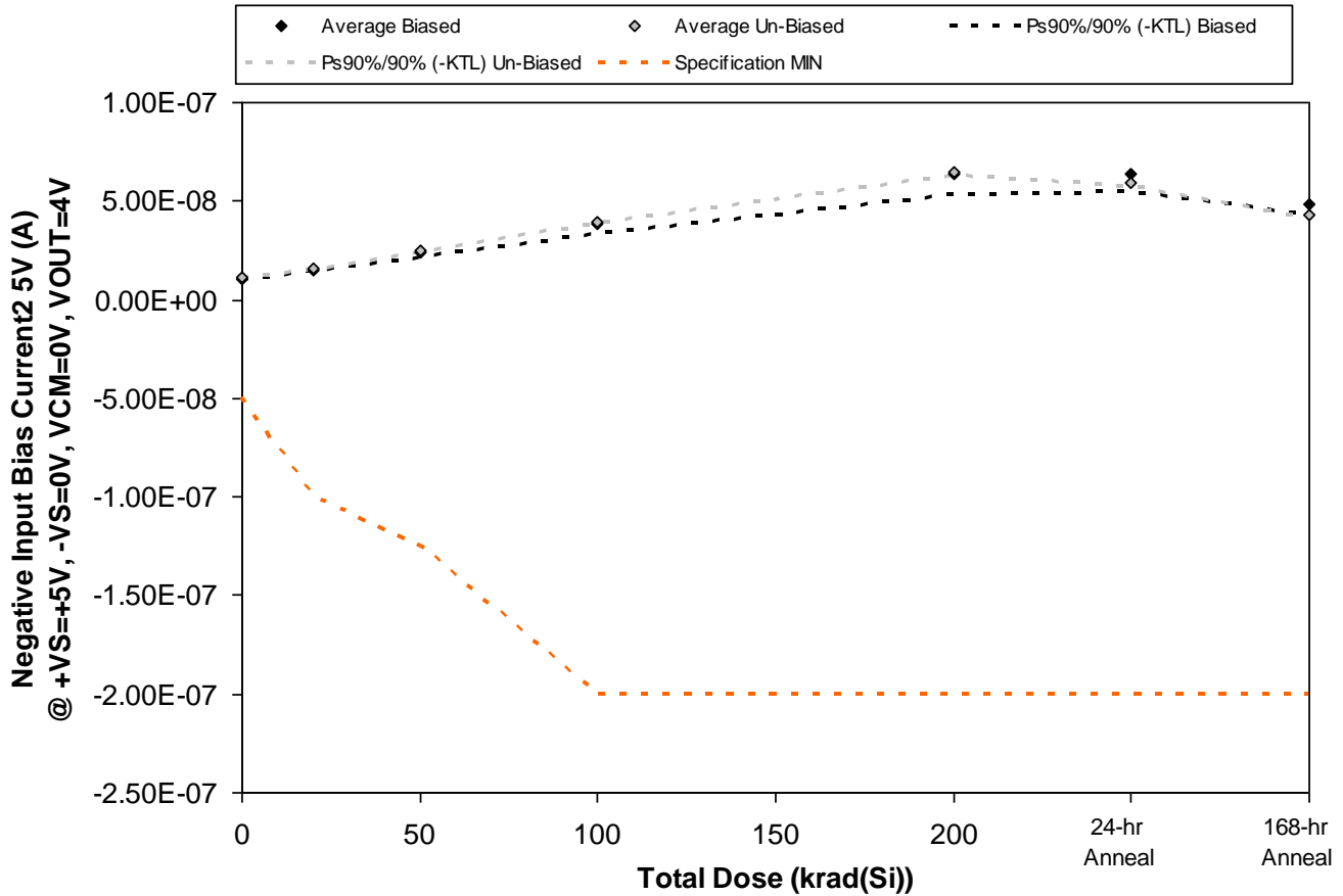
Figure 5.34. Plot of Negative Input Bias Current2 5V (A) @ +VS=+5V, -VS=0V, VCM=0V, VOUT=4V versus total dose. The solid diamonds are the average of the measured data points for the samples irradiated under electrical bias while the shaded diamonds are the average of the measured data points for the samples irradiated with all pins tied to ground. The black lines (solid and/or dashed) are the upper and/or lower confidence limits, as determined by KTL statistics, on the samples irradiated under electrical bias while the gray lines (solid and/or dashed) are the upper and/or lower confidence limits, as determined by KTL statistics, on the samples irradiated in the unbiased condition. The red dotted line(s) are the pre- and/or post-irradiation minimum and/or maximum specification value as defined in the datasheet and/or test plan.
