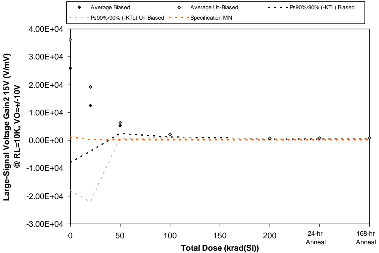
Figure 5.16. Plot of Large-Signal Voltage Gain2 15V (V/mV) @ RL=10K, VO=+-10V versus total dose. The solid diamonds are the average of the measured data points for the samples irradiated under electrical bias while the shaded diamonds are the average of the measured data points for the samples irradiated with all pins tied to ground. The black lines (solid and/or dashed) are the upper and/or lower confidence limits, as determined by KTL statistics, on the samples irradiated under electrical bias while the gray lines (solid and/or dashed) are the upper and/or lower confidence limits, as determined by KTL statistics, on the samples irradiated in the unbiased condition. The red dotted line(s) are the pre- and/or post-irradiation minimum and/or maximum specification value as defined in the datasheet and/or test plan.
