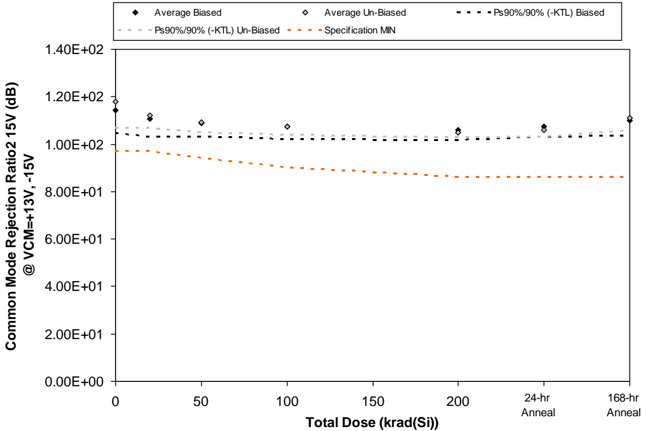
Figure 5.12. Plot of Common Mode Rejection Ratio2 15V (dB) @ VCM=+13V, -15V versus total dose. The solid diamonds are the average of the measured data points for the samples irradiated under electrical bias while the shaded diamonds are the average of the measured data points for the samples irradiated with all pins tied to ground. The black lines (solid and/or dashed) are the upper and/or lower confidence limits, as determined by KTL statistics, on the samples irradiated under electrical bias while the gray lines (solid and/or dashed) are the upper and/or lower confidence limits, as determined by KTL statistics, on the samples irradiated in the unbiased condition. The red dotted line(s) are the pre- and/or post-irradiation minimum and/or maximum specification value as defined in the datasheet and/or test plan.
