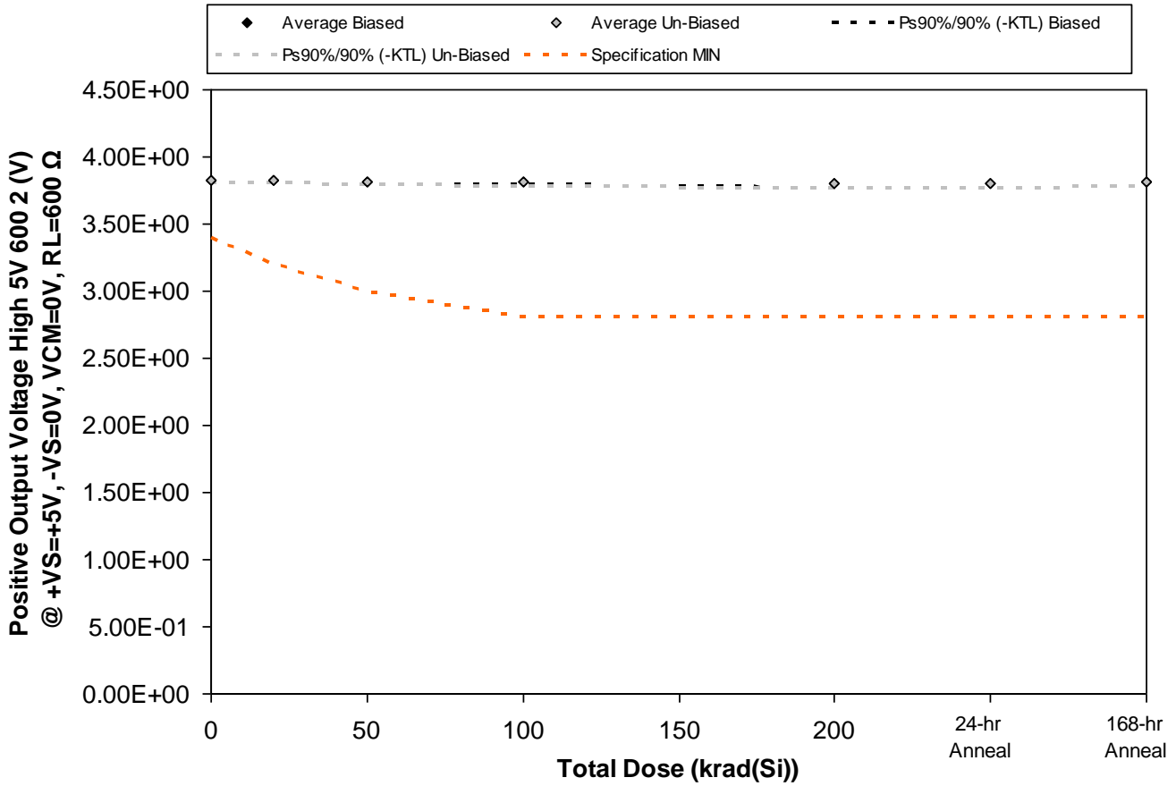
Figure 5.38. Plot of Positive Output Voltage High 5V 600 2 (V) @ +VS=+5V, -VS=0V, VCM=0V, RL=600Ω versus total dose. The solid diamonds are the average of the measured data points for the samples irradiated under electrical bias while the shaded diamonds are the average of the measured data points for the samples irradiated with all pins tied to ground. The black lines (solid and/or dashed) are the upper and/or lower confidence limits, as determined by KTL statistics, on the samples irradiated under electrical bias while the gray lines (solid and/or dashed) are the upper and/or lower confidence limits, as determined by KTL statistics, on the samples irradiated in the unbiased condition. The red dotted line(s) are the pre- and/or post-irradiation minimum and/or maximum specification value as defined in the datasheet and/or test plan.
