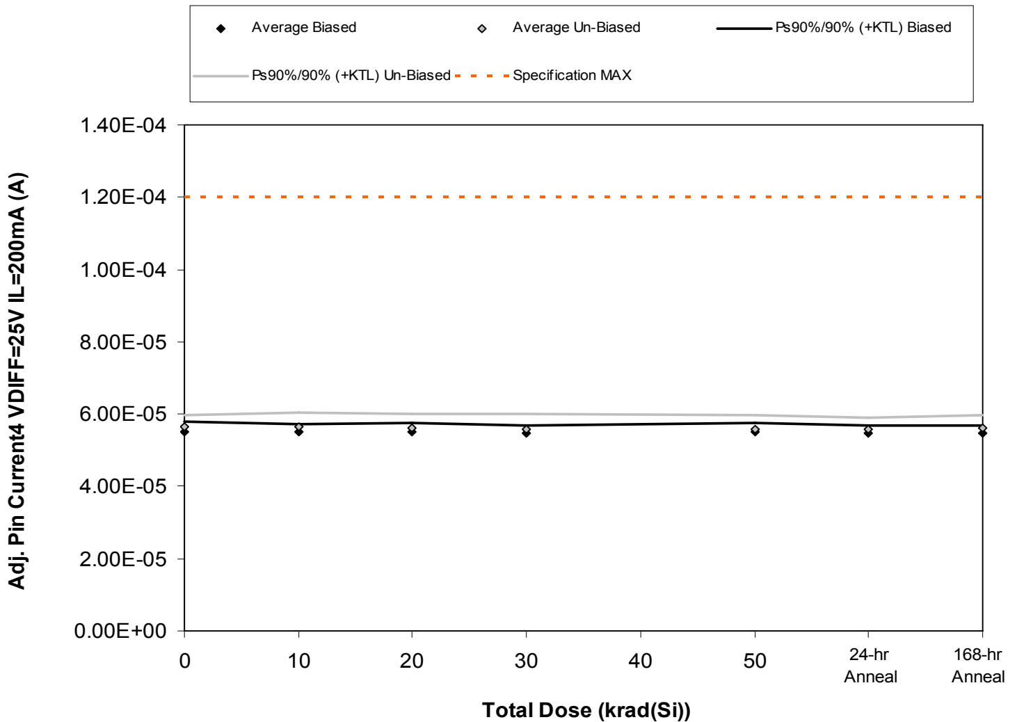
Figure 5.13. Plot of Adj. Pin Current4 VDIFF=25V IL=200mA (A) versus total dose. The solid diamonds are the average of the measured data points for the samples irradiated under electrical bias while the shaded diamonds are the average of the measured data points for the samples irradiated with all pins tied to ground. The black lines (solid and/or dashed) are the average of the data points after application of the KTL statistics on the samples irradiated under electrical bias while the gray lines (solid and/or dashed) are the average of the data points after application of the KTL statistics on the samples irradiated in the unbiased condition. The red dotted line(s) are the pre- and/or post-irradiation minimum and/or maximum specification value as defined in the datasheet and/or test plan.
