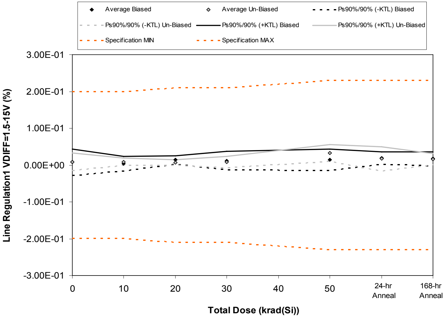
Figure 5.7. Plot of Line Regulation1 VDIFF=1.5-15V (%) versus total dose. The solid diamonds are the average of the measured data points for the samples irradiated under electrical bias while the shaded diamonds are the average of the measured data points for the samples irradiated with all pins tied to ground. The black lines (solid and/or dashed) are the average of the data points after application of the KTL statistics on the samples irradiated under electrical bias while the gray lines (solid and/or dashed) are the average of the data points after application of the KTL statistics on the samples irradiated in the unbiased condition. The red dotted line(s) are the pre- and/or post-irradiation minimum and/or maximum specification value as defined in the datasheet and/or test plan.
