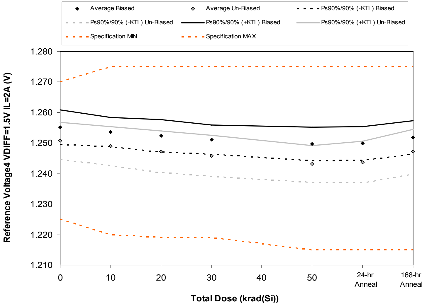
Figure 5.4. Plot of Reference Voltage4 VDIFF=1.5V IL=2A (V) versus total dose. The solid diamonds are the average of the measured data points for the samples irradiated under electrical bias while the shaded diamonds are the average of the measured data points for the samples irradiated with all pins tied to ground. The black lines (solid and/or dashed) are the average of the data points after application of the KTL statistics on the samples irradiated under electrical bias while the gray lines (solid and/or dashed) are the average of the data points after application of the KTL statistics on the samples irradiated in the unbiased condition. The red dotted line(s) are the pre- and/or post-irradiation minimum and/or maximum specification value as defined in the datasheet and/or test plan.
