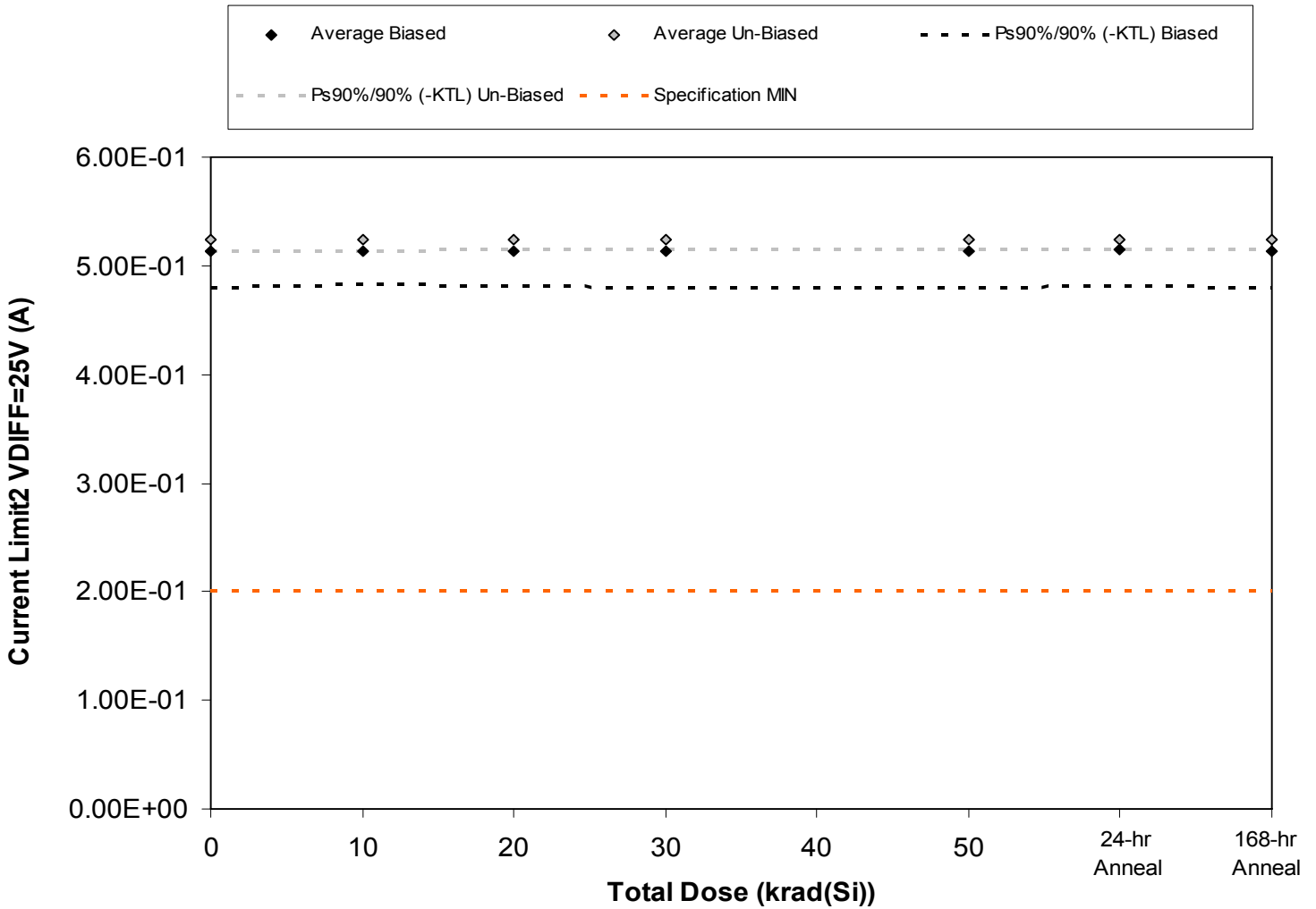
Figure 5.19. Plot of Current Limit2 VDIFF=25V (A) versus total dose. The solid diamonds are the average of the measured data points for the samples irradiated under electrical bias while the shaded diamonds are the average of the measured data points for the samples irradiated with all pins tied to ground. The black lines (solid and/or dashed) are the average of the data points after application of the KTL statistics on the samples irradiated under electrical bias while the gray lines (solid and/or dashed) are the average of the data points after application of the KTL statistics on the samples irradiated in the unbiased condition. The red dotted line(s) are the pre- and/or post-irradiation minimum and/or maximum specification value as defined in the datasheet and/or test plan.
