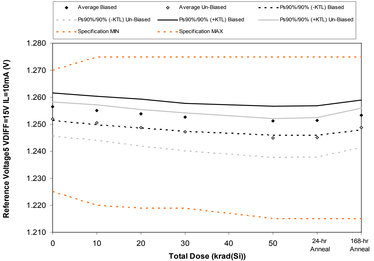
Figure 5.5. Plot of Reference Voltage5 VDIFF=15V IL=10mA (V) versus total dose. The solid diamonds are the average of the measured data points for the samples irradiated under electrical bias while the shaded diamonds are the average of the measured data points for the samples irradiated with all pins tied to ground. The black lines (solid and/or dashed) are the average of the data points after application of the KTL statistics on the samples irradiated under electrical bias while the gray lines (solid and/or dashed) are the average of the data points after application of the KTL statistics on the samples irradiated in the unbiased condition. The red dotted line(s) are the pre- and/or post-irradiation minimum and/or maximum specification value as defined in the datasheet and/or test plan.
