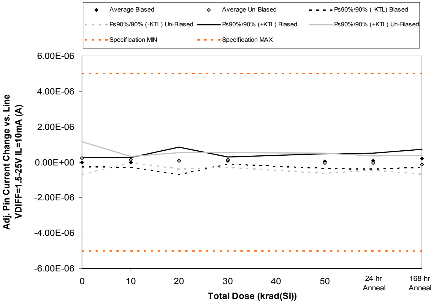
Figure 5.16. Plot of Adj. Pin Current Change vs. Line VDIFF=1.5-25V IL=10mA (A) versus total dose. The solid diamonds are the average of the measured data points for the samples irradiated under electrical bias while the shaded diamonds are the average of the measured data points for the samples irradiated with all pins tied to ground. The black lines (solid and/or dashed) are the average of the data points after application of the KTL statistics on the samples irradiated under electrical bias while the gray lines (solid and/or dashed) are the average of the data points after application of the KTL statistics on the samples irradiated in the unbiased condition. The red dotted line(s) are the pre- and/or post-irradiation minimum and/or maximum specification value as defined in the datasheet and/or test plan.
