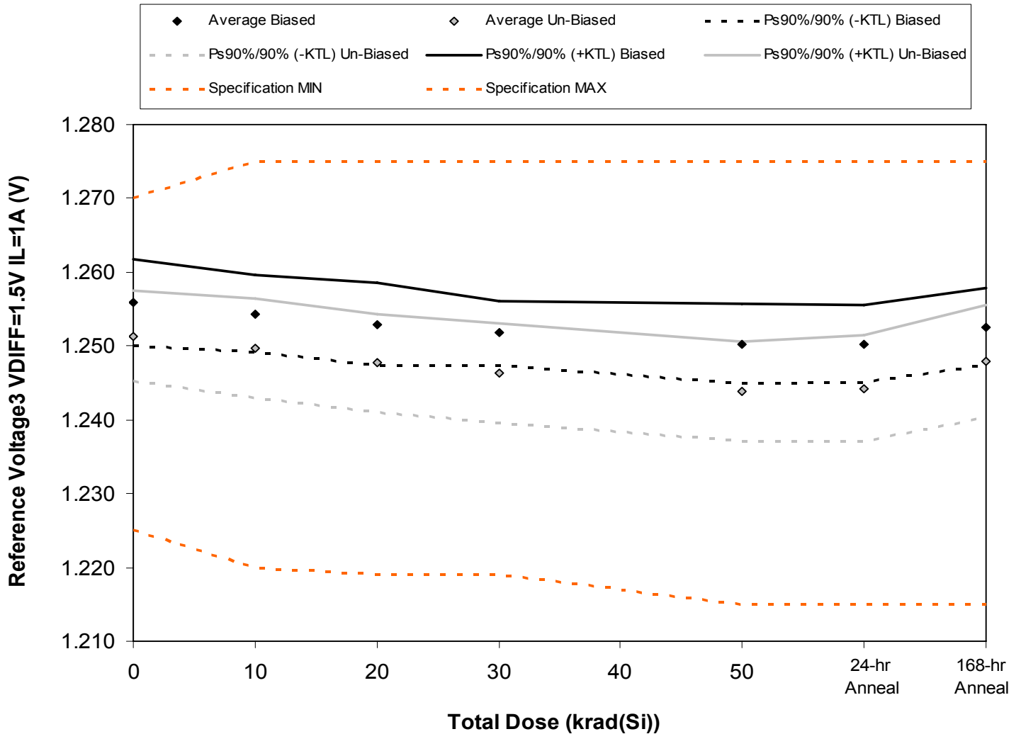
Figure 5.3. Plot of Reference Voltage3 VDIFF=1.5V IL=1A (V) versus total dose. The solid diamonds are the average of the measured data points for the samples irradiated under electrical bias while the shaded diamonds are the average of the measured data points for the samples irradiated with all pins tied to ground. The black lines (solid and/or dashed) are the average of the data points after application of the KTL statistics on the samples irradiated under electrical bias while the gray lines (solid and/or dashed) are the average of the data points after application of the KTL statistics on the samples irradiated in the unbiased condition. The red dotted line(s) are the pre- and/or post-irradiation minimum and/or maximum specification value as defined in the datasheet and/or test plan.
