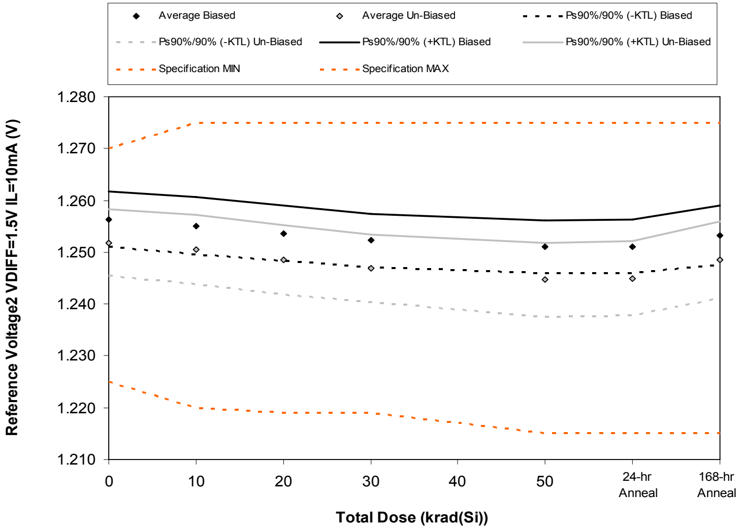
Figure 5.2. Plot of Reference Voltage2 VDIFF=1.5V IL=10mA (V) versus total dose. The solid diamonds are the average of the measured data points for the samples irradiated under electrical bias while the shaded diamonds are the average of the measured data points for the samples irradiated with all pins tied to ground. The black lines (solid and/or dashed) are the average of the data points after application of the KTL statistics on the samples irradiated under electrical bias while the gray lines (solid and/or dashed) are the average of the data points after application of the KTL statistics on the samples irradiated in the unbiased condition. The red dotted line(s) are the pre- and/or post-irradiation minimum and/or maximum specification value as defined in the datasheet and/or test plan.
