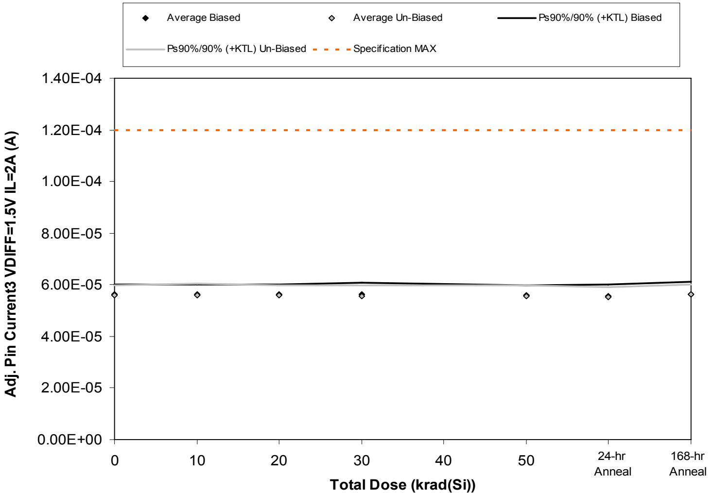
Figure 5.12. Plot of Adj. Pin Current3 VDIFF=1.5V IL=2A (A) versus total dose. The solid diamonds are the average of the measured data points for the samples irradiated under electrical bias while the shaded diamonds are the average of the measured data points for the samples irradiated with all pins tied to ground. The black lines (solid and/or dashed) are the average of the data points after application of the KTL statistics on the samples irradiated under electrical bias while the gray lines (solid and/or dashed) are the average of the data points after application of the KTL statistics on the samples irradiated in the unbiased condition. The red dotted line(s) are the pre- and/or post-irradiation minimum and/or maximum specification value as defined in the datasheet and/or test plan.
