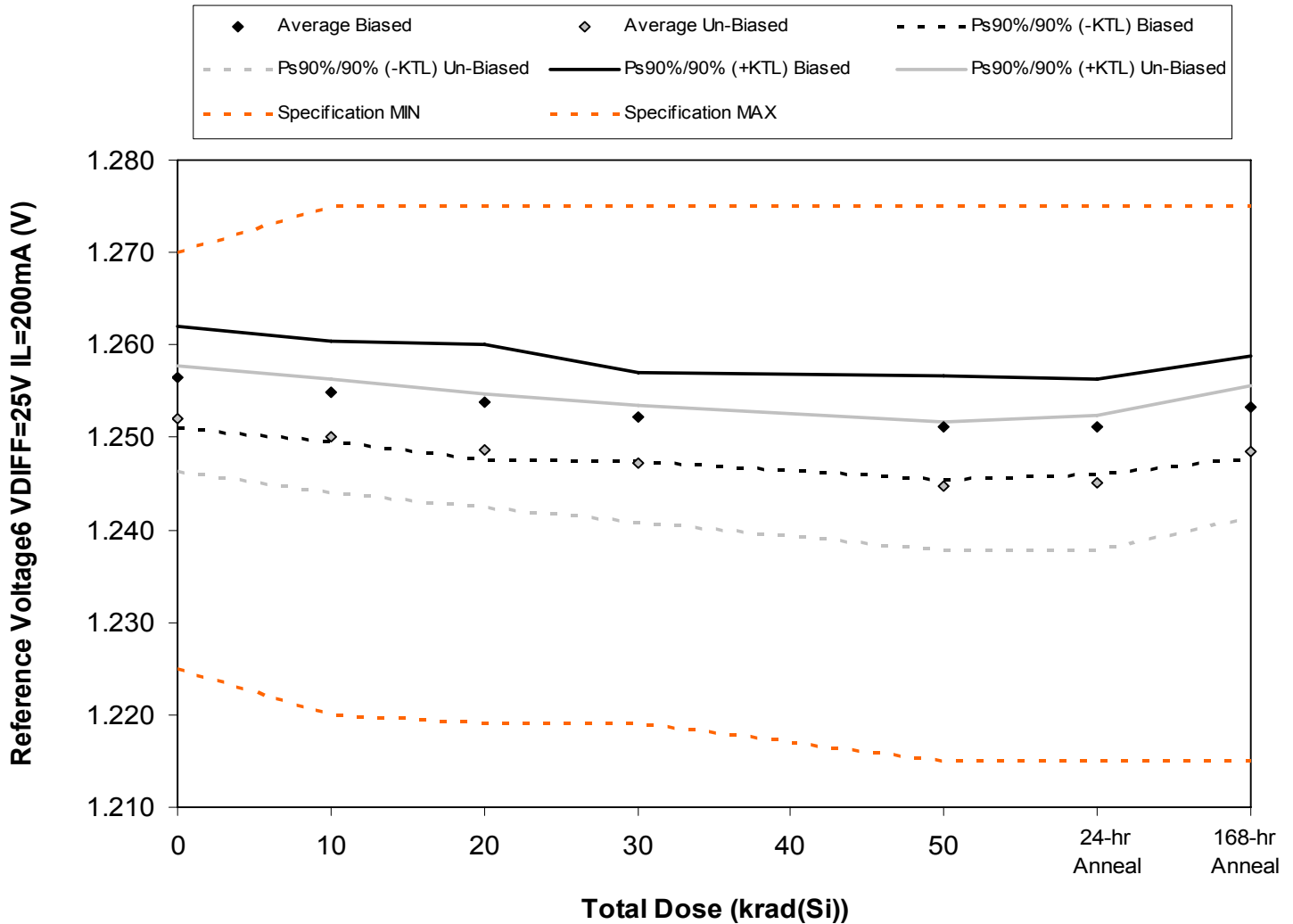
Figure 5.6. Plot of Reference Voltage6 VDIFF=25V IL=200mA (V) versus total dose. The solid diamonds are the average of the measured data points for the samples irradiated under electrical bias while the shaded diamonds are the average of the measured data points for the samples irradiated with all pins tied to ground. The black lines (solid and/or dashed) are the average of the data points after application of the KTL statistics on the samples irradiated under electrical bias while the gray lines (solid and/or dashed) are the average of the data points after application of the KTL statistics on the samples irradiated in the unbiased condition. The red dotted line(s) are the pre- and/or post-irradiation minimum and/or maximum specification value as defined in the datasheet and/or test plan.
