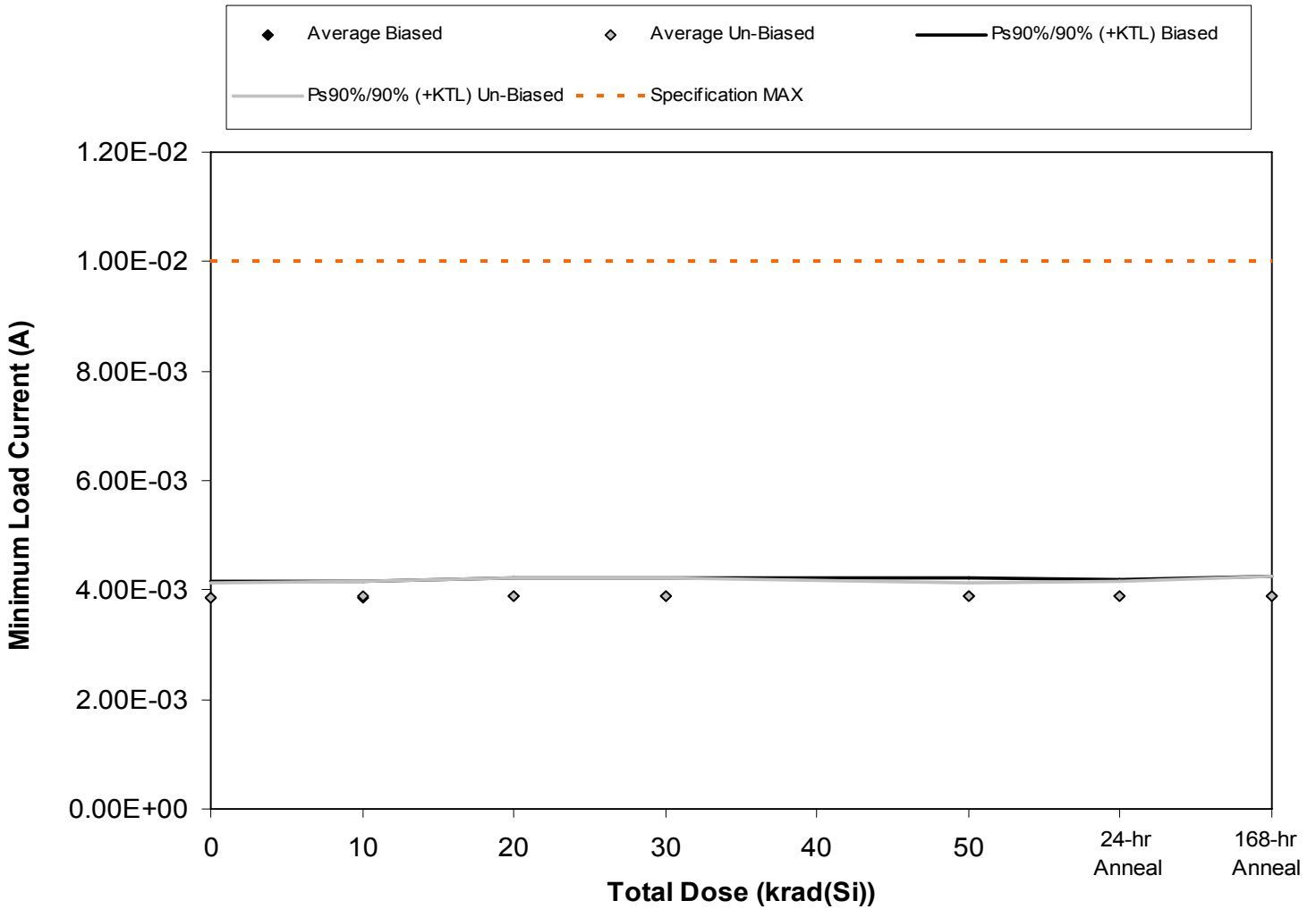
Figure 5.17. Plot of Minimum Load Current (A) versus total dose. The solid diamonds are the average of the measured data points for the samples irradiated under electrical bias while the shaded diamonds are the average of the measured data points for the samples irradiated with all pins tied to ground. The black lines (solid and/or dashed) are the average of the data points after application of the KTL statistics on the samples irradiated under electrical bias while the gray lines (solid and/or dashed) are the average of the data points after application of the KTL statistics on the samples irradiated in the unbiased condition. The red dotted line(s) are the pre- and/or post-irradiation minimum and/or maximum specification value as defined in the datasheet and/or test plan.
