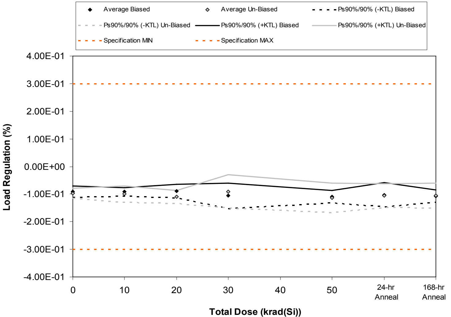
Figure 5.9. Plot of Load Regulation (%) versus total dose. The solid diamonds are the average of the measured data points for the samples irradiated under electrical bias while the shaded diamonds are the average of the measured data points for the samples irradiated with all pins tied to ground. The black lines (solid and/or dashed) are the average of the data points after application of the KTL statistics on the samples irradiated under electrical bias while the gray lines (solid and/or dashed) are the average of the data points after application of the KTL statistics on the samples irradiated in the unbiased condition. The red dotted line(s) are the pre- and/or post-irradiation minimum and/or maximum specification value as defined in the datasheet and/or test plan.
