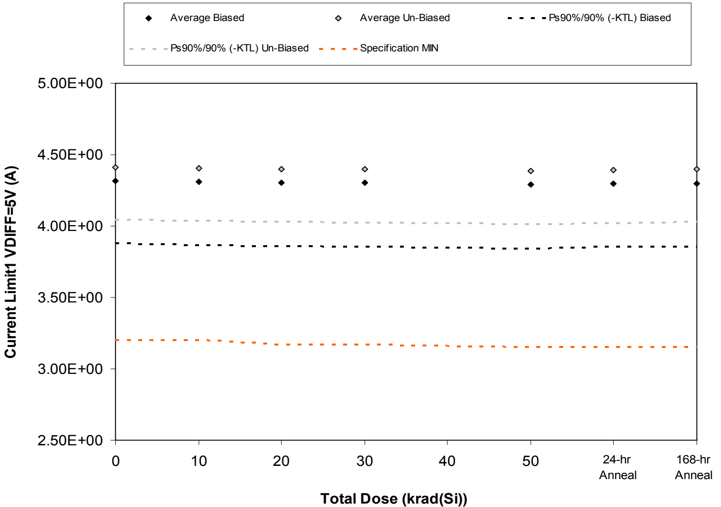
Figure 5.18. Plot of Current Limit1 VDIFF=5V (A) versus total dose. The solid diamonds are the average of the measured data points for the samples irradiated under electrical bias while the shaded diamonds are the average of the measured data points for the samples irradiated with all pins tied to ground. The black lines (solid and/or dashed) are the average of the data points after application of the KTL statistics on the samples irradiated under electrical bias while the gray lines (solid and/or dashed) are the average of the data points after application of the KTL statistics on the samples irradiated in the unbiased condition. The red dotted line(s) are the pre- and/or post-irradiation minimum and/or maximum specification value as defined in the datasheet and/or test plan.
