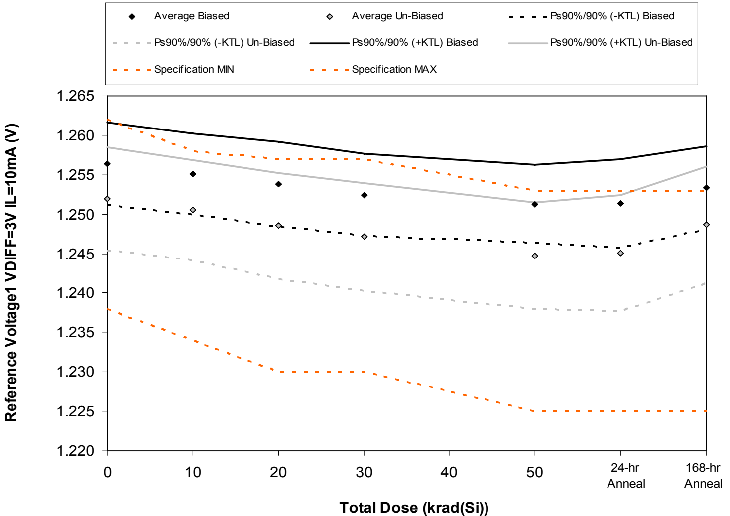
Figure 5.1. Plot of Reference Voltage1 VDIFF=3V IL=10mA (V) versus total dose. The solid diamonds are the average of the measured data points for the samples irradiated under electrical bias while the shaded diamonds are the average of the measured data points for the samples irradiated with all pins tied to ground. The black lines (solid and/or dashed) are the average of the data points after application of the KTL statistics on the samples irradiated under electrical bias while the gray lines (solid and/or dashed) are the average of the data points after application of the KTL statistics on the samples irradiated in the unbiased condition. The red dotted line(s) are the pre- and/or post-irradiation minimum and/or maximum specification value as defined in the datasheet and/or test plan.
