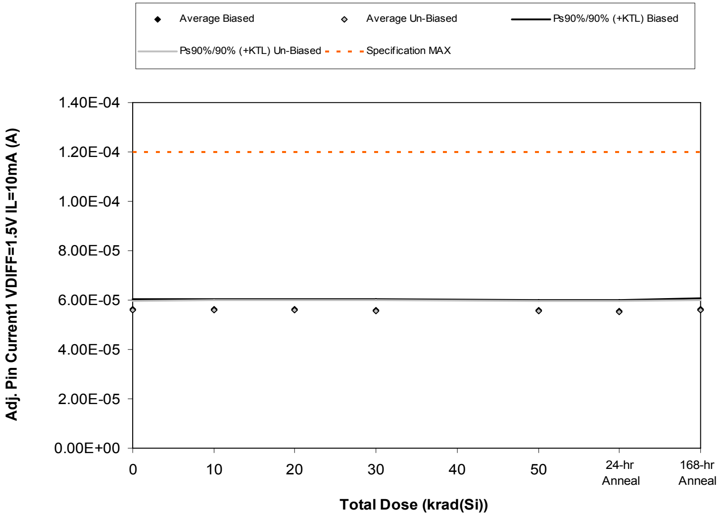
Figure 5.10. Plot of Adj. Pin Current1 VDIFF=1.5V IL=10mA (A) versus total dose. The solid diamonds are the average of the measured data points for the samples irradiated under electrical bias while the shaded diamonds are the average of the measured data points for the samples irradiated with all pins tied to ground. The black lines (solid and/or dashed) are the average of the data points after application of the KTL statistics on the samples irradiated under electrical bias while the gray lines (solid and/or dashed) are the average of the data points after application of the KTL statistics on the samples irradiated in the unbiased condition. The red dotted line(s) are the pre- and/or post-irradiation minimum and/or maximum specification value as defined in the datasheet and/or test plan.
