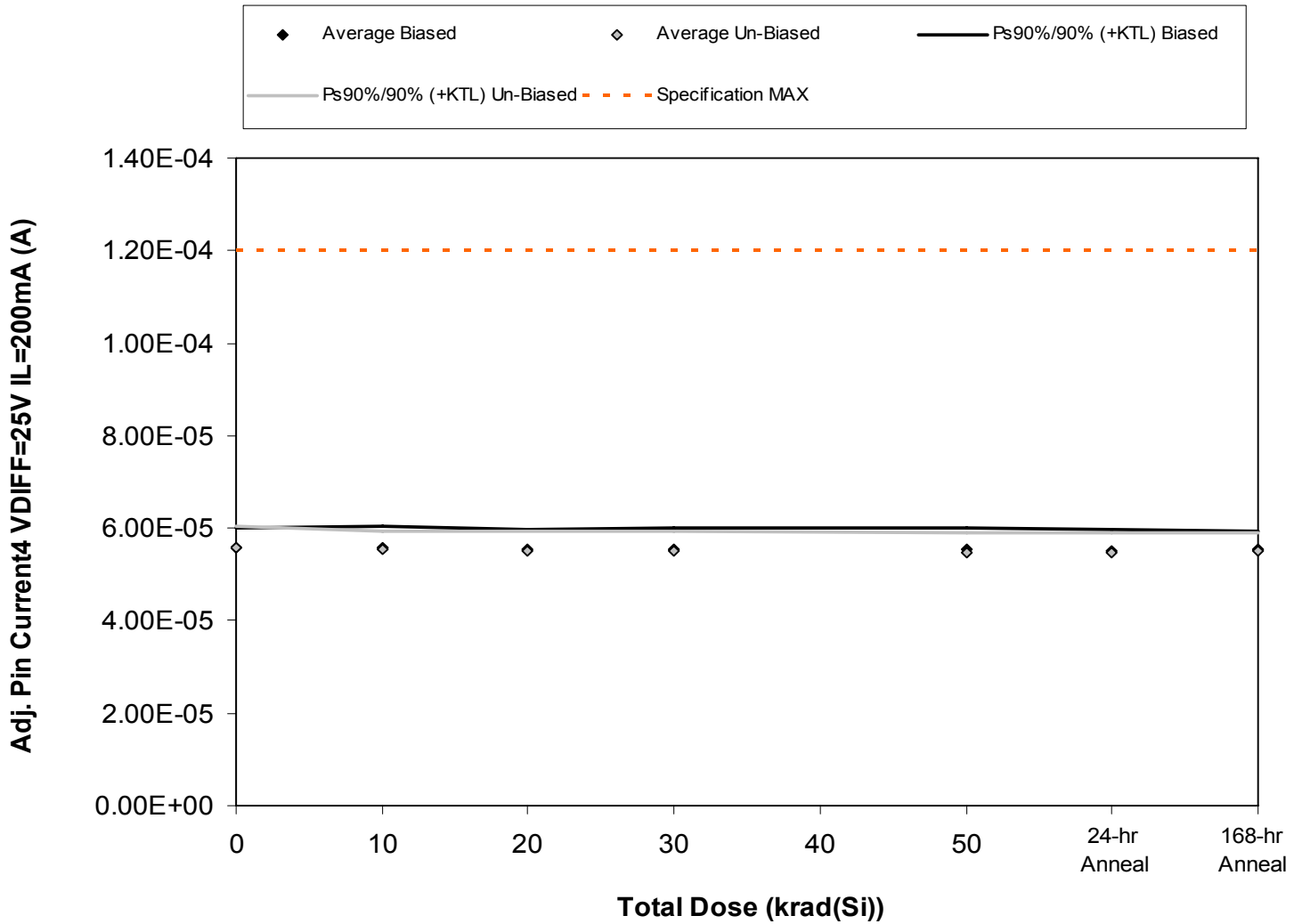
Figure 5.13. Plot of Adj. Pin Current 4 VDIFF=25V IL=200mA (A) versus total dose. The solid diamonds are the average of the measured data points for the samples irradiated under electrical bias while the shaded diamonds are the average of the measured data points for the samples irradiated with all pins tied to ground. The black lines (solid and/or dashed) are the average of the data points after application of the KTL statistics on the samples irradiated under electrical bias while the gray lines (solid and/or dashed) are the average of the data points after application of the KTL statistics on the samples irradiated in the unbiased condition. The red dotted line(s) are the pre- and/or post-irradiation minimum and/or maximum specification value as defined in the datasheet and/or test plan.
