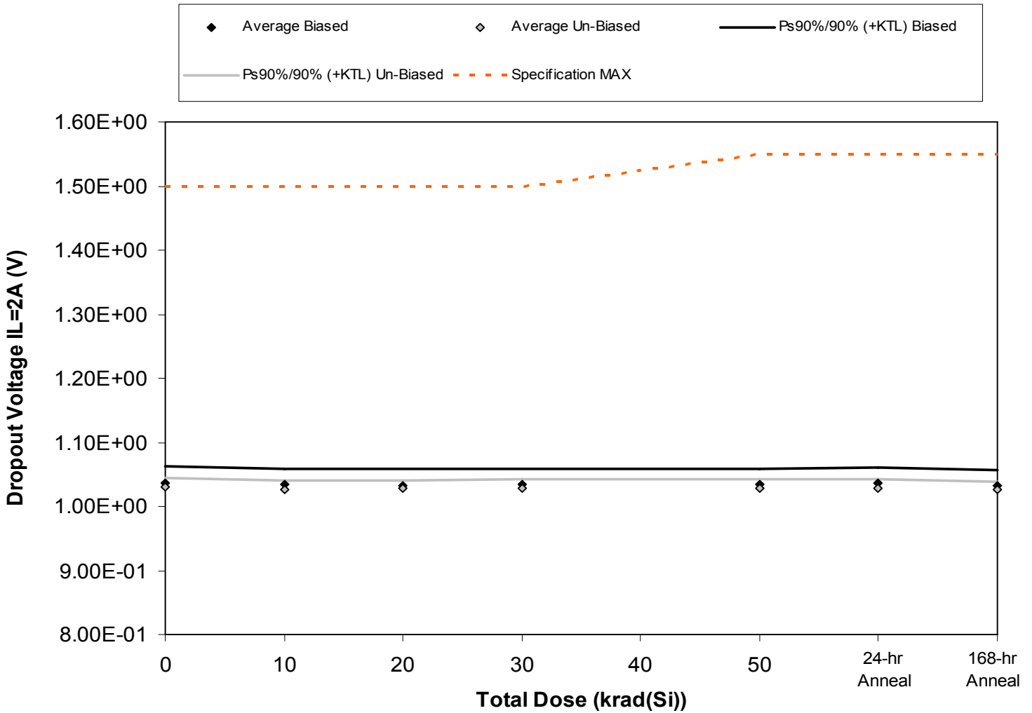
Figure 5.20. Plot of Dropout Voltage I_L=2A (V) versus total dose. The solid diamonds are the average of the measured data points for the samples irradiated under electrical bias while the shaded diamonds are the average of the measured data points for the samples irradiated with all pins tied to ground. The black lines (solid and/or dashed) are the average of the data points after application of the KTL statistics on the samples irradiated under electrical bias while the gray lines (solid and/or dashed) are the average of the data points after application of the KTL statistics on the samples irradiated in the unbiased condition. The red dotted line(s) are the pre- and/or post-irradiation minimum and/or maximum specification value as defined in the datasheet and/or test plan.
