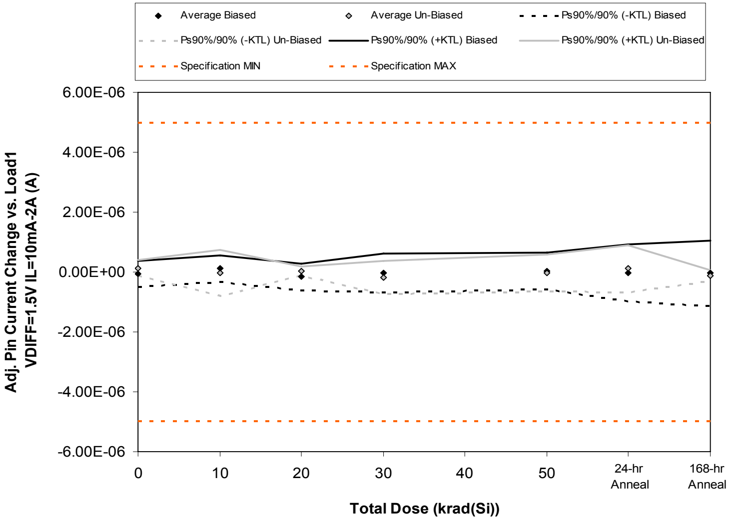
Figure 5.14. Plot of Adj. Pin Current Change vs. Load1 VDIFF=1.5V IL=10mA-2A (A) versus total dose. The solid diamonds are the average of the measured data points for the samples irradiated under electrical bias while the shaded diamonds are the average of the measured data points for the samples irradiated with all pins tied to ground. The black lines (solid and/or dashed) are the average of the data points after application of the KTL statistics on the samples irradiated under electrical bias while the gray lines (solid and/or dashed) are the average of the data points after application of the KTL statistics on the samples irradiated in the unbiased condition. The red dotted line(s) are the pre- and/or post-irradiation minimum and/or maximum specification value as defined in the datasheet and/or test plan.
