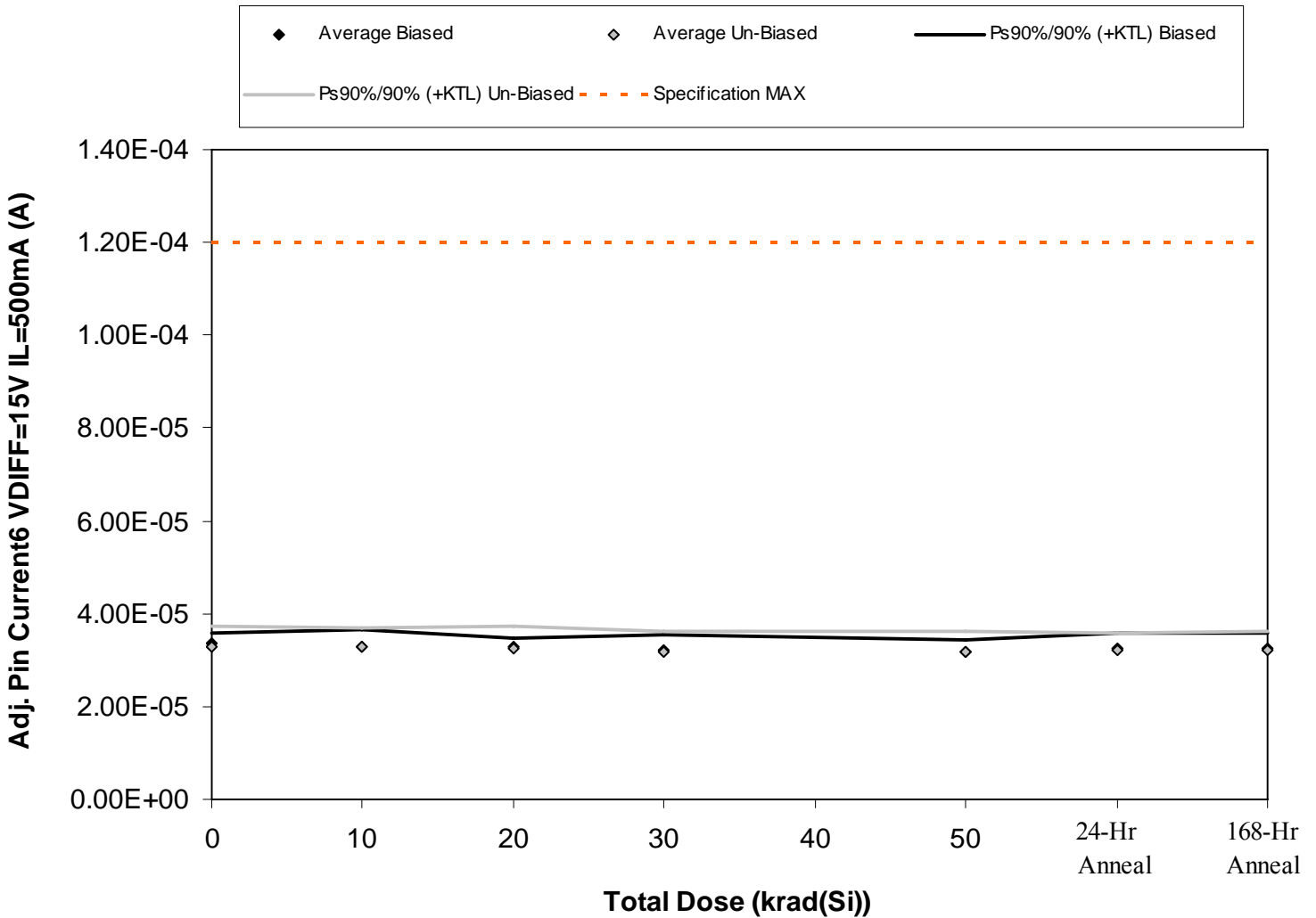
Figure 5.13. Plot of Adj. Pin Current6 VDIFF=15V IL=500mA (A) versus total dose. The solid diamonds are the average of the measured data points for the samples irradiated under electrical bias while the shaded diamonds are the average of the measured data points for the samples irradiated with all pins tied to ground. The black lines (solid and/or dashed) are the average of the data points after application of the KTL statistics on the samples irradiated under electrical bias while the gray lines (solid and/or dashed) are the average of the data points after application of the KTL statistics on the samples irradiated in the unbiased condition. The red dotted line(s) are the pre- and/or post-irradiation minimum and/or maximum specification value as defined in the datasheet and/or test plan.
