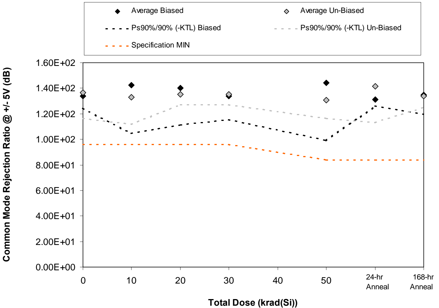
Figure 5.7. Plot of the common mode rejection ratio (CMRR) at V_S = \pm 5V versus total dose. The data show no significant degradation with total dose. The solid diamonds are the average of the measured data points for the sample irradiated under electrical bias while the shaded diamonds are the average of the measured data points for the units irradiated with all pins tied to ground. The black lines (solid or dashed) are the average of the data points after application of the KTL statistics on the sample irradiated in the biased condition while the shaded lines (solid or dashed) are the average of the data points after application of the KTL statistics on the sample irradiated in the unbiased condition. The red dotted line(s) are the pre- and/or post-irradiation minimum and/or maximum specification value as defined in the datasheet and/or test plan.
