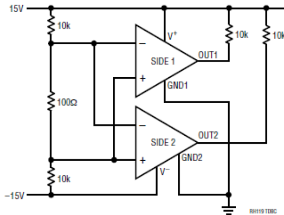
Figure B.1. Irradiation bias circuit. This figure was extracted from Linear Technology RH119 Datasheet I.D No. 66-10-0176 Revision C.
