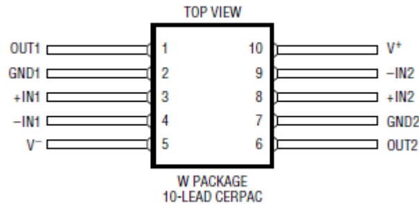
Figure B.2. W Package drawing (for reference only). This figure was extracted from Linear Technology RH119 Datasheet I.D No. 66-10-0176 Revision C.
