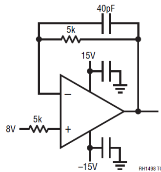
Figure B.1. Irradiation bias drawing for the units to be irradiated under electrical bias. This figure was extracted from Linear Technology RH1498M Datasheet.
