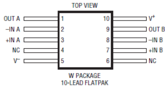
Figure B.2. W package drawing (for reference only). This figure was extracted from the Linear Technology RH1498M Datasheet.
