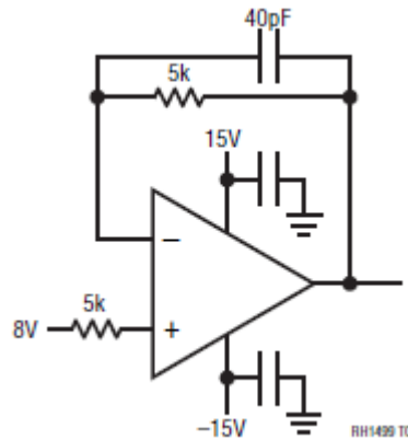
Figure B.1. Irradiation bias circuit. This figure was extracted from Linear Technology RH1499M datasheet, ID No 66-10-1499.
