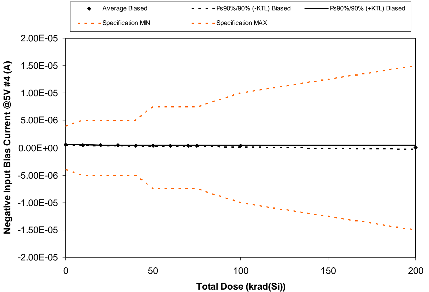
Figure 5.96. Plot of Negative Input Bias Current @5V #4 (A) versus total dose. The solid diamonds are the average of the measured data points for the samples irradiated under electrical bias and the black lines (solid and/or dashed) are the average of the data points after application of the KTL statistics on the samples irradiated under electrical bias. The red dotted line(s) are the pre- and/or post-irradiation minimum and/or maximum specification value as defined in the datasheet and/or test plan.
