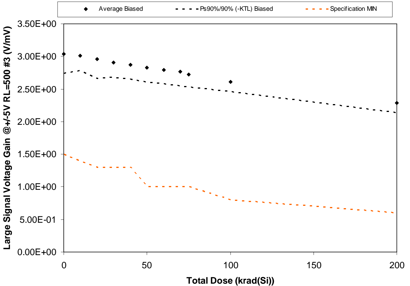
Figure 5.29. Plot of Large Signal Voltage Gain @ +/-5V RL=500 #3 (V/mV) versus total dose. The solid diamonds are the average of the measured data points for the samples irradiated under electrical bias and the black lines (solid and/or dashed) are the average of the data points after application of the KTL statistics on the samples irradiated under electrical bias. The red dotted line(s) are the pre- and/or post-irradiation minimum and/or maximum specification value as defined in the datasheet and/or test plan.
