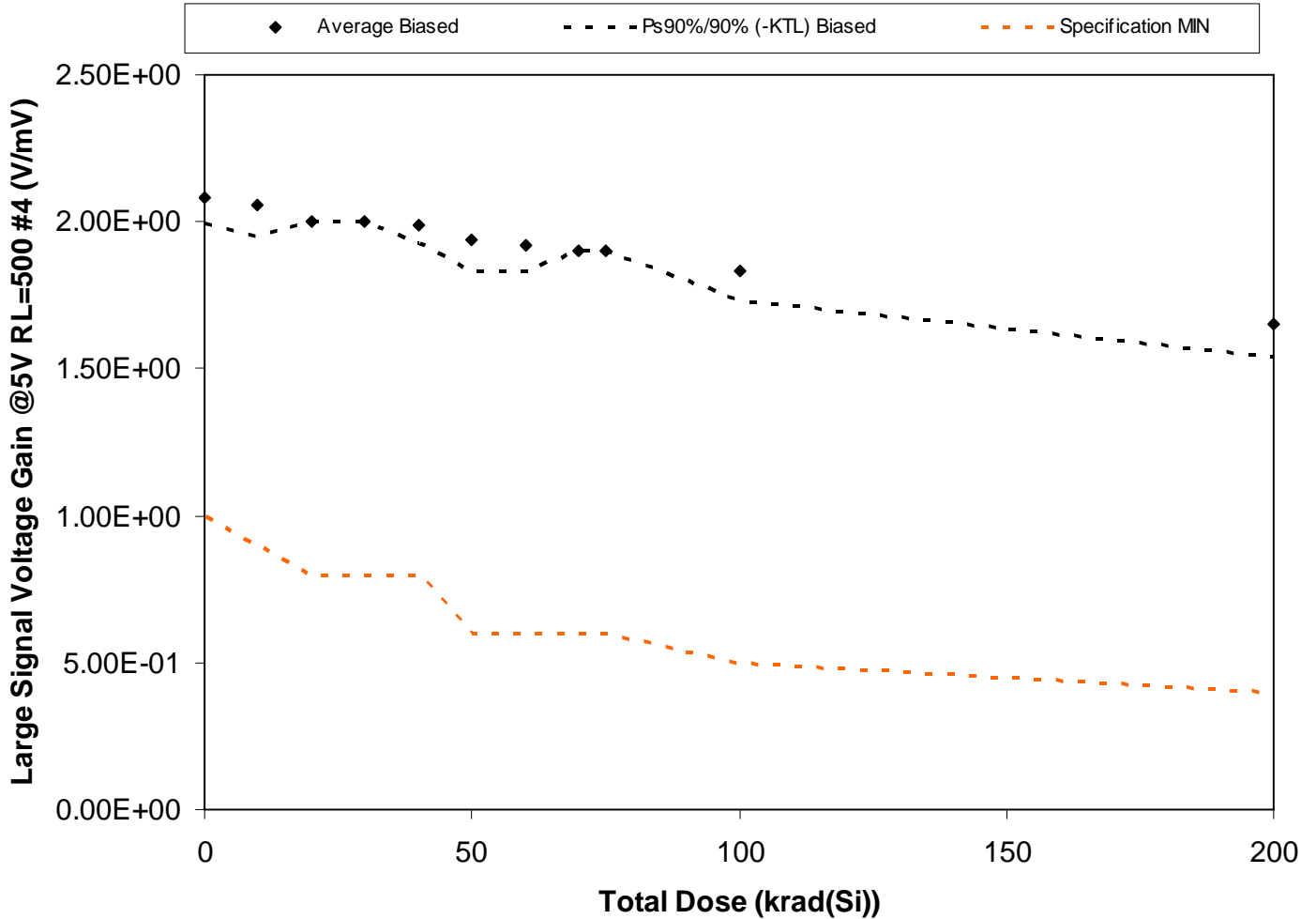
Figure 5.104. Plot of Large Signal Voltage Gain @5V RL=500 #4 (V/mV) versus total dose. The solid diamonds are the average of the measured data points for the samples irradiated under electrical bias and the black lines (solid and/or dashed) are the average of the data points after application of the KTL statistics on the samples irradiated under electrical bias. The red dotted line(s) are the pre- and/or post-irradiation minimum and/or maximum specification value as defined in the datasheet and/or test plan.
