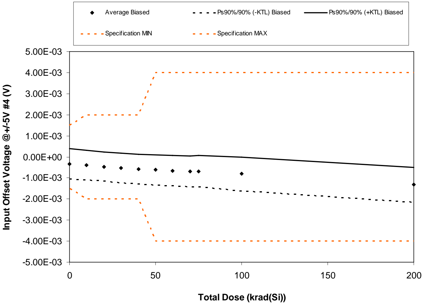
Figure 5.6. Plot of Input Offset Voltage @ +/-5V #4 (V) versus total dose. The solid diamonds are the average of the measured data points for the samples irradiated under electrical bias and the black lines (solid and/or dashed) are the average of the data points after application of the KTL statistics on the samples irradiated under electrical bias. The red dotted line(s) are the pre- and/or post-irradiation minimum and/or maximum specification value as defined in the datasheet and/or test plan.
