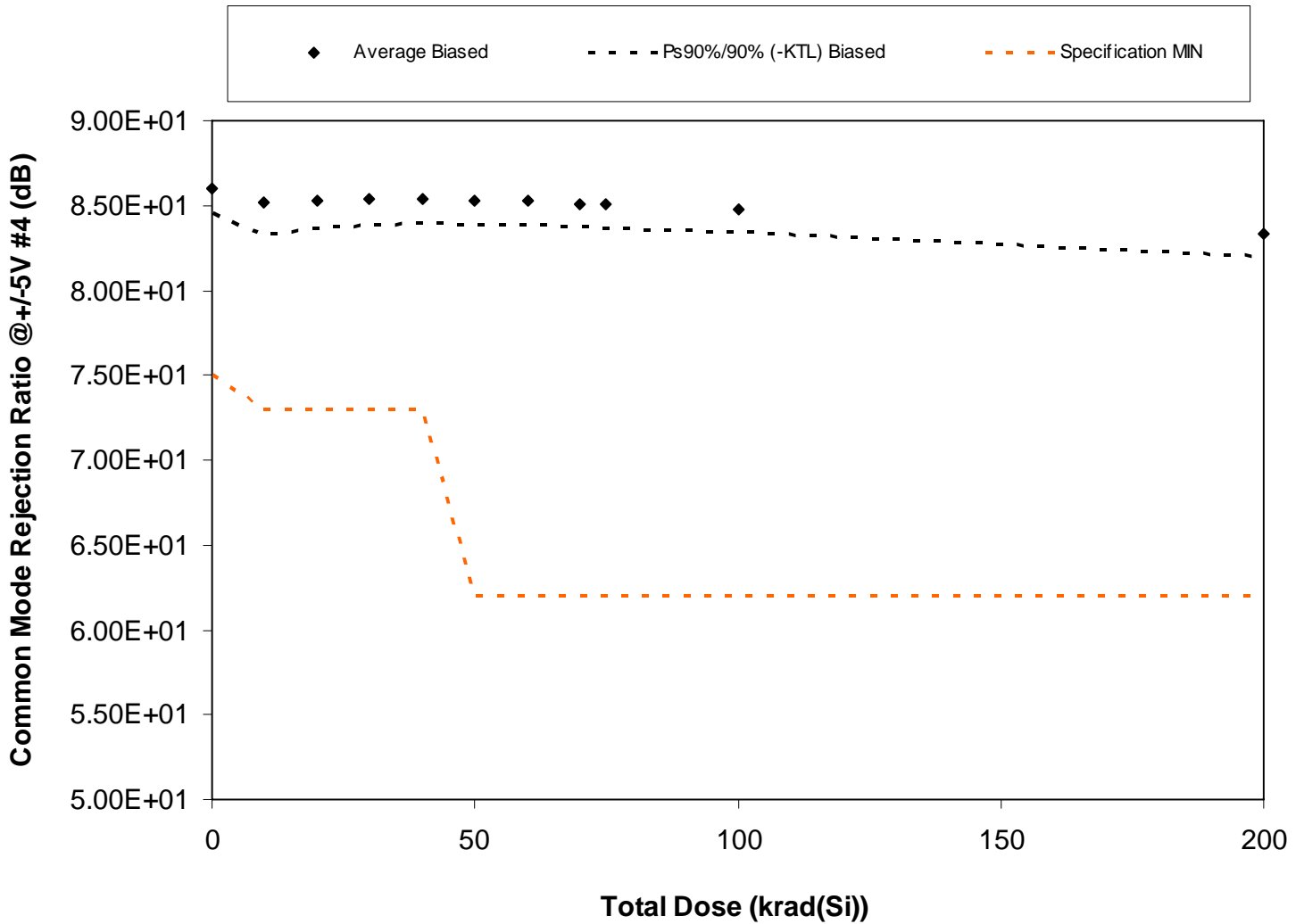
Figure 5.22. Plot of Common Mode Rejection Ratio @ +/-5V #4 (dB) versus total dose. The solid diamonds are the average of the measured data points for the samples irradiated under electrical bias and the black lines (solid and/or dashed) are the average of the data points after application of the KTL statistics on the samples irradiated under electrical bias. The red dotted line(s) are the pre- and/or post-irradiation minimum and/or maximum specification value as defined in the datasheet and/or test plan.
