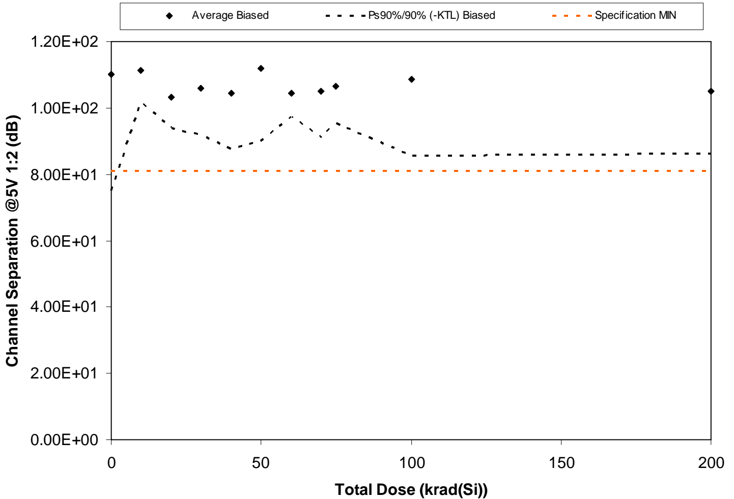
Figure 5.109. Plot of Channel Separation @5V 1:2 (dB) versus total dose. The solid diamonds are the average of the measured data points for the samples irradiated under electrical bias and the black lines (solid and/or dashed) are the average of the data points after application of the KTL statistics on the samples irradiated under electrical bias. The red dotted line(s) are the pre- and/or post-irradiation minimum and/or maximum specification value as defined in the datasheet and/or test plan.
