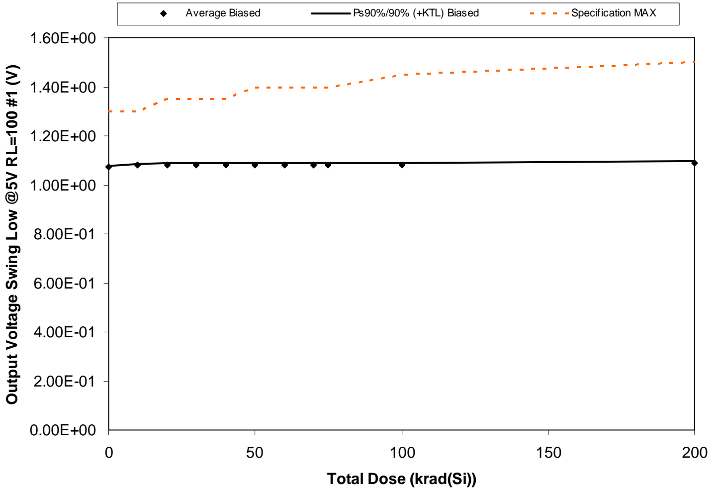
Figure 5.133. Plot of Output Voltage Swing Low @5V RL=100 #1 (V) versus total dose. The solid diamonds are the average of the measured data points for the samples irradiated under electrical bias and the black lines (solid and/or dashed) are the average of the data points after application of the KTL statistics on the samples irradiated under electrical bias. The red dotted line(s) are the pre- and/or post-irradiation minimum and/or maximum specification value as defined in the datasheet and/or test plan.
