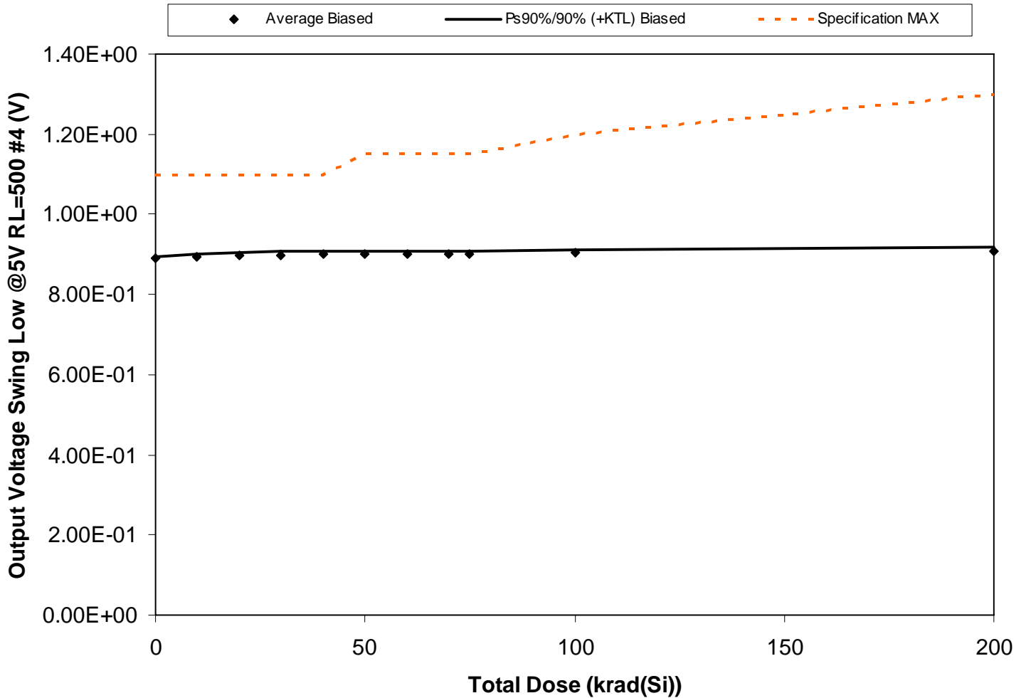
Figure 5.132. Plot of Output Voltage Swing Low @5V RL=500 #4 (V) versus total dose. The solid diamonds are the average of the measured data points for the samples irradiated under electrical bias and the black lines (solid and/or dashed) are the average of the data points after application of the KTL statistics on the samples irradiated under electrical bias. The red dotted line(s) are the pre- and/or post-irradiation minimum and/or maximum specification value as defined in the datasheet and/or test plan.
