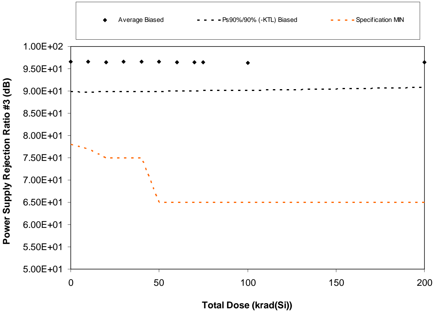
Figure 5.25. Plot of Power Supply Rejection Ratio #3 (dB) versus total dose. The solid diamonds are the average of the measured data points for the samples irradiated under electrical bias and the black lines (solid and/or dashed) are the average of the data points after application of the KTL statistics on the samples irradiated under electrical bias. The red dotted line(s) are the pre- and/or post-irradiation minimum and/or maximum specification value as defined in the datasheet and/or test plan.
