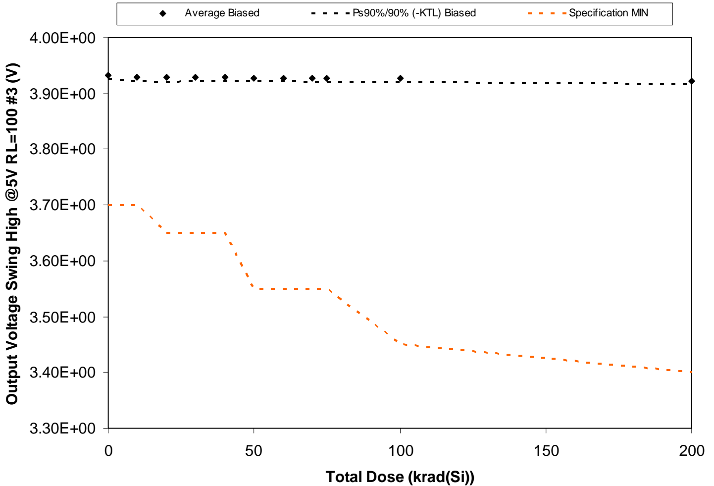
Figure 5.127. Plot of Output Voltage Swing High @5V RL=100 #3 (V) versus total dose. The solid diamonds are the average of the measured data points for the samples irradiated under electrical bias and the black lines (solid and/or dashed) are the average of the data points after application of the KTL statistics on the samples irradiated under electrical bias. The red dotted line(s) are the pre- and/or post-irradiation minimum and/or maximum specification value as defined in the datasheet and/or test plan.
