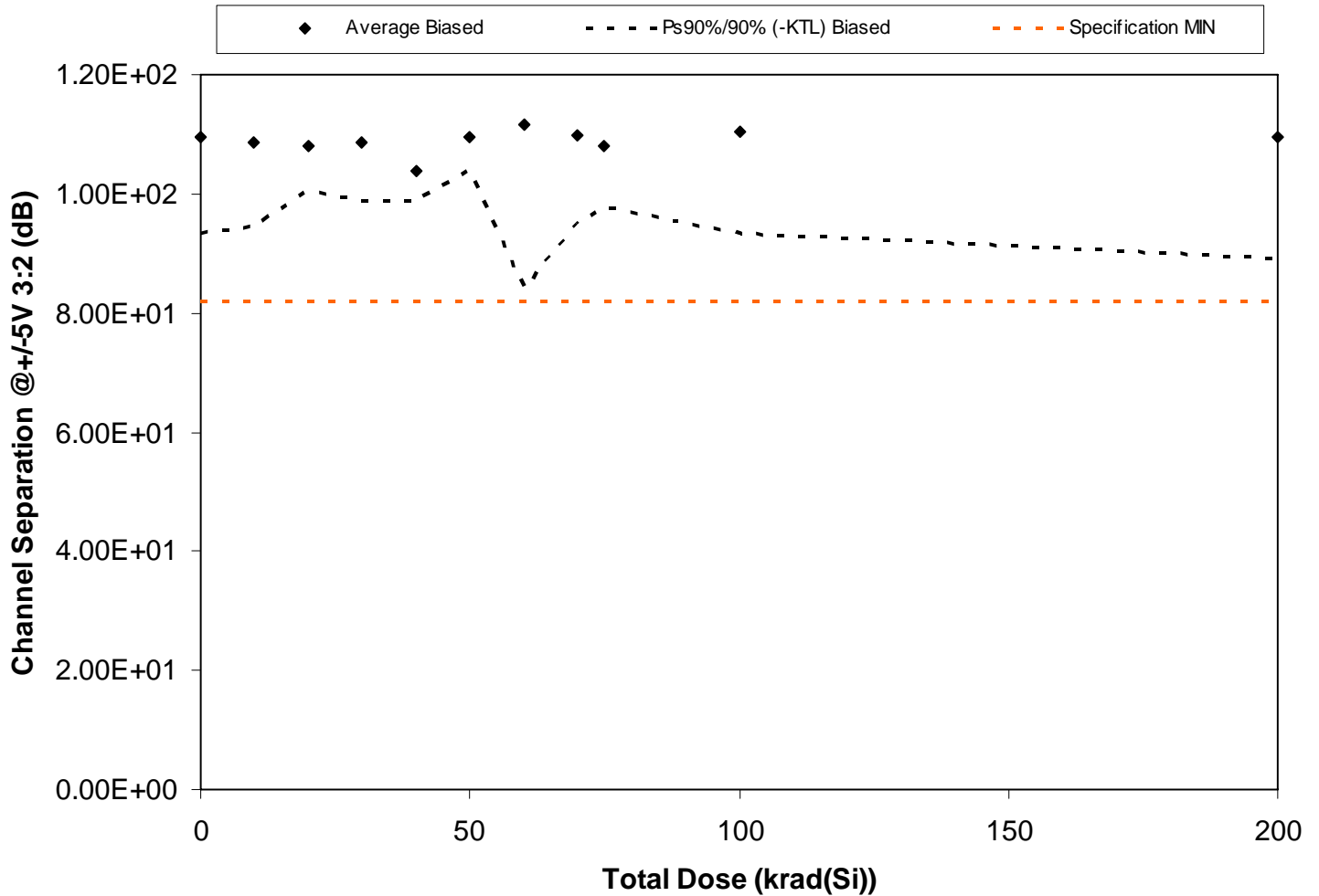
Figure 5.42. Plot of Channel Separation @ +/-5V 3:2 (dB) versus total dose. The solid diamonds are the average of the measured data points for the samples irradiated under electrical bias and the black lines (solid and/or dashed) are the average of the data points after application of the KTL statistics on the samples irradiated under electrical bias. The red dotted line(s) are the pre- and/or post-irradiation minimum and/or maximum specification value as defined in the datasheet and/or test plan.
