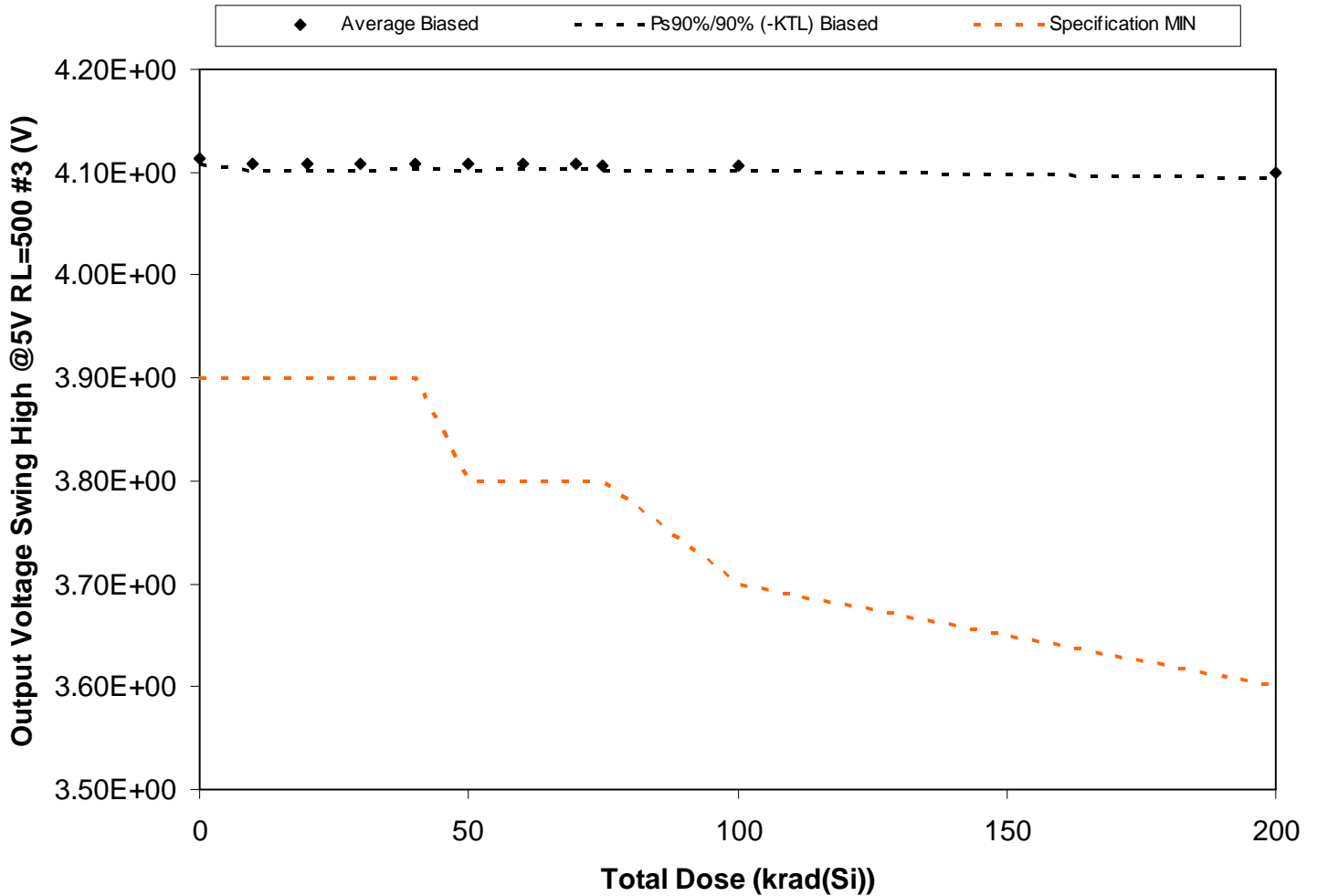
Figure 5.123. Plot of Output Voltage Swing High @5V RL=500 #3 (V) versus total dose. The solid diamonds are the average of the measured data points for the samples irradiated under electrical bias and the black lines (solid and/or dashed) are the average of the data points after application of the KTL statistics on the samples irradiated under electrical bias. The red dotted line(s) are the pre- and/or post-irradiation minimum and/or maximum specification value as defined in the datasheet and/or test plan.
