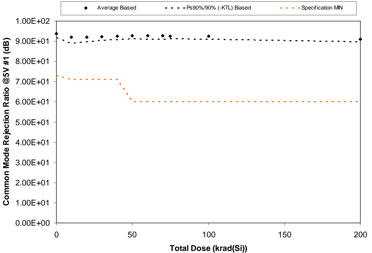
Figure 5.97. Plot of Common Mode Rejection Ratio @5V #1 (dB) versus total dose. The solid diamonds are the average of the measured data points for the samples irradiated under electrical bias and the black lines (solid and/or dashed) are the average of the data points after application of the KTL statistics on the samples irradiated under electrical bias. The red dotted line(s) are the pre- and/or post-irradiation minimum and/or maximum specification value as defined in the datasheet and/or test plan.
