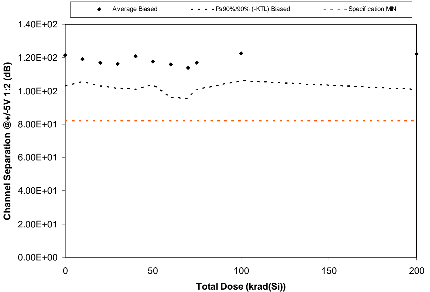
Figure 5.35. Plot of Channel Separation @ +/-5V 1:2 (dB) versus total dose. The solid diamonds are the average of the measured data points for the samples irradiated under electrical bias and the black lines (solid and/or dashed) are the average of the data points after application of the KTL statistics on the samples irradiated under electrical bias. The red dotted line(s) are the pre- and/or post-irradiation minimum and/or maximum specification value as defined in the datasheet and/or test plan.
