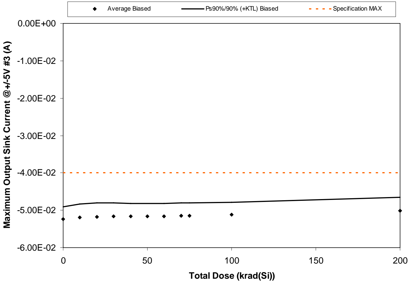
Figure 5.69. Plot of Maximum Output Sink Current @ +/-5V #3 (A) versus total dose. The solid diamonds are the average of the measured data points for the samples irradiated under electrical bias and the black lines (solid and/or dashed) are the average of the data points after application of the KTL statistics on the samples irradiated under electrical bias. The red dotted line(s) are the pre- and/or post-irradiation minimum and/or maximum specification value as defined in the datasheet and/or test plan.
