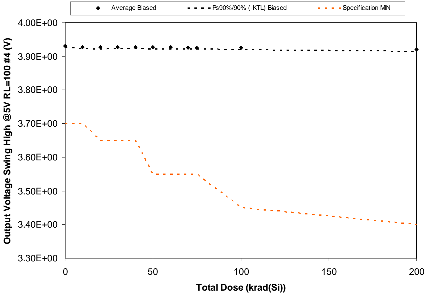
Figure 5.128. Plot of Output Voltage Swing High @5V RL=100 #4 (V) versus total dose. The solid diamonds are the average of the measured data points for the samples irradiated under electrical bias and the black lines (solid and/or dashed) are the average of the data points after application of the KTL statistics on the samples irradiated under electrical bias. The red dotted line(s) are the pre- and/or post-irradiation minimum and/or maximum specification value as defined in the datasheet and/or test plan.
