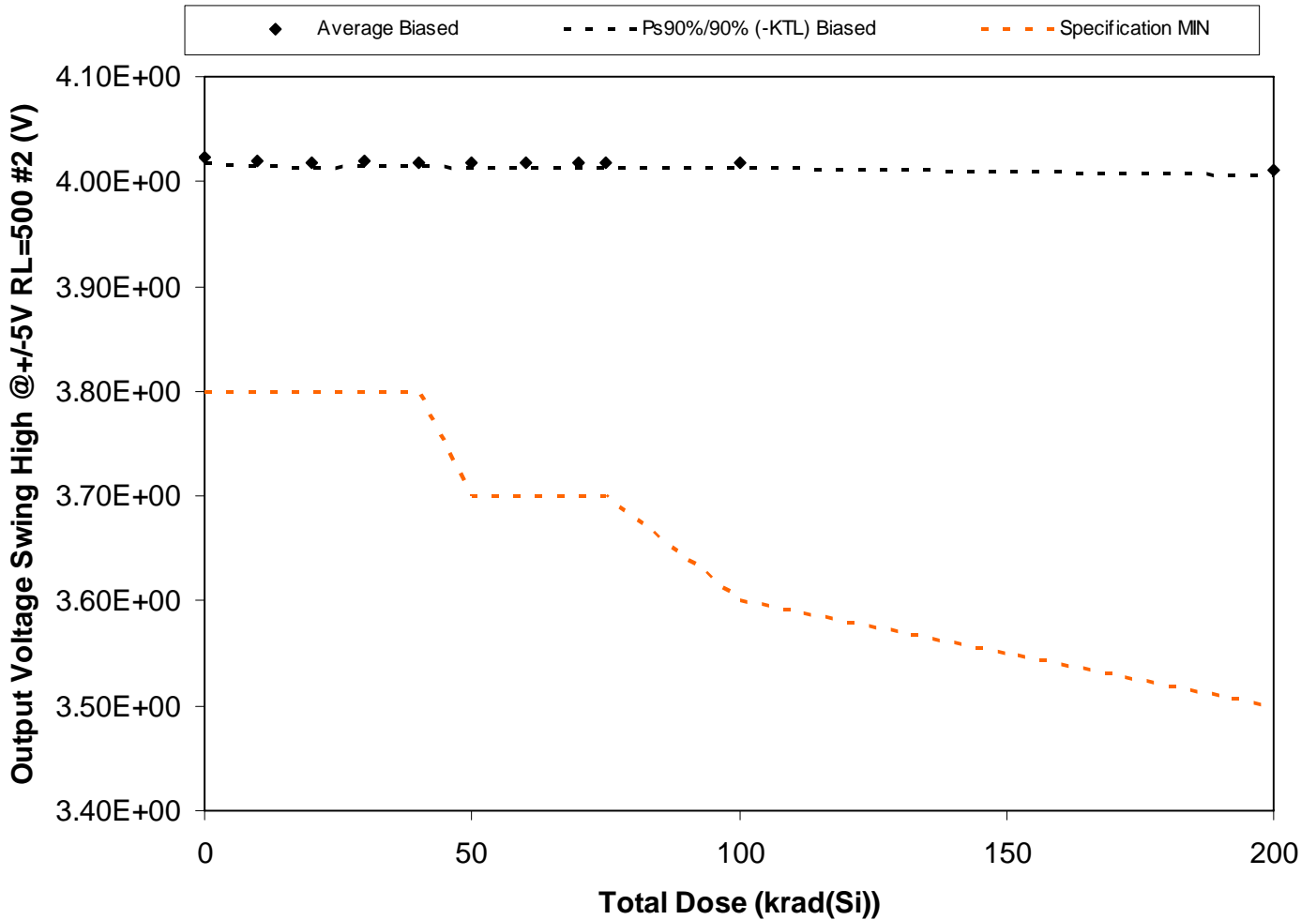
Figure 5.48. Plot of Output Voltage Swing High @ +/-5V RL=500 #2 (V) versus total dose. The solid diamonds are the average of the measured data points for the samples irradiated under electrical bias and the black lines (solid and/or dashed) are the average of the data points after application of the KTL statistics on the samples irradiated under electrical bias. The red dotted line(s) are the pre- and/or post-irradiation minimum and/or maximum specification value as defined in the datasheet and/or test plan.
