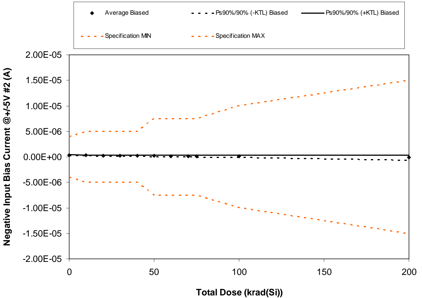
Figure 5.16. Plot of Negative Input Bias Current @ +/-5V #2 (A) versus total dose. The solid diamonds are the average of the measured data points for the samples irradiated under electrical bias and the black lines (solid and/or dashed) are the average of the data points after application of the KTL statistics on the samples irradiated under electrical bias. The red dotted line(s) are the pre- and/or post-irradiation minimum and/or maximum specification value as defined in the datasheet and/or test plan.
