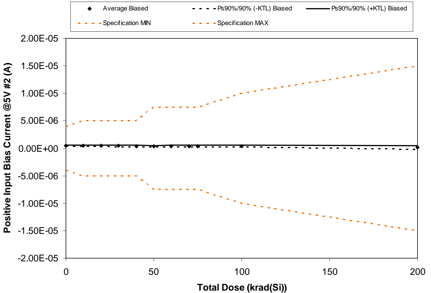
Figure 5.90. Plot of Positive Input Bias Current @5V #2 (A) versus total dose. The solid diamonds are the average of the measured data points for the samples irradiated under electrical bias and the black lines (solid and/or dashed) are the average of the data points after application of the KTL statistics on the samples irradiated under electrical bias. The red dotted line(s) are the pre- and/or post-irradiation minimum and/or maximum specification value as defined in the datasheet and/or test plan.
