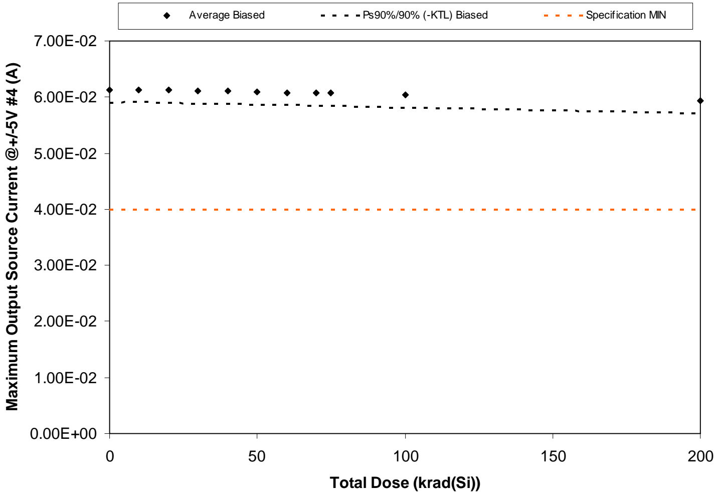
Figure 5.66. Plot of Maximum Output Source Current @ +/-5V #4 (A) versus total dose. The solid diamonds are the average of the measured data points for the samples irradiated under electrical bias and the black lines (solid and/or dashed) are the average of the data points after application of the KTL statistics on the samples irradiated under electrical bias. The red dotted line(s) are the pre- and/or post-irradiation minimum and/or maximum specification value as defined in the datasheet and/or test plan.
