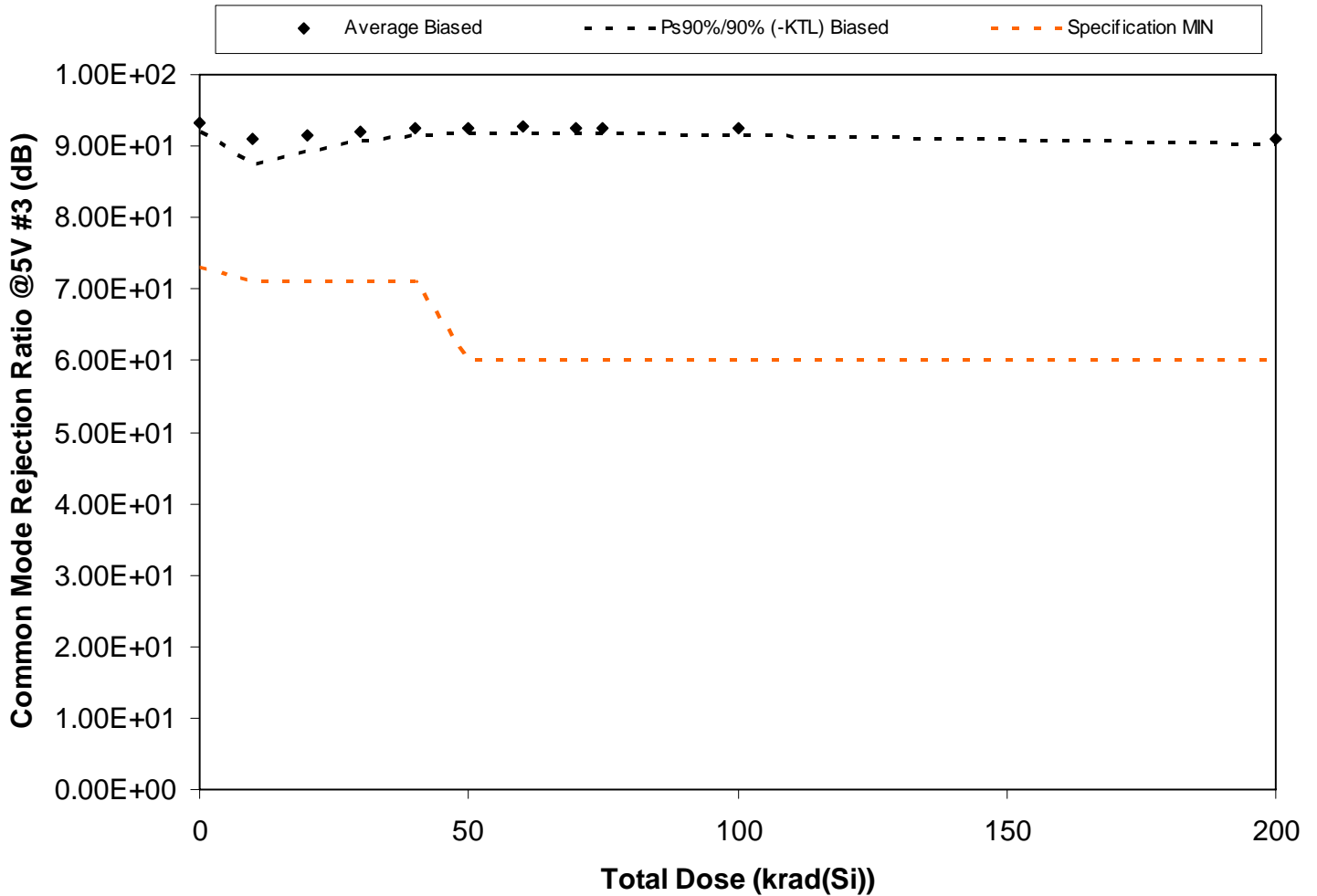
Figure 5.99. Plot of Common Mode Rejection Ratio @5V #3 (dB) versus total dose. The solid diamonds are the average of the measured data points for the samples irradiated under electrical bias and the black lines (solid and/or dashed) are the average of the data points after application of the KTL statistics on the samples irradiated under electrical bias. The red dotted line(s) are the pre- and/or post-irradiation minimum and/or maximum specification value as defined in the datasheet and/or test plan.
