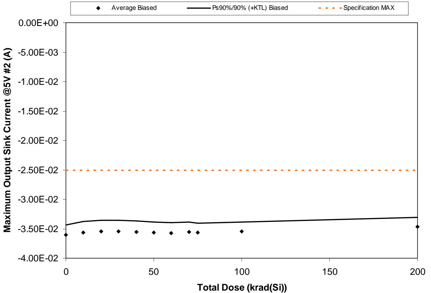
Figure 5.142. Plot of Maximum Output Sink Current @5V #2 (A) versus total dose. The solid diamonds are the average of the measured data points for the samples irradiated under electrical bias and the black lines (solid and/or dashed) are the average of the data points after application of the KTL statistics on the samples irradiated under electrical bias. The red dotted line(s) are the pre- and/or post-irradiation minimum and/or maximum specification value as defined in the datasheet and/or test plan.
