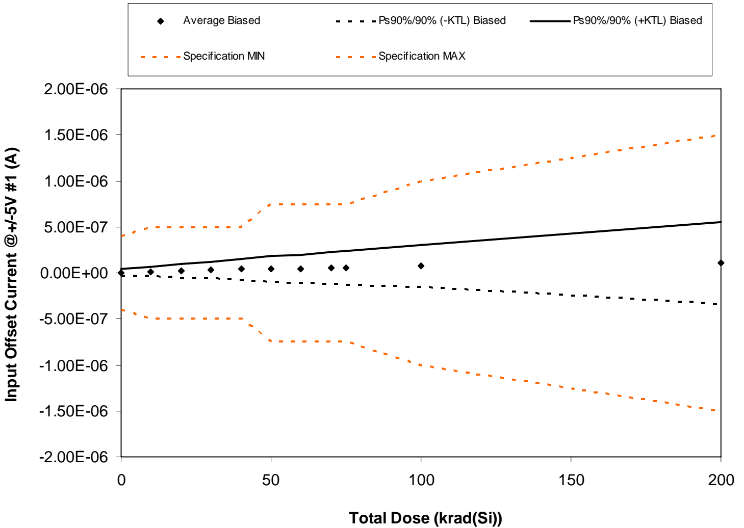
Figure 5.7. Plot of Input Offset Current @ +/-5V #1 (A) versus total dose. The solid diamonds are the average of the measured data points for the samples irradiated under electrical bias and the black lines (solid and/or dashed) are the average of the data points after application of the KTL statistics on the samples irradiated under electrical bias. The red dotted line(s) are the pre- and/or post-irradiation minimum and/or maximum specification value as defined in the datasheet and/or test plan.
