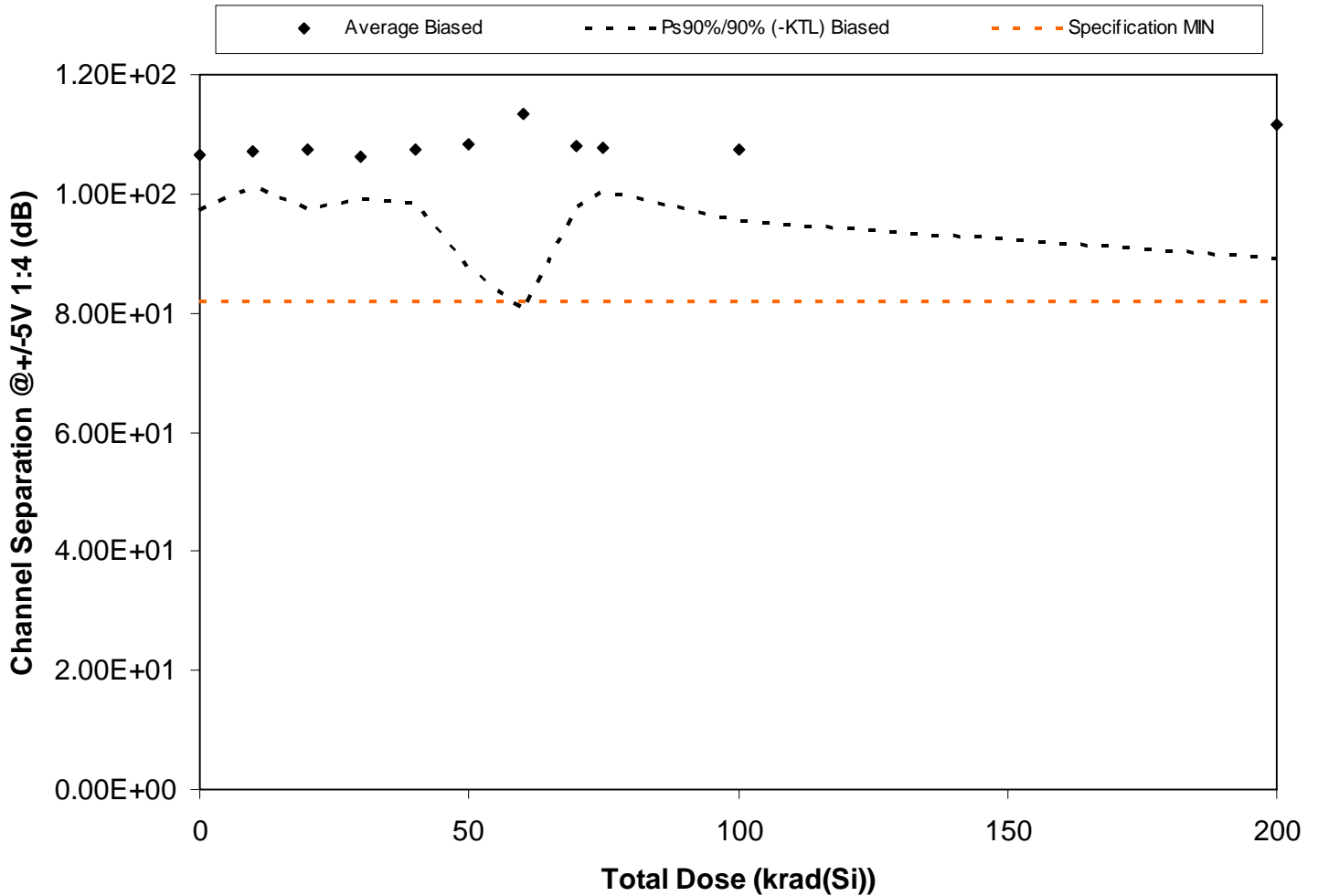
Figure 5.37. Plot of Channel Separation @ +/-5V 1:4 (dB) versus total dose. The solid diamonds are the average of the measured data points for the samples irradiated under electrical bias and the black lines (solid and/or dashed) are the average of the data points after application of the KTL statistics on the samples irradiated under electrical bias. The red dotted line(s) are the pre- and/or post-irradiation minimum and/or maximum specification value as defined in the datasheet and/or test plan.
