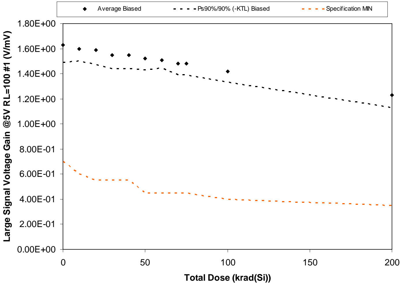
Figure 5.105. Plot of Large Signal Voltage Gain @5V RL=100 #1 (V/mV) versus total dose. The solid diamonds are the average of the measured data points for the samples irradiated under electrical bias and the black lines (solid and/or dashed) are the average of the data points after application of the KTL statistics on the samples irradiated under electrical bias. The red dotted line(s) are the pre- and/or post-irradiation minimum and/or maximum specification value as defined in the datasheet and/or test plan.
