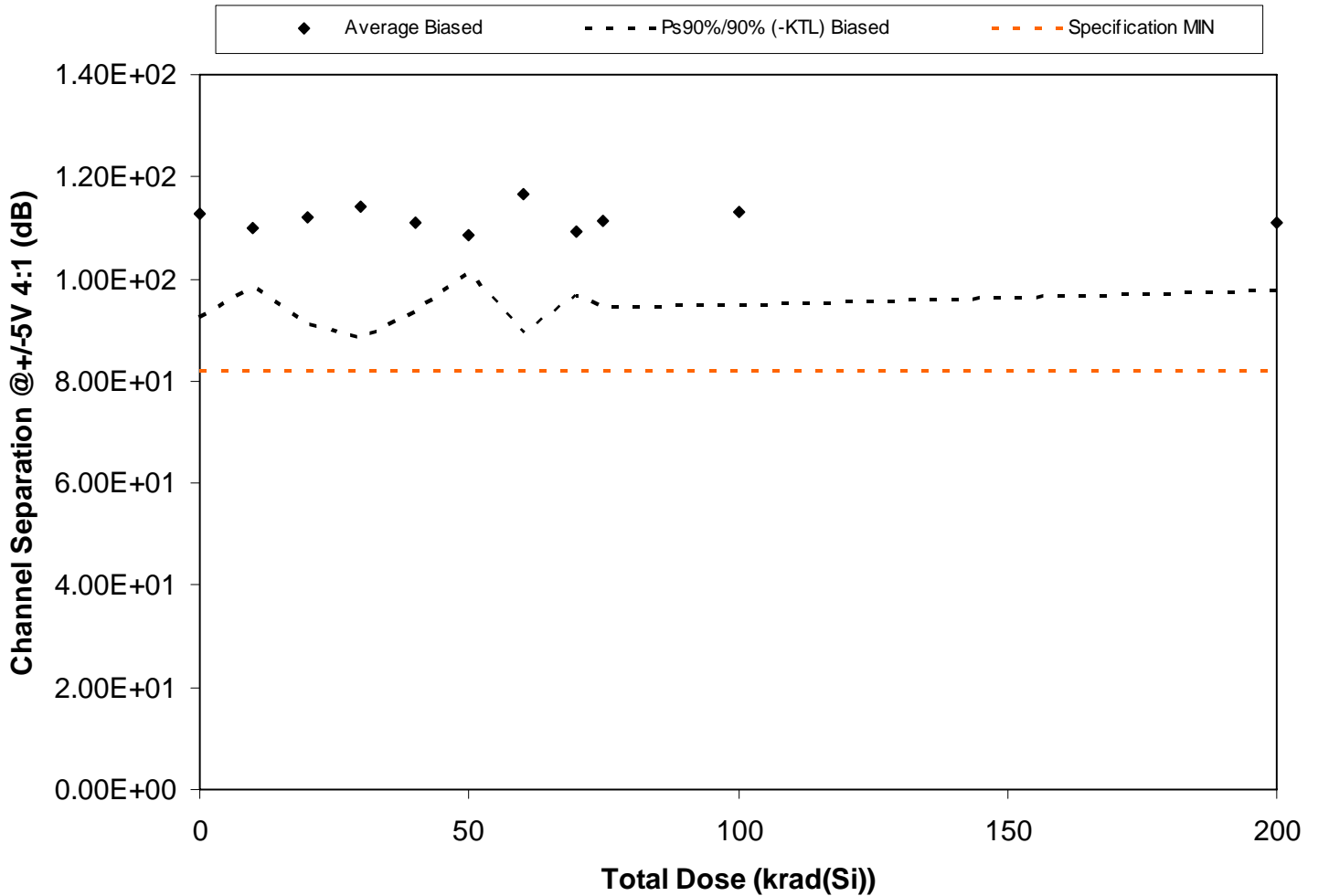
Figure 5.44. Plot of Channel Separation @ +/-5V 4:1 (dB) versus total dose. The solid diamonds are the average of the measured data points for the samples irradiated under electrical bias and the black lines (solid and/or dashed) are the average of the data points after application of the KTL statistics on the samples irradiated under electrical bias. The red dotted line(s) are the pre- and/or post-irradiation minimum and/or maximum specification value as defined in the datasheet and/or test plan.
