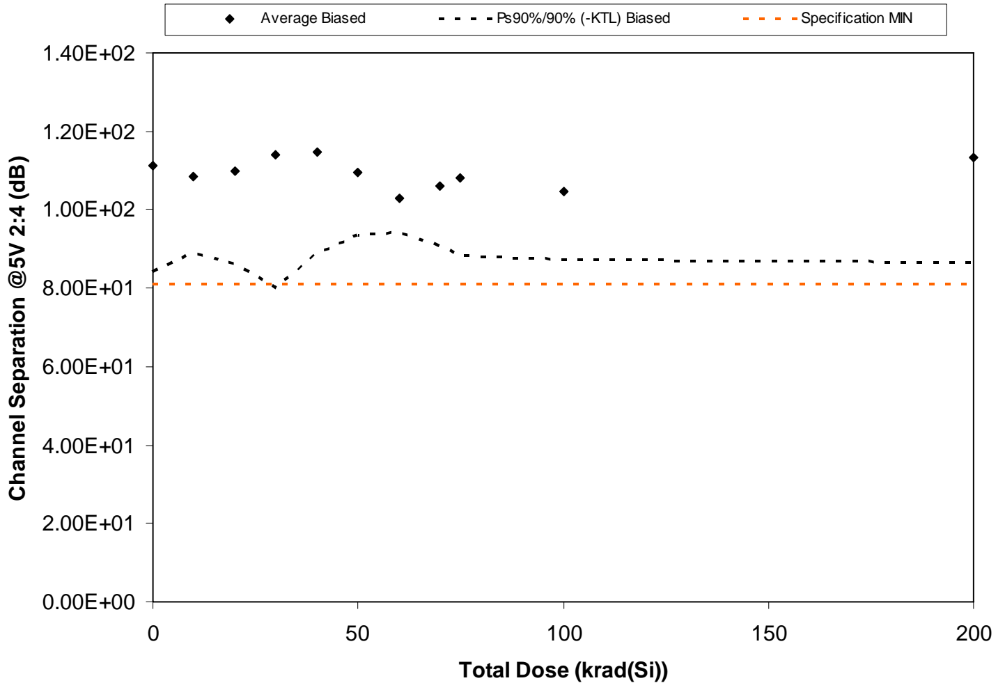
Figure 5.114. Plot of Channel Separation @5V 2:4 (dB) versus total dose. The solid diamonds are the average of the measured data points for the samples irradiated under electrical bias and the black lines (solid and/or dashed) are the average of the data points after application of the KTL statistics on the samples irradiated under electrical bias. The red dotted line(s) are the pre- and/or post-irradiation minimum and/or maximum specification value as defined in the datasheet and/or test plan.
