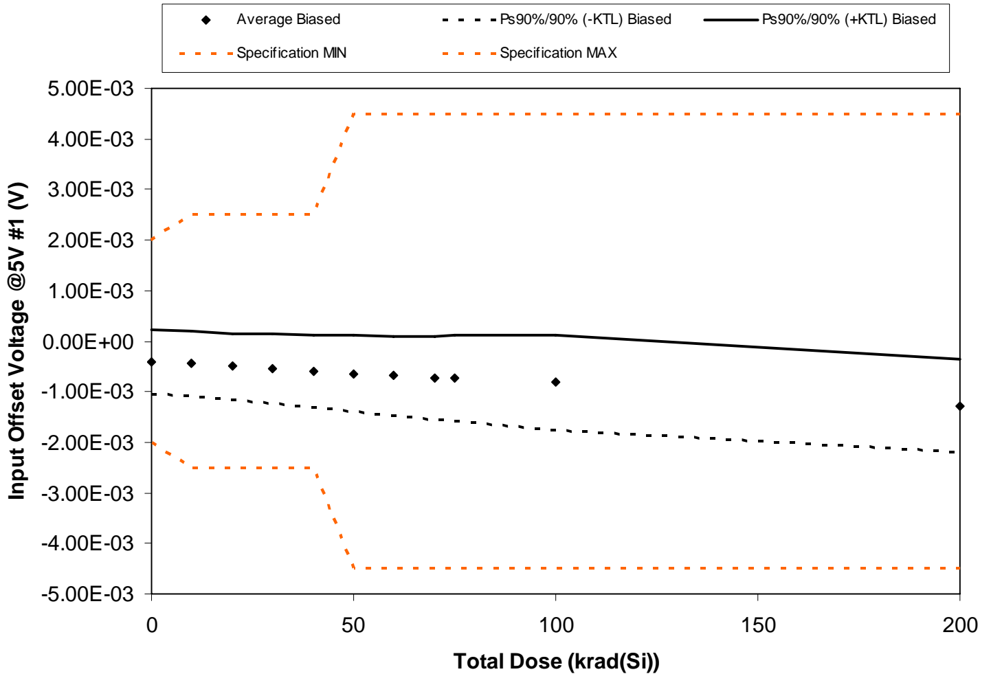
Figure 5.81. Plot of Input Offset Voltage @5V #1 (V) versus total dose. The solid diamonds are the average of the measured data points for the samples irradiated under electrical bias and the black lines (solid and/or dashed) are the average of the data points after application of the KTL statistics on the samples irradiated under electrical bias. The red dotted line(s) are the pre- and/or post-irradiation minimum and/or maximum specification value as defined in the datasheet and/or test plan.
