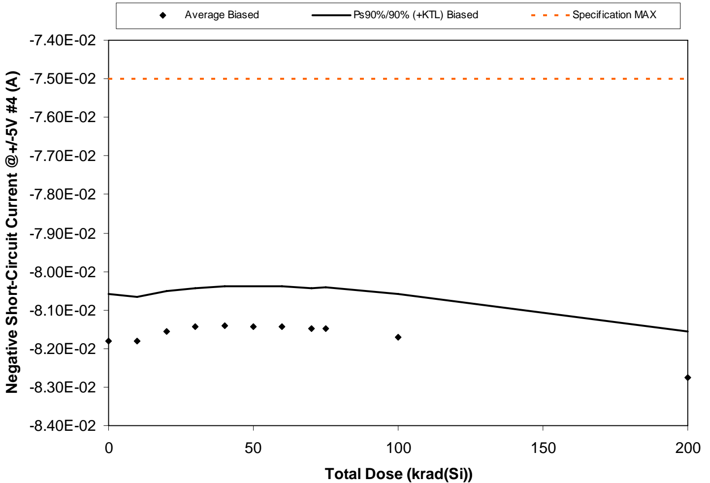
Figure 5.78. Plot of Negative Short-Circuit Current @ +/-5V #4 (A) versus total dose. The solid diamonds are the average of the measured data points for the samples irradiated under electrical bias and the black lines (solid and/or dashed) are the average of the data points after application of the KTL statistics on the samples irradiated under electrical bias. The red dotted line(s) are the pre- and/or post-irradiation minimum and/or maximum specification value as defined in the datasheet and/or test plan.
