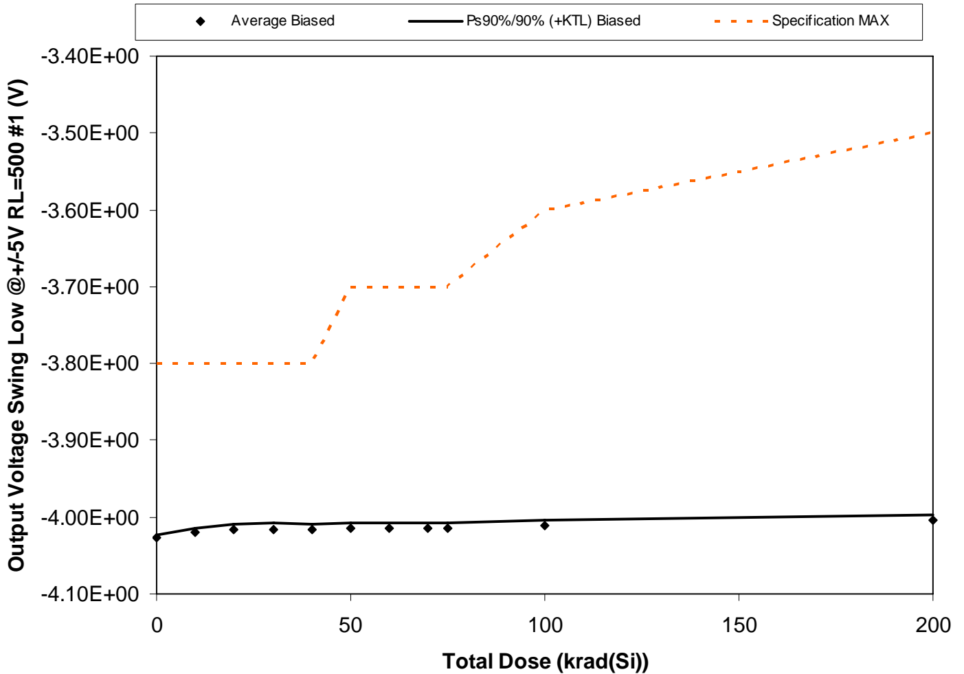
Figure 5.55. Plot of Output Voltage Swing Low @ +/-5V RL=500 #1 (V) versus total dose. The solid diamonds are the average of the measured data points for the samples irradiated under electrical bias and the black lines (solid and/or dashed) are the average of the data points after application of the KTL statistics on the samples irradiated under electrical bias. The red dotted line(s) are the pre- and/or post-irradiation minimum and/or maximum specification value as defined in the datasheet and/or test plan.
