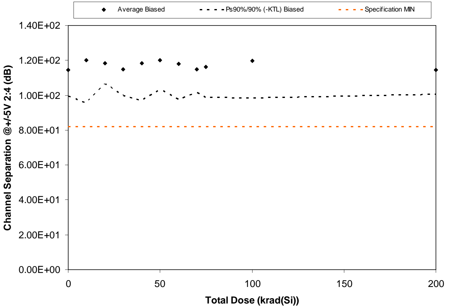
Figure 5.40. Plot of Channel Separation @ +/-5V 2:4 (dB) versus total dose. The solid diamonds are the average of the measured data points for the samples irradiated under electrical bias and the black lines (solid and/or dashed) are the average of the data points after application of the KTL statistics on the samples irradiated under electrical bias. The red dotted line(s) are the pre- and/or post-irradiation minimum and/or maximum specification value as defined in the datasheet and/or test plan.
