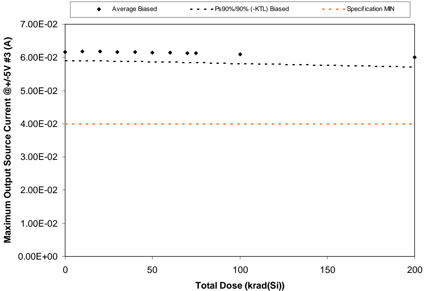
Figure 5.65. Plot of Maximum Output Source Current @ +/-5V #3 (A) versus total dose. The solid diamonds are the average of the measured data points for the samples irradiated under electrical bias and the black lines (solid and/or dashed) are the average of the data points after application of the KTL statistics on the samples irradiated under electrical bias. The red dotted line(s) are the pre- and/or post-irradiation minimum and/or maximum specification value as defined in the datasheet and/or test plan.
