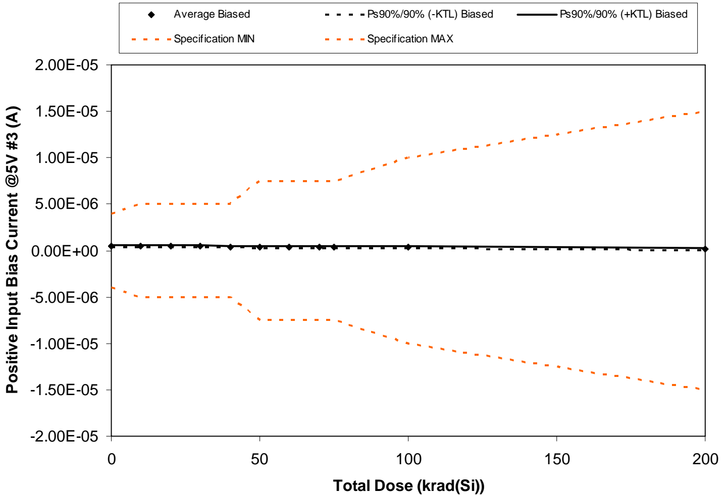
Figure 5.91. Plot of Positive Input Bias Current @5V #3 (A) versus total dose. The solid diamonds are the average of the measured data points for the samples irradiated under electrical bias and the black lines (solid and/or dashed) are the average of the data points after application of the KTL statistics on the samples irradiated under electrical bias. The red dotted line(s) are the pre- and/or post-irradiation minimum and/or maximum specification value as defined in the datasheet and/or test plan.
