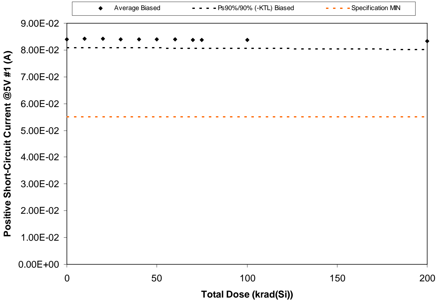
Figure 5.145. Plot of Positive Short-Circuit Current @5V #1 (A) versus total dose. The solid diamonds are the average of the measured data points for the samples irradiated under electrical bias and the black lines (solid and/or dashed) are the average of the data points after application of the KTL statistics on the samples irradiated under electrical bias. The red dotted line(s) are the pre- and/or post-irradiation minimum and/or maximum specification value as defined in the datasheet and/or test plan.
