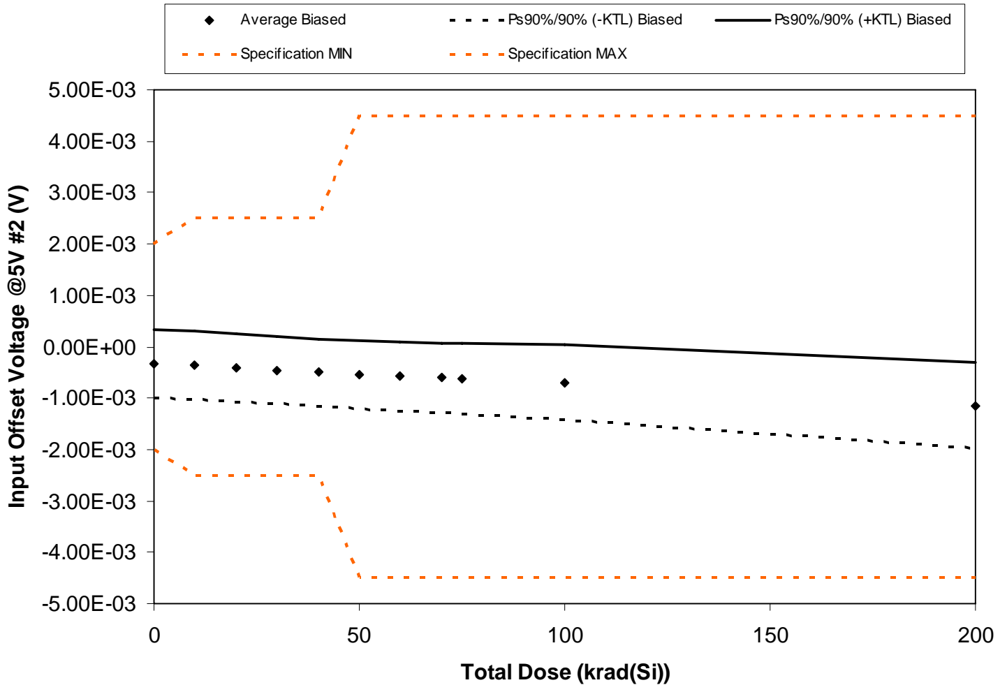
Figure 5.82. Plot of Input Offset Voltage @5V #2 (V) versus total dose. The solid diamonds are the average of the measured data points for the samples irradiated under electrical bias and the black lines (solid and/or dashed) are the average of the data points after application of the KTL statistics on the samples irradiated under electrical bias. The red dotted line(s) are the pre- and/or post-irradiation minimum and/or maximum specification value as defined in the datasheet and/or test plan.
