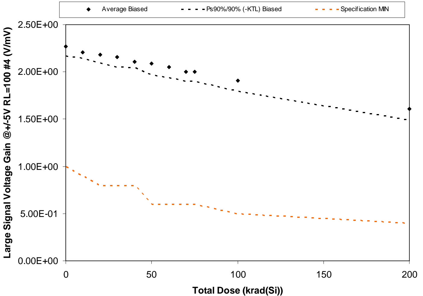
Figure 5.34. Plot of Large Signal Voltage Gain @ +/-5V RL=100 #4 (V/mV) versus total dose. The solid diamonds are the average of the measured data points for the samples irradiated under electrical bias and the black lines (solid and/or dashed) are the average of the data points after application of the KTL statistics on the samples irradiated under electrical bias. The red dotted line(s) are the pre- and/or post-irradiation minimum and/or maximum specification value as defined in the datasheet and/or test plan.
