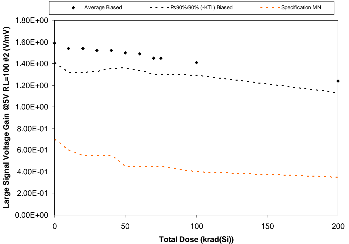
Figure 5.106. Plot of Large Signal Voltage Gain @5V RL=100 #2 (V/mV) versus total dose. The solid diamonds are the average of the measured data points for the samples irradiated under electrical bias and the black lines (solid and/or dashed) are the average of the data points after application of the KTL statistics on the samples irradiated under electrical bias. The red dotted line(s) are the pre- and/or post-irradiation minimum and/or maximum specification value as defined in the datasheet and/or test plan.
