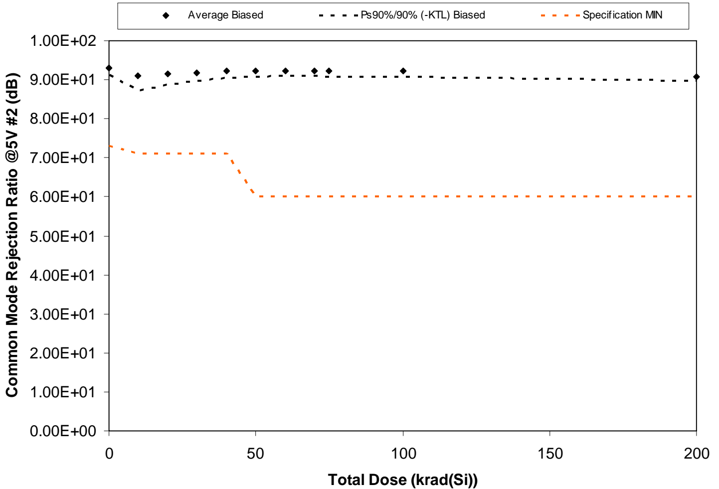
Figure 5.98. Plot of Common Mode Rejection Ratio @5V #2 (dB) versus total dose. The solid diamonds are the average of the measured data points for the samples irradiated under electrical bias and the black lines (solid and/or dashed) are the average of the data points after application of the KTL statistics on the samples irradiated under electrical bias. The red dotted line(s) are the pre- and/or post-irradiation minimum and/or maximum specification value as defined in the datasheet and/or test plan.
