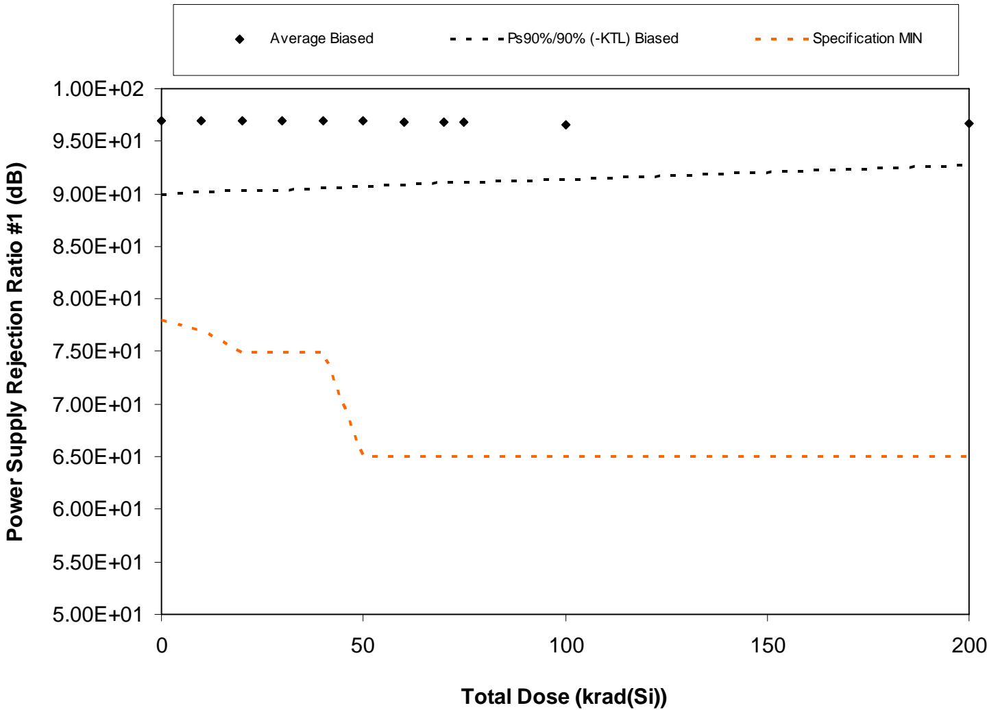
Figure 5.23. Plot of Power Supply Rejection Ratio #1 (dB) versus total dose. The solid diamonds are the average of the measured data points for the samples irradiated under electrical bias and the black lines (solid and/or dashed) are the average of the data points after application of the KTL statistics on the samples irradiated under electrical bias. The red dotted line(s) are the pre- and/or post-irradiation minimum and/or maximum specification value as defined in the datasheet and/or test plan.
