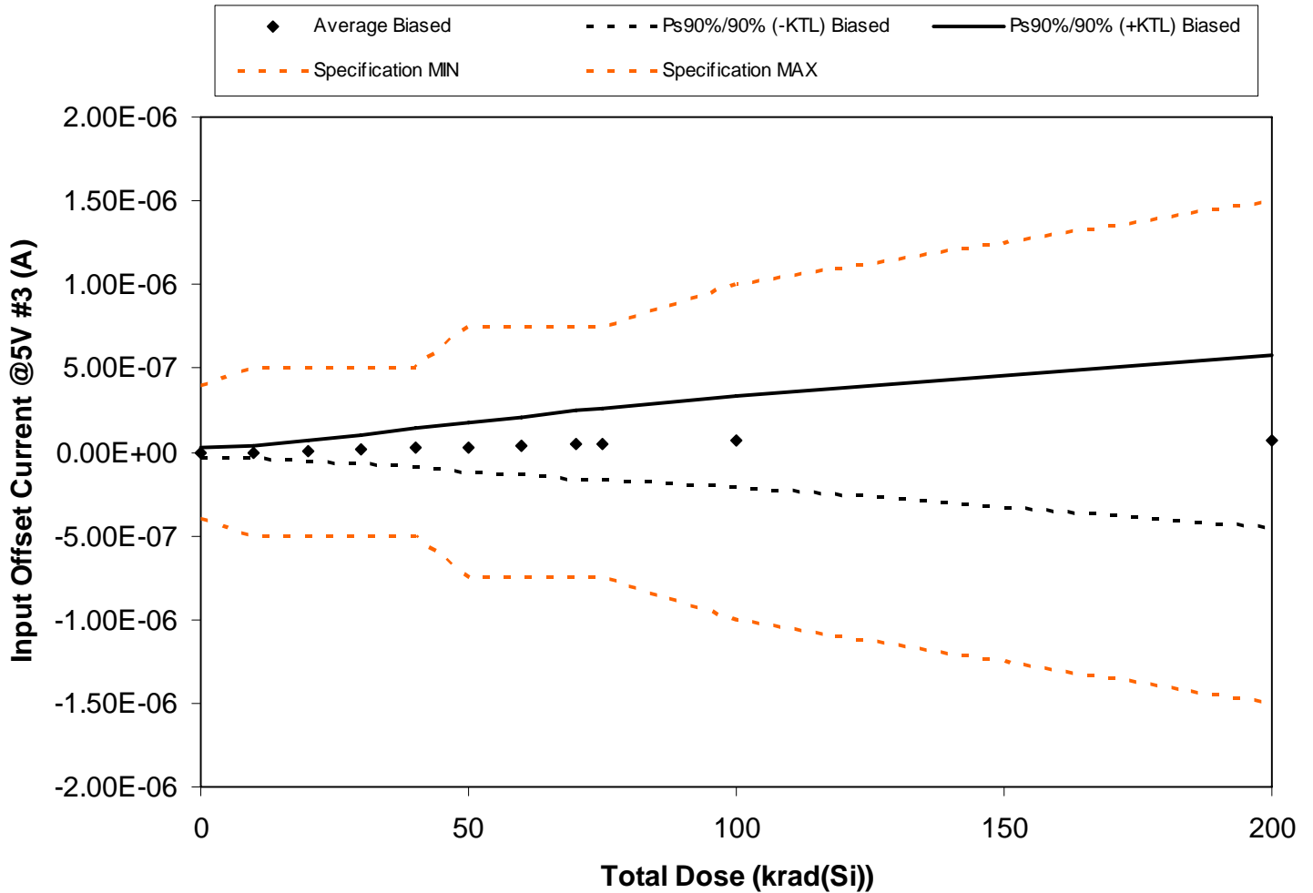
Figure 5.87. Plot of Input Offset Current @5V #3 (A) versus total dose. The solid diamonds are the average of the measured data points for the samples irradiated under electrical bias and the black lines (solid and/or dashed) are the average of the data points after application of the KTL statistics on the samples irradiated under electrical bias. The red dotted line(s) are the pre- and/or post-irradiation minimum and/or maximum specification value as defined in the datasheet and/or test plan.
