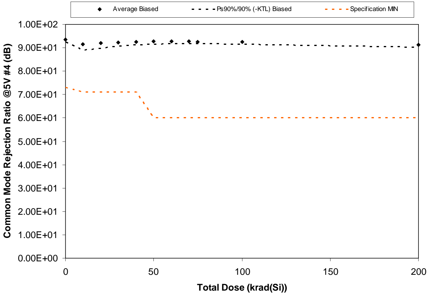
Figure 5.100. Plot of Common Mode Rejection Ratio @5V #4 (dB) versus total dose. The solid diamonds are the average of the measured data points for the samples irradiated under electrical bias and the black lines (solid and/or dashed) are the average of the data points after application of the KTL statistics on the samples irradiated under electrical bias. The red dotted line(s) are the pre- and/or post-irradiation minimum and/or maximum specification value as defined in the datasheet and/or test plan.
