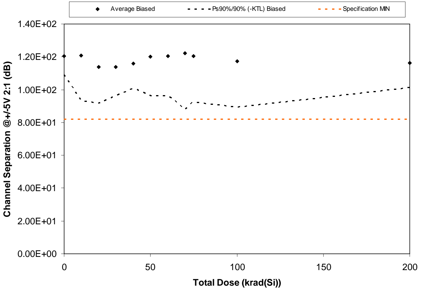
Figure 5.38. Plot of Channel Separation @ +/-5V 2:1 (dB) versus total dose. The solid diamonds are the average of the measured data points for the samples irradiated under electrical bias and the black lines (solid and/or dashed) are the average of the data points after application of the KTL statistics on the samples irradiated under electrical bias. The red dotted line(s) are the pre- and/or post-irradiation minimum and/or maximum specification value as defined in the datasheet and/or test plan.
