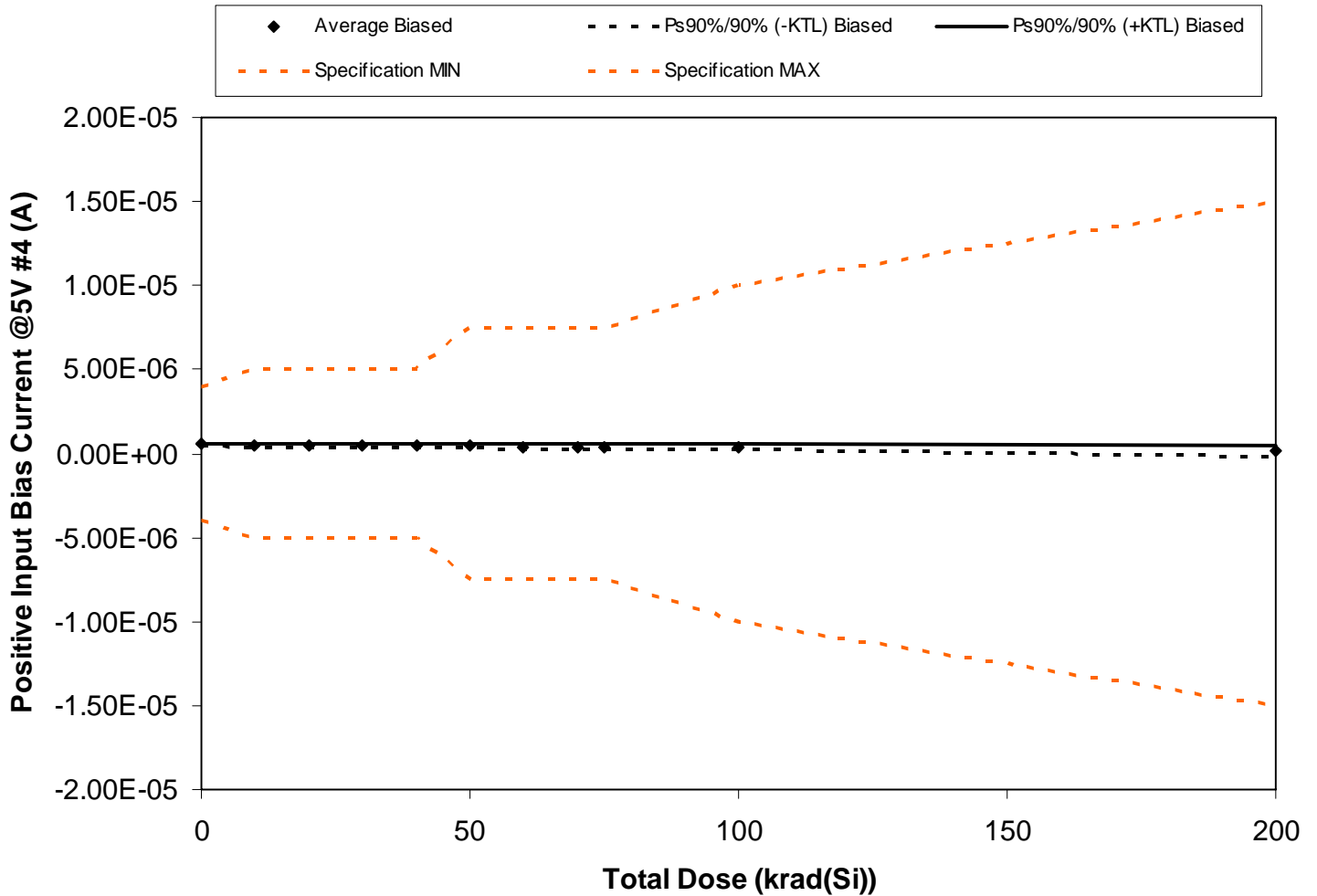
Figure 5.92. Plot of Positive Input Bias Current @5V #4 (A) versus total dose. The solid diamonds are the average of the measured data points for the samples irradiated under electrical bias and the black lines (solid and/or dashed) are the average of the data points after application of the KTL statistics on the samples irradiated under electrical bias. The red dotted line(s) are the pre- and/or post-irradiation minimum and/or maximum specification value as defined in the datasheet and/or test plan.
