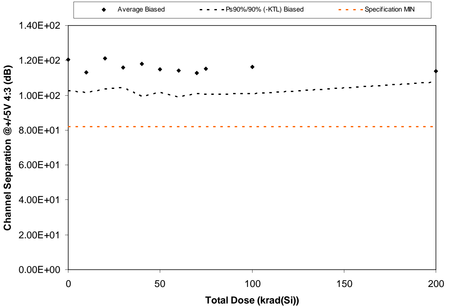
Figure 5.46. Plot of Channel Separation @ +/-5V 4:3 (dB) versus total dose. The solid diamonds are the average of the measured data points for the samples irradiated under electrical bias and the black lines (solid and/or dashed) are the average of the data points after application of the KTL statistics on the samples irradiated under electrical bias. The red dotted line(s) are the pre- and/or post-irradiation minimum and/or maximum specification value as defined in the datasheet and/or test plan.
