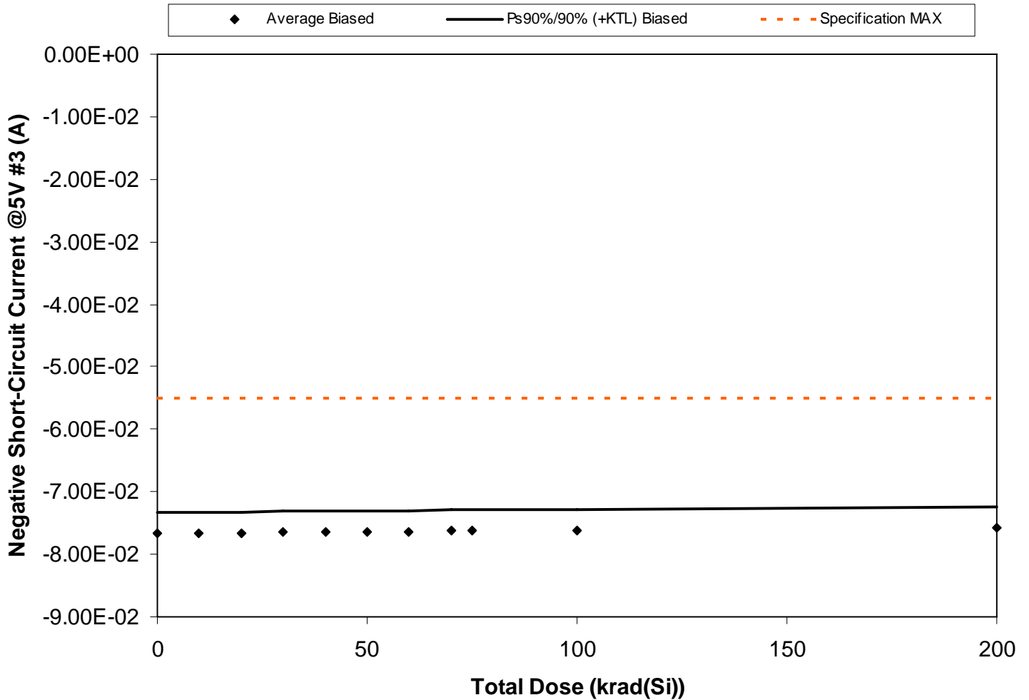
Figure 5.151. Plot of Negative Short-Circuit Current @5V #3 (A) versus total dose. The solid diamonds are the average of the measured data points for the samples irradiated under electrical bias and the black lines (solid and/or dashed) are the average of the data points after application of the KTL statistics on the samples irradiated under electrical bias. The red dotted line(s) are the pre- and/or post-irradiation minimum and/or maximum specification value as defined in the datasheet and/or test plan.
