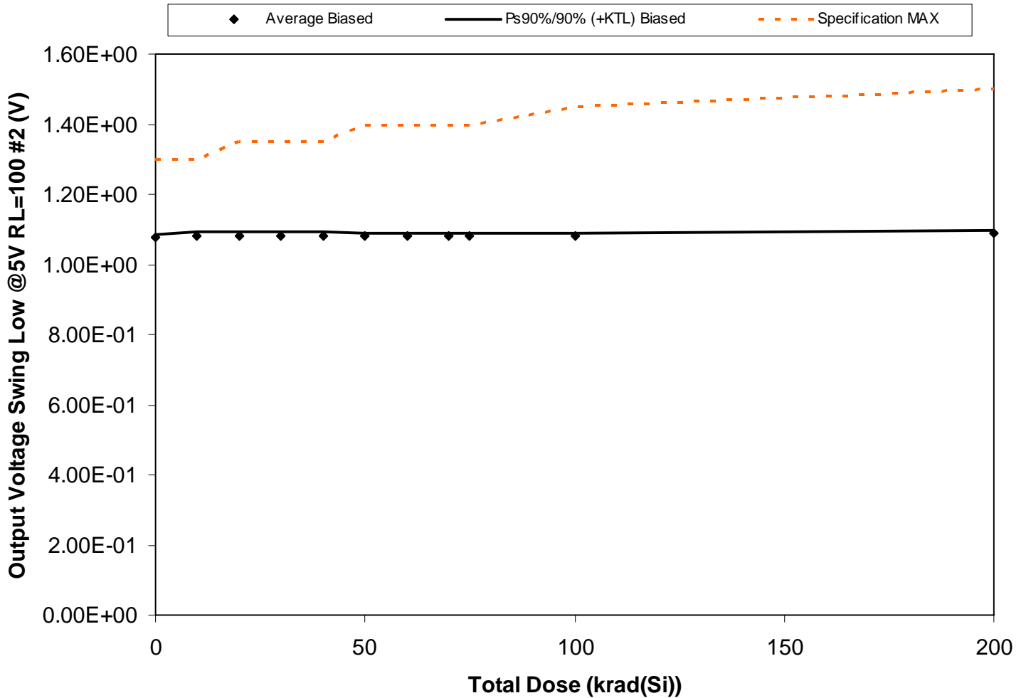
Figure 5.134. Plot of Output Voltage Swing Low @5V RL=100 #2 (V) versus total dose. The solid diamonds are the average of the measured data points for the samples irradiated under electrical bias and the black lines (solid and/or dashed) are the average of the data points after application of the KTL statistics on the samples irradiated under electrical bias. The red dotted line(s) are the pre- and/or post-irradiation minimum and/or maximum specification value as defined in the datasheet and/or test plan.
