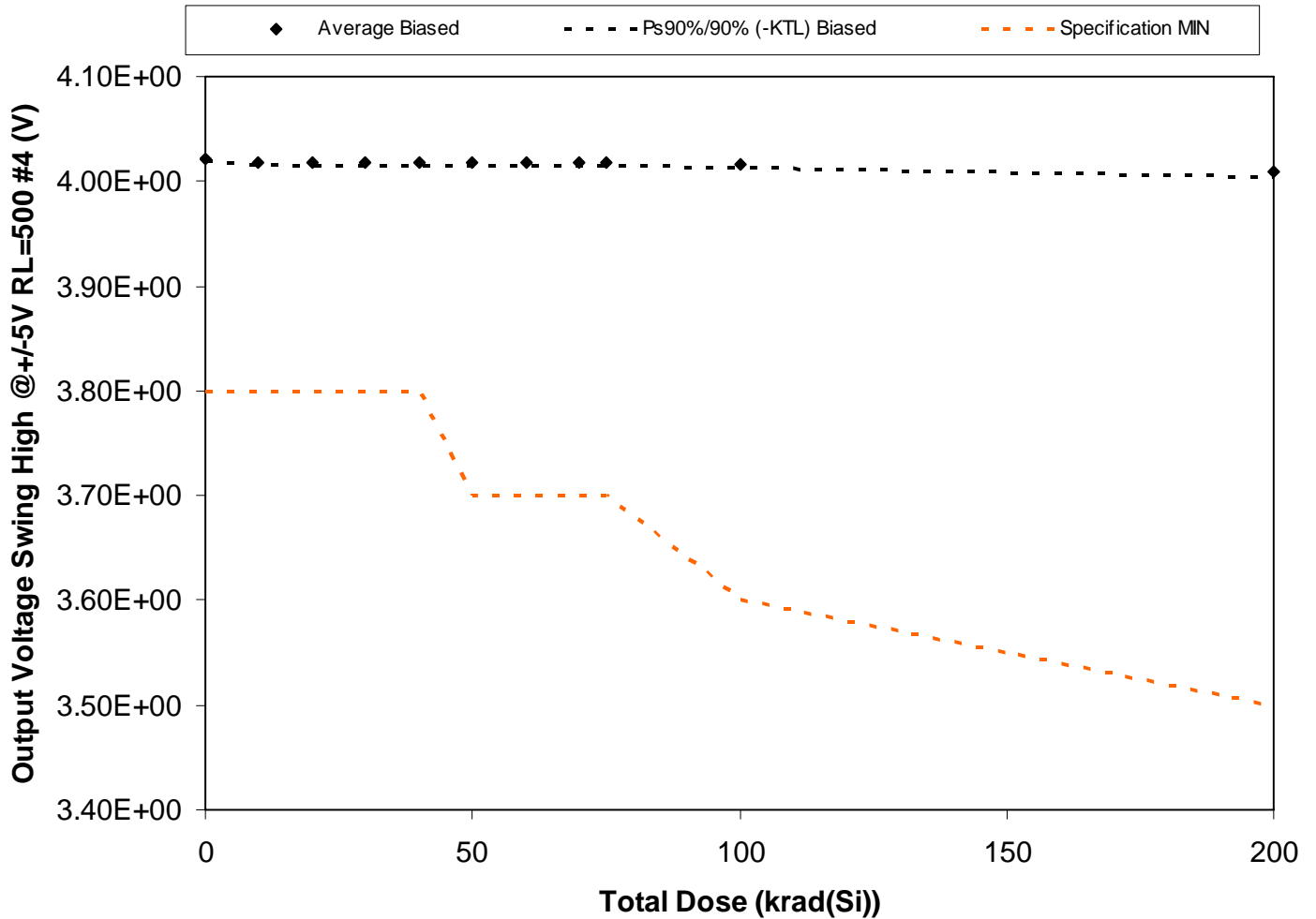
Figure 5.50. Plot of Output Voltage Swing High @ +/-5V RL=500 #4 (V) versus total dose. The solid diamonds are the average of the measured data points for the samples irradiated under electrical bias and the black lines (solid and/or dashed) are the average of the data points after application of the KTL statistics on the samples irradiated under electrical bias. The red dotted line(s) are the pre- and/or post-irradiation minimum and/or maximum specification value as defined in the datasheet and/or test plan.
