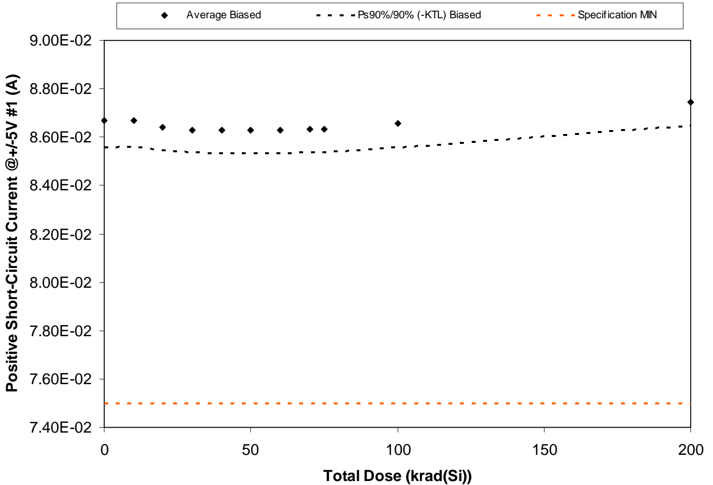
Figure 5.71. Plot of Positive Short-Circuit Current @ +/-5V #1 (A) versus total dose. The solid diamonds are the average of the measured data points for the samples irradiated under electrical bias and the black lines (solid and/or dashed) are the average of the data points after application of the KTL statistics on the samples irradiated under electrical bias. The red dotted line(s) are the pre- and/or post-irradiation minimum and/or maximum specification value as defined in the datasheet and/or test plan.
