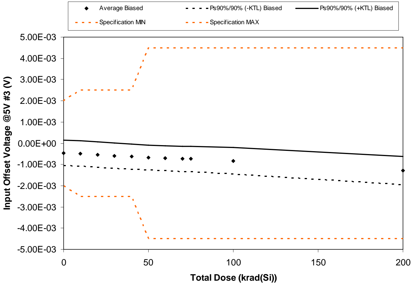
Figure 5.83. Plot of Input Offset Voltage @5V #3 (V) versus total dose. The solid diamonds are the average of the measured data points for the samples irradiated under electrical bias and the black lines (solid and/or dashed) are the average of the data points after application of the KTL statistics on the samples irradiated under electrical bias. The red dotted line(s) are the pre- and/or post-irradiation minimum and/or maximum specification value as defined in the datasheet and/or test plan.
