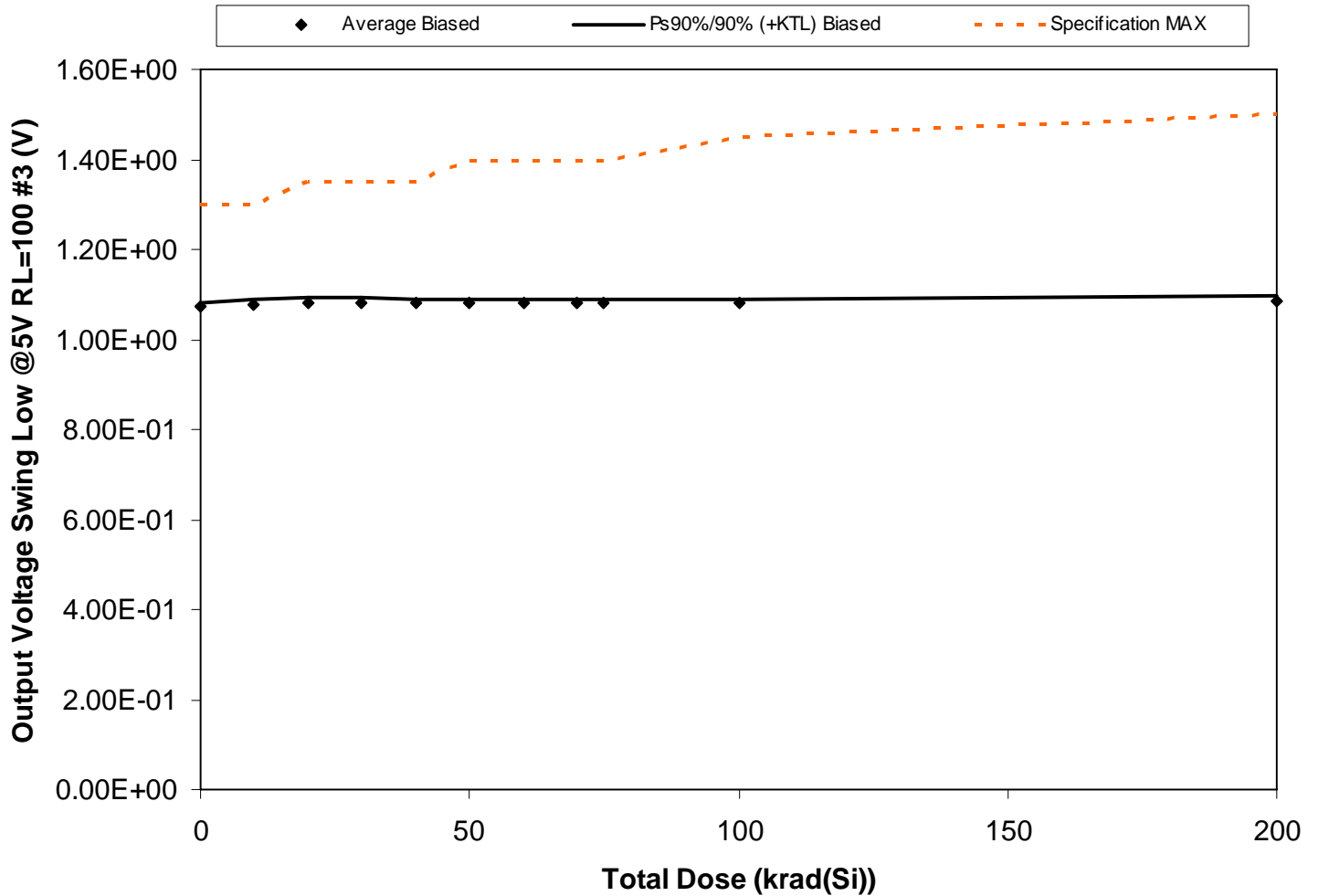
Figure 5.135. Plot of Output Voltage Swing Low @5V RL=100 #3 (V) versus total dose. The solid diamonds are the average of the measured data points for the samples irradiated under electrical bias and the black lines (solid and/or dashed) are the average of the data points after application of the KTL statistics on the samples irradiated under electrical bias. The red dotted line(s) are the pre- and/or post-irradiation minimum and/or maximum specification value as defined in the datasheet and/or test plan.
