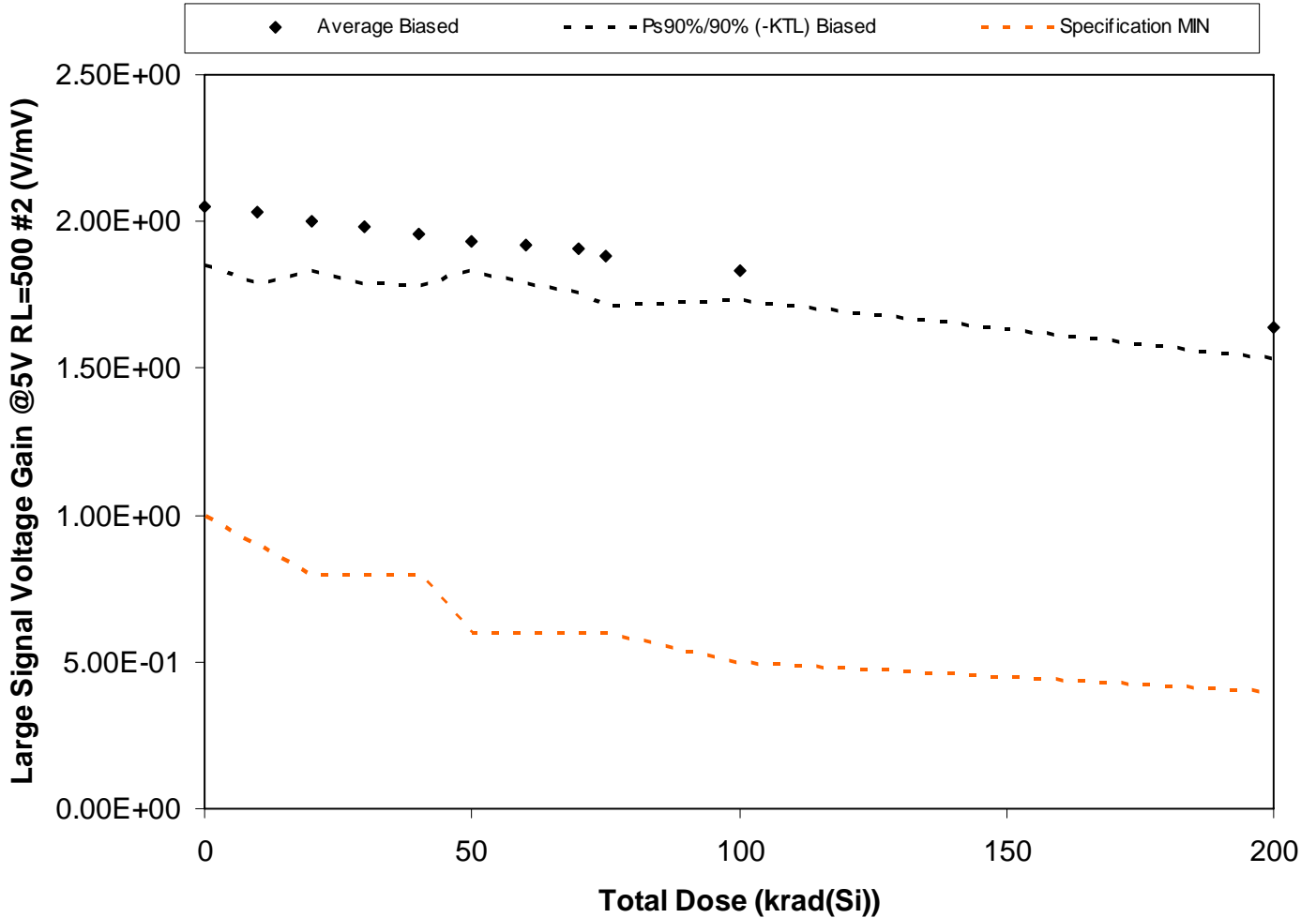
Figure 5.102. Plot of Large Signal Voltage Gain @5V RL=500 #2 (V/mV) versus total dose. The solid diamonds are the average of the measured data points for the samples irradiated under electrical bias and the black lines (solid and/or dashed) are the average of the data points after application of the KTL statistics on the samples irradiated under electrical bias. The red dotted line(s) are the pre- and/or post-irradiation minimum and/or maximum specification value as defined in the datasheet and/or test plan.
