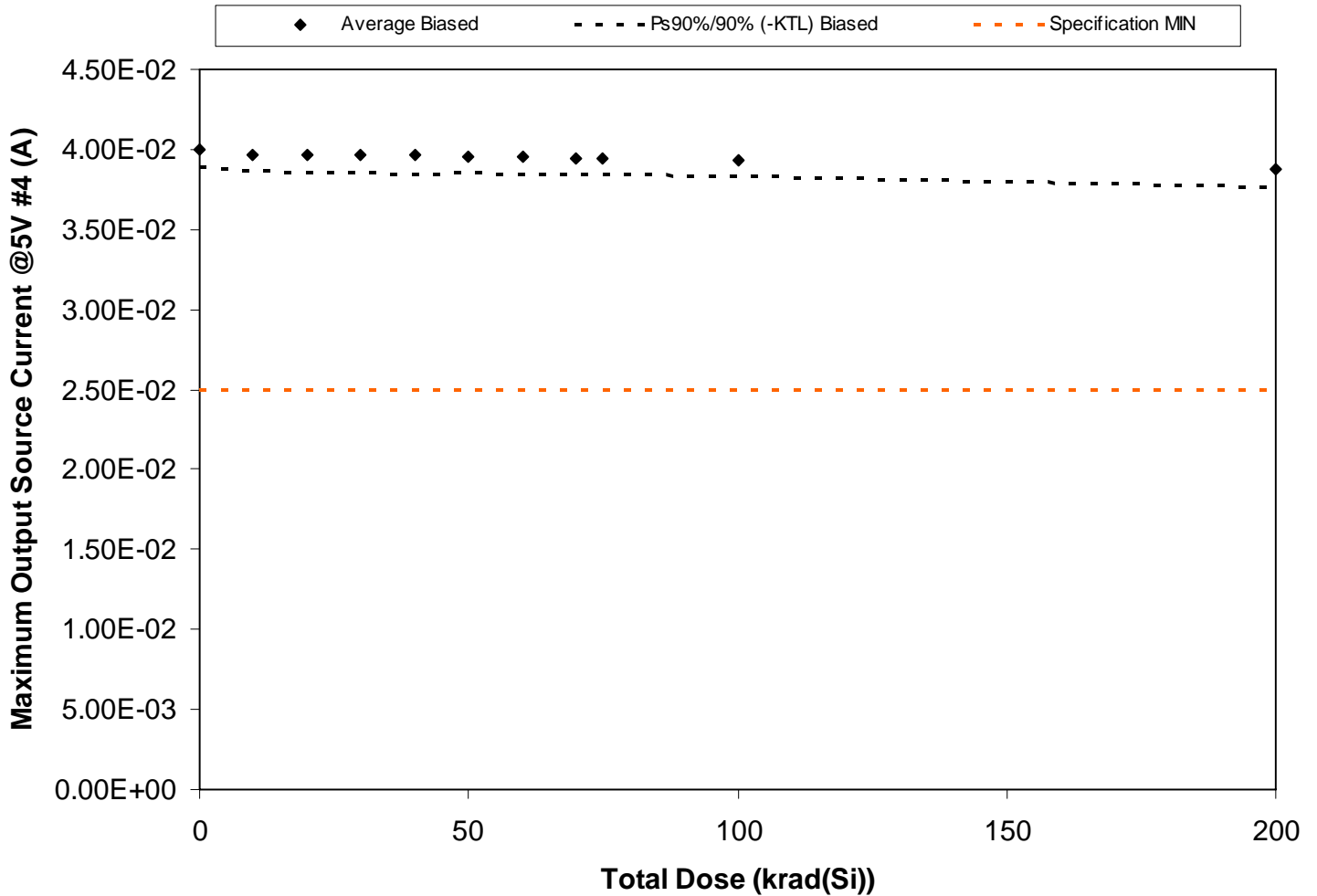
Figure 5.140. Plot of Maximum Output Source Current @5V #4 (A) versus total dose. The solid diamonds are the average of the measured data points for the samples irradiated under electrical bias and the black lines (solid and/or dashed) are the average of the data points after application of the KTL statistics on the samples irradiated under electrical bias. The red dotted line(s) are the pre- and/or post-irradiation minimum and/or maximum specification value as defined in the datasheet and/or test plan.
