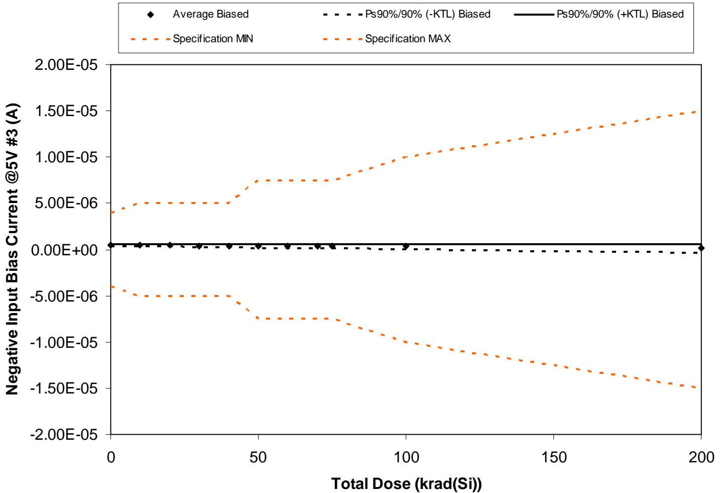
Figure 5.95. Plot of Negative Input Bias Current @5V #3 (A) versus total dose. The solid diamonds are the average of the measured data points for the samples irradiated under electrical bias and the black lines (solid and/or dashed) are the average of the data points after application of the KTL statistics on the samples irradiated under electrical bias. The red dotted line(s) are the pre- and/or post-irradiation minimum and/or maximum specification value as defined in the datasheet and/or test plan.
