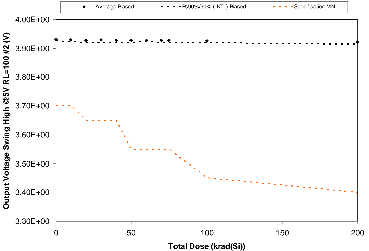
Figure 5.126. Plot of Output Voltage Swing High @5V RL=100 #2 (V) versus total dose. The solid diamonds are the average of the measured data points for the samples irradiated under electrical bias and the black lines (solid and/or dashed) are the average of the data points after application of the KTL statistics on the samples irradiated under electrical bias. The red dotted line(s) are the pre- and/or post-irradiation minimum and/or maximum specification value as defined in the datasheet and/or test plan.
