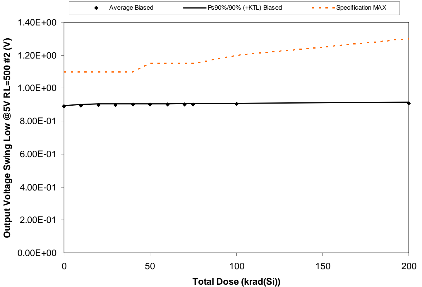
Figure 5.130. Plot of Output Voltage Swing Low @5V RL=500 #2 (V) versus total dose. The solid diamonds are the average of the measured data points for the samples irradiated under electrical bias and the black lines (solid and/or dashed) are the average of the data points after application of the KTL statistics on the samples irradiated under electrical bias. The red dotted line(s) are the pre- and/or post-irradiation minimum and/or maximum specification value as defined in the datasheet and/or test plan.
