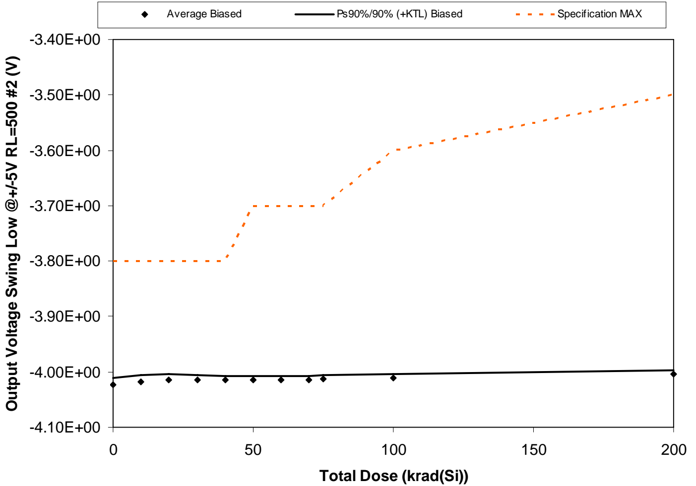
Figure 5.56. Plot of Output Voltage Swing Low @ +/-5V RL=500 #2 (V) versus total dose. The solid diamonds are the average of the measured data points for the samples irradiated under electrical bias and the black lines (solid and/or dashed) are the average of the data points after application of the KTL statistics on the samples irradiated under electrical bias. The red dotted line(s) are the pre- and/or post-irradiation minimum and/or maximum specification value as defined in the datasheet and/or test plan.
