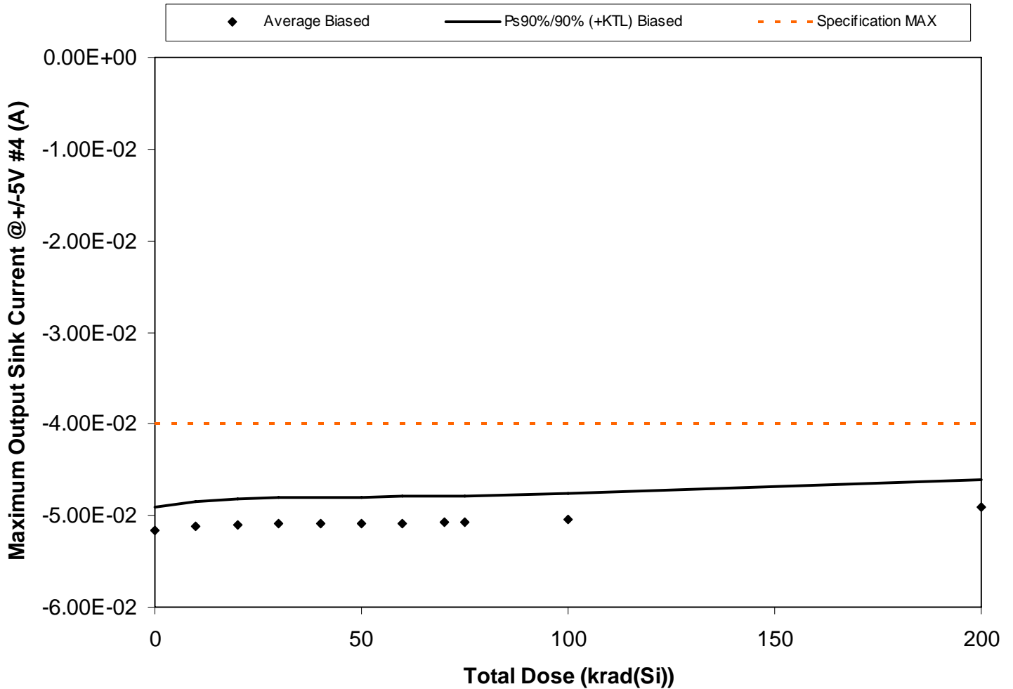
Figure 5.70. Plot of Maximum Output Sink Current @ +/-5V #4 (A) versus total dose. The solid diamonds are the average of the measured data points for the samples irradiated under electrical bias and the black lines (solid and/or dashed) are the average of the data points after application of the KTL statistics on the samples irradiated under electrical bias. The red dotted line(s) are the pre- and/or post-irradiation minimum and/or maximum specification value as defined in the datasheet and/or test plan.
