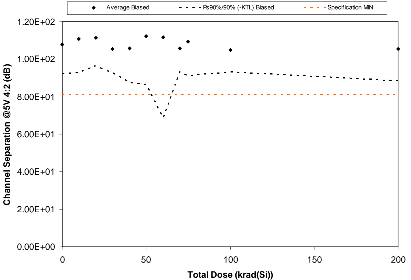
Figure 5.119. Plot of Channel Separation @5V 4:2 (dB) versus total dose. The solid diamonds are the average of the measured data points for the samples irradiated under electrical bias and the black lines (solid and/or dashed) are the average of the data points after application of the KTL statistics on the samples irradiated under electrical bias. The red dotted line(s) are the pre- and/or post-irradiation minimum and/or maximum specification value as defined in the datasheet and/or test plan.
