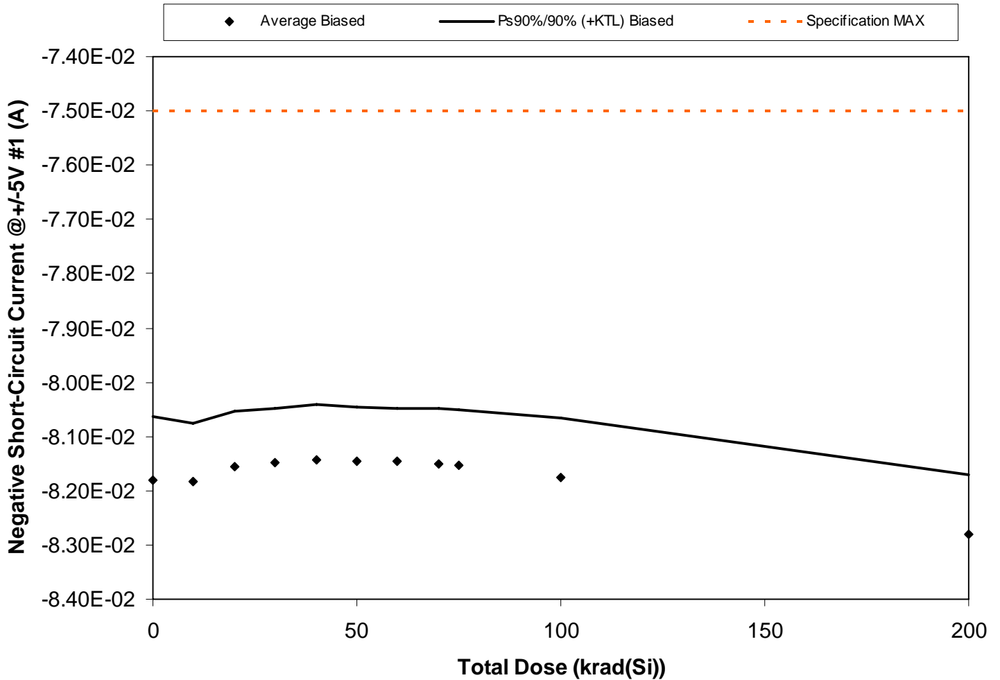
Figure 5.75. Plot of Negative Short-Circuit Current @ +/-5V #1 (A) versus total dose. The solid diamonds are the average of the measured data points for the samples irradiated under electrical bias and the black lines (solid and/or dashed) are the average of the data points after application of the KTL statistics on the samples irradiated under electrical bias. The red dotted line(s) are the pre- and/or post-irradiation minimum and/or maximum specification value as defined in the datasheet and/or test plan.
