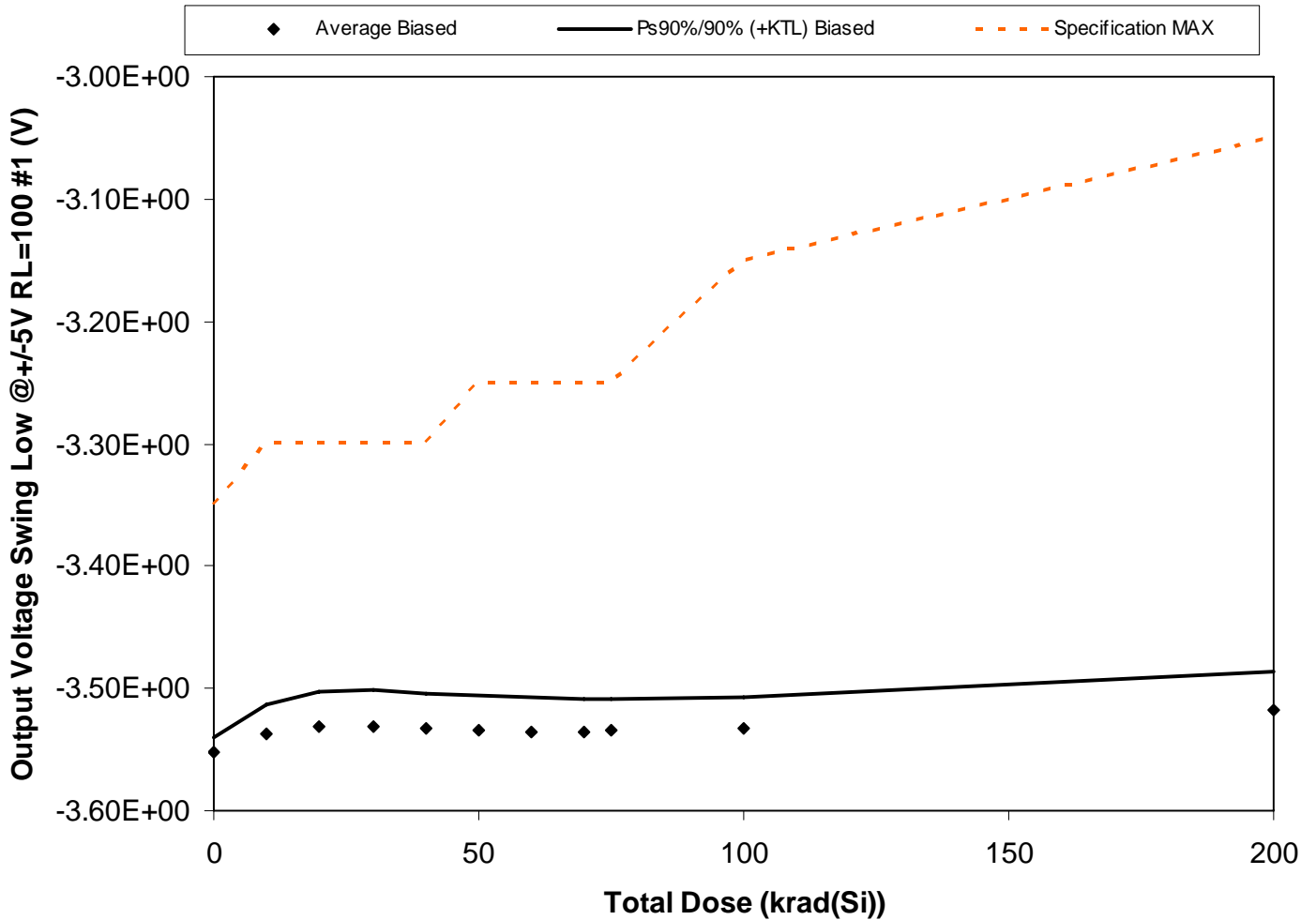
Figure 5.59. Plot of Output Voltage Swing Low @ +/-5V RL=100 #1 (V) versus total dose. The solid diamonds are the average of the measured data points for the samples irradiated under electrical bias and the black lines (solid and/or dashed) are the average of the data points after application of the KTL statistics on the samples irradiated under electrical bias. The red dotted line(s) are the pre- and/or post-irradiation minimum and/or maximum specification value as defined in the datasheet and/or test plan.
