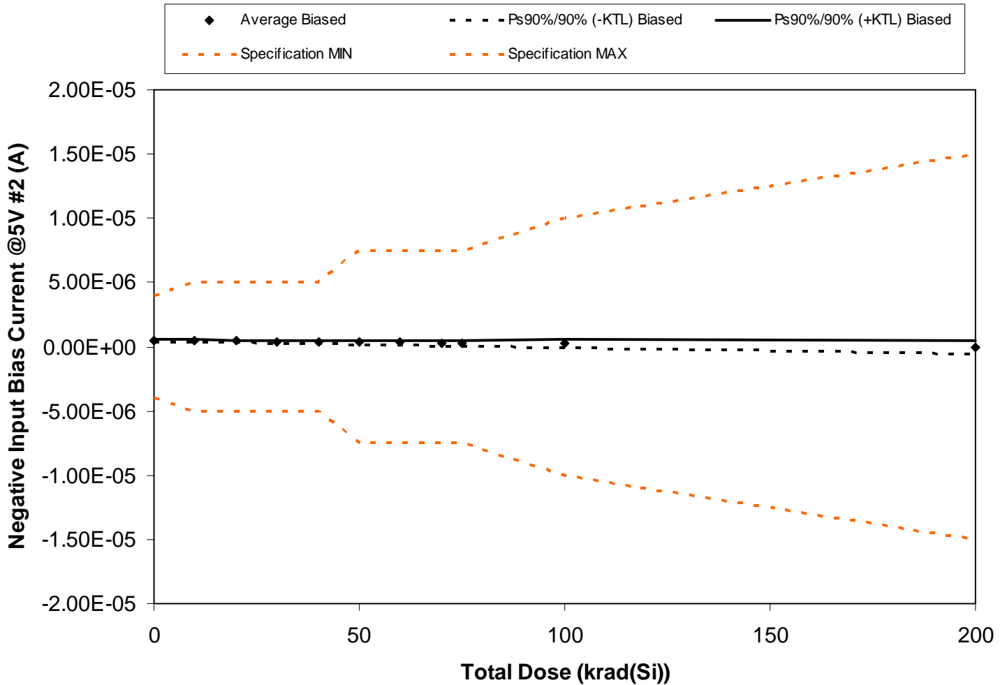
Figure 5.94. Plot of Negative Input Bias Current @5V #2 (A) versus total dose. The solid diamonds are the average of the measured data points for the samples irradiated under electrical bias and the black lines (solid and/or dashed) are the average of the data points after application of the KTL statistics on the samples irradiated under electrical bias. The red dotted line(s) are the pre- and/or post-irradiation minimum and/or maximum specification value as defined in the datasheet and/or test plan.
