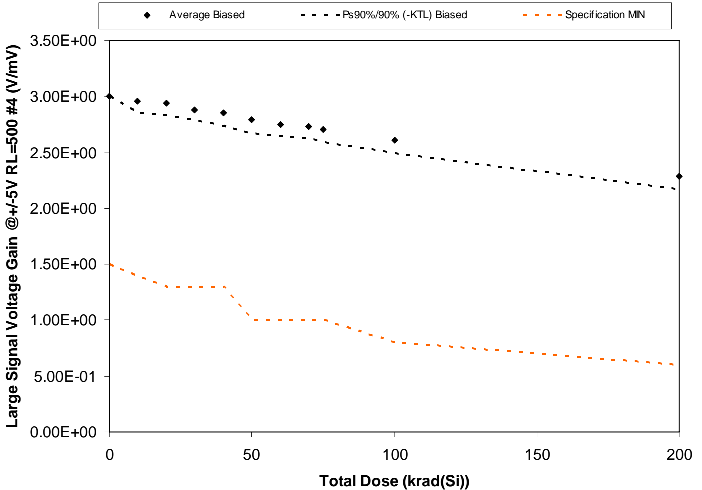
Figure 5.30. Plot of Large Signal Voltage Gain @ +/-5V RL=500 #4 (V/mV) versus total dose. The solid diamonds are the average of the measured data points for the samples irradiated under electrical bias and the black lines (solid and/or dashed) are the average of the data points after application of the KTL statistics on the samples irradiated under electrical bias. The red dotted line(s) are the pre- and/or post-irradiation minimum and/or maximum specification value as defined in the datasheet and/or test plan.
