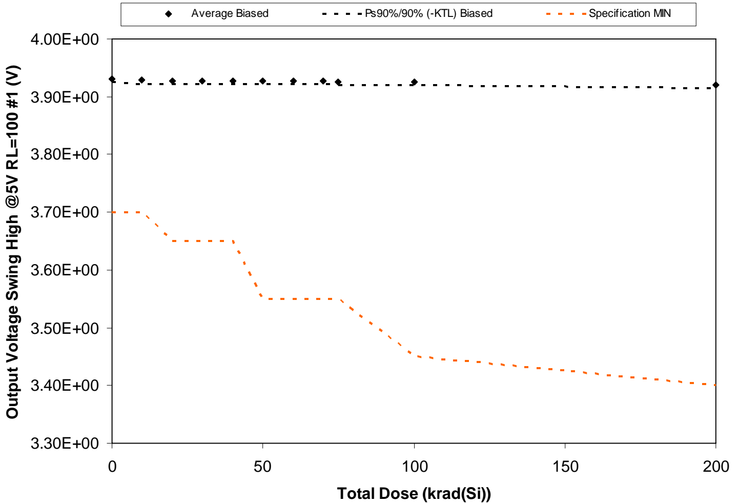
Figure 5.125. Plot of Output Voltage Swing High @5V RL=100 #1 (V) versus total dose. The solid diamonds are the average of the measured data points for the samples irradiated under electrical bias and the black lines (solid and/or dashed) are the average of the data points after application of the KTL statistics on the samples irradiated under electrical bias. The red dotted line(s) are the pre- and/or post-irradiation minimum and/or maximum specification value as defined in the datasheet and/or test plan.
