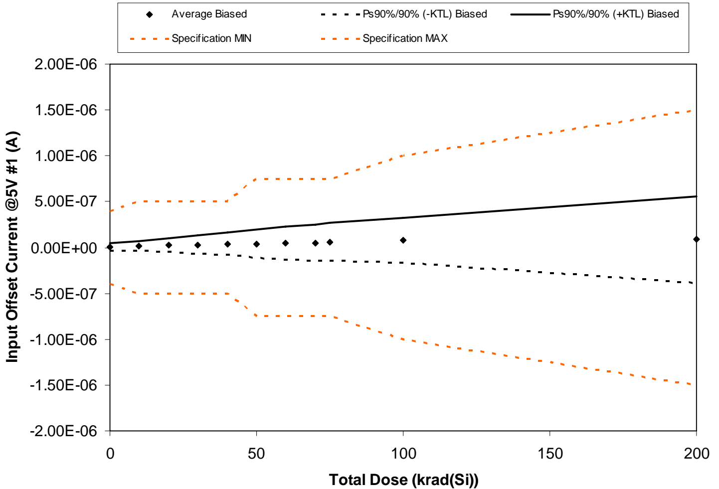
Figure 5.85. Plot of Input Offset Current @5V #1 (A) versus total dose. The solid diamonds are the average of the measured data points for the samples irradiated under electrical bias and the black lines (solid and/or dashed) are the average of the data points after application of the KTL statistics on the samples irradiated under electrical bias. The red dotted line(s) are the pre- and/or post-irradiation minimum and/or maximum specification value as defined in the datasheet and/or test plan.
