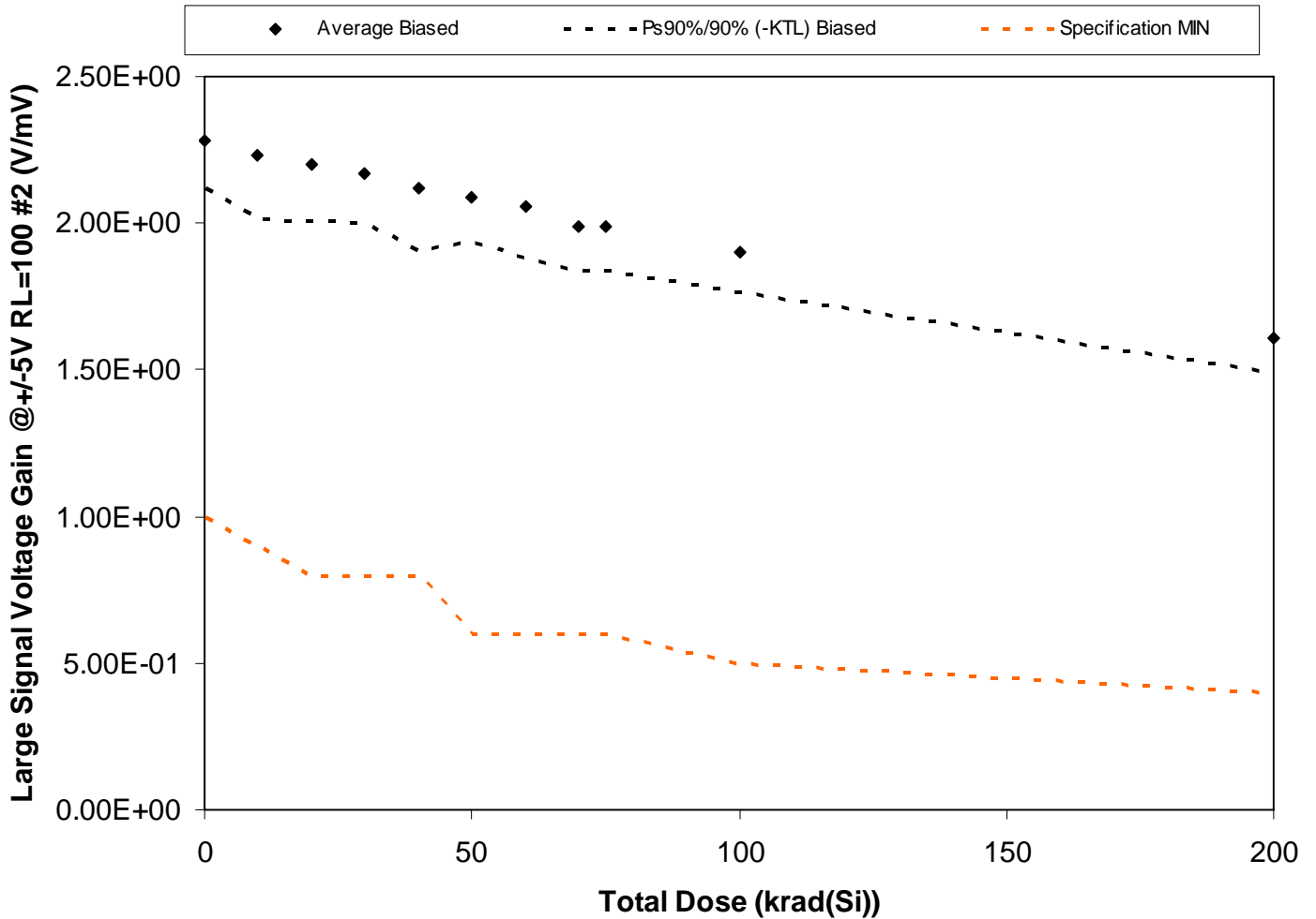
Figure 5.32. Plot of Large Signal Voltage Gain @ +/-5V RL=100 #2 (V/mV) versus total dose. The solid diamonds are the average of the measured data points for the samples irradiated under electrical bias and the black lines (solid and/or dashed) are the average of the data points after application of the KTL statistics on the samples irradiated under electrical bias. The red dotted line(s) are the pre- and/or post-irradiation minimum and/or maximum specification value as defined in the datasheet and/or test plan.
