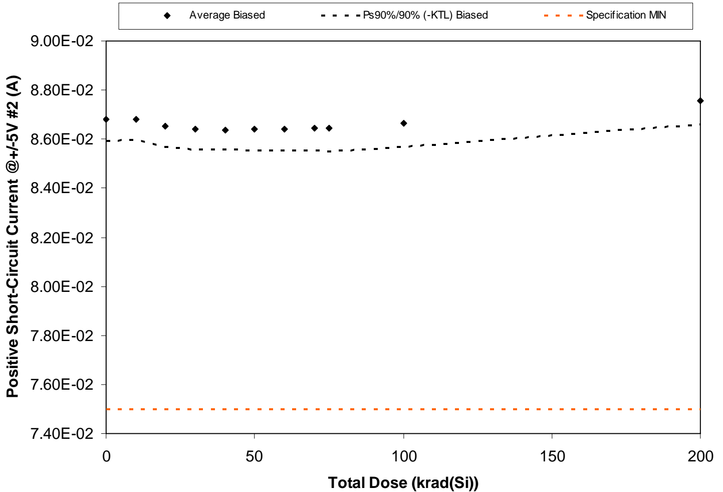
Figure 5.72. Plot of Positive Short-Circuit Current @ +/-5V #2 (A) versus total dose. The solid diamonds are the average of the measured data points for the samples irradiated under electrical bias and the black lines (solid and/or dashed) are the average of the data points after application of the KTL statistics on the samples irradiated under electrical bias. The red dotted line(s) are the pre- and/or post-irradiation minimum and/or maximum specification value as defined in the datasheet and/or test plan.
