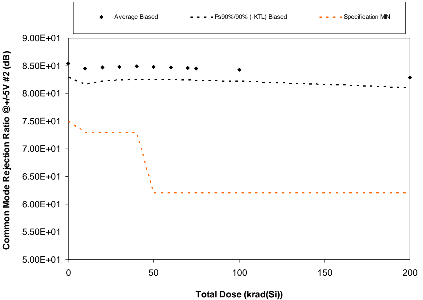
Figure 5.20. Plot of Common Mode Rejection Ratio @ +/-5V #2 (dB) versus total dose. The solid diamonds are the average of the measured data points for the samples irradiated under electrical bias and the black lines (solid and/or dashed) are the average of the data points after application of the KTL statistics on the samples irradiated under electrical bias. The red dotted line(s) are the pre- and/or post-irradiation minimum and/or maximum specification value as defined in the datasheet and/or test plan.
