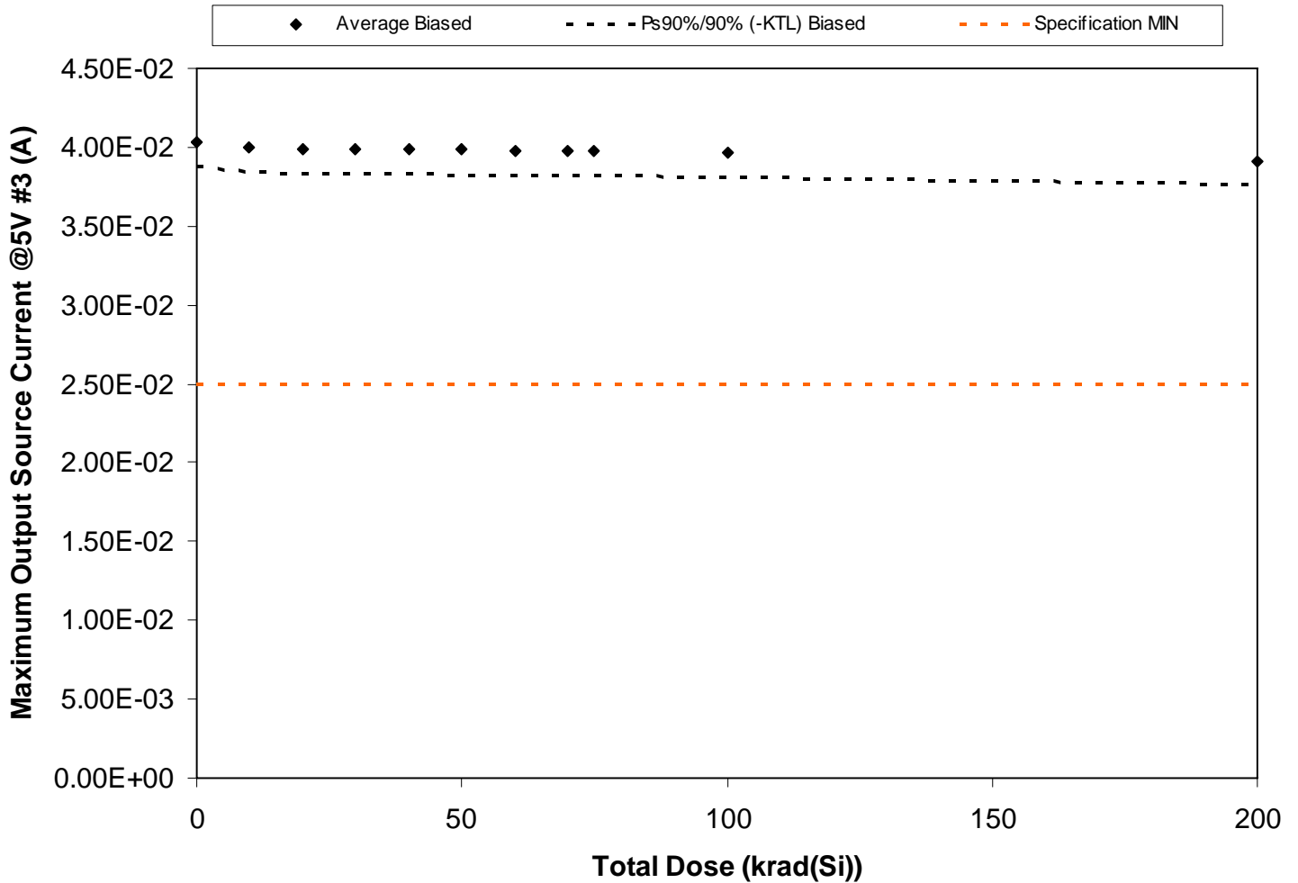
Figure 5.139. Plot of Maximum Output Source Current @5V #3 (A) versus total dose. The solid diamonds are the average of the measured data points for the samples irradiated under electrical bias and the black lines (solid and/or dashed) are the average of the data points after application of the KTL statistics on the samples irradiated under electrical bias. The red dotted line(s) are the pre- and/or post-irradiation minimum and/or maximum specification value as defined in the datasheet and/or test plan.
