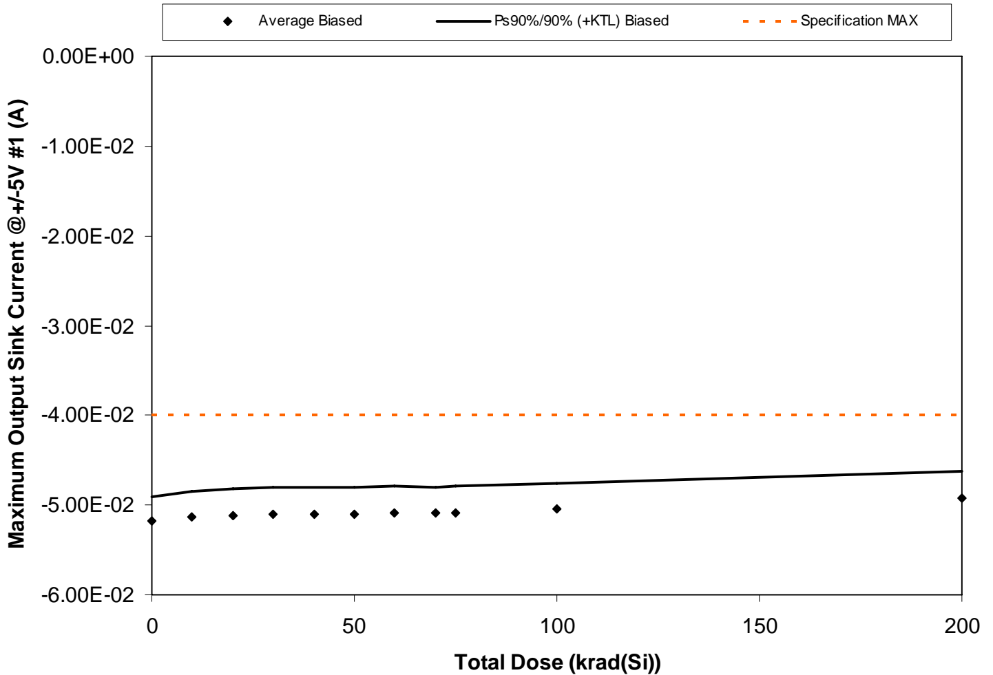
Figure 5.67. Plot of Maximum Output Sink Current @ +/-5V #1 (A) versus total dose. The solid diamonds are the average of the measured data points for the samples irradiated under electrical bias and the black lines (solid and/or dashed) are the average of the data points after application of the KTL statistics on the samples irradiated under electrical bias. The red dotted line(s) are the pre- and/or post-irradiation minimum and/or maximum specification value as defined in the datasheet and/or test plan.
