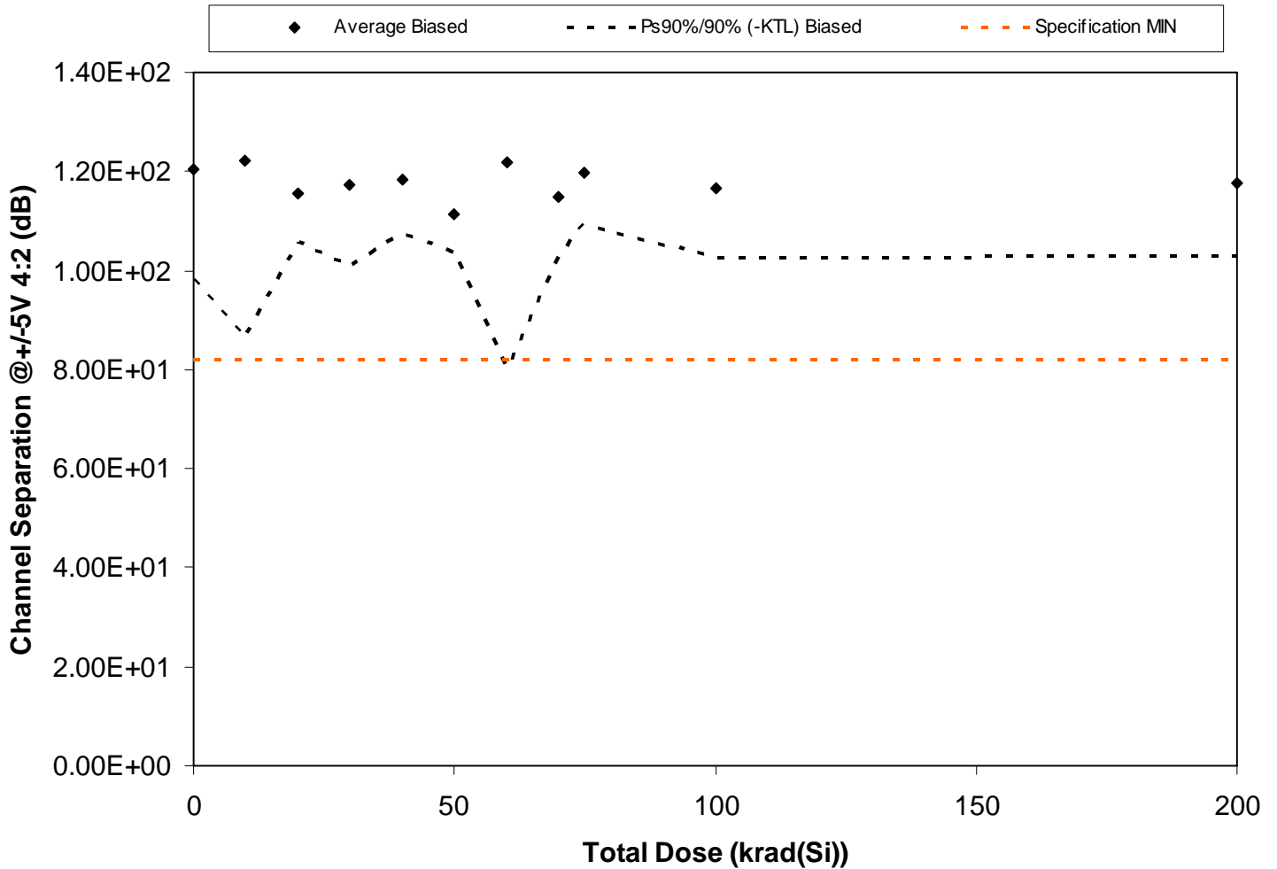
Figure 5.45. Plot of Channel Separation @ +/-5V 4:2 (dB) versus total dose. The solid diamonds are the average of the measured data points for the samples irradiated under electrical bias and the black lines (solid and/or dashed) are the average of the data points after application of the KTL statistics on the samples irradiated under electrical bias. The red dotted line(s) are the pre- and/or post-irradiation minimum and/or maximum specification value as defined in the datasheet and/or test plan.
