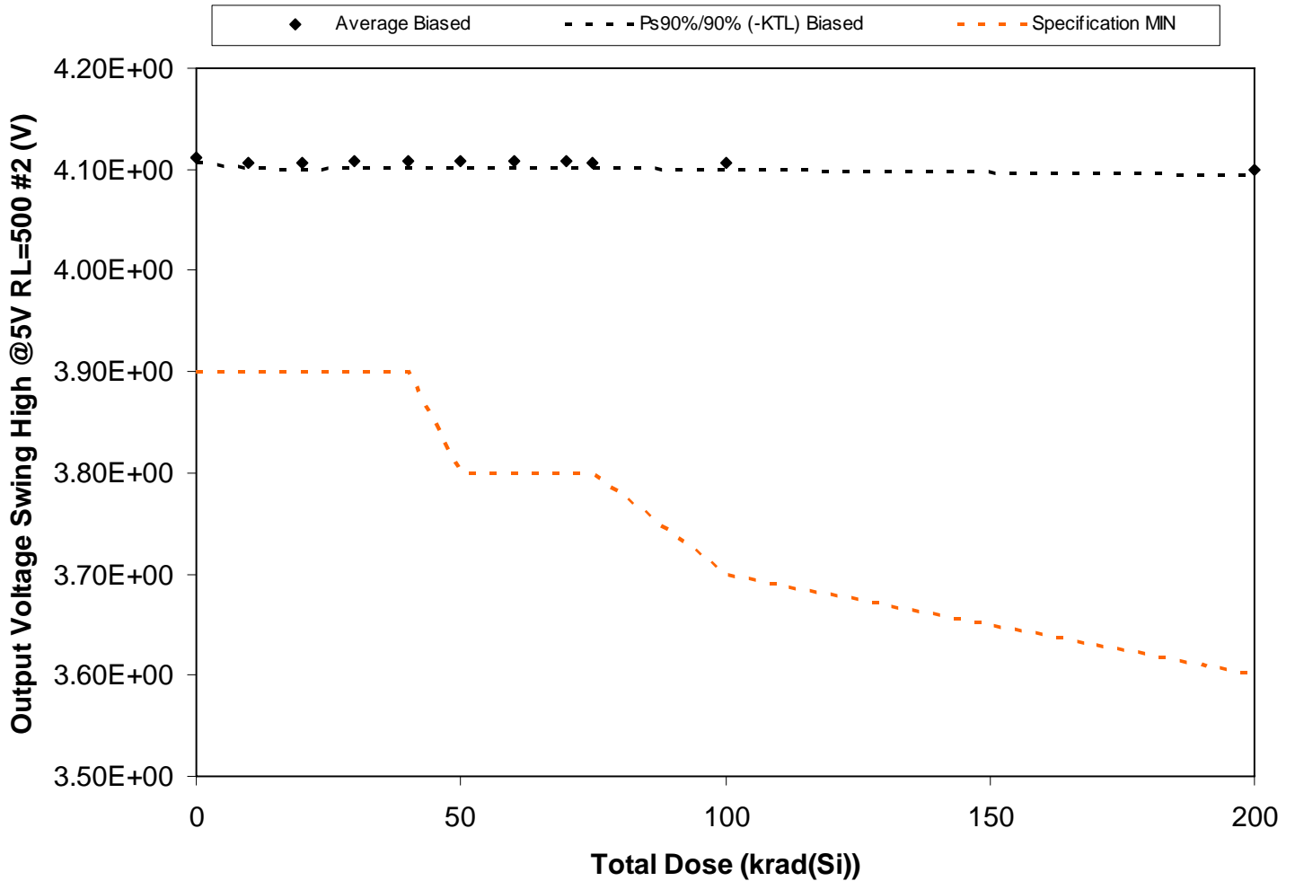
Figure 5.122. Plot of Output Voltage Swing High @5V RL=500 #2 (V) versus total dose. The solid diamonds are the average of the measured data points for the samples irradiated under electrical bias and the black lines (solid and/or dashed) are the average of the data points after application of the KTL statistics on the samples irradiated under electrical bias. The red dotted line(s) are the pre- and/or post-irradiation minimum and/or maximum specification value as defined in the datasheet and/or test plan.
