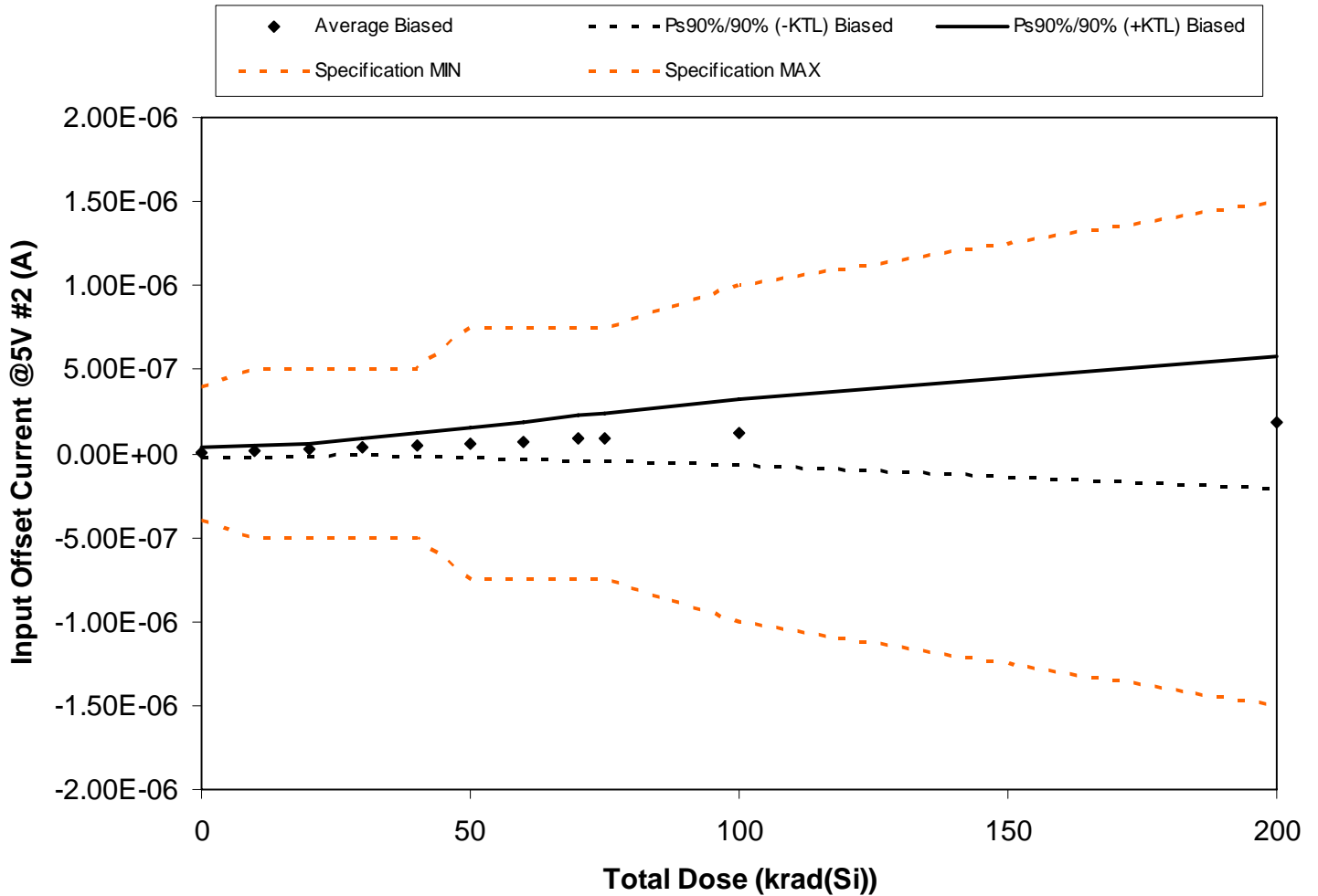
Figure 5.86. Plot of Input Offset Current @5V #2 (A) versus total dose. The solid diamonds are the average of the measured data points for the samples irradiated under electrical bias and the black lines (solid and/or dashed) are the average of the data points after application of the KTL statistics on the samples irradiated under electrical bias. The red dotted line(s) are the pre- and/or post-irradiation minimum and/or maximum specification value as defined in the datasheet and/or test plan.
