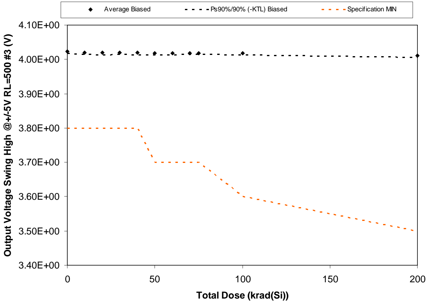
Figure 5.49. Plot of Output Voltage Swing High @ +/-5V RL=500 #3 (V) versus total dose. The solid diamonds are the average of the measured data points for the samples irradiated under electrical bias and the black lines (solid and/or dashed) are the average of the data points after application of the KTL statistics on the samples irradiated under electrical bias. The red dotted line(s) are the pre- and/or post-irradiation minimum and/or maximum specification value as defined in the datasheet and/or test plan.
