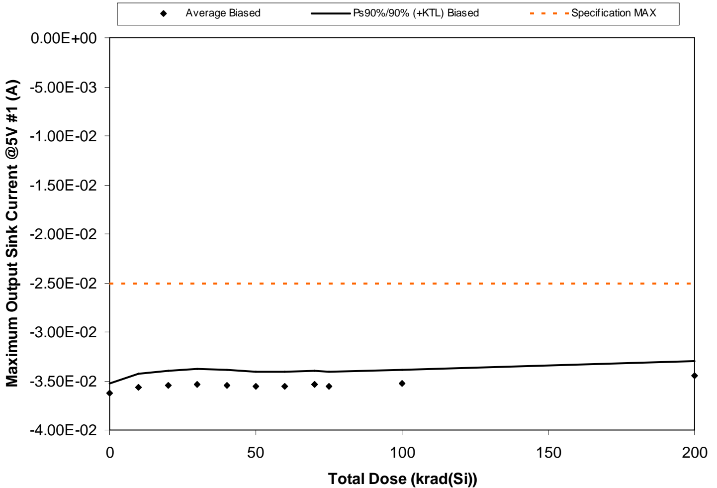
Figure 5.141. Plot of Maximum Output Sink Current @5V #1 (A) versus total dose. The solid diamonds are the average of the measured data points for the samples irradiated under electrical bias and the black lines (solid and/or dashed) are the average of the data points after application of the KTL statistics on the samples irradiated under electrical bias. The red dotted line(s) are the pre- and/or post-irradiation minimum and/or maximum specification value as defined in the datasheet and/or test plan.
