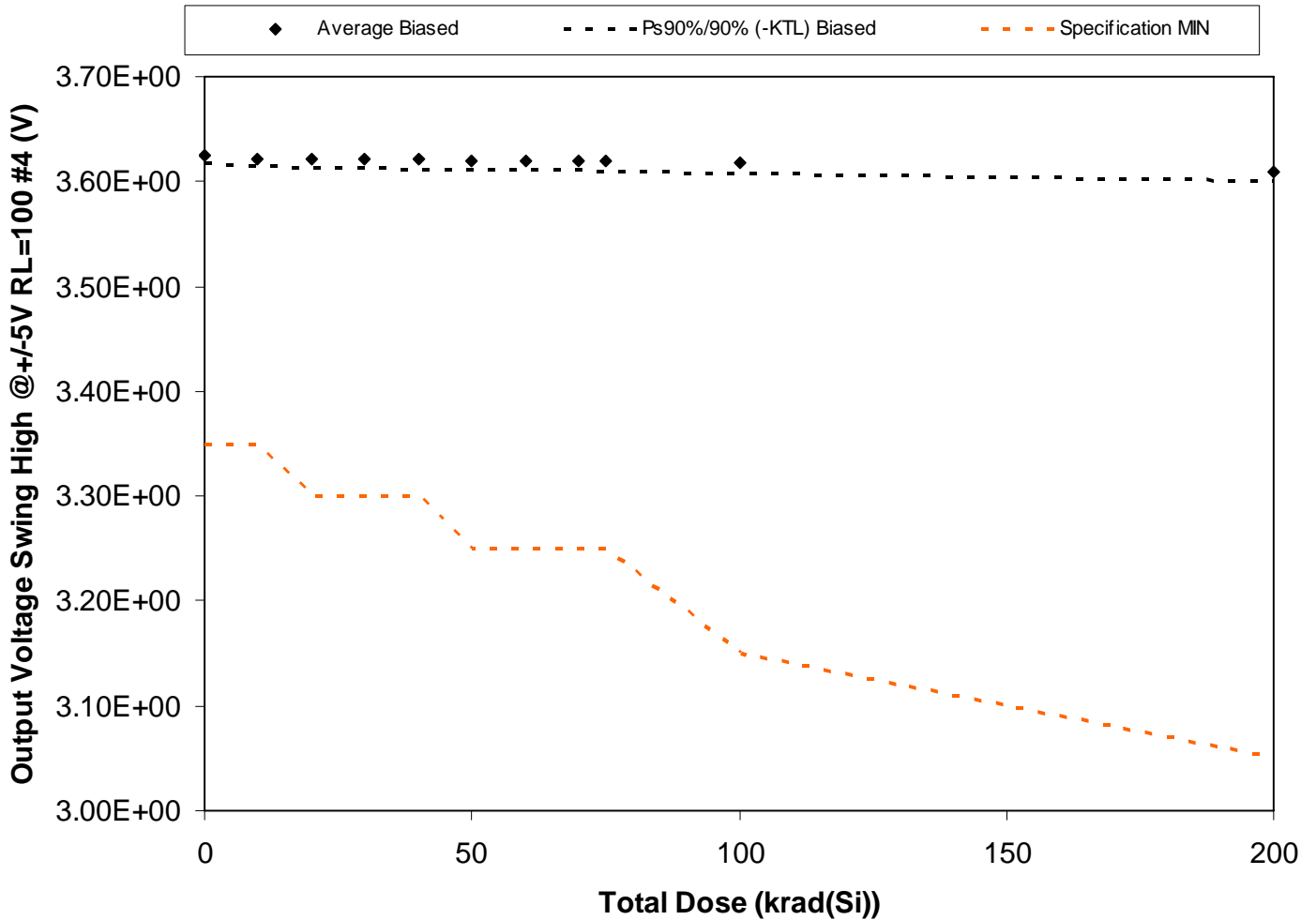
Figure 5.54. Plot of Output Voltage Swing High @ +/-5V RL=100 #4 (V) versus total dose. The solid diamonds are the average of the measured data points for the samples irradiated under electrical bias and the black lines (solid and/or dashed) are the average of the data points after application of the KTL statistics on the samples irradiated under electrical bias. The red dotted line(s) are the pre- and/or post-irradiation minimum and/or maximum specification value as defined in the datasheet and/or test plan.
