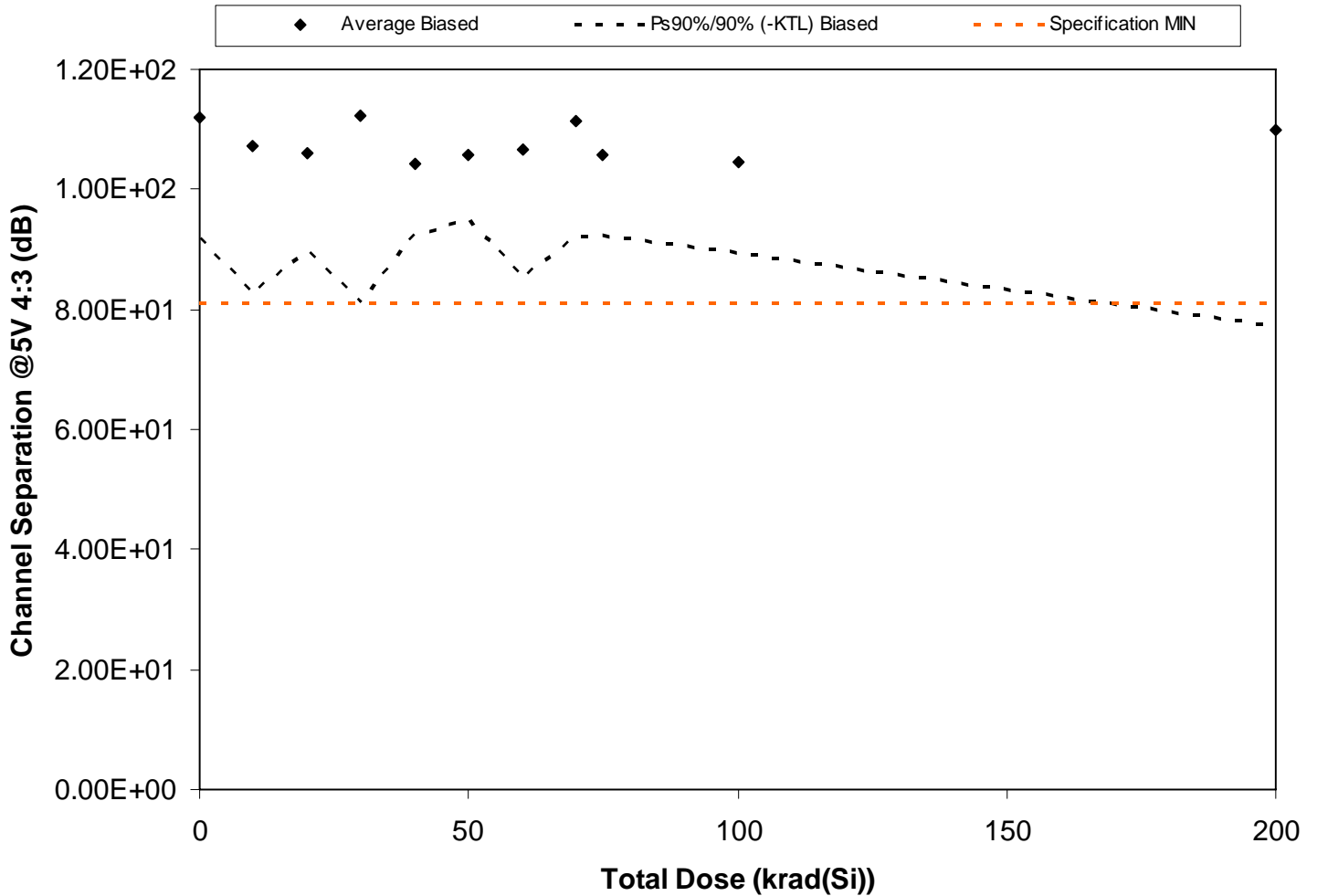
Figure 5.120. Plot of Channel Separation @5V 4:3 (dB) versus total dose. The solid diamonds are the average of the measured data points for the samples irradiated under electrical bias and the black lines (solid and/or dashed) are the average of the data points after application of the KTL statistics on the samples irradiated under electrical bias. The red dotted line(s) are the pre- and/or post-irradiation minimum and/or maximum specification value as defined in the datasheet and/or test plan.
