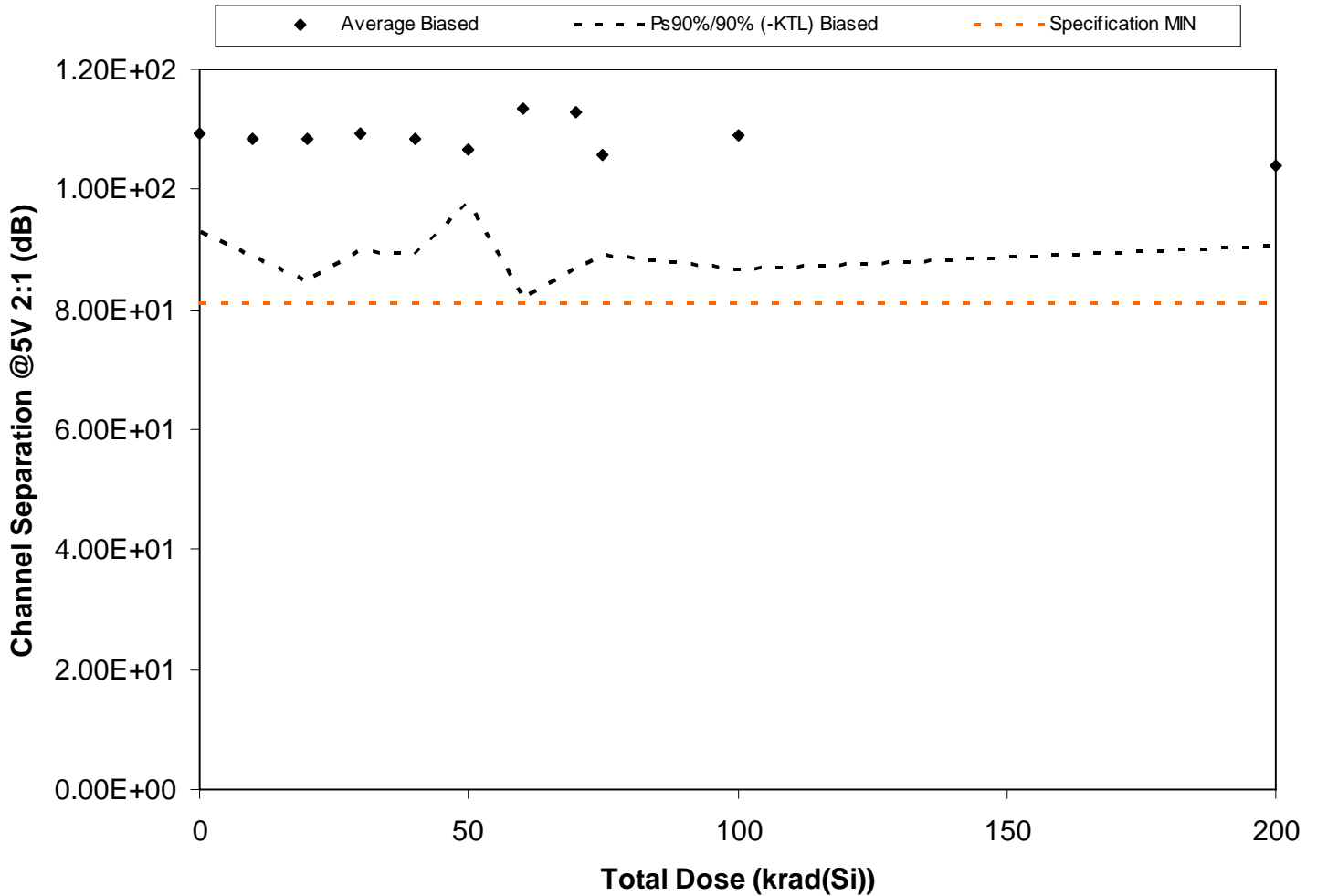
Figure 5.112. Plot of Channel Separation @5V 2:1 (dB) versus total dose. The solid diamonds are the average of the measured data points for the samples irradiated under electrical bias and the black lines (solid and/or dashed) are the average of the data points after application of the KTL statistics on the samples irradiated under electrical bias. The red dotted line(s) are the pre- and/or post-irradiation minimum and/or maximum specification value as defined in the datasheet and/or test plan.
