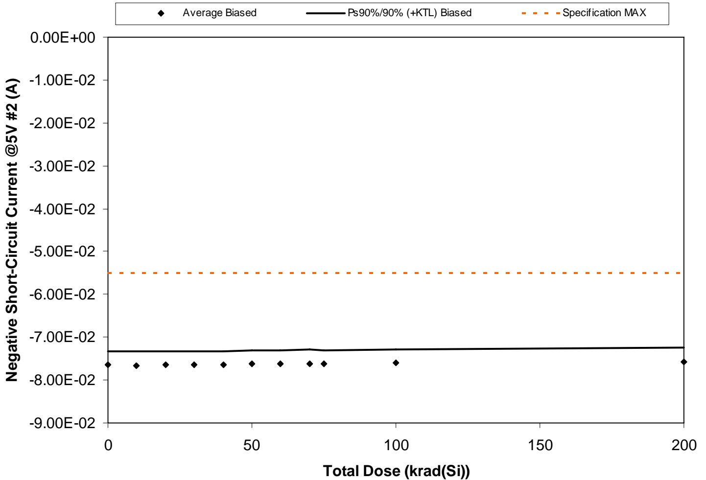
Figure 5.150. Plot of Negative Short-Circuit Current @5V #2 (A) versus total dose. The solid diamonds are the average of the measured data points for the samples irradiated under electrical bias and the black lines (solid and/or dashed) are the average of the data points after application of the KTL statistics on the samples irradiated under electrical bias. The red dotted line(s) are the pre- and/or post-irradiation minimum and/or maximum specification value as defined in the datasheet and/or test plan.
