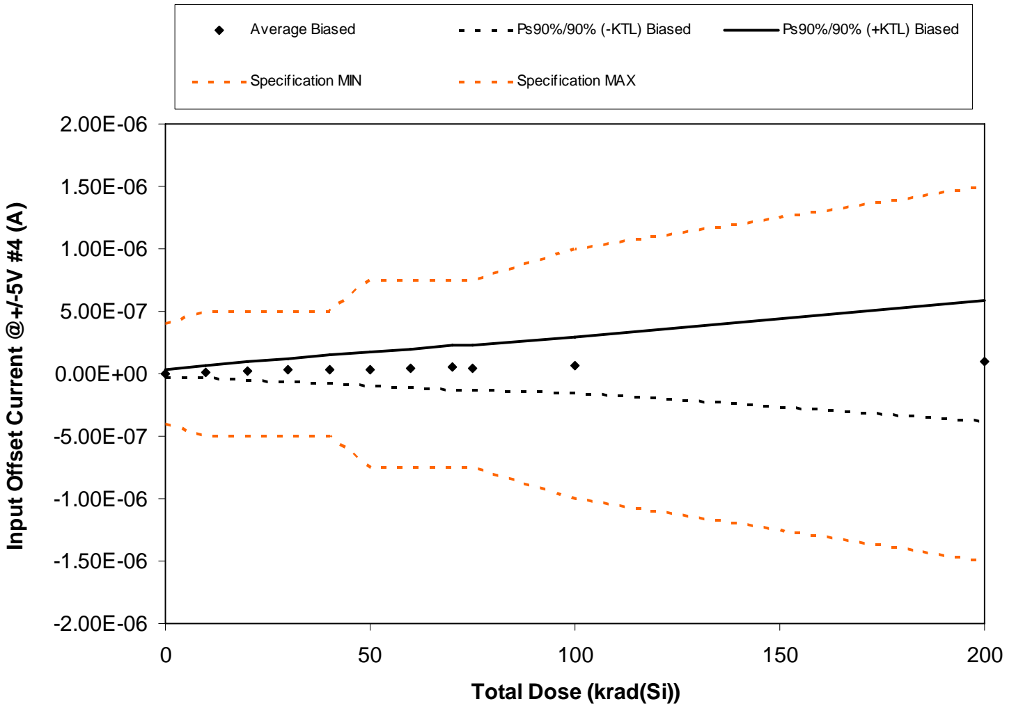
Figure 5.10. Plot of Input Offset Current @ +/-5V #4 (A) versus total dose. The solid diamonds are the average of the measured data points for the samples irradiated under electrical bias and the black lines (solid and/or dashed) are the average of the data points after application of the KTL statistics on the samples irradiated under electrical bias. The red dotted line(s) are the pre- and/or post-irradiation minimum and/or maximum specification value as defined in the datasheet and/or test plan.
