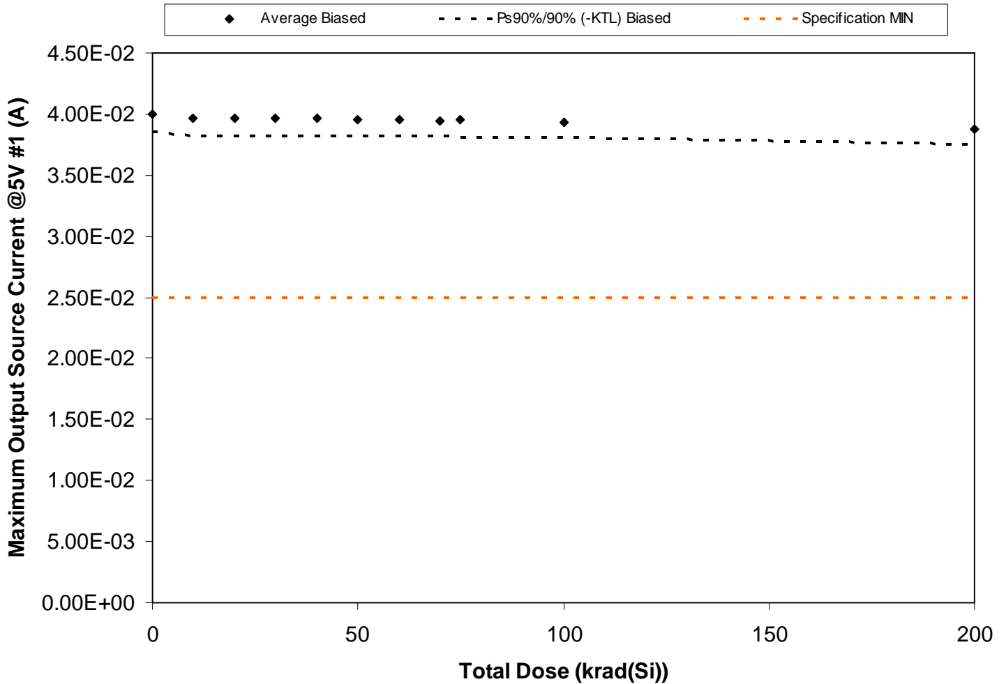
Figure 5.137. Plot of Maximum Output Source Current @5V #1 (A) versus total dose. The solid diamonds are the average of the measured data points for the samples irradiated under electrical bias and the black lines (solid and/or dashed) are the average of the data points after application of the KTL statistics on the samples irradiated under electrical bias. The red dotted line(s) are the pre- and/or post-irradiation minimum and/or maximum specification value as defined in the datasheet and/or test plan.
