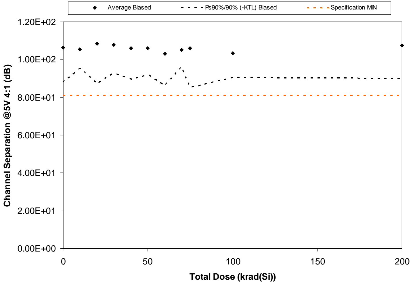
Figure 5.118. Plot of Channel Separation @5V 4:1 (dB) versus total dose. The solid diamonds are the average of the measured data points for the samples irradiated under electrical bias and the black lines (solid and/or dashed) are the average of the data points after application of the KTL statistics on the samples irradiated under electrical bias. The red dotted line(s) are the pre- and/or post-irradiation minimum and/or maximum specification value as defined in the datasheet and/or test plan.
