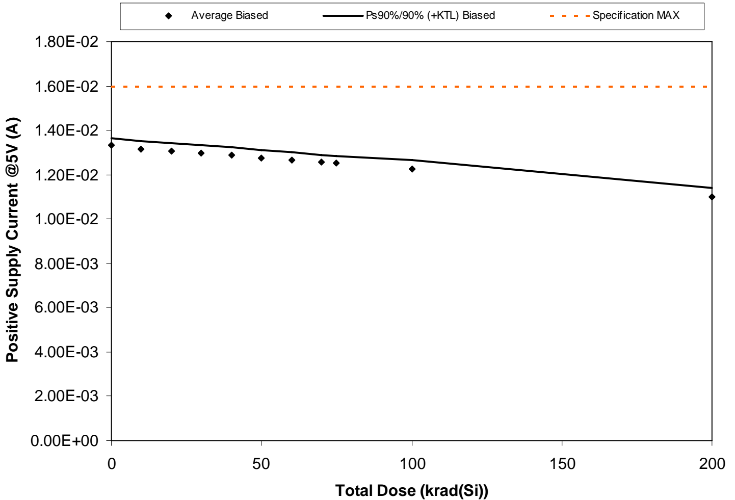
Figure 5.79. Plot of Positive Supply Current @5V (A) versus total dose. The solid diamonds are the average of the measured data points for the samples irradiated under electrical bias and the black lines (solid and/or dashed) are the average of the data points after application of the KTL statistics on the samples irradiated under electrical bias. The red dotted line(s) are the pre- and/or post-irradiation minimum and/or maximum specification value as defined in the datasheet and/or test plan.
