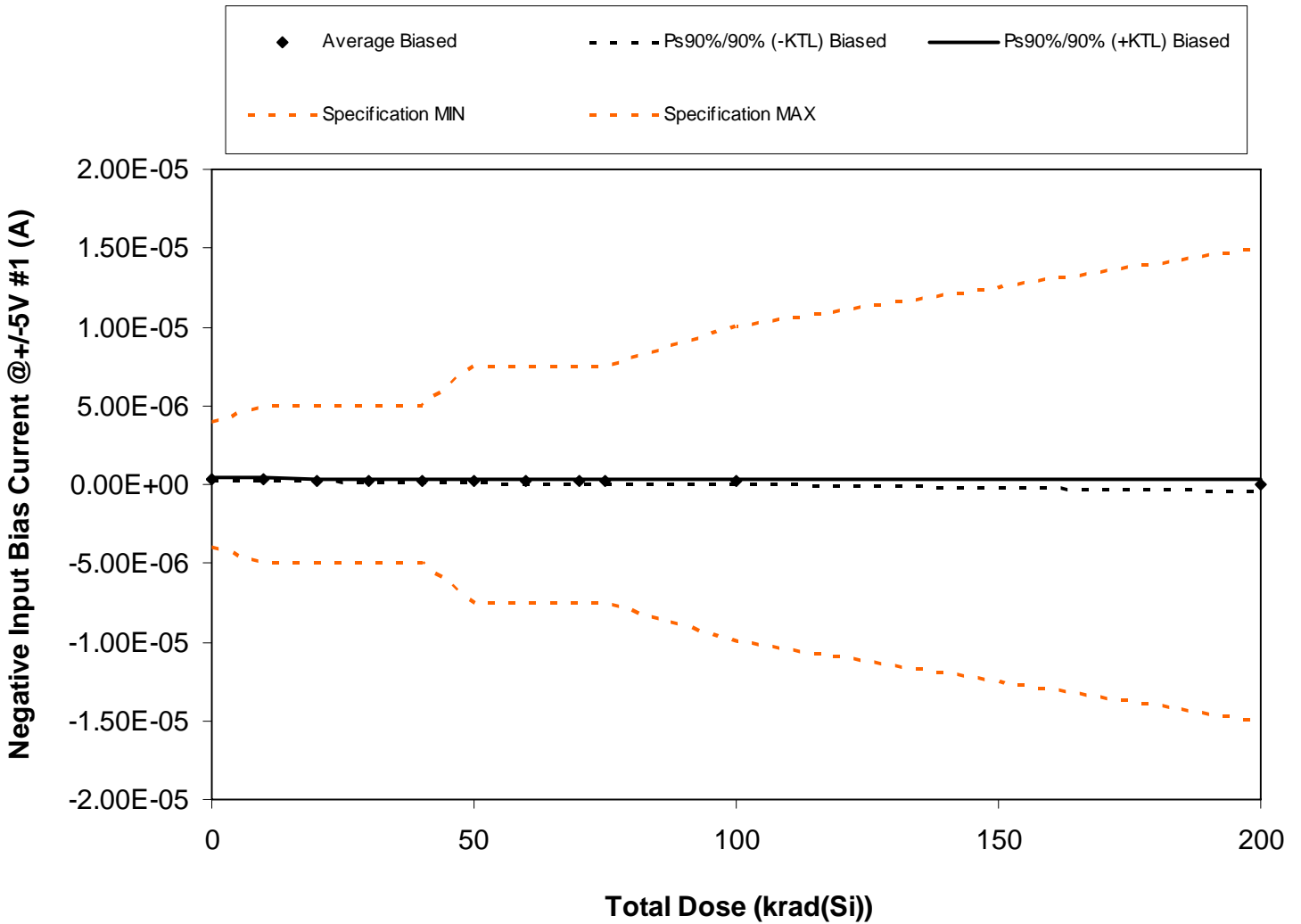
Figure 5.15. Plot of Negative Input Bias Current @ +/-5V #1 (A) versus total dose. The solid diamonds are the average of the measured data points for the samples irradiated under electrical bias and the black lines (solid and/or dashed) are the average of the data points after application of the KTL statistics on the samples irradiated under electrical bias. The red dotted line(s) are the pre- and/or post-irradiation minimum and/or maximum specification value as defined in the datasheet and/or test plan.
