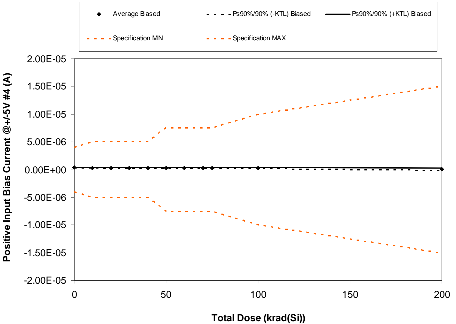
Figure 5.14. Plot of Positive Input Bias Current @ +/-5V #4 (A) versus total dose. The solid diamonds are the average of the measured data points for the samples irradiated under electrical bias and the black lines (solid and/or dashed) are the average of the data points after application of the KTL statistics on the samples irradiated under electrical bias. The red dotted line(s) are the pre- and/or post-irradiation minimum and/or maximum specification value as defined in the datasheet and/or test plan.
