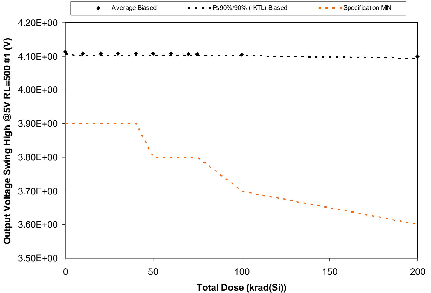
Figure 5.121. Plot of Output Voltage Swing High @5V RL=500 #1 (V) versus total dose. The solid diamonds are the average of the measured data points for the samples irradiated under electrical bias and the black lines (solid and/or dashed) are the average of the data points after application of the KTL statistics on the samples irradiated under electrical bias. The red dotted line(s) are the pre- and/or post-irradiation minimum and/or maximum specification value as defined in the datasheet and/or test plan.
