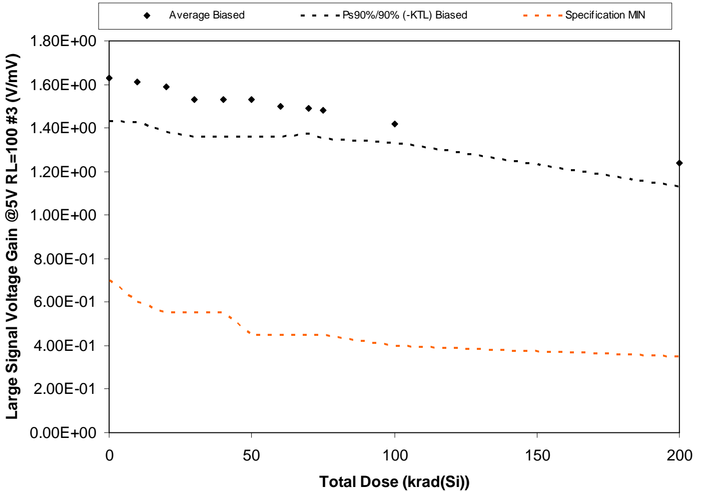
Figure 5.107. Plot of Large Signal Voltage Gain @5V RL=100 #3 (V/mV) versus total dose. The solid diamonds are the average of the measured data points for the samples irradiated under electrical bias and the black lines (solid and/or dashed) are the average of the data points after application of the KTL statistics on the samples irradiated under electrical bias. The red dotted line(s) are the pre- and/or post-irradiation minimum and/or maximum specification value as defined in the datasheet and/or test plan.
