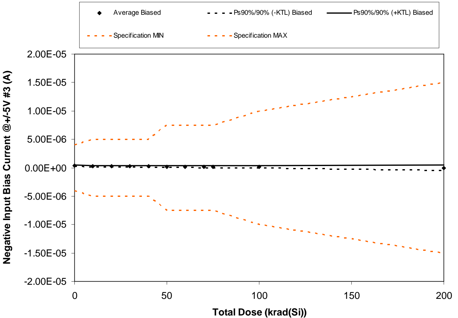
Figure 5.17. Plot of Negative Input Bias Current @ +/-5V #3 (A) versus total dose. The solid diamonds are the average of the measured data points for the samples irradiated under electrical bias and the black lines (solid and/or dashed) are the average of the data points after application of the KTL statistics on the samples irradiated under electrical bias. The red dotted line(s) are the pre- and/or post-irradiation minimum and/or maximum specification value as defined in the datasheet and/or test plan.
