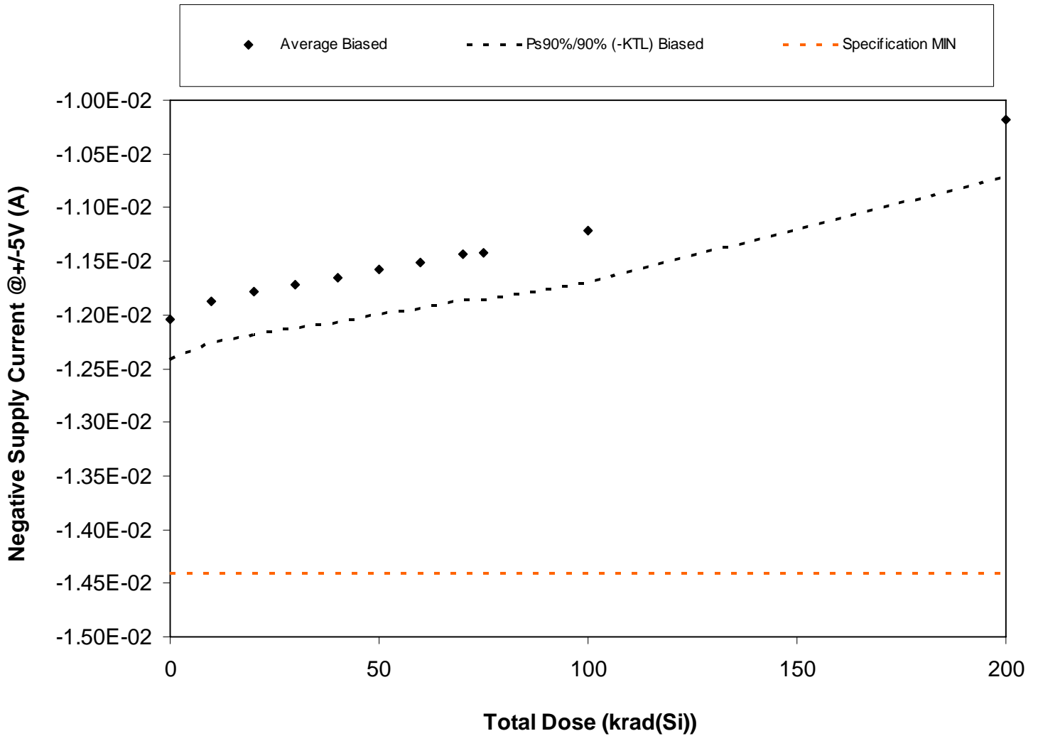
Figure 5.2. Plot of Negative Supply Current @ +/-5V (A) versus total dose. The solid diamonds are the average of the measured data points for the samples irradiated under electrical bias and the black lines (solid and/or dashed) are the average of the data points after application of the KTL statistics on the samples irradiated under electrical bias. The red dotted line(s) are the pre- and/or post-irradiation minimum and/or maximum specification value as defined in the datasheet and/or test plan.
