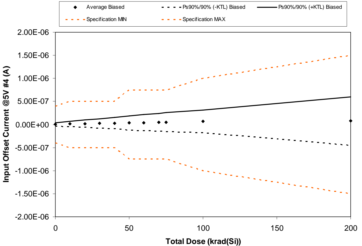
Figure 5.88. Plot of Input Offset Current @5V #4 (A) versus total dose. The solid diamonds are the average of the measured data points for the samples irradiated under electrical bias and the black lines (solid and/or dashed) are the average of the data points after application of the KTL statistics on the samples irradiated under electrical bias. The red dotted line(s) are the pre- and/or post-irradiation minimum and/or maximum specification value as defined in the datasheet and/or test plan.
