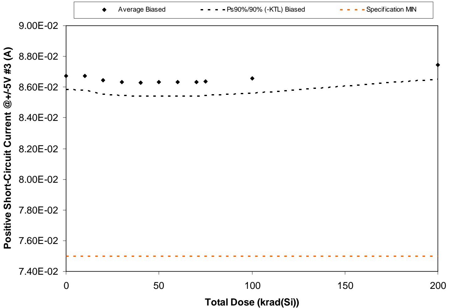
Figure 5.73. Plot of Positive Short-Circuit Current @ +/-5V #3 (A) versus total dose. The solid diamonds are the average of the measured data points for the samples irradiated under electrical bias and the black lines (solid and/or dashed) are the average of the data points after application of the KTL statistics on the samples irradiated under electrical bias. The red dotted line(s) are the pre- and/or post-irradiation minimum and/or maximum specification value as defined in the datasheet and/or test plan.
