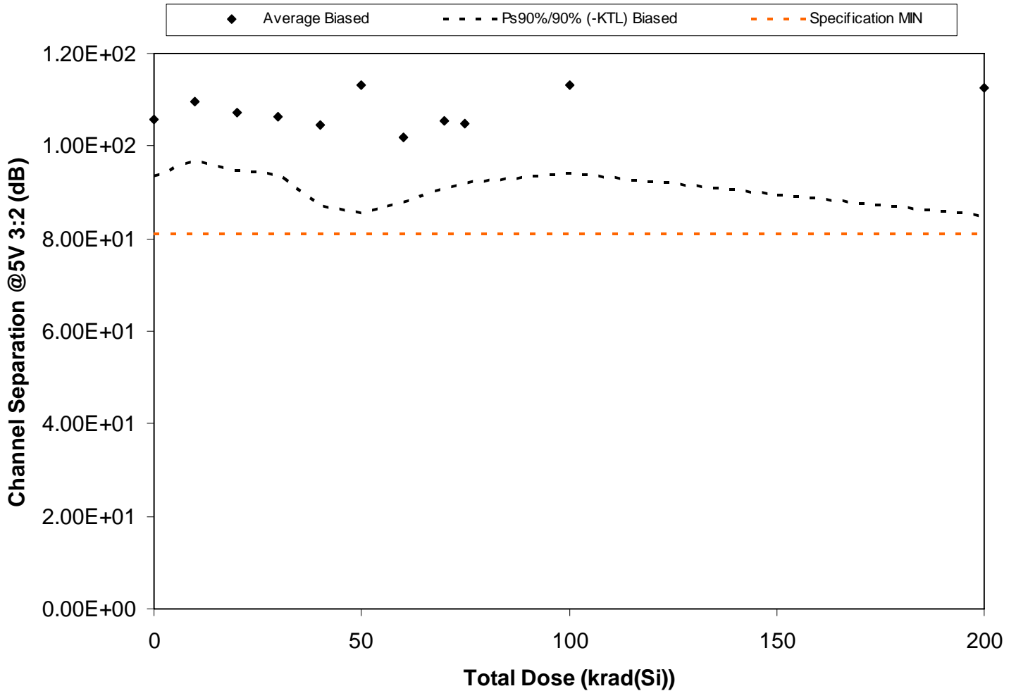
Figure 5.116. Plot of Channel Separation @5V 3:2 (dB) versus total dose. The solid diamonds are the average of the measured data points for the samples irradiated under electrical bias and the black lines (solid and/or dashed) are the average of the data points after application of the KTL statistics on the samples irradiated under electrical bias. The red dotted line(s) are the pre- and/or post-irradiation minimum and/or maximum specification value as defined in the datasheet and/or test plan.
