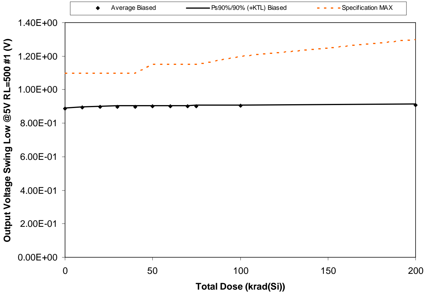
Figure 5.129. Plot of Output Voltage Swing Low @5V RL=500 #1 (V) versus total dose. The solid diamonds are the average of the measured data points for the samples irradiated under electrical bias and the black lines (solid and/or dashed) are the average of the data points after application of the KTL statistics on the samples irradiated under electrical bias. The red dotted line(s) are the pre- and/or post-irradiation minimum and/or maximum specification value as defined in the datasheet and/or test plan.
