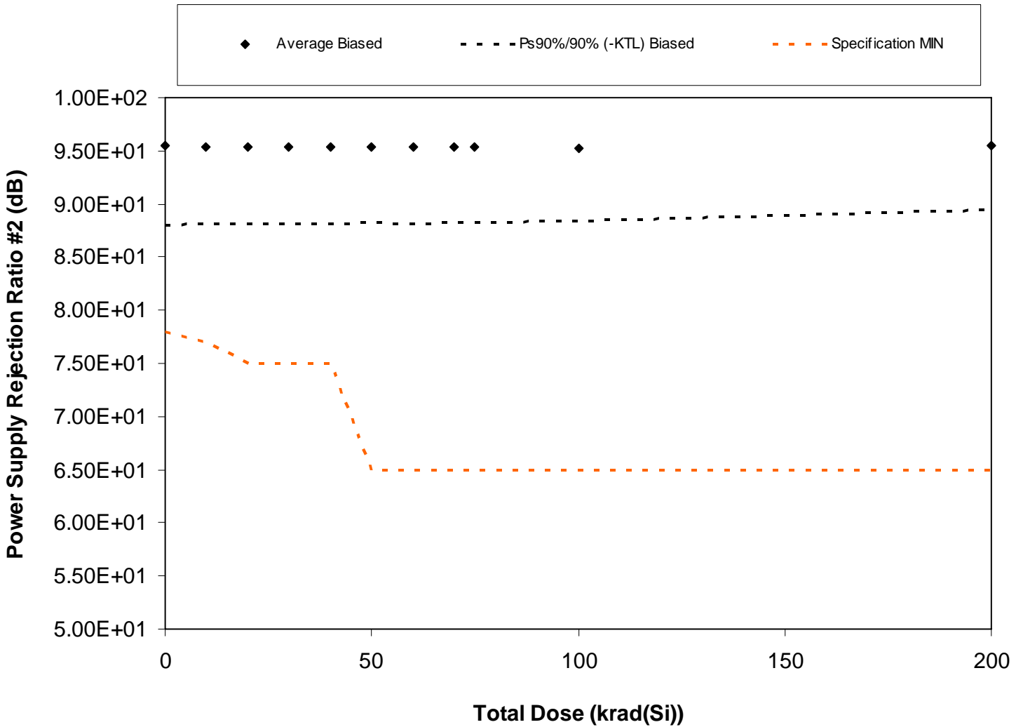
Figure 5.24. Plot of Power Supply Rejection Ratio #2 (dB) versus total dose. The solid diamonds are the average of the measured data points for the samples irradiated under electrical bias and the black lines (solid and/or dashed) are the average of the data points after application of the KTL statistics on the samples irradiated under electrical bias. The red dotted line(s) are the pre- and/or post-irradiation minimum and/or maximum specification value as defined in the datasheet and/or test plan.
