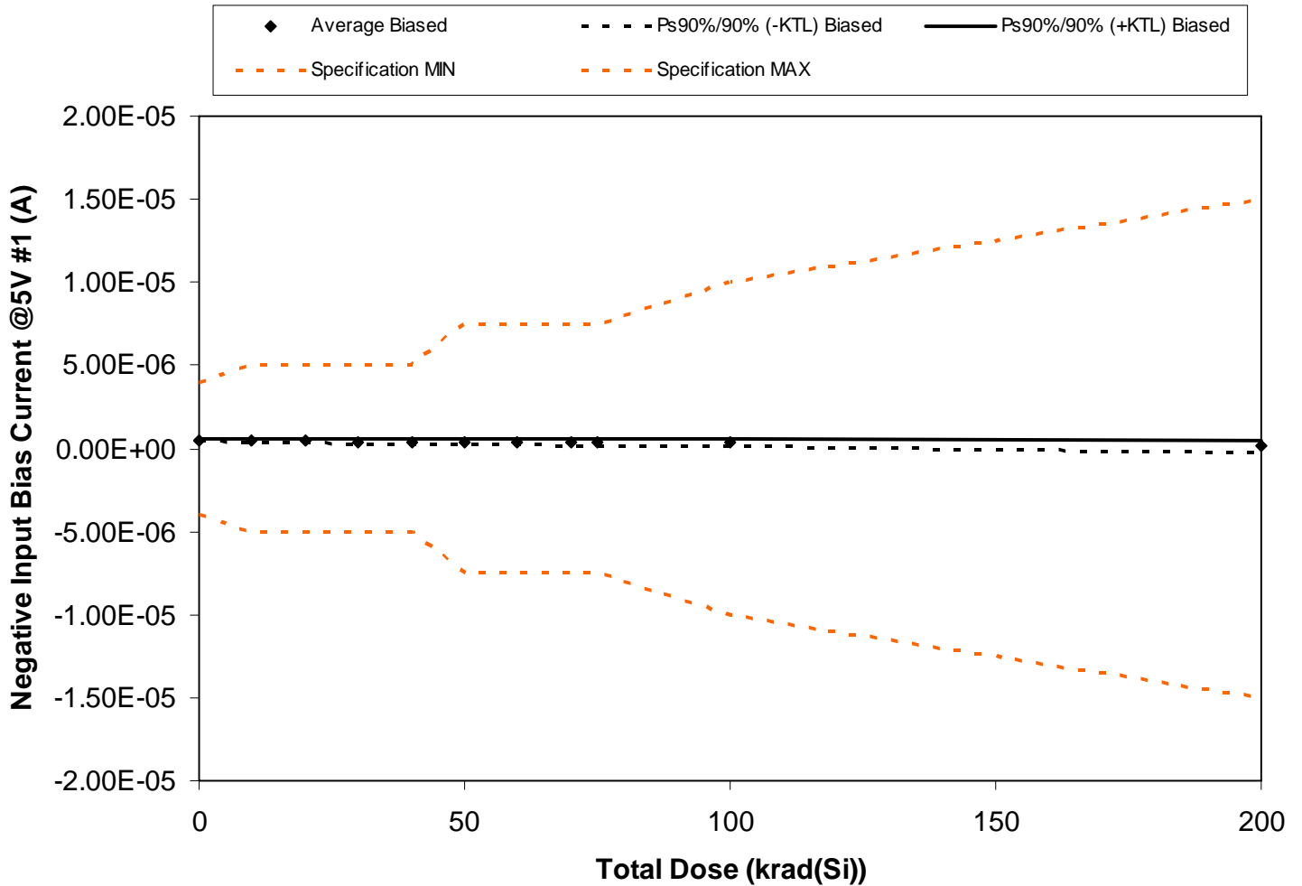
Figure 5.93. Plot of Negative Input Bias Current @5V #1 (A) versus total dose. The solid diamonds are the average of the measured data points for the samples irradiated under electrical bias and the black lines (solid and/or dashed) are the average of the data points after application of the KTL statistics on the samples irradiated under electrical bias. The red dotted line(s) are the pre- and/or post-irradiation minimum and/or maximum specification value as defined in the datasheet and/or test plan.
