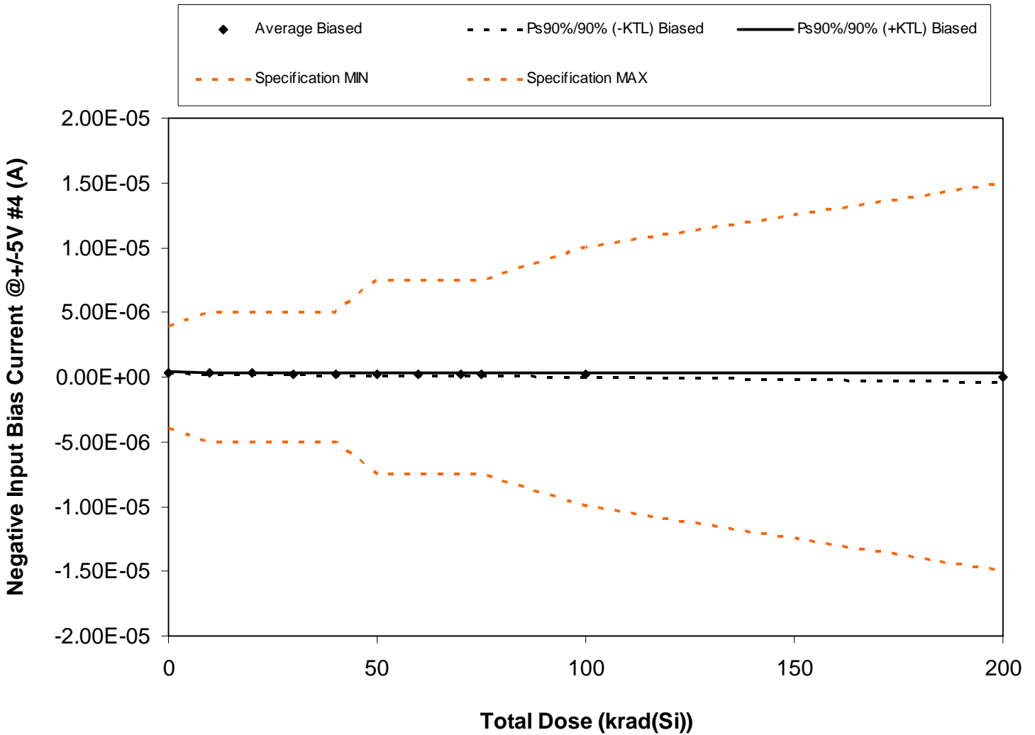
Figure 5.18. Plot of Negative Input Bias Current @ +/-5V #4 (A) versus total dose. The solid diamonds are the average of the measured data points for the samples irradiated under electrical bias and the black lines (solid and/or dashed) are the average of the data points after application of the KTL statistics on the samples irradiated under electrical bias. The red dotted line(s) are the pre- and/or post-irradiation minimum and/or maximum specification value as defined in the datasheet and/or test plan.
