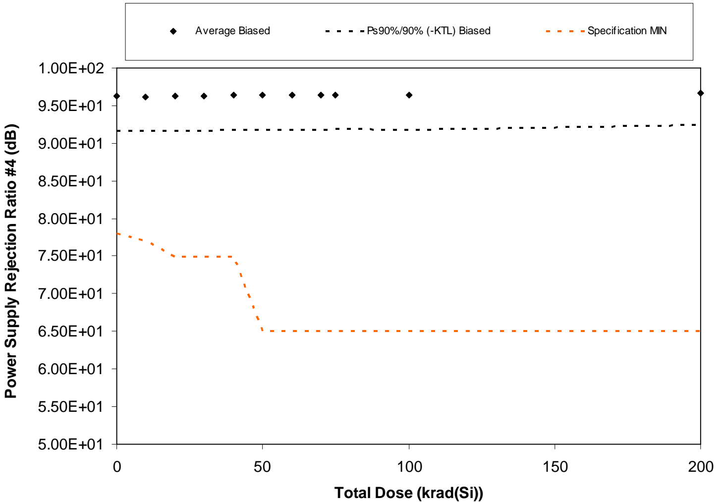
Figure 5.26. Plot of Power Supply Rejection Ratio #4 (dB) versus total dose. The solid diamonds are the average of the measured data points for the samples irradiated under electrical bias and the black lines (solid and/or dashed) are the average of the data points after application of the KTL statistics on the samples irradiated under electrical bias. The red dotted line(s) are the pre- and/or post-irradiation minimum and/or maximum specification value as defined in the datasheet and/or test plan.
