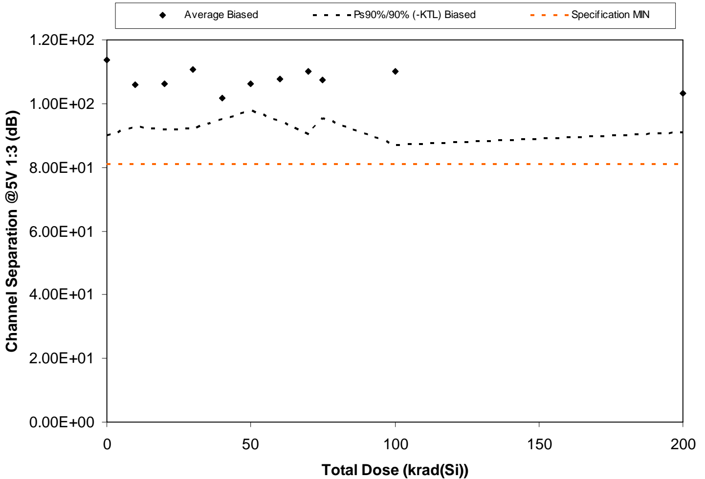
Figure 5.110. Plot of Channel Separation @5V 1:3 (dB) versus total dose. The solid diamonds are the average of the measured data points for the samples irradiated under electrical bias and the black lines (solid and/or dashed) are the average of the data points after application of the KTL statistics on the samples irradiated under electrical bias. The red dotted line(s) are the pre- and/or post-irradiation minimum and/or maximum specification value as defined in the datasheet and/or test plan.
