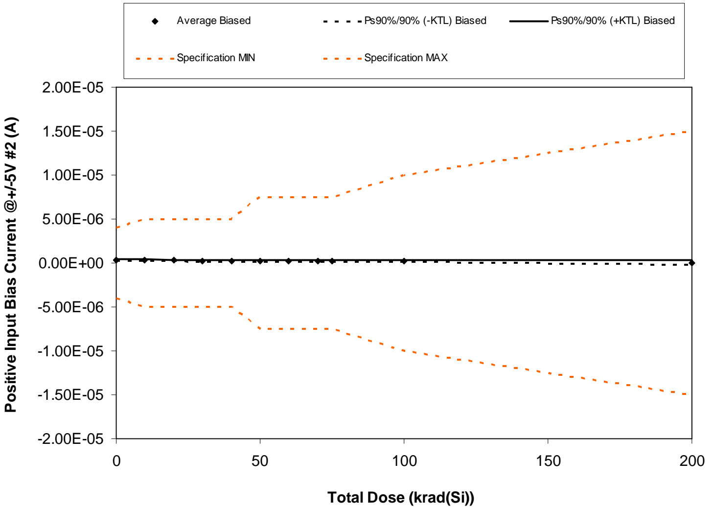
Figure 5.12. Plot of Positive Input Bias Current @ +/-5V #2 (A) versus total dose. The solid diamonds are the average of the measured data points for the samples irradiated under electrical bias and the black lines (solid and/or dashed) are the average of the data points after application of the KTL statistics on the samples irradiated under electrical bias. The red dotted line(s) are the pre- and/or post-irradiation minimum and/or maximum specification value as defined in the datasheet and/or test plan.
