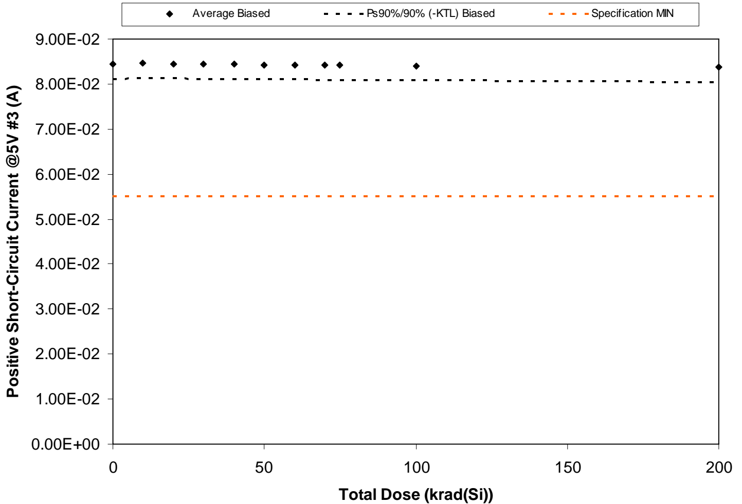
Figure 5.147. Plot of Positive Short-Circuit Current @5V #3 (A) versus total dose. The solid diamonds are the average of the measured data points for the samples irradiated under electrical bias and the black lines (solid and/or dashed) are the average of the data points after application of the KTL statistics on the samples irradiated under electrical bias. The red dotted line(s) are the pre- and/or post-irradiation minimum and/or maximum specification value as defined in the datasheet and/or test plan.
