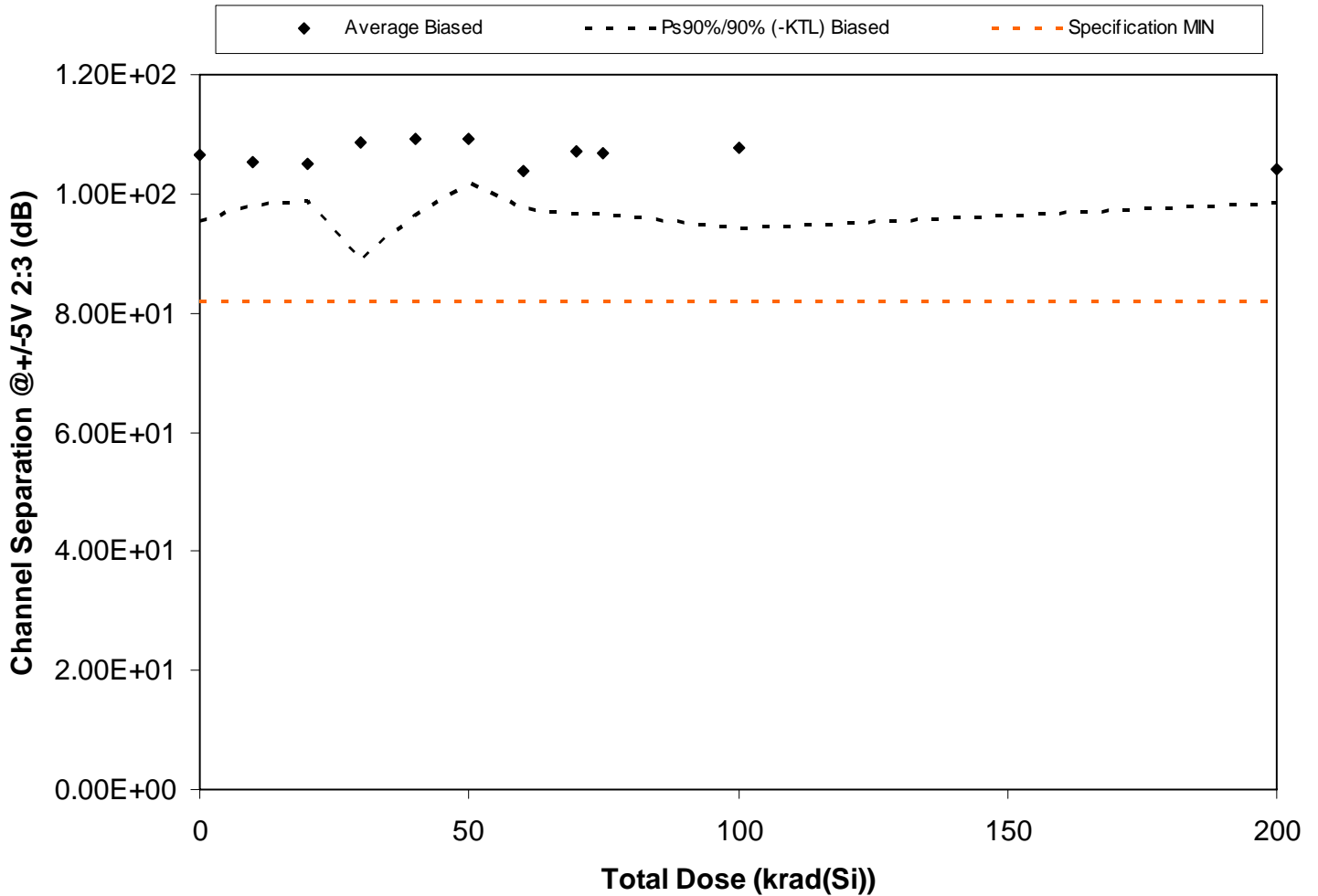
Figure 5.39. Plot of Channel Separation @ +/-5V 2:3 (dB) versus total dose. The solid diamonds are the average of the measured data points for the samples irradiated under electrical bias and the black lines (solid and/or dashed) are the average of the data points after application of the KTL statistics on the samples irradiated under electrical bias. The red dotted line(s) are the pre- and/or post-irradiation minimum and/or maximum specification value as defined in the datasheet and/or test plan.
