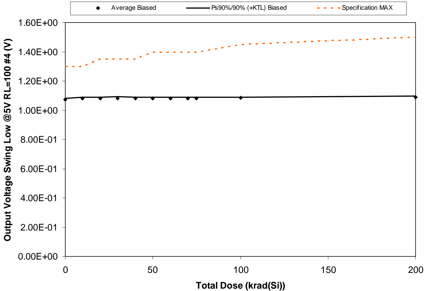
Figure 5.136. Plot of Output Voltage Swing Low @5V RL=100 #4 (V) versus total dose. The solid diamonds are the average of the measured data points for the samples irradiated under electrical bias and the black lines (solid and/or dashed) are the average of the data points after application of the KTL statistics on the samples irradiated under electrical bias. The red dotted line(s) are the pre- and/or post-irradiation minimum and/or maximum specification value as defined in the datasheet and/or test plan.
