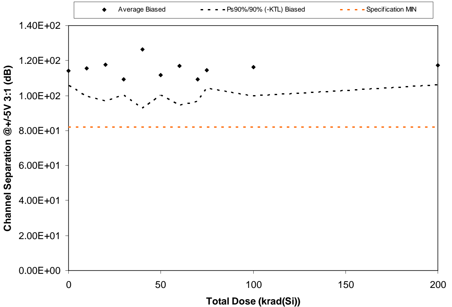
Figure 5.41. Plot of Channel Separation @ +/-5V 3:1 (dB) versus total dose. The solid diamonds are the average of the measured data points for the samples irradiated under electrical bias and the black lines (solid and/or dashed) are the average of the data points after application of the KTL statistics on the samples irradiated under electrical bias. The red dotted line(s) are the pre- and/or post-irradiation minimum and/or maximum specification value as defined in the datasheet and/or test plan.
