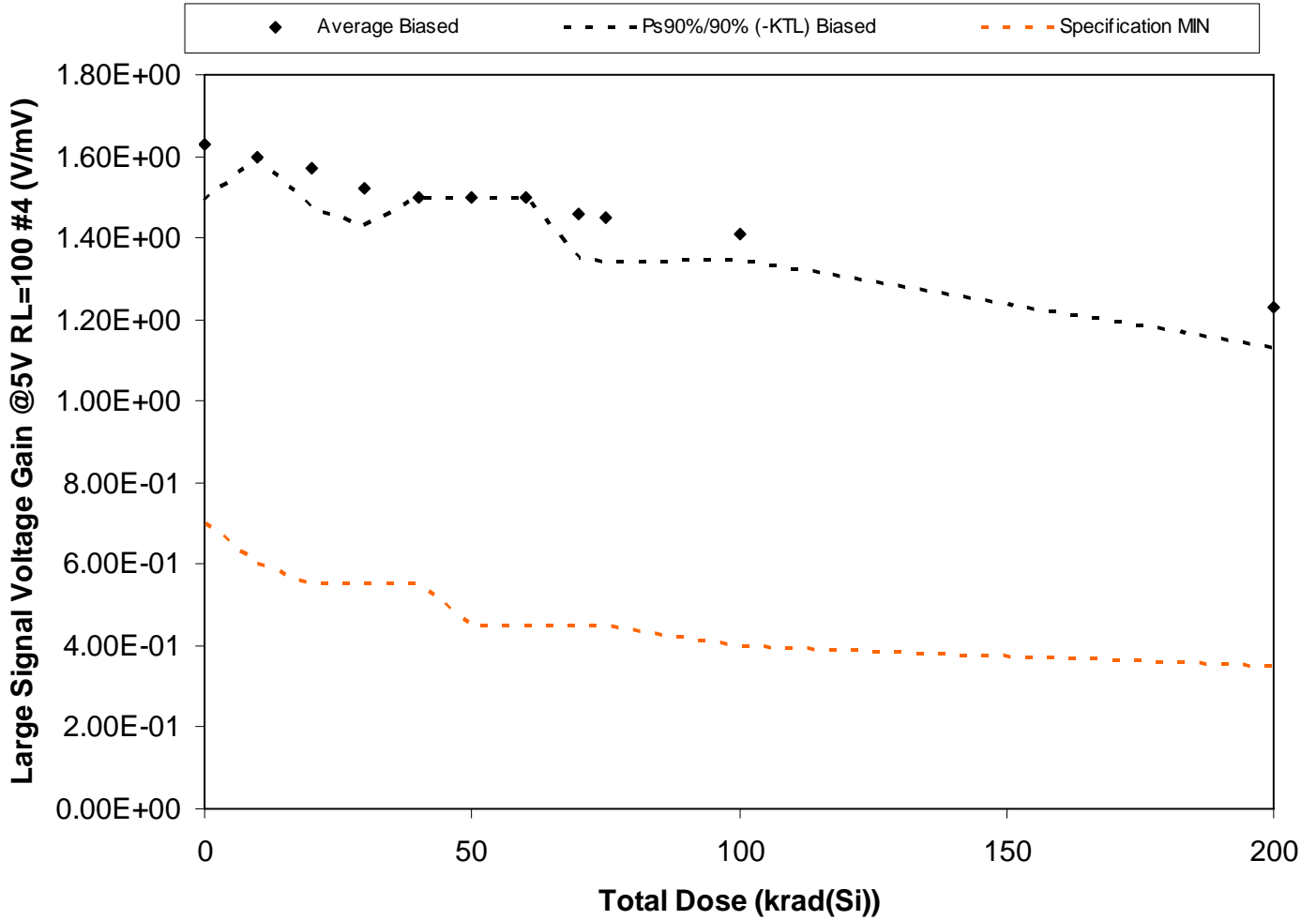
Figure 5.108. Plot of Large Signal Voltage Gain @5V RL=100 #4 (V/mV) versus total dose. The solid diamonds are the average of the measured data points for the samples irradiated under electrical bias and the black lines (solid and/or dashed) are the average of the data points after application of the KTL statistics on the samples irradiated under electrical bias. The red dotted line(s) are the pre- and/or post-irradiation minimum and/or maximum specification value as defined in the datasheet and/or test plan.
