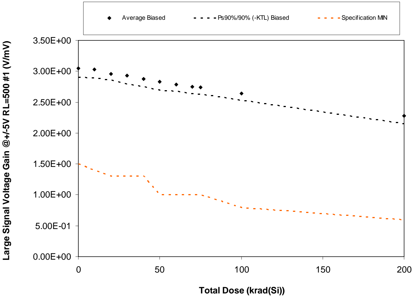
Figure 5.27. Plot of Large Signal Voltage Gain @ +/-5V RL=500 #1 (V/mV) versus total dose. The solid diamonds are the average of the measured data points for the samples irradiated under electrical bias and the black lines (solid and/or dashed) are the average of the data points after application of the KTL statistics on the samples irradiated under electrical bias. The red dotted line(s) are the pre- and/or post-irradiation minimum and/or maximum specification value as defined in the datasheet and/or test plan.
