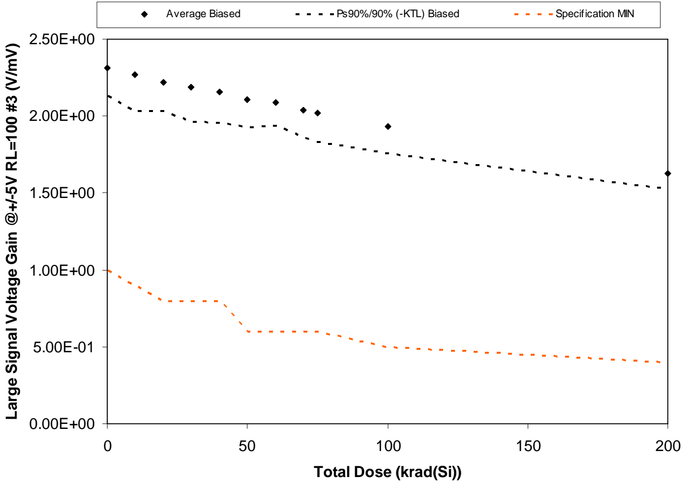
Figure 5.33. Plot of Large Signal Voltage Gain @ +/-5V RL=100 #3 (V/mV) versus total dose. The solid diamonds are the average of the measured data points for the samples irradiated under electrical bias and the black lines (solid and/or dashed) are the average of the data points after application of the KTL statistics on the samples irradiated under electrical bias. The red dotted line(s) are the pre- and/or post-irradiation minimum and/or maximum specification value as defined in the datasheet and/or test plan.
