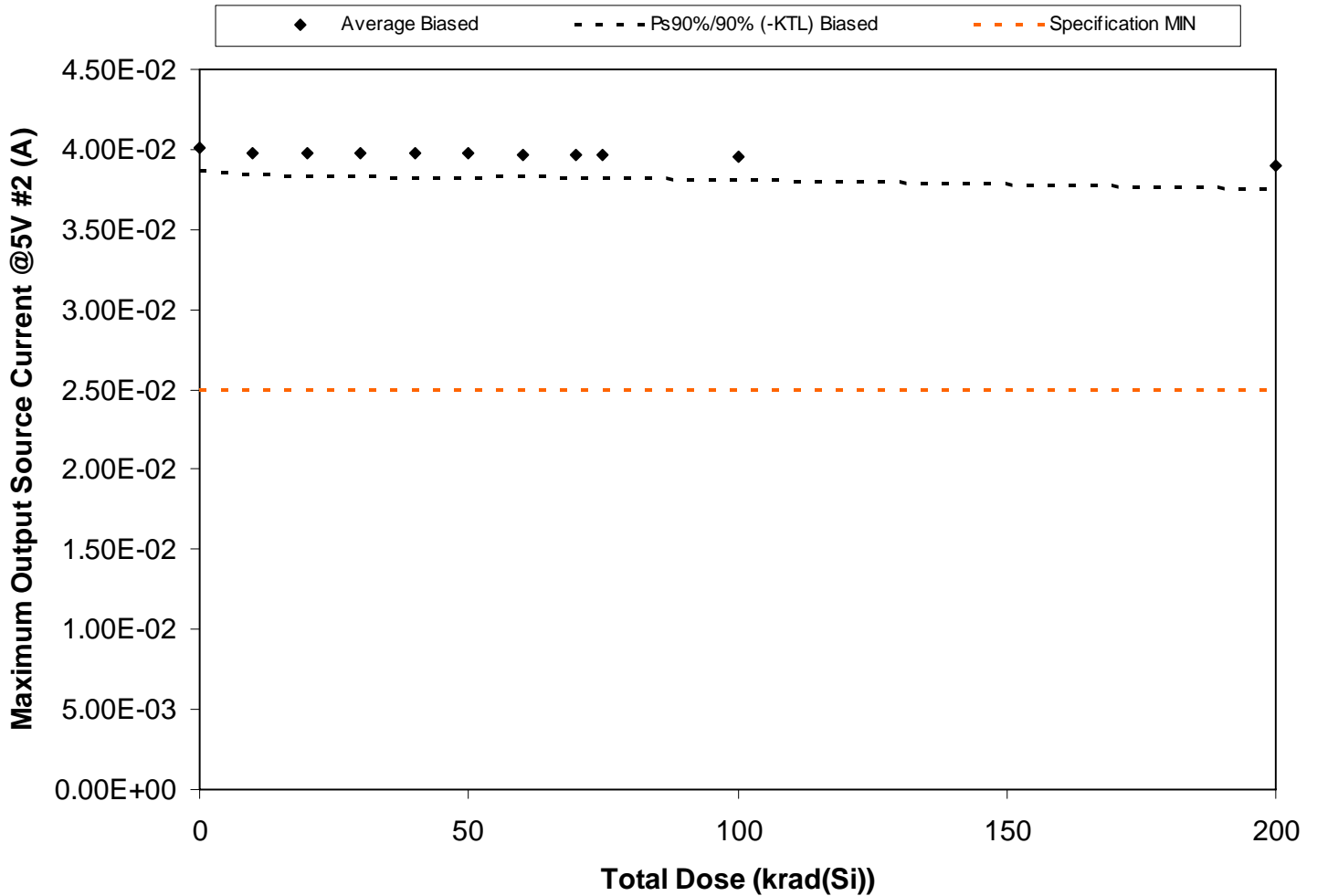
Figure 5.138. Plot of Maximum Output Source Current @5V #2 (A) versus total dose. The solid diamonds are the average of the measured data points for the samples irradiated under electrical bias and the black lines (solid and/or dashed) are the average of the data points after application of the KTL statistics on the samples irradiated under electrical bias. The red dotted line(s) are the pre- and/or post-irradiation minimum and/or maximum specification value as defined in the datasheet and/or test plan.
