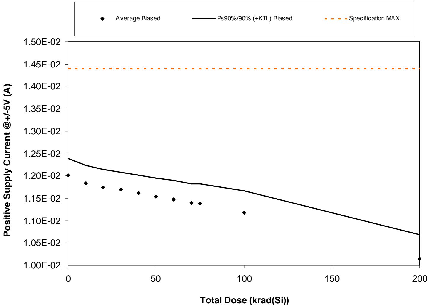
Figure 5.1. Plot of Positive Supply Current @ +/-5V (A) versus total dose. The solid diamonds are the average of the measured data points for the samples irradiated under electrical bias and the black lines (solid and/or dashed) are the average of the data points after application of the KTL statistics on the samples irradiated under electrical bias. The red dotted line(s) are the pre- and/or post-irradiation minimum and/or maximum specification value as defined in the datasheet and/or test plan.
