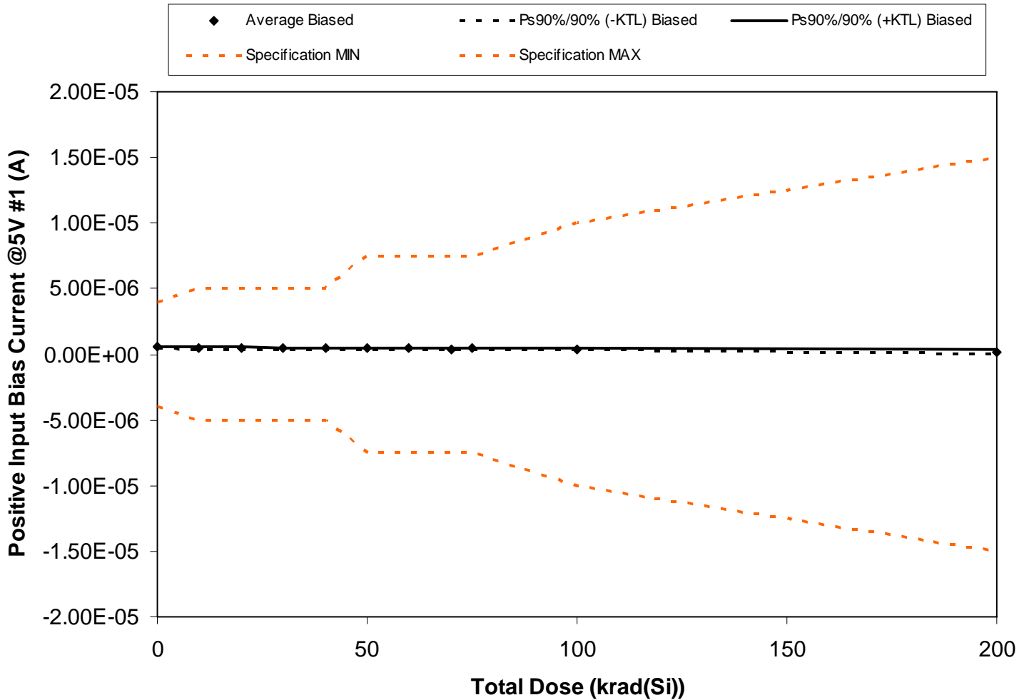
Figure 5.89. Plot of Positive Input Bias Current @5V #1 (A) versus total dose. The solid diamonds are the average of the measured data points for the samples irradiated under electrical bias and the black lines (solid and/or dashed) are the average of the data points after application of the KTL statistics on the samples irradiated under electrical bias. The red dotted line(s) are the pre- and/or post-irradiation minimum and/or maximum specification value as defined in the datasheet and/or test plan.
