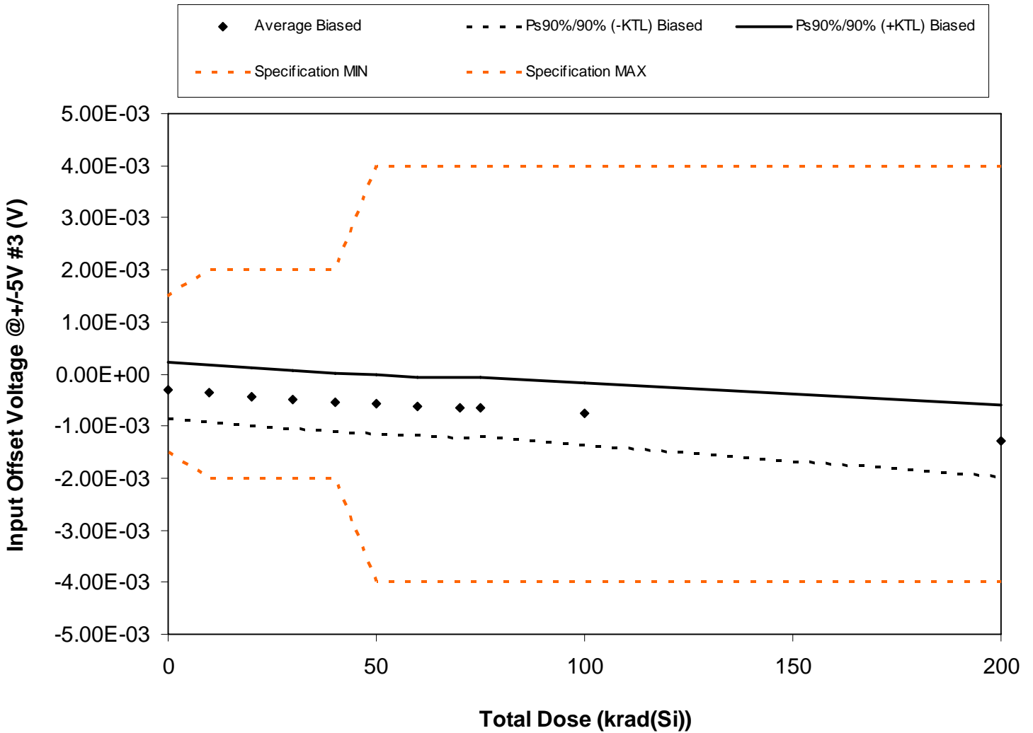
Figure 5.5. Plot of Input Offset Voltage @ +/-5V #3 (V) versus total dose. The solid diamonds are the average of the measured data points for the samples irradiated under electrical bias and the black lines (solid and/or dashed) are the average of the data points after application of the KTL statistics on the samples irradiated under electrical bias. The red dotted line(s) are the pre- and/or post-irradiation minimum and/or maximum specification value as defined in the datasheet and/or test plan.
