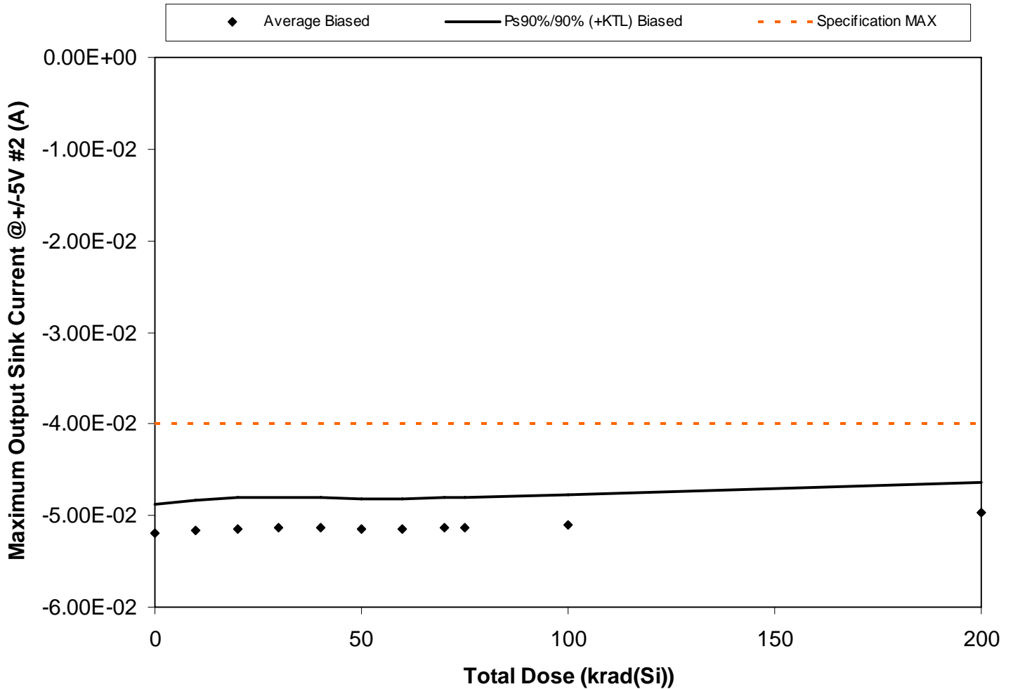
Figure 5.68. Plot of Maximum Output Sink Current @ +/-5V #2 (A) versus total dose. The solid diamonds are the average of the measured data points for the samples irradiated under electrical bias and the black lines (solid and/or dashed) are the average of the data points after application of the KTL statistics on the samples irradiated under electrical bias. The red dotted line(s) are the pre- and/or post-irradiation minimum and/or maximum specification value as defined in the datasheet and/or test plan.
