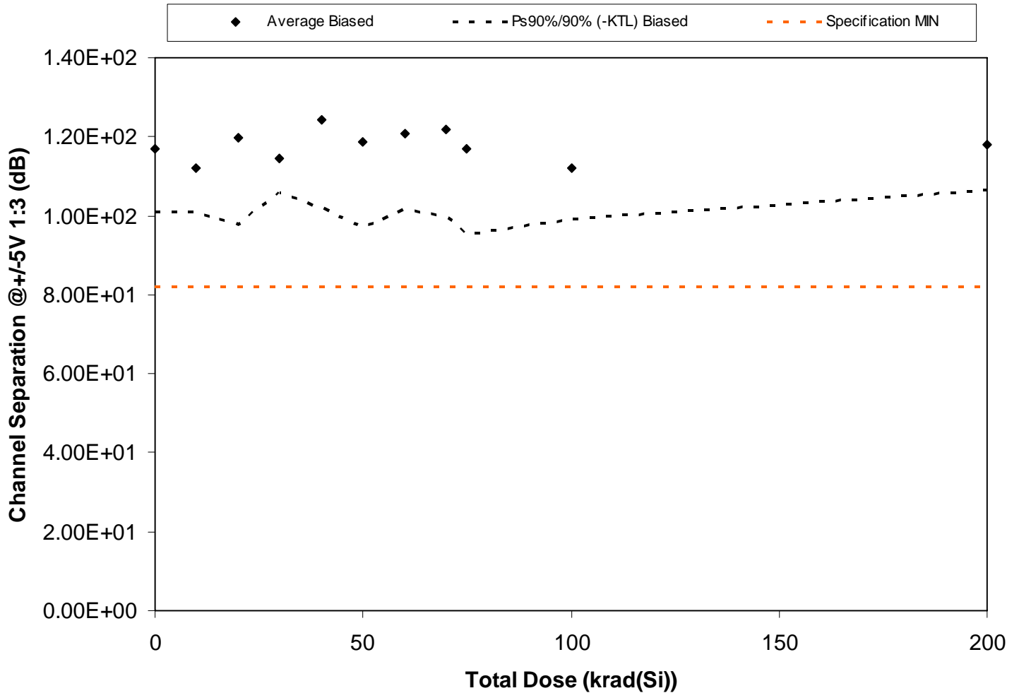
Figure 5.36. Plot of Channel Separation @ +/-5V 1:3 (dB) versus total dose. The solid diamonds are the average of the measured data points for the samples irradiated under electrical bias and the black lines (solid and/or dashed) are the average of the data points after application of the KTL statistics on the samples irradiated under electrical bias. The red dotted line(s) are the pre- and/or post-irradiation minimum and/or maximum specification value as defined in the datasheet and/or test plan.
