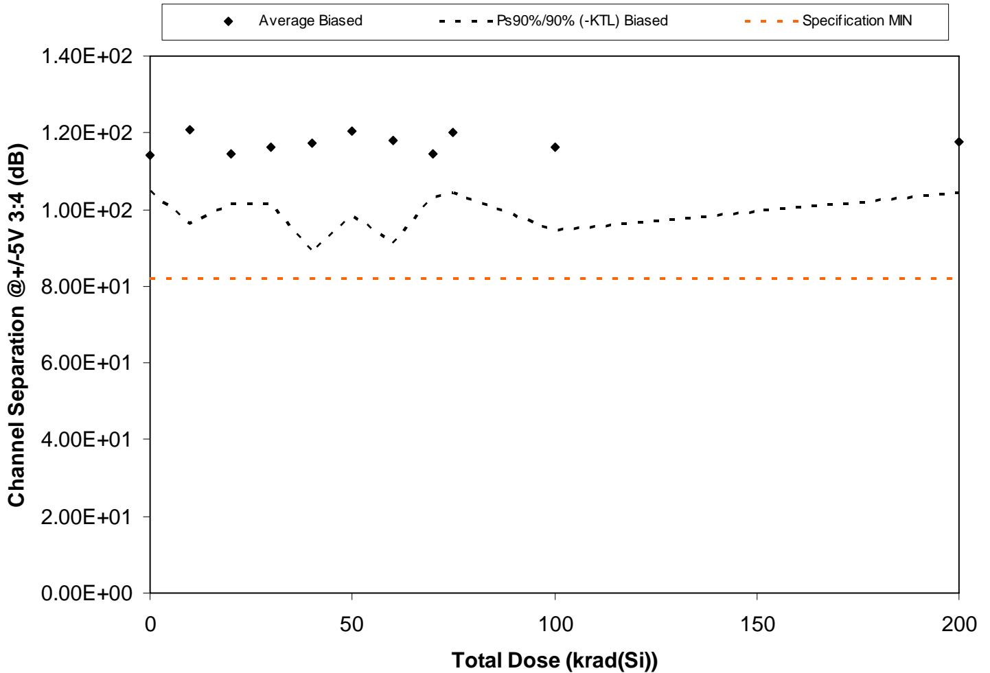
Figure 5.43. Plot of Channel Separation @ +/-5V 3:4 (dB) versus total dose. The solid diamonds are the average of the measured data points for the samples irradiated under electrical bias and the black lines (solid and/or dashed) are the average of the data points after application of the KTL statistics on the samples irradiated under electrical bias. The red dotted line(s) are the pre- and/or post-irradiation minimum and/or maximum specification value as defined in the datasheet and/or test plan.
