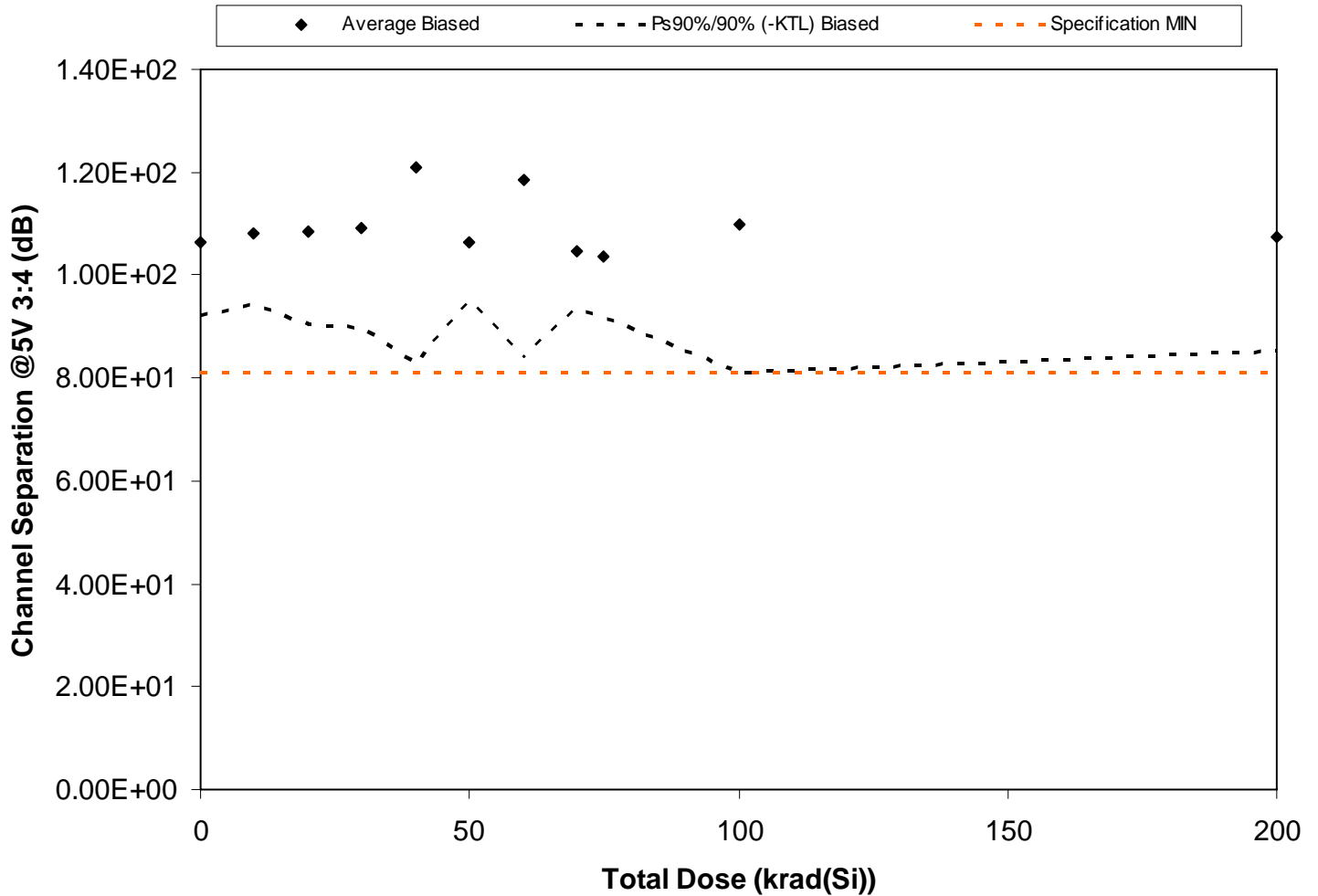
Figure 5.117. Plot of Channel Separation @5V 3:4 (dB) versus total dose. The solid diamonds are the average of the measured data points for the samples irradiated under electrical bias and the black lines (solid and/or dashed) are the average of the data points after application of the KTL statistics on the samples irradiated under electrical bias. The red dotted line(s) are the pre- and/or post-irradiation minimum and/or maximum specification value as defined in the datasheet and/or test plan.
