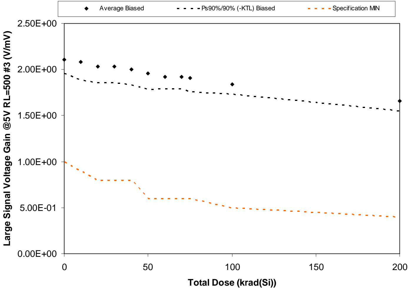
Figure 5.103. Plot of Large Signal Voltage Gain @5V RL=500 #3 (V/mV) versus total dose. The solid diamonds are the average of the measured data points for the samples irradiated under electrical bias and the black lines (solid and/or dashed) are the average of the data points after application of the KTL statistics on the samples irradiated under electrical bias. The red dotted line(s) are the pre- and/or post-irradiation minimum and/or maximum specification value as defined in the datasheet and/or test plan.
