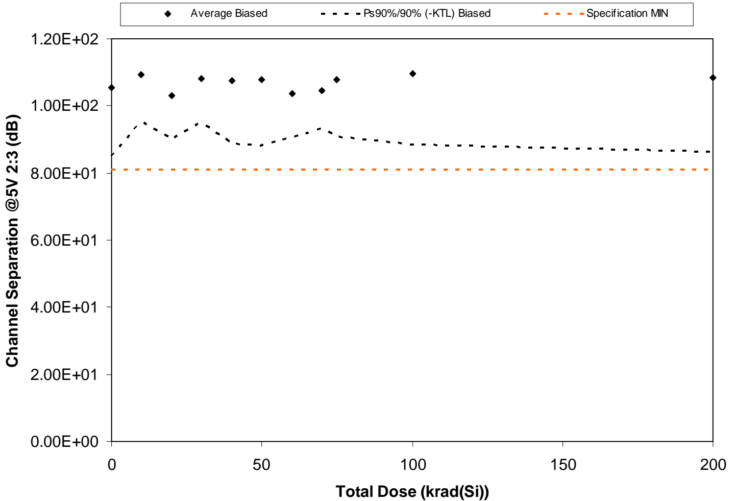
Figure 5.113. Plot of Channel Separation @5V 2:3 (dB) versus total dose. The solid diamonds are the average of the measured data points for the samples irradiated under electrical bias and the black lines (solid and/or dashed) are the average of the data points after application of the KTL statistics on the samples irradiated under electrical bias. The red dotted line(s) are the pre- and/or post-irradiation minimum and/or maximum specification value as defined in the datasheet and/or test plan.
