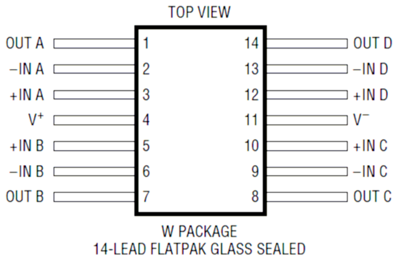
Figure B.2. W package drawing (for reference only). This figure was extracted from LINEAR TECHNOLOGY CORPORATION RH1814M Datasheet.
