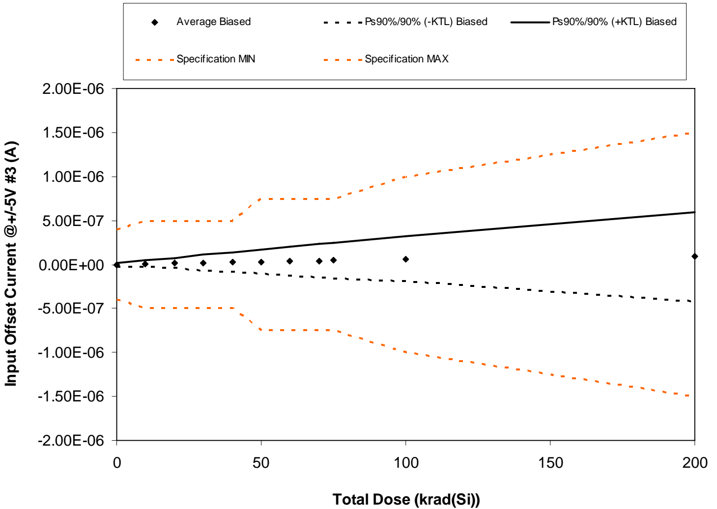
Figure 5.9. Plot of Input Offset Current @ +/-5V #3 (A) versus total dose. The solid diamonds are the average of the measured data points for the samples irradiated under electrical bias and the black lines (solid and/or dashed) are the average of the data points after application of the KTL statistics on the samples irradiated under electrical bias. The red dotted line(s) are the pre- and/or post-irradiation minimum and/or maximum specification value as defined in the datasheet and/or test plan.
