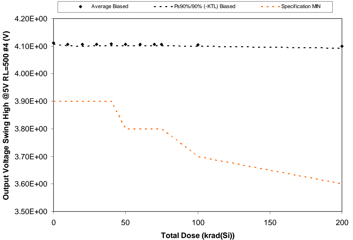
Figure 5.124. Plot of Output Voltage Swing High @5V RL=500 #4 (V) versus total dose. The solid diamonds are the average of the measured data points for the samples irradiated under electrical bias and the black lines (solid and/or dashed) are the average of the data points after application of the KTL statistics on the samples irradiated under electrical bias. The red dotted line(s) are the pre- and/or post-irradiation minimum and/or maximum specification value as defined in the datasheet and/or test plan.
