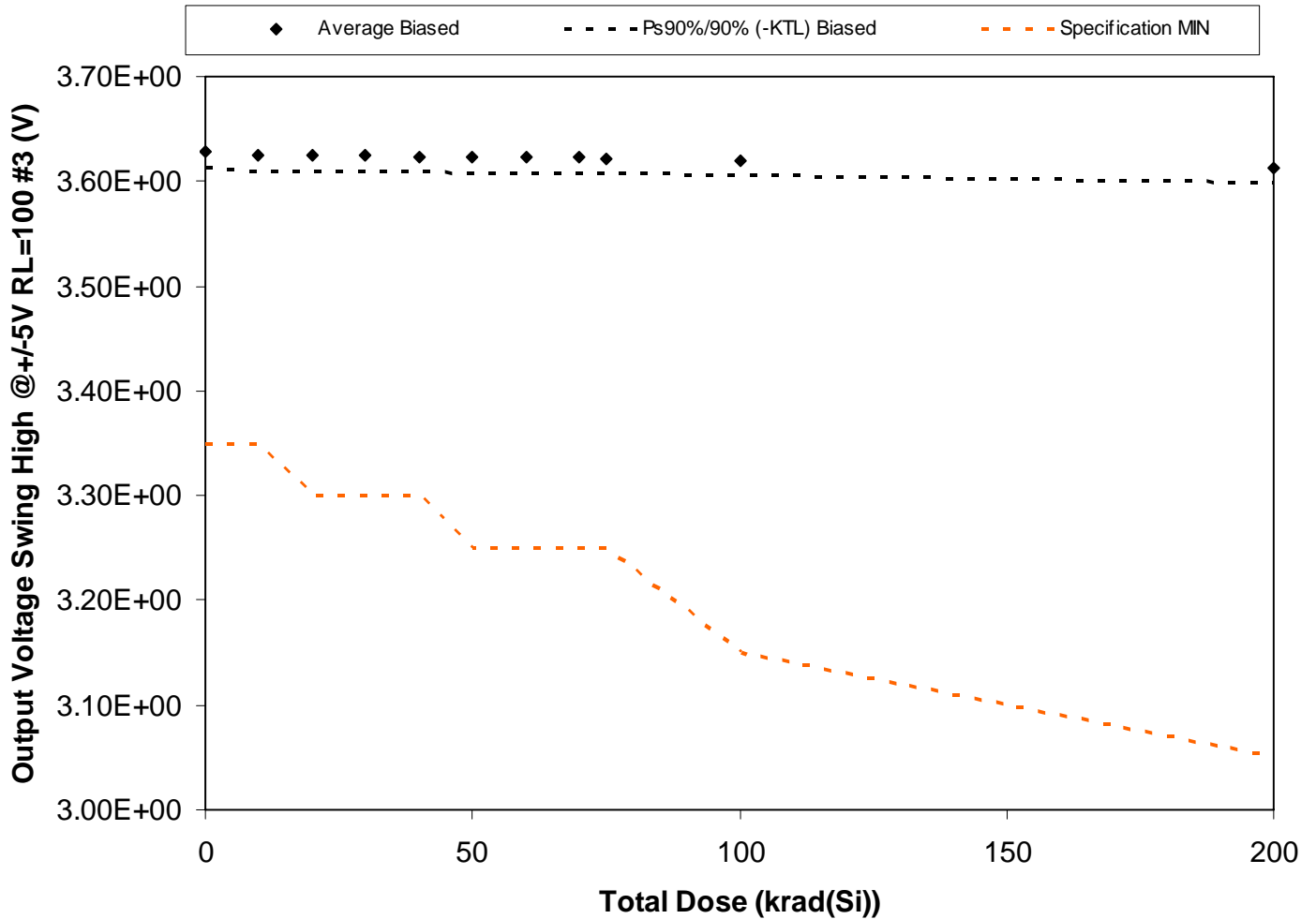
Figure 5.53. Plot of Output Voltage Swing High @ +/-5V RL=100 #3 (V) versus total dose. The solid diamonds are the average of the measured data points for the samples irradiated under electrical bias and the black lines (solid and/or dashed) are the average of the data points after application of the KTL statistics on the samples irradiated under electrical bias. The red dotted line(s) are the pre- and/or post-irradiation minimum and/or maximum specification value as defined in the datasheet and/or test plan.
