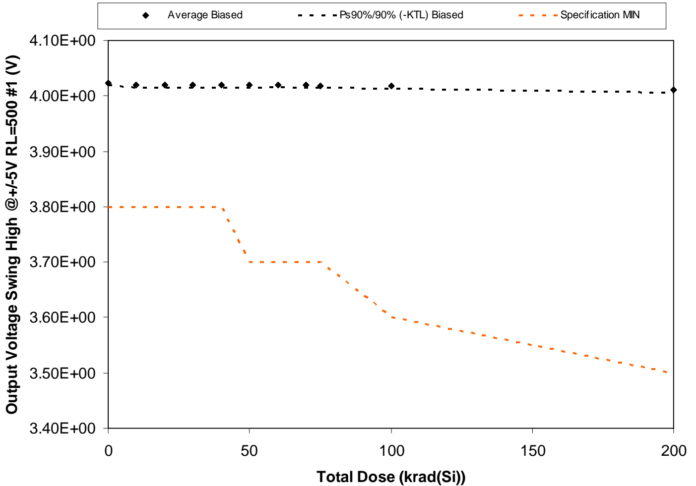
Figure 5.47. Plot of Output Voltage Swing High @ +/-5V RL=500 #1 (V) versus total dose. The solid diamonds are the average of the measured data points for the samples irradiated under electrical bias and the black lines (solid and/or dashed) are the average of the data points after application of the KTL statistics on the samples irradiated under electrical bias. The red dotted line(s) are the pre- and/or post-irradiation minimum and/or maximum specification value as defined in the datasheet and/or test plan.
