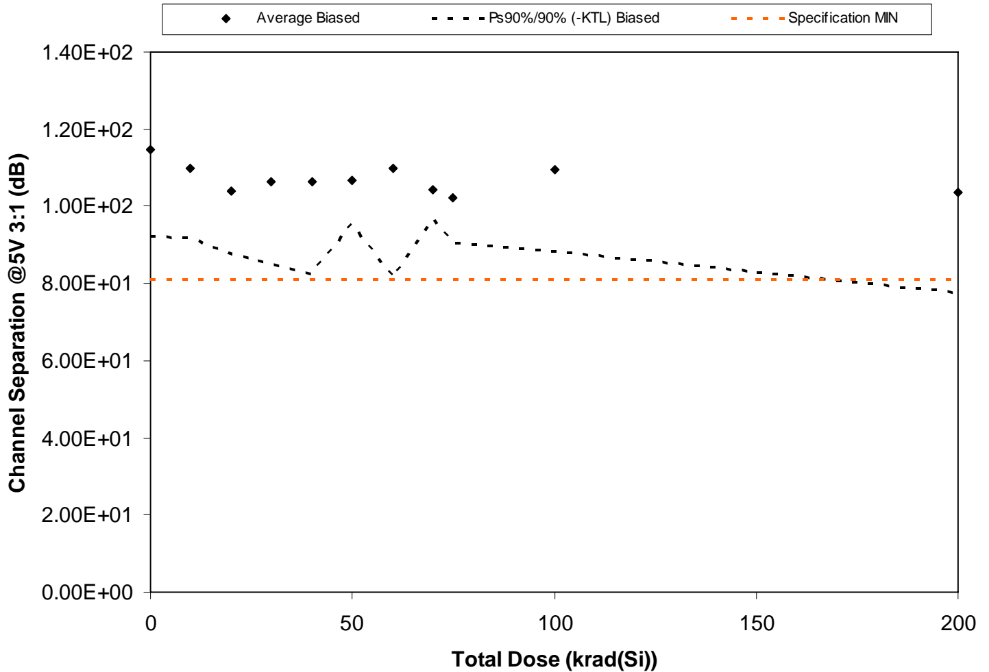
Figure 5.115. Plot of Channel Separation @5V 3:1 (dB) versus total dose. The solid diamonds are the average of the measured data points for the samples irradiated under electrical bias and the black lines (solid and/or dashed) are the average of the data points after application of the KTL statistics on the samples irradiated under electrical bias. The red dotted line(s) are the pre- and/or post-irradiation minimum and/or maximum specification value as defined in the datasheet and/or test plan.
