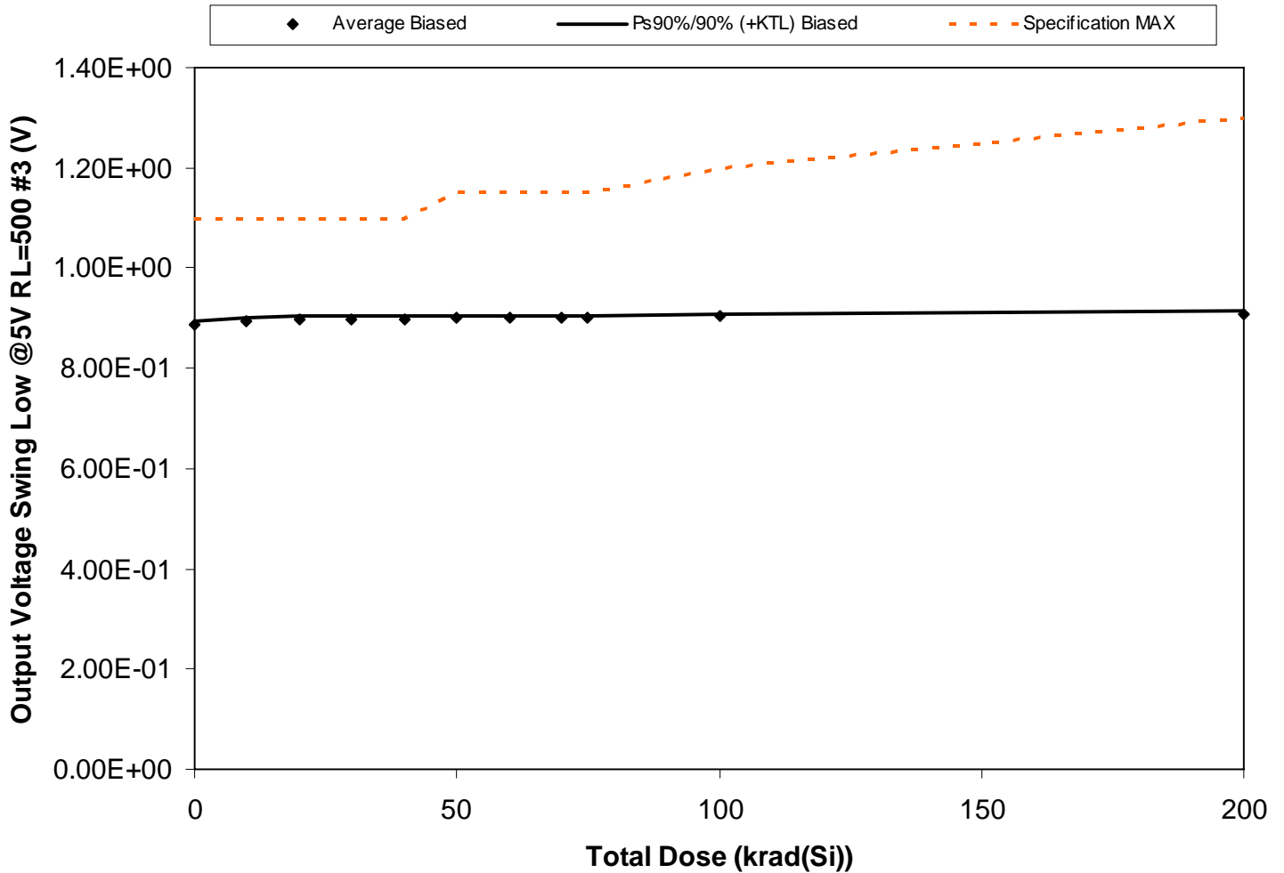
Figure 5.131. Plot of Output Voltage Swing Low @5V RL=500 #3 (V) versus total dose. The solid diamonds are the average of the measured data points for the samples irradiated under electrical bias and the black lines (solid and/or dashed) are the average of the data points after application of the KTL statistics on the samples irradiated under electrical bias. The red dotted line(s) are the pre- and/or post-irradiation minimum and/or maximum specification value as defined in the datasheet and/or test plan.
