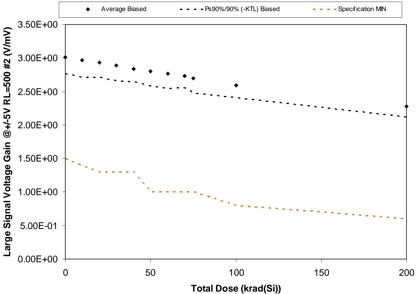
Figure 5.28. Plot of Large Signal Voltage Gain @ +/-5V RL=500 #2 (V/mV) versus total dose. The solid diamonds are the average of the measured data points for the samples irradiated under electrical bias and the black lines (solid and/or dashed) are the average of the data points after application of the KTL statistics on the samples irradiated under electrical bias. The red dotted line(s) are the pre- and/or post-irradiation minimum and/or maximum specification value as defined in the datasheet and/or test plan.
