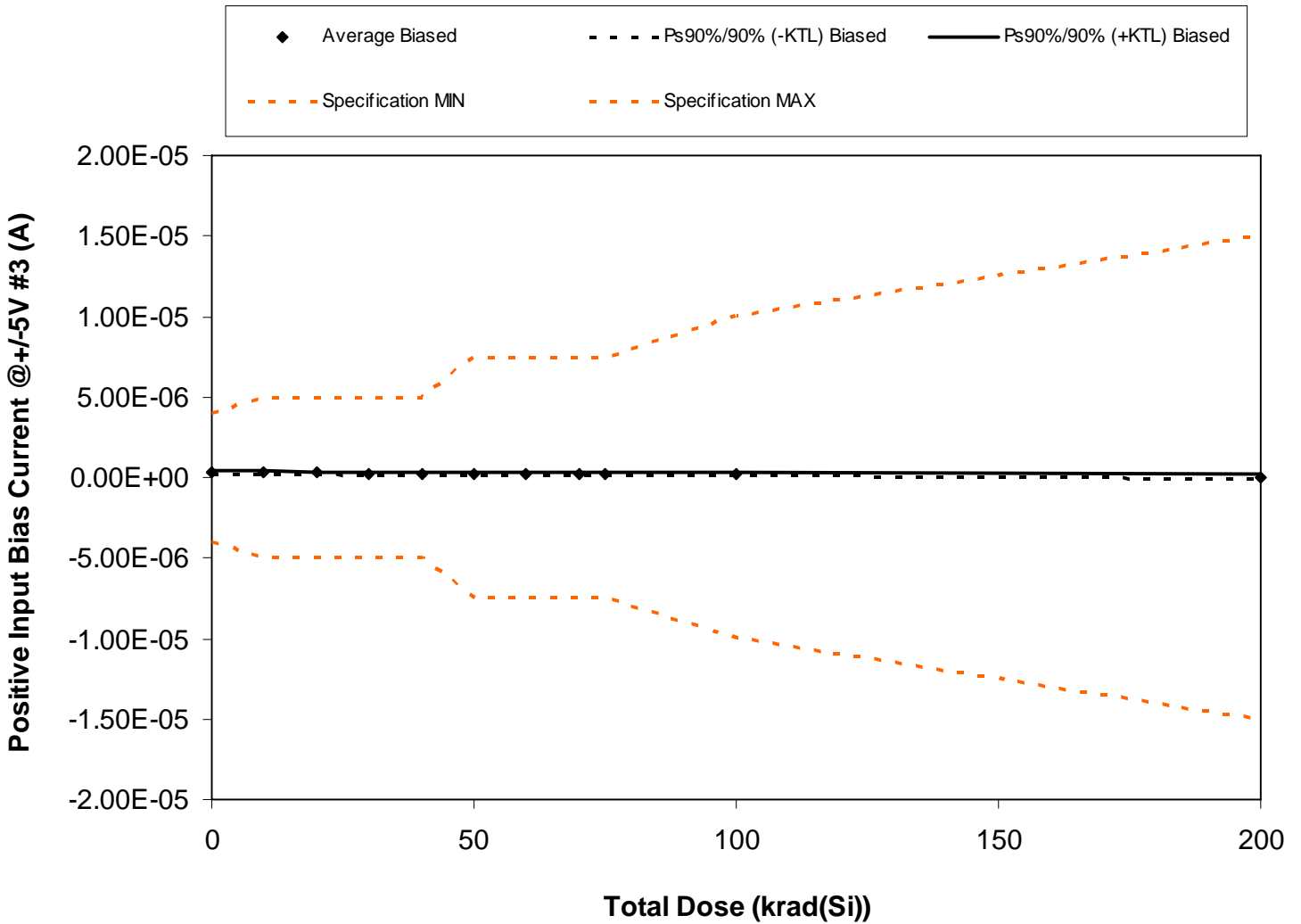
Figure 5.13. Plot of Positive Input Bias Current @ +/-5V #3 (A) versus total dose. The solid diamonds are the average of the measured data points for the samples irradiated under electrical bias and the black lines (solid and/or dashed) are the average of the data points after application of the KTL statistics on the samples irradiated under electrical bias. The red dotted line(s) are the pre- and/or post-irradiation minimum and/or maximum specification value as defined in the datasheet and/or test plan.
