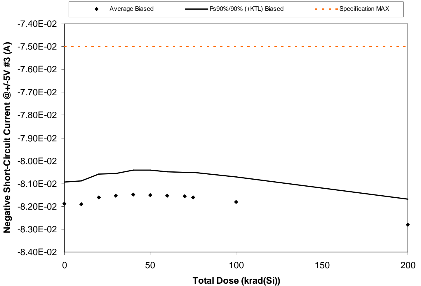
Figure 5.77. Plot of Negative Short-Circuit Current @ +/-5V #3 (A) versus total dose. The solid diamonds are the average of the measured data points for the samples irradiated under electrical bias and the black lines (solid and/or dashed) are the average of the data points after application of the KTL statistics on the samples irradiated under electrical bias. The red dotted line(s) are the pre- and/or post-irradiation minimum and/or maximum specification value as defined in the datasheet and/or test plan.
