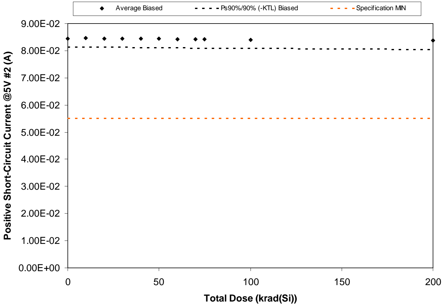
Figure 5.146. Plot of Positive Short-Circuit Current @5V #2 (A) versus total dose. The solid diamonds are the average of the measured data points for the samples irradiated under electrical bias and the black lines (solid and/or dashed) are the average of the data points after application of the KTL statistics on the samples irradiated under electrical bias. The red dotted line(s) are the pre- and/or post-irradiation minimum and/or maximum specification value as defined in the datasheet and/or test plan.
