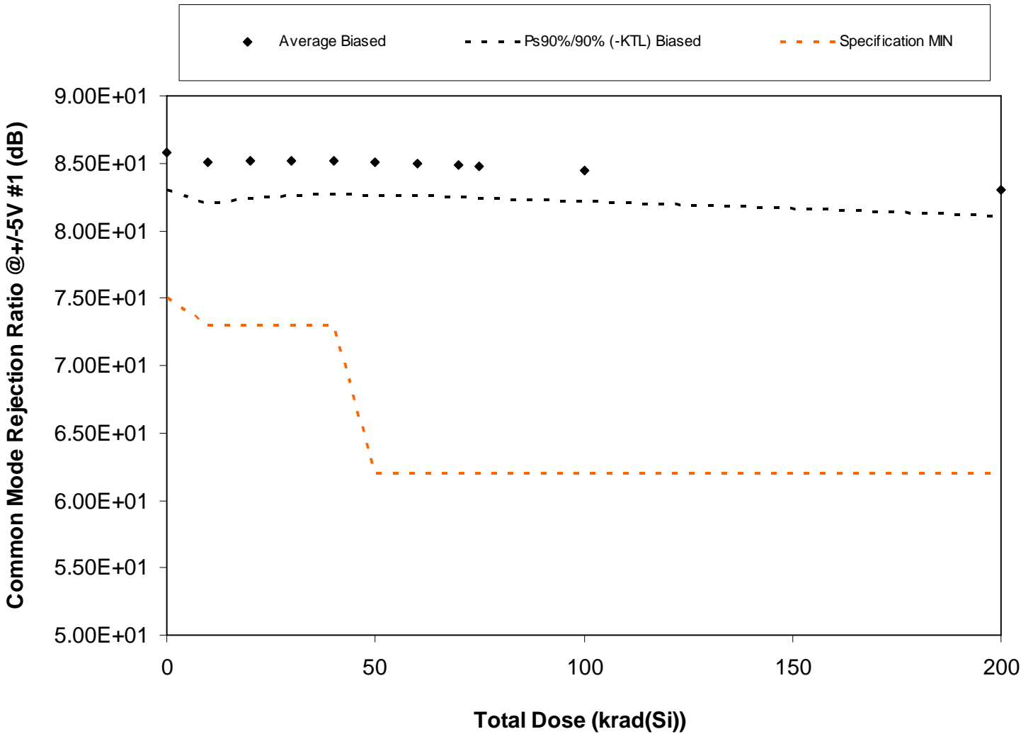
Figure 5.19. Plot of Common Mode Rejection Ratio @ +/-5V #1 (dB) versus total dose. The solid diamonds are the average of the measured data points for the samples irradiated under electrical bias and the black lines (solid and/or dashed) are the average of the data points after application of the KTL statistics on the samples irradiated under electrical bias. The red dotted line(s) are the pre- and/or post-irradiation minimum and/or maximum specification value as defined in the datasheet and/or test plan.
