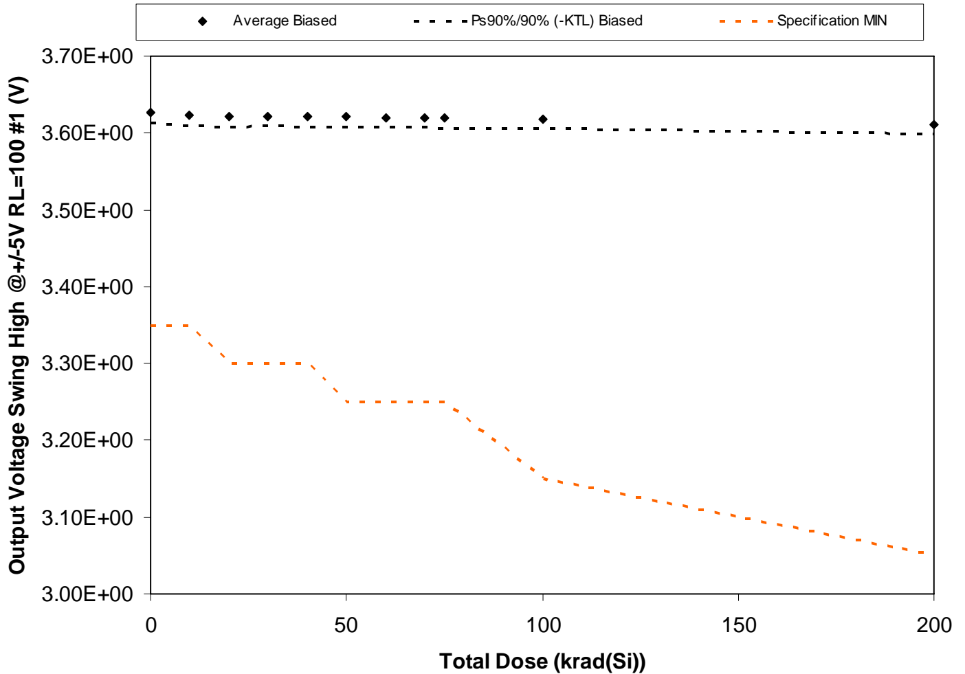
Figure 5.51. Plot of Output Voltage Swing High @ +/-5V RL=100 #1 (V) versus total dose. The solid diamonds are the average of the measured data points for the samples irradiated under electrical bias and the black lines (solid and/or dashed) are the average of the data points after application of the KTL statistics on the samples irradiated under electrical bias. The red dotted line(s) are the pre- and/or post-irradiation minimum and/or maximum specification value as defined in the datasheet and/or test plan.
