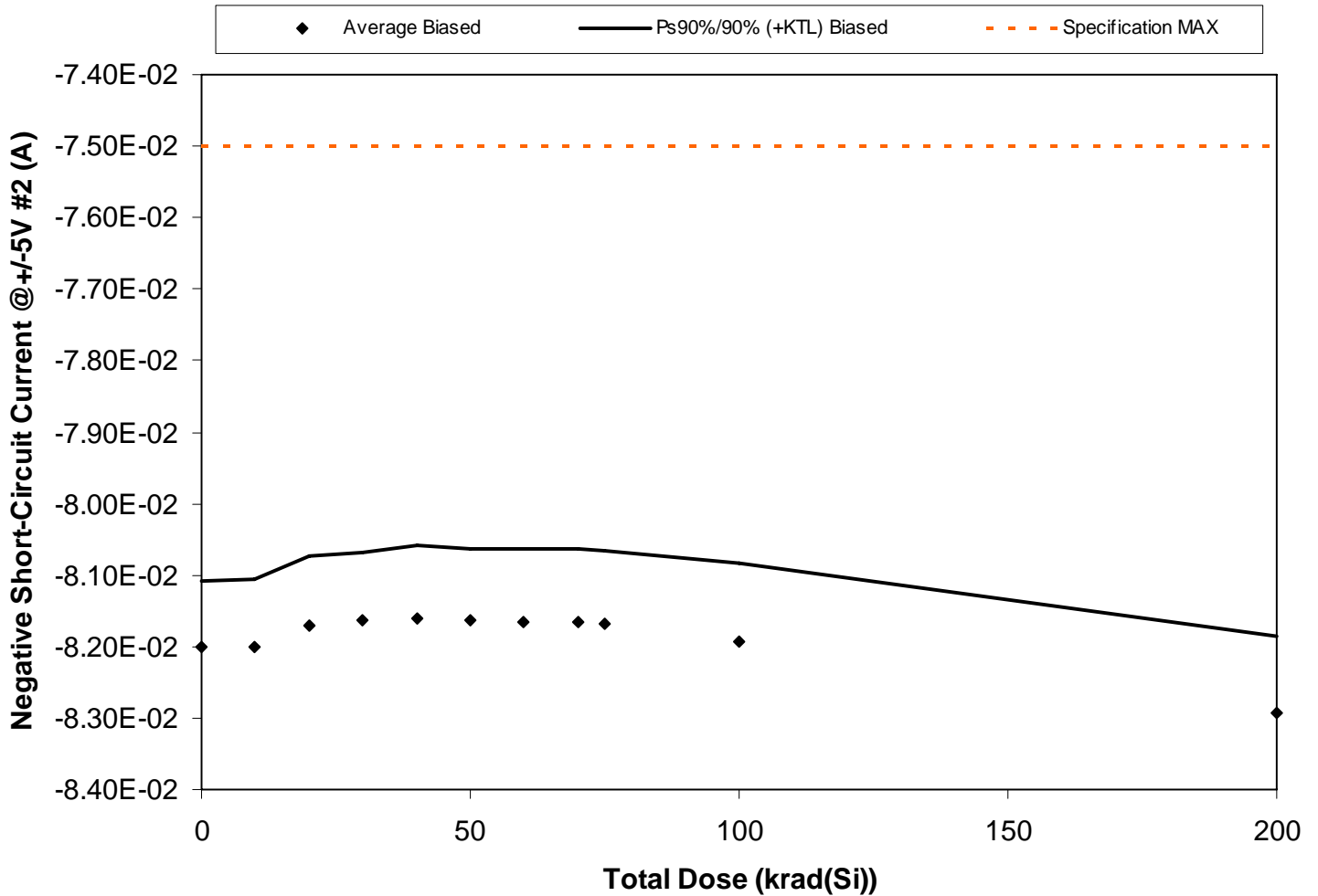
Figure 5.76. Plot of Negative Short-Circuit Current @ +/-5V #2 (A) versus total dose. The solid diamonds are the average of the measured data points for the samples irradiated under electrical bias and the black lines (solid and/or dashed) are the average of the data points after application of the KTL statistics on the samples irradiated under electrical bias. The red dotted line(s) are the pre- and/or post-irradiation minimum and/or maximum specification value as defined in the datasheet and/or test plan.
