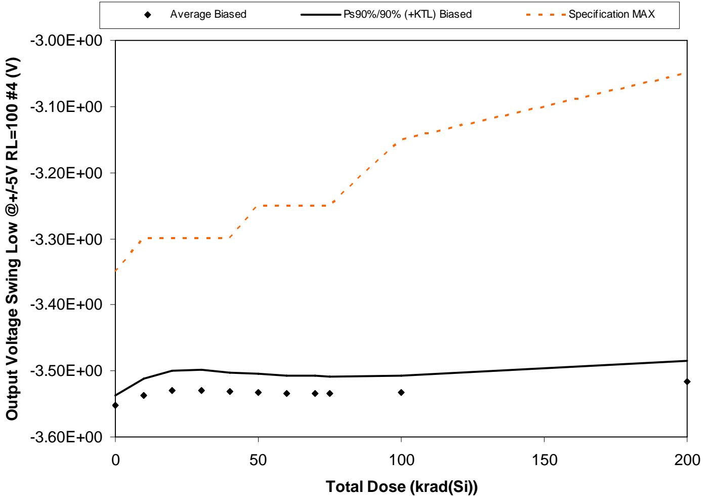
Figure 5.62. Plot of Output Voltage Swing Low @ +/-5V RL=100 #4 (V) versus total dose. The solid diamonds are the average of the measured data points for the samples irradiated under electrical bias and the black lines (solid and/or dashed) are the average of the data points after application of the KTL statistics on the samples irradiated under electrical bias. The red dotted line(s) are the pre- and/or post-irradiation minimum and/or maximum specification value as defined in the datasheet and/or test plan.
