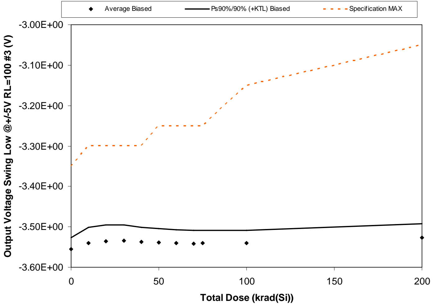
Figure 5.61. Plot of Output Voltage Swing Low @ +/-5V RL=100 #3 (V) versus total dose. The solid diamonds are the average of the measured data points for the samples irradiated under electrical bias and the black lines (solid and/or dashed) are the average of the data points after application of the KTL statistics on the samples irradiated under electrical bias. The red dotted line(s) are the pre- and/or post-irradiation minimum and/or maximum specification value as defined in the datasheet and/or test plan.
