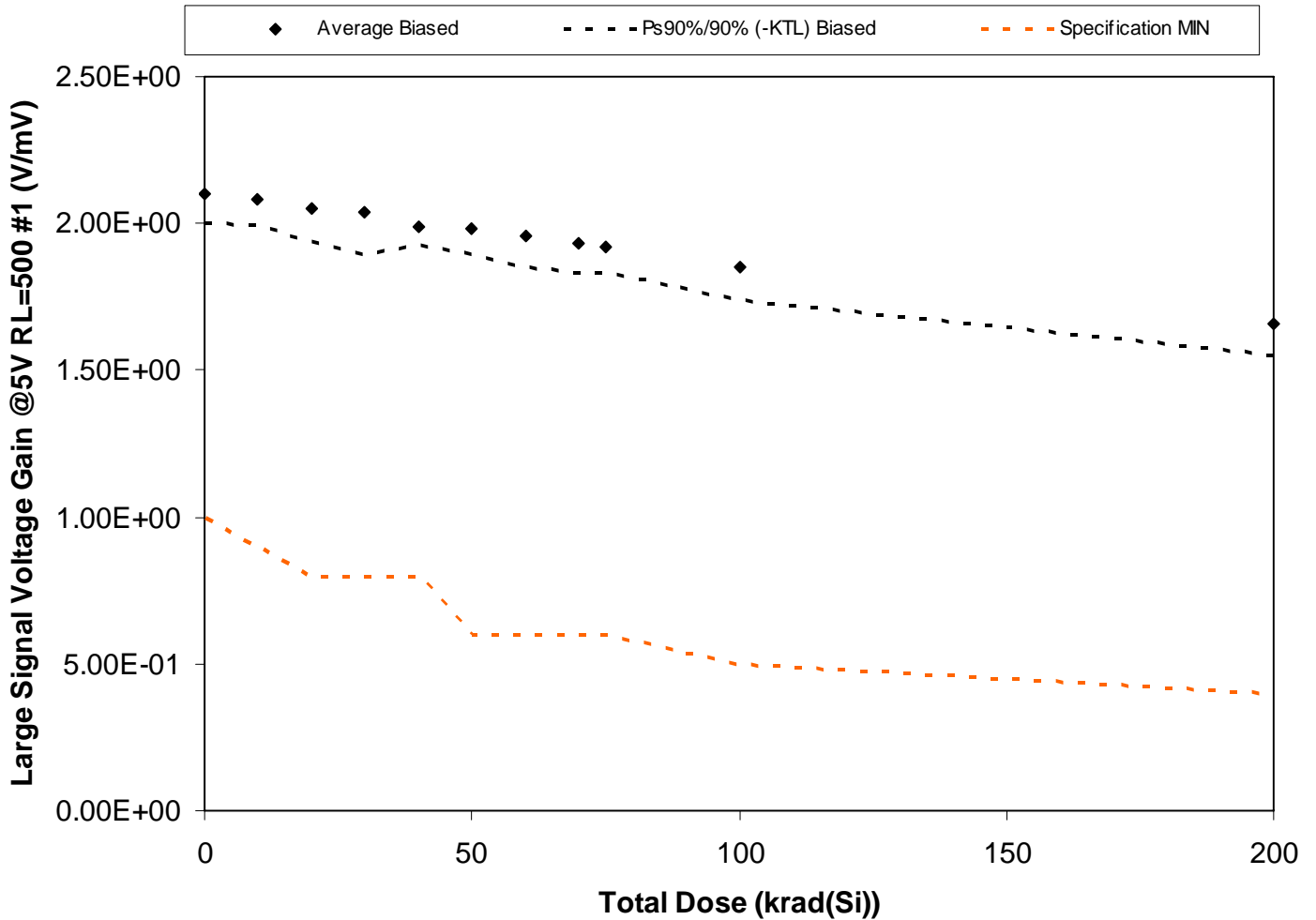
Figure 5.101. Plot of Large Signal Voltage Gain @5V RL=500 #1 (V/mV) versus total dose. The solid diamonds are the average of the measured data points for the samples irradiated under electrical bias and the black lines (solid and/or dashed) are the average of the data points after application of the KTL statistics on the samples irradiated under electrical bias. The red dotted line(s) are the pre- and/or post-irradiation minimum and/or maximum specification value as defined in the datasheet and/or test plan.
