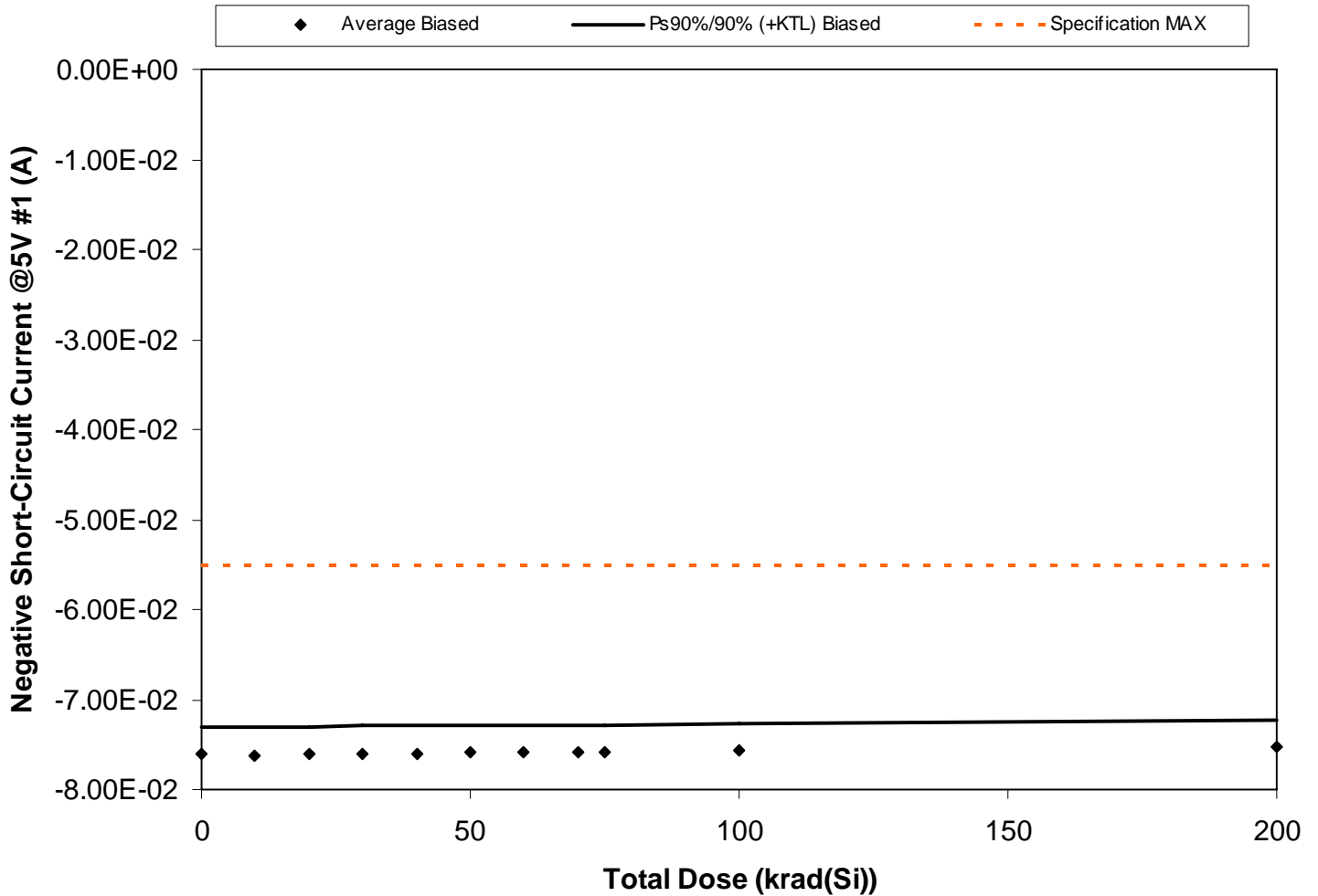
Figure 5.149. Plot of Negative Short-Circuit Current @5V #1 (A) versus total dose. The solid diamonds are the average of the measured data points for the samples irradiated under electrical bias and the black lines (solid and/or dashed) are the average of the data points after application of the KTL statistics on the samples irradiated under electrical bias. The red dotted line(s) are the pre- and/or post-irradiation minimum and/or maximum specification value as defined in the datasheet and/or test plan.
