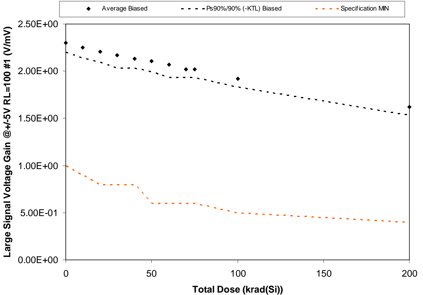
Figure 5.31. Plot of Large Signal Voltage Gain @ +/-5V RL=100 #1 (V/mV) versus total dose. The solid diamonds are the average of the measured data points for the samples irradiated under electrical bias and the black lines (solid and/or dashed) are the average of the data points after application of the KTL statistics on the samples irradiated under electrical bias. The red dotted line(s) are the pre- and/or post-irradiation minimum and/or maximum specification value as defined in the datasheet and/or test plan.
