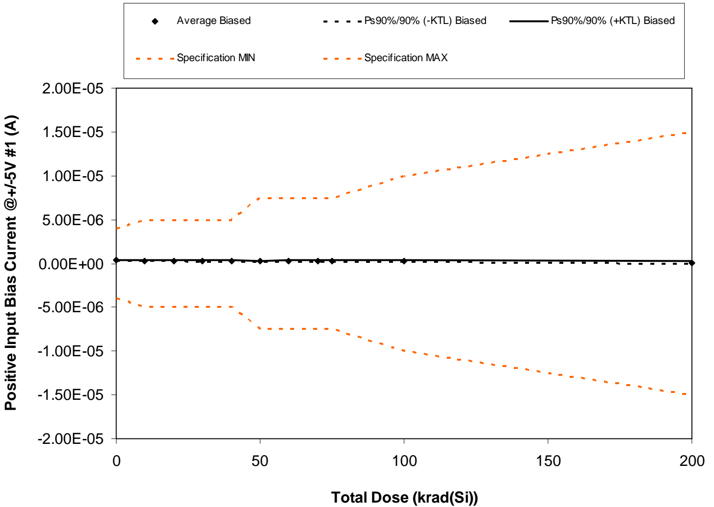
Figure 5.11. Plot of Positive Input Bias Current @ +/-5V #1 (A) versus total dose. The solid diamonds are the average of the measured data points for the samples irradiated under electrical bias and the black lines (solid and/or dashed) are the average of the data points after application of the KTL statistics on the samples irradiated under electrical bias. The red dotted line(s) are the pre- and/or post-irradiation minimum and/or maximum specification value as defined in the datasheet and/or test plan.
