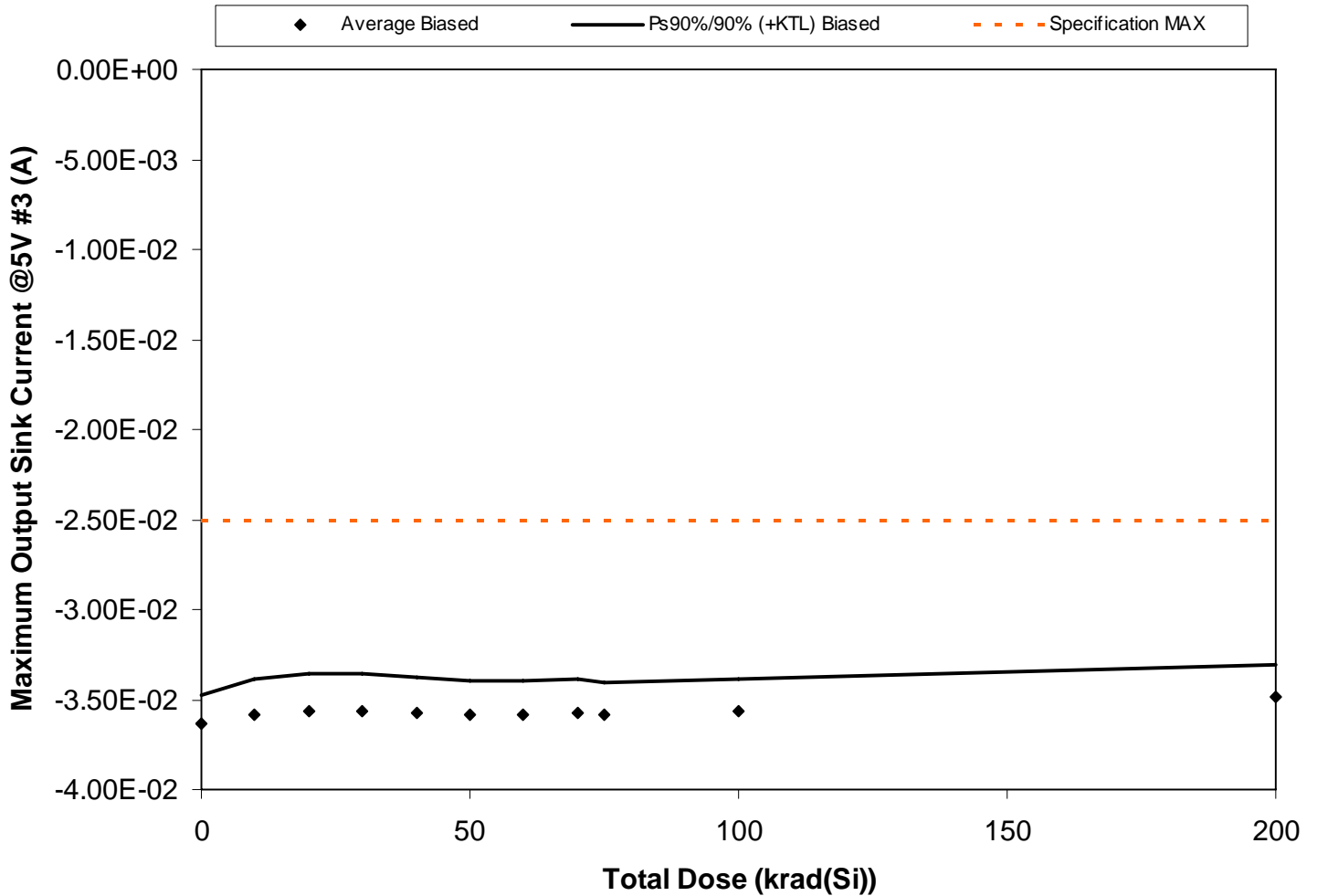
Figure 5.143. Plot of Maximum Output Sink Current @5V #3 (A) versus total dose. The solid diamonds are the average of the measured data points for the samples irradiated under electrical bias and the black lines (solid and/or dashed) are the average of the data points after application of the KTL statistics on the samples irradiated under electrical bias. The red dotted line(s) are the pre- and/or post-irradiation minimum and/or maximum specification value as defined in the datasheet and/or test plan.
