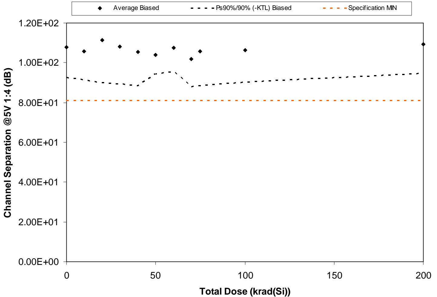
Figure 5.111. Plot of Channel Separation @5V 1:4 (dB) versus total dose. The solid diamonds are the average of the measured data points for the samples irradiated under electrical bias and the black lines (solid and/or dashed) are the average of the data points after application of the KTL statistics on the samples irradiated under electrical bias. The red dotted line(s) are the pre- and/or post-irradiation minimum and/or maximum specification value as defined in the datasheet and/or test plan.
