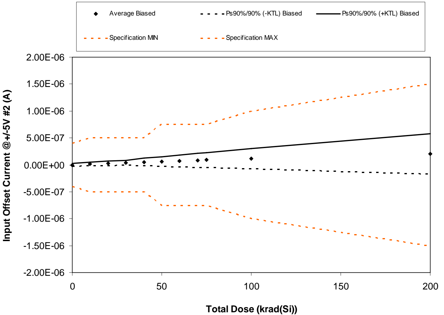
Figure 5.8. Plot of Input Offset Current @ +/-5V #2 (A) versus total dose. The solid diamonds are the average of the measured data points for the samples irradiated under electrical bias and the black lines (solid and/or dashed) are the average of the data points after application of the KTL statistics on the samples irradiated under electrical bias. The red dotted line(s) are the pre- and/or post-irradiation minimum and/or maximum specification value as defined in the datasheet and/or test plan.
