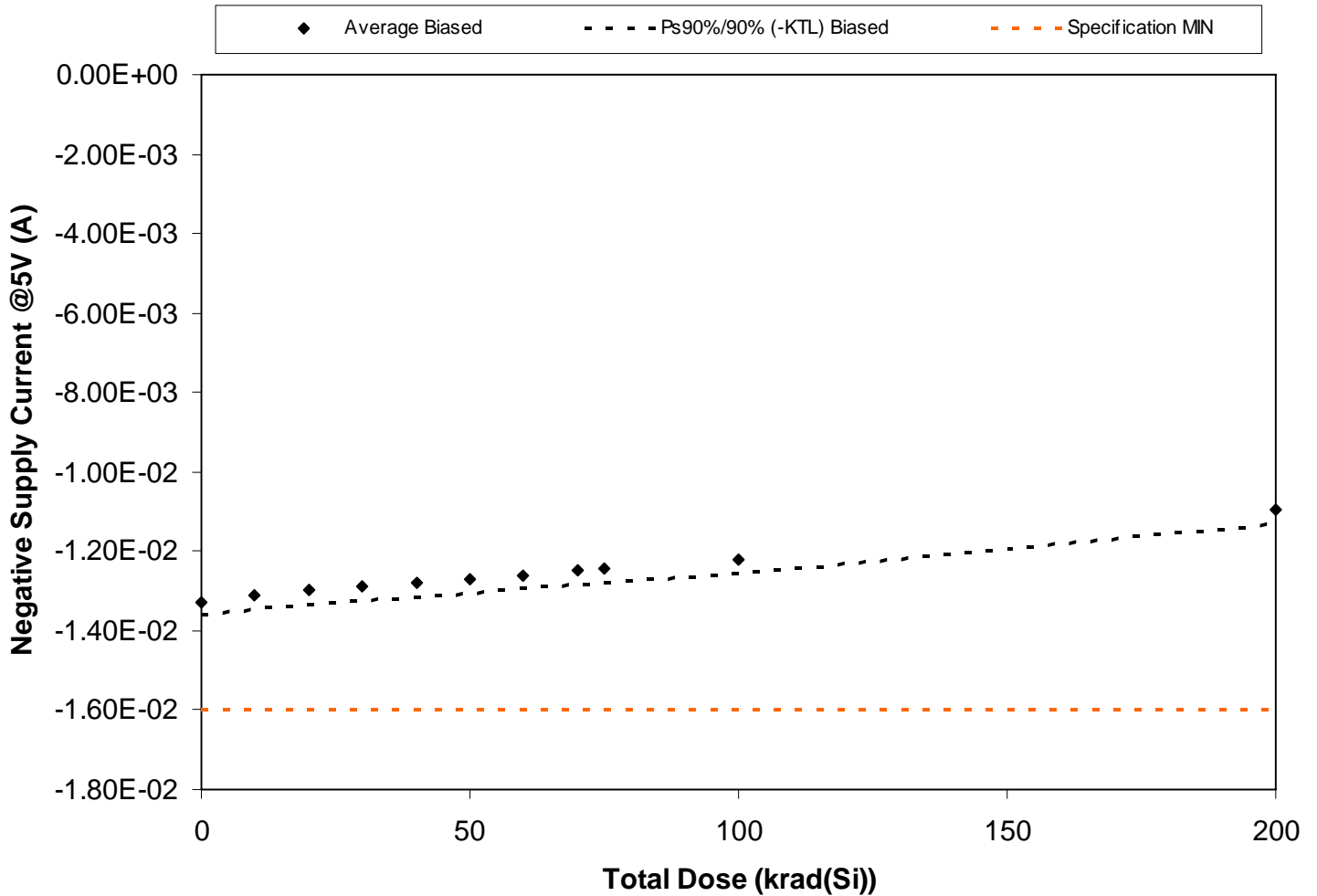
Figure 5.80. Plot of Negative Supply Current @5V (A) versus total dose. The solid diamonds are the average of the measured data points for the samples irradiated under electrical bias and the black lines (solid and/or dashed) are the average of the data points after application of the KTL statistics on the samples irradiated under electrical bias. The red dotted line(s) are the pre- and/or post-irradiation minimum and/or maximum specification value as defined in the datasheet and/or test plan.
