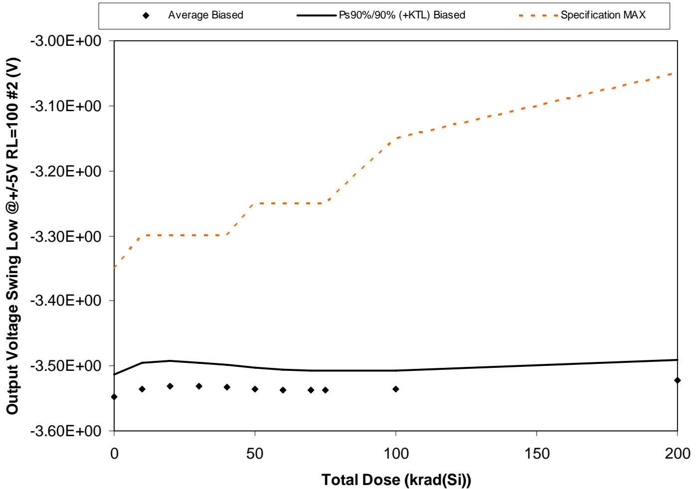
Figure 5.60. Plot of Output Voltage Swing Low @ +/-5V RL=100 #2 (V) versus total dose. The solid diamonds are the average of the measured data points for the samples irradiated under electrical bias and the black lines (solid and/or dashed) are the average of the data points after application of the KTL statistics on the samples irradiated under electrical bias. The red dotted line(s) are the pre- and/or post-irradiation minimum and/or maximum specification value as defined in the datasheet and/or test plan.
