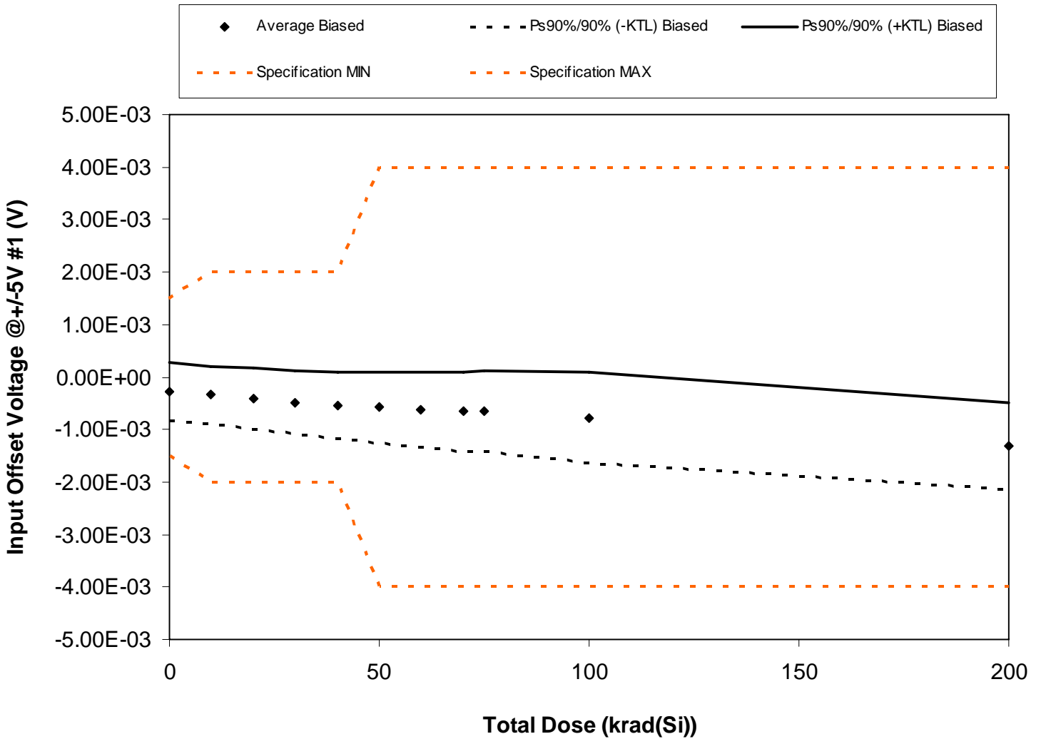
Figure 5.3. Plot of Input Offset Voltage @ +/-5V #1 (V) versus total dose. The solid diamonds are the average of the measured data points for the samples irradiated under electrical bias and the black lines (solid and/or dashed) are the average of the data points after application of the KTL statistics on the samples irradiated under electrical bias. The red dotted line(s) are the pre- and/or post-irradiation minimum and/or maximum specification value as defined in the datasheet and/or test plan.
