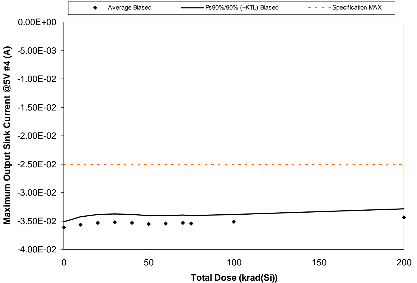
Figure 5.144. Plot of Maximum Output Sink Current @5V #4 (A) versus total dose. The solid diamonds are the average of the measured data points for the samples irradiated under electrical bias and the black lines (solid and/or dashed) are the average of the data points after application of the KTL statistics on the samples irradiated under electrical bias. The red dotted line(s) are the pre- and/or post-irradiation minimum and/or maximum specification value as defined in the datasheet and/or test plan.
