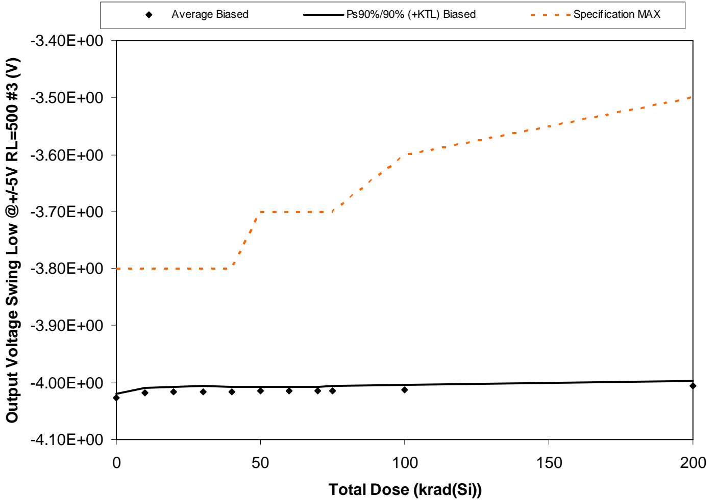
Figure 5.57. Plot of Output Voltage Swing Low @ +/-5V RL=500 #3 (V) versus total dose. The solid diamonds are the average of the measured data points for the samples irradiated under electrical bias and the black lines (solid and/or dashed) are the average of the data points after application of the KTL statistics on the samples irradiated under electrical bias. The red dotted line(s) are the pre- and/or post-irradiation minimum and/or maximum specification value as defined in the datasheet and/or test plan.
