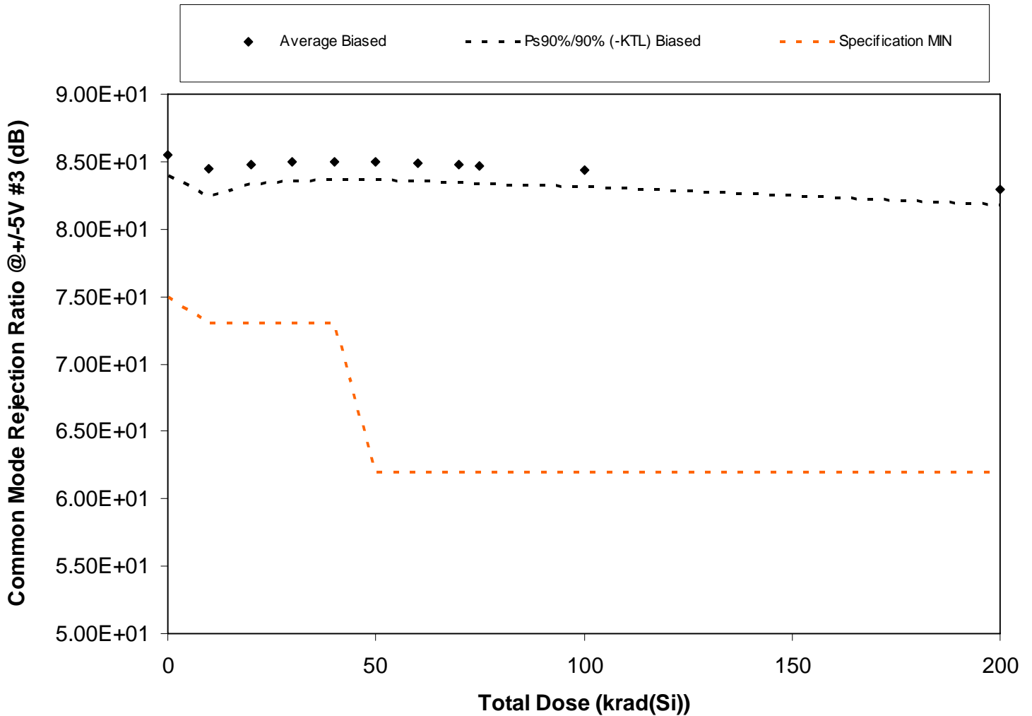
Figure 5.21. Plot of Common Mode Rejection Ratio @ +/-5V #3 (dB) versus total dose. The solid diamonds are the average of the measured data points for the samples irradiated under electrical bias and the black lines (solid and/or dashed) are the average of the data points after application of the KTL statistics on the samples irradiated under electrical bias. The red dotted line(s) are the pre- and/or post-irradiation minimum and/or maximum specification value as defined in the datasheet and/or test plan.
