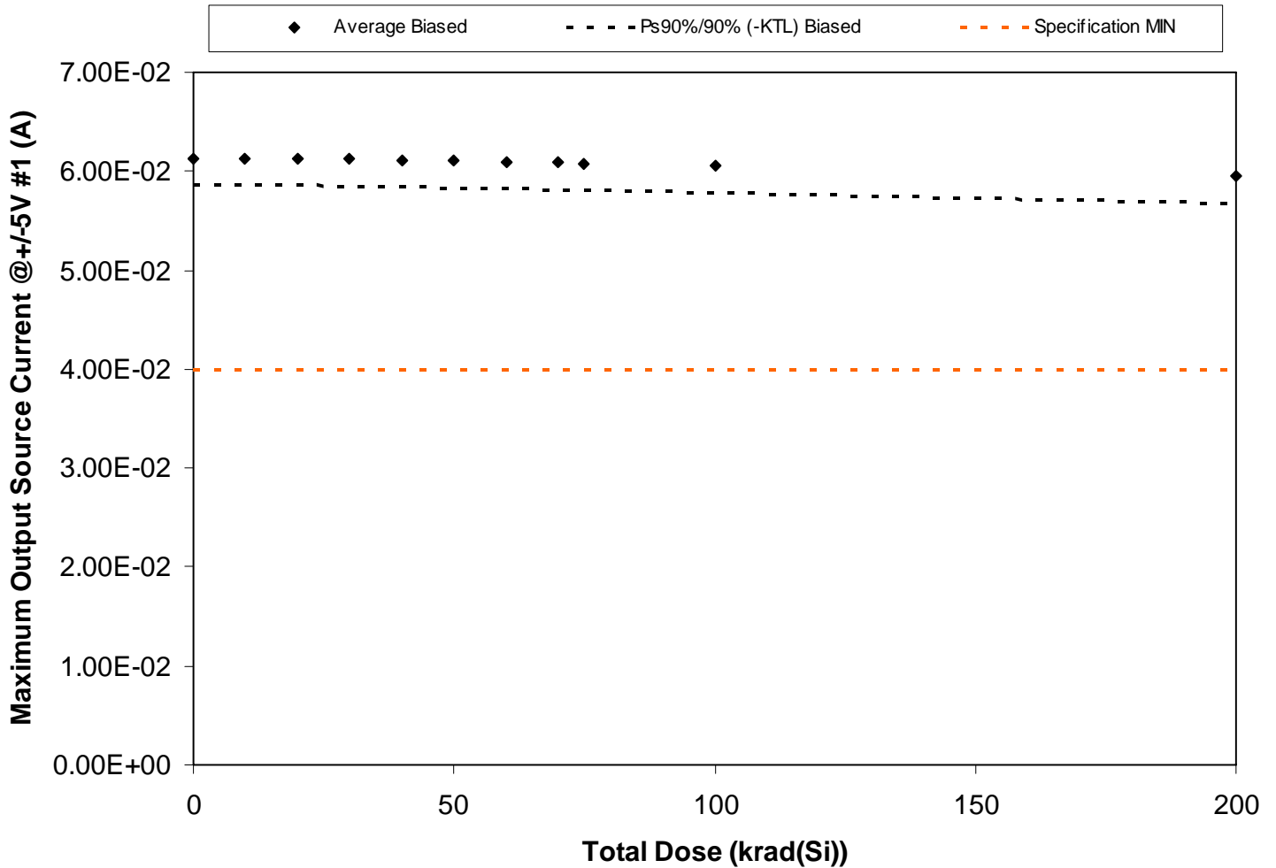
Figure 5.63. Plot of Maximum Output Source Current @ +/-5V #1 (A) versus total dose. The solid diamonds are the average of the measured data points for the samples irradiated under electrical bias and the black lines (solid and/or dashed) are the average of the data points after application of the KTL statistics on the samples irradiated under electrical bias. The red dotted line(s) are the pre- and/or post-irradiation minimum and/or maximum specification value as defined in the datasheet and/or test plan.
