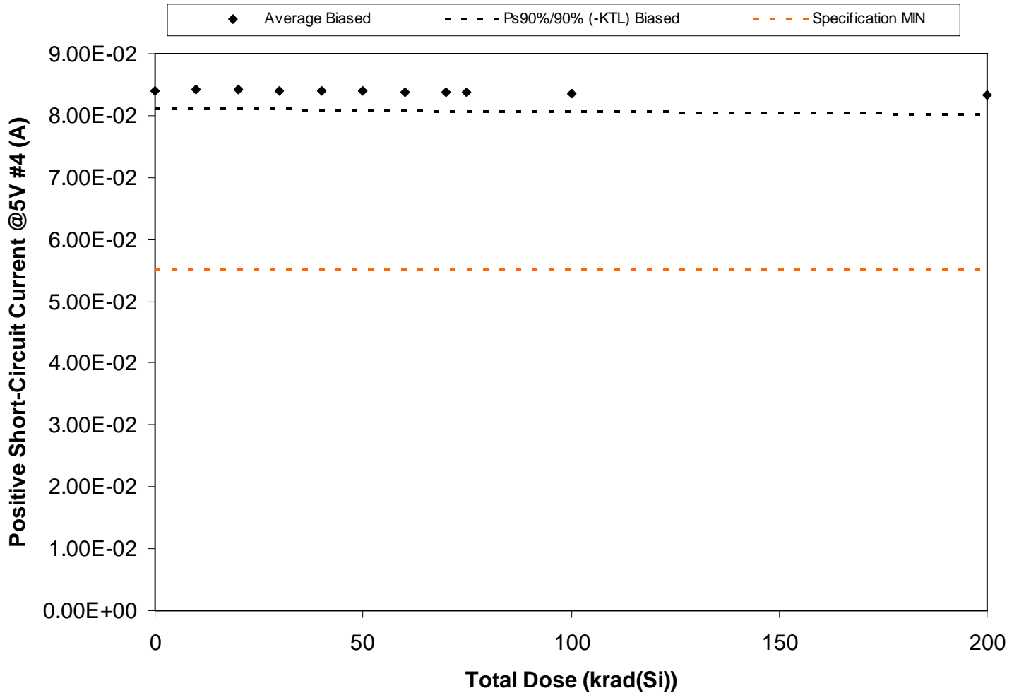
Figure 5.148. Plot of Positive Short-Circuit Current @5V #4 (A) versus total dose. The solid diamonds are the average of the measured data points for the samples irradiated under electrical bias and the black lines (solid and/or dashed) are the average of the data points after application of the KTL statistics on the samples irradiated under electrical bias. The red dotted line(s) are the pre- and/or post-irradiation minimum and/or maximum specification value as defined in the datasheet and/or test plan.
