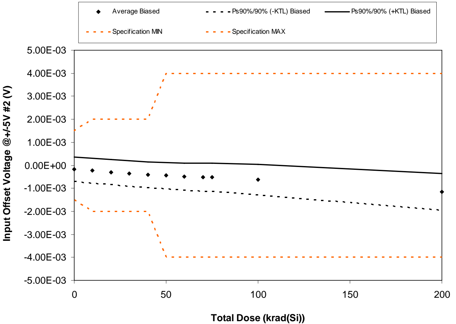
Figure 5.4. Plot of Input Offset Voltage @ +/-5V #2 (V) versus total dose. The solid diamonds are the average of the measured data points for the samples irradiated under electrical bias and the black lines (solid and/or dashed) are the average of the data points after application of the KTL statistics on the samples irradiated under electrical bias. The red dotted line(s) are the pre- and/or post-irradiation minimum and/or maximum specification value as defined in the datasheet and/or test plan.
