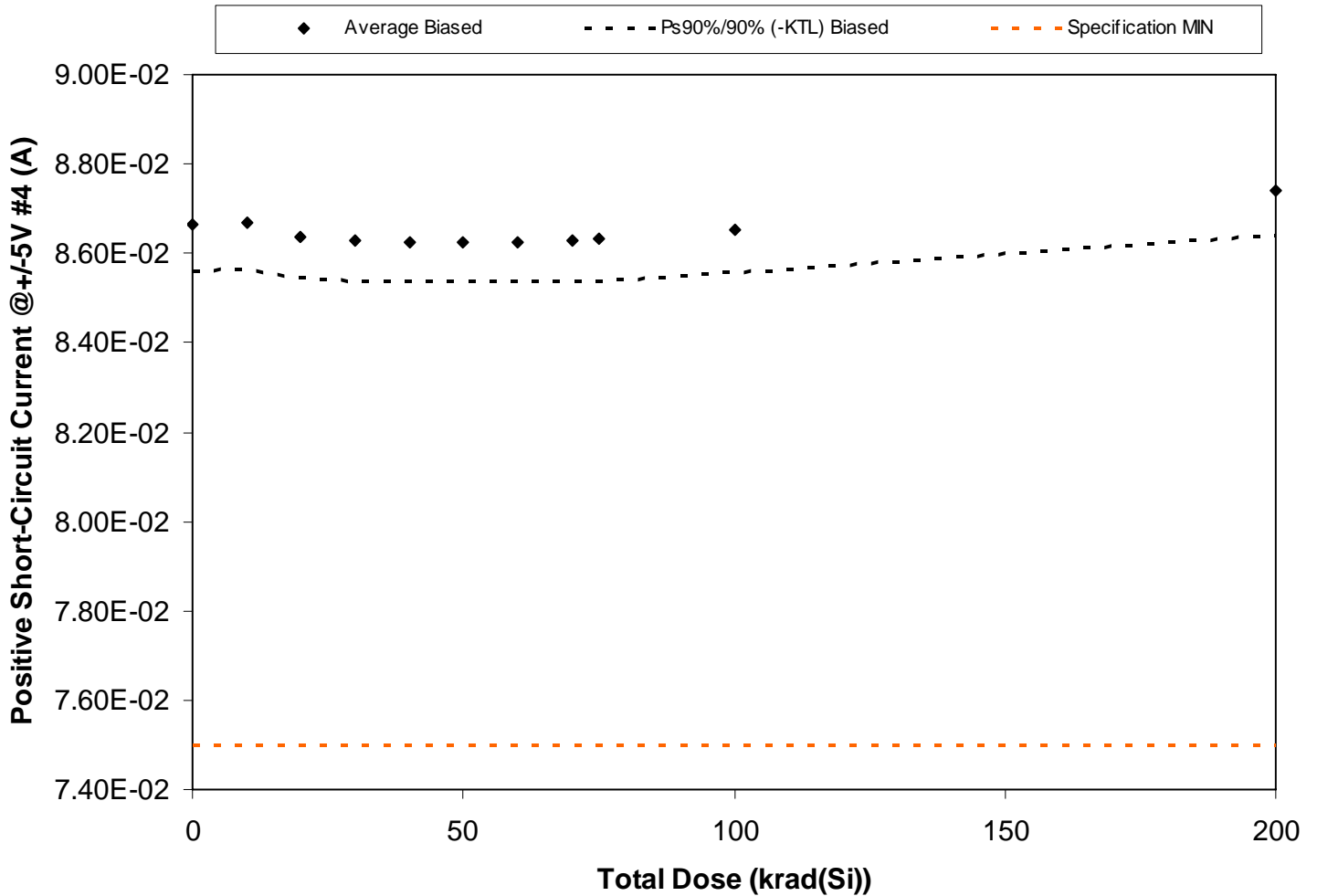
Figure 5.74. Plot of Positive Short-Circuit Current @ +/-5V #4 (A) versus total dose. The solid diamonds are the average of the measured data points for the samples irradiated under electrical bias and the black lines (solid and/or dashed) are the average of the data points after application of the KTL statistics on the samples irradiated under electrical bias. The red dotted line(s) are the pre- and/or post-irradiation minimum and/or maximum specification value as defined in the datasheet and/or test plan.
