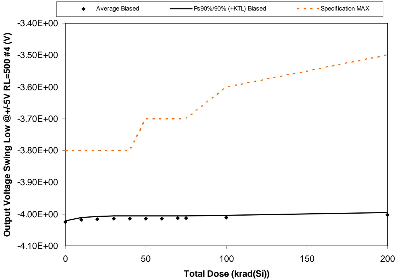
Figure 5.58. Plot of Output Voltage Swing Low @ +/-5V RL=500 #4 (V) versus total dose. The solid diamonds are the average of the measured data points for the samples irradiated under electrical bias and the black lines (solid and/or dashed) are the average of the data points after application of the KTL statistics on the samples irradiated under electrical bias. The red dotted line(s) are the pre- and/or post-irradiation minimum and/or maximum specification value as defined in the datasheet and/or test plan.
