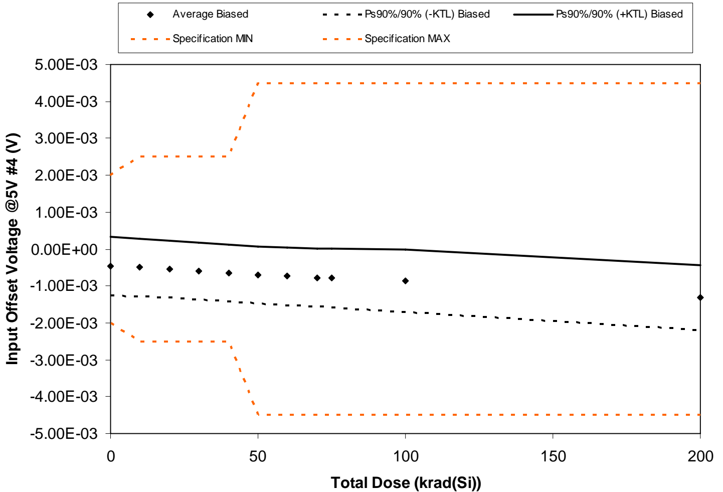
Figure 5.84. Plot of Input Offset Voltage @5V #4 (V) versus total dose. The solid diamonds are the average of the measured data points for the samples irradiated under electrical bias and the black lines (solid and/or dashed) are the average of the data points after application of the KTL statistics on the samples irradiated under electrical bias. The red dotted line(s) are the pre- and/or post-irradiation minimum and/or maximum specification value as defined in the datasheet and/or test plan.
