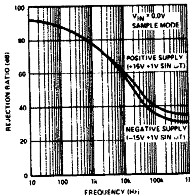
SAMPLE MODE POWER SUPPLY REJECTION
