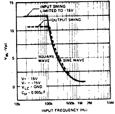
MAXIMUM INPUT SIGNAL AMPLITUDE vs FREQUENCY
