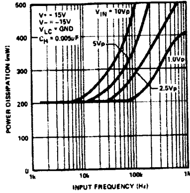
POWER DISSIPATION vs INPUT FREQUENCY = V_p \sin \omega T
