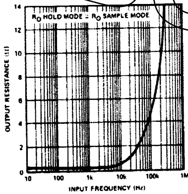
OUTPUT RESISTANCE vs FREQUENCY
