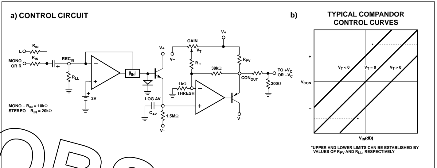
FIGURE 8: Compressor Control Circuit and Typical Curves
