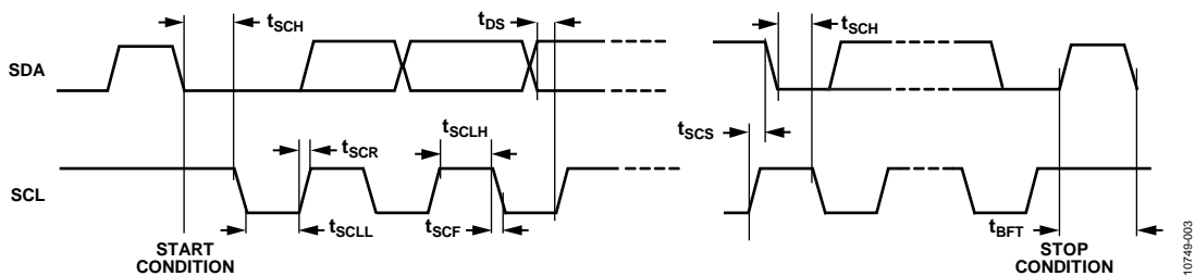
Figure 3. I 2 C Port Timing
