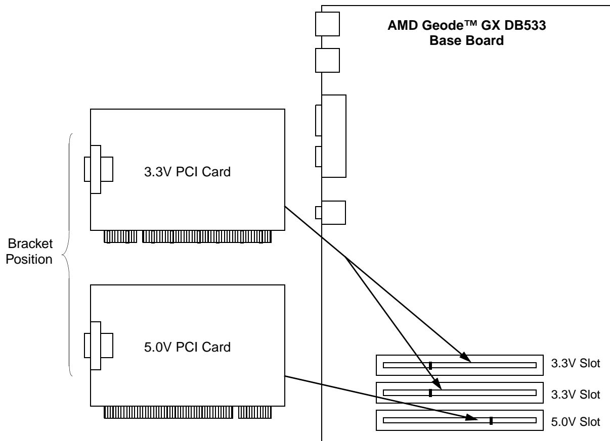
5V PCI Card Positioning
