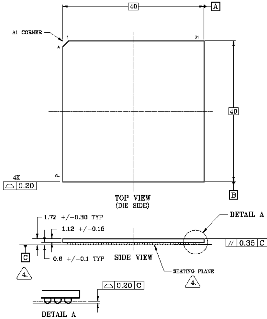
Figure 10-2. BGD432 Package - Top View
