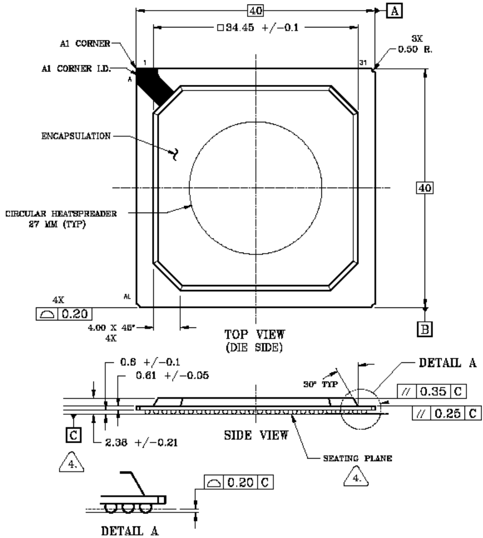
Figure 10-4. BGU481 Package - Top View
