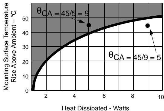
Figure 10-1. Heatsink Example
