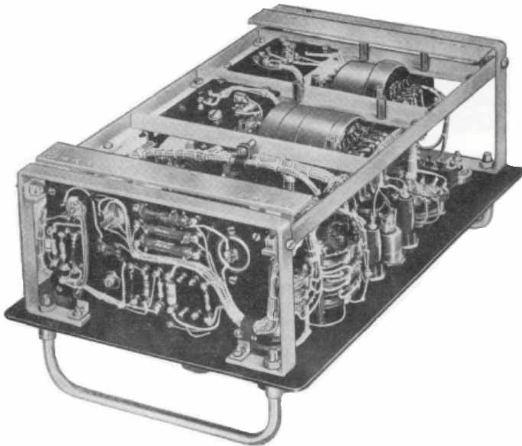
FIG. 6. INSTRUMENT CHASSIS
