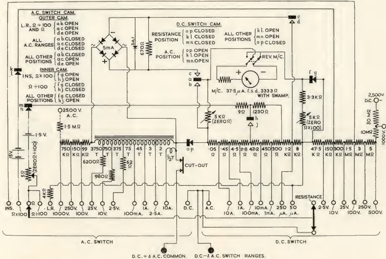
CIRCUIT DIAGRAM OF THE MODEL 8 AVOMETER
