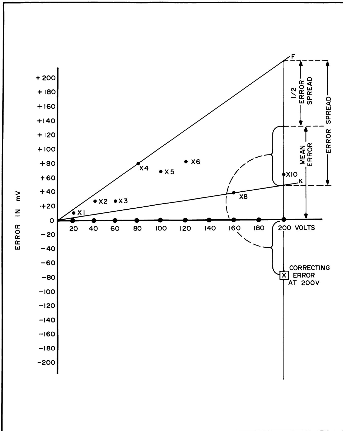
Figure 5-7. Error Correcting Graph
