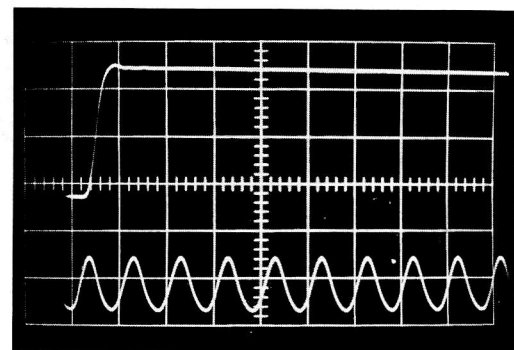
Figure 3-6. Rise Time Display
