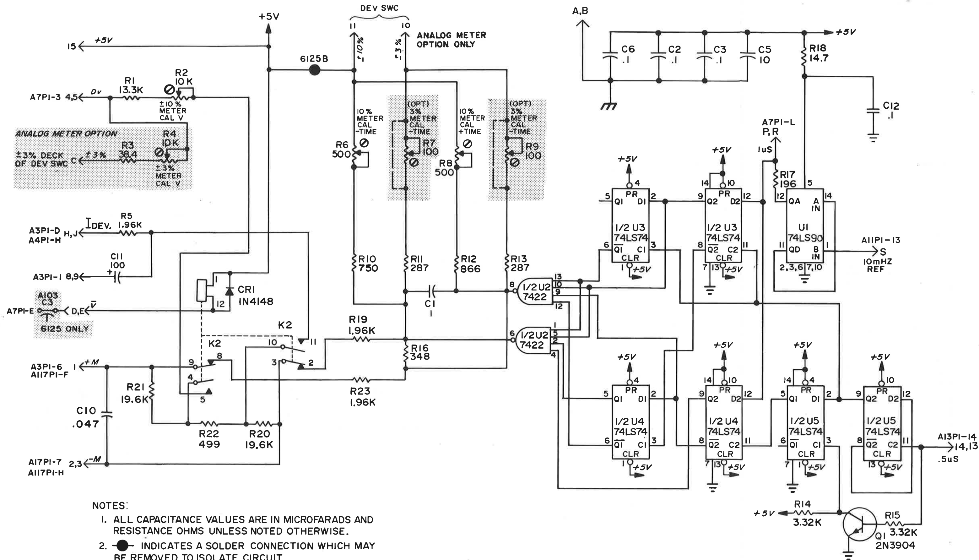
Figure 6-19A. A18 6125B/C Time Deviation Board (Serial Prefix 022-)
