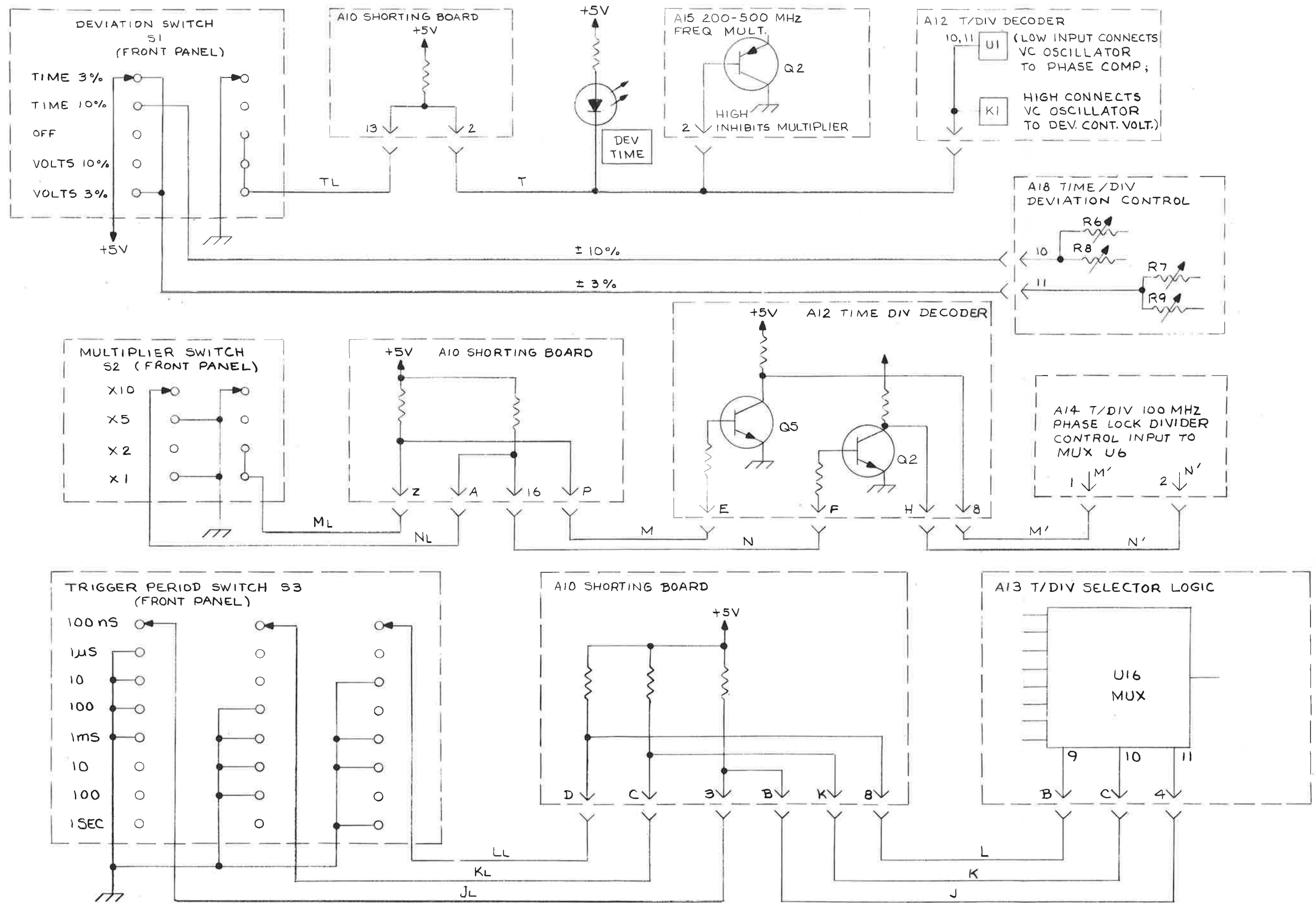
Figure 4-13. Time Deviation, Multiplier and Trigger Period Control Logic
