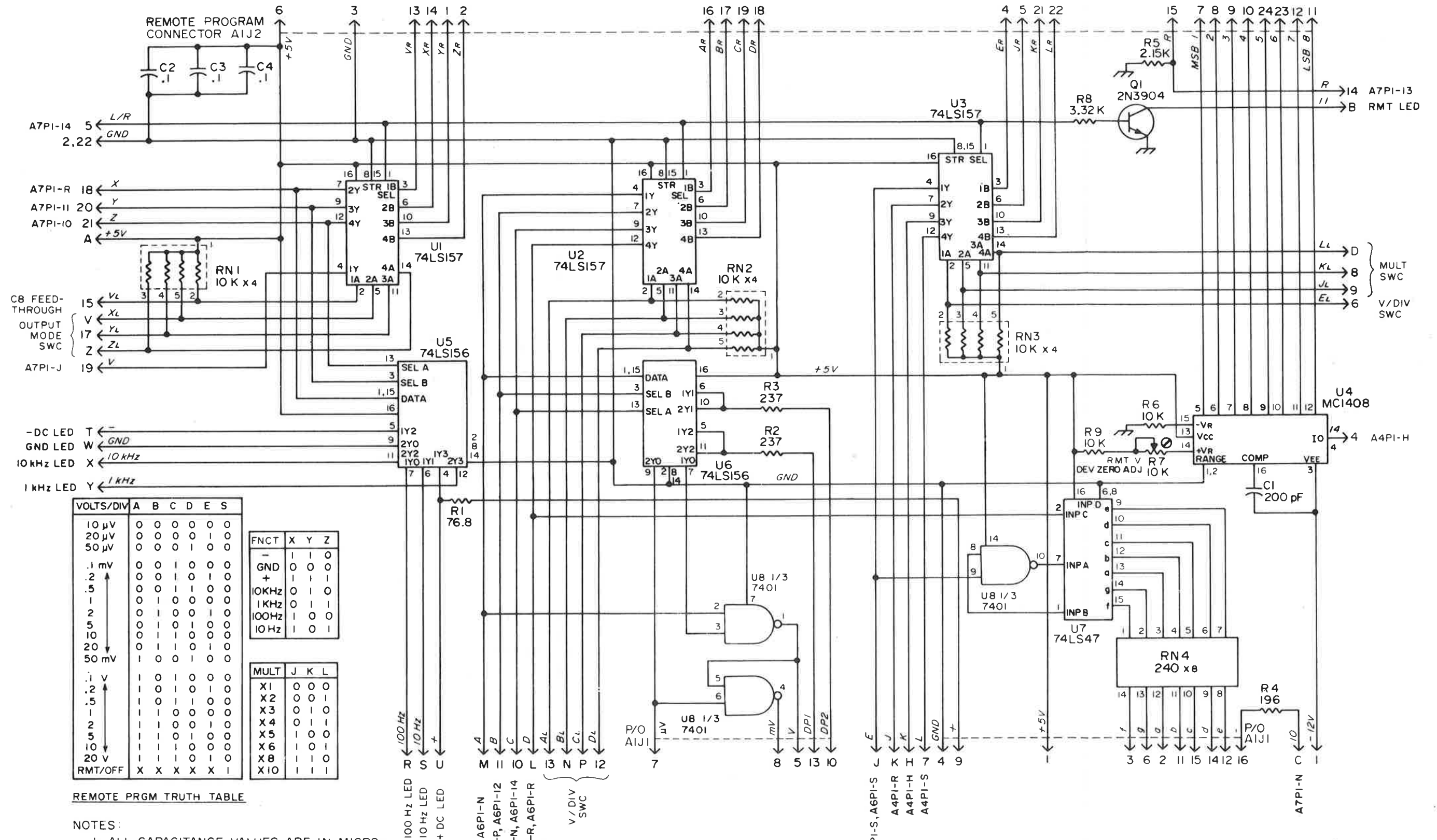
Figure 6-2. A1 6125C Volts Remote Program Input
