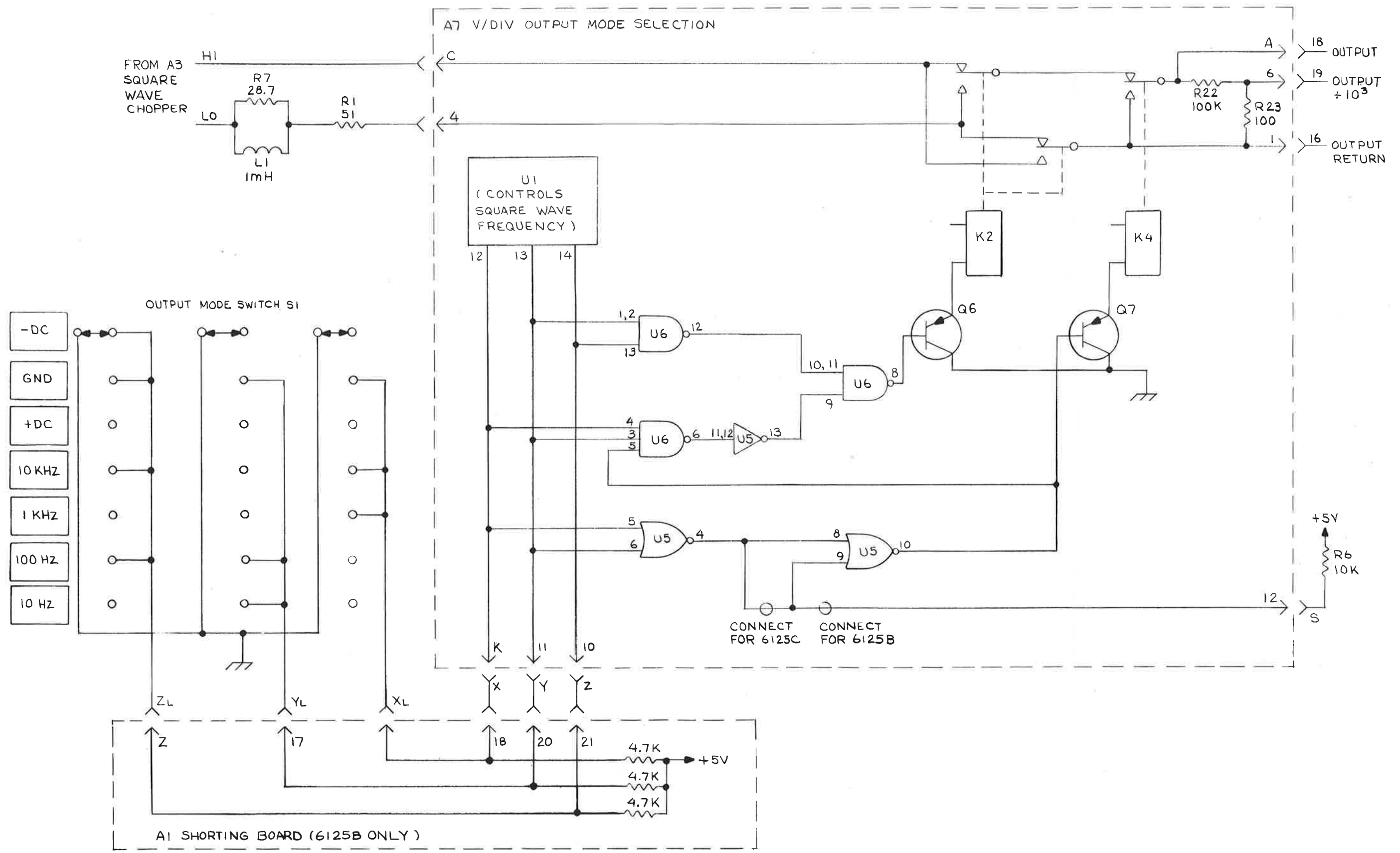
Figure 4-4. Simplified Schematic, Output Mode Selection
