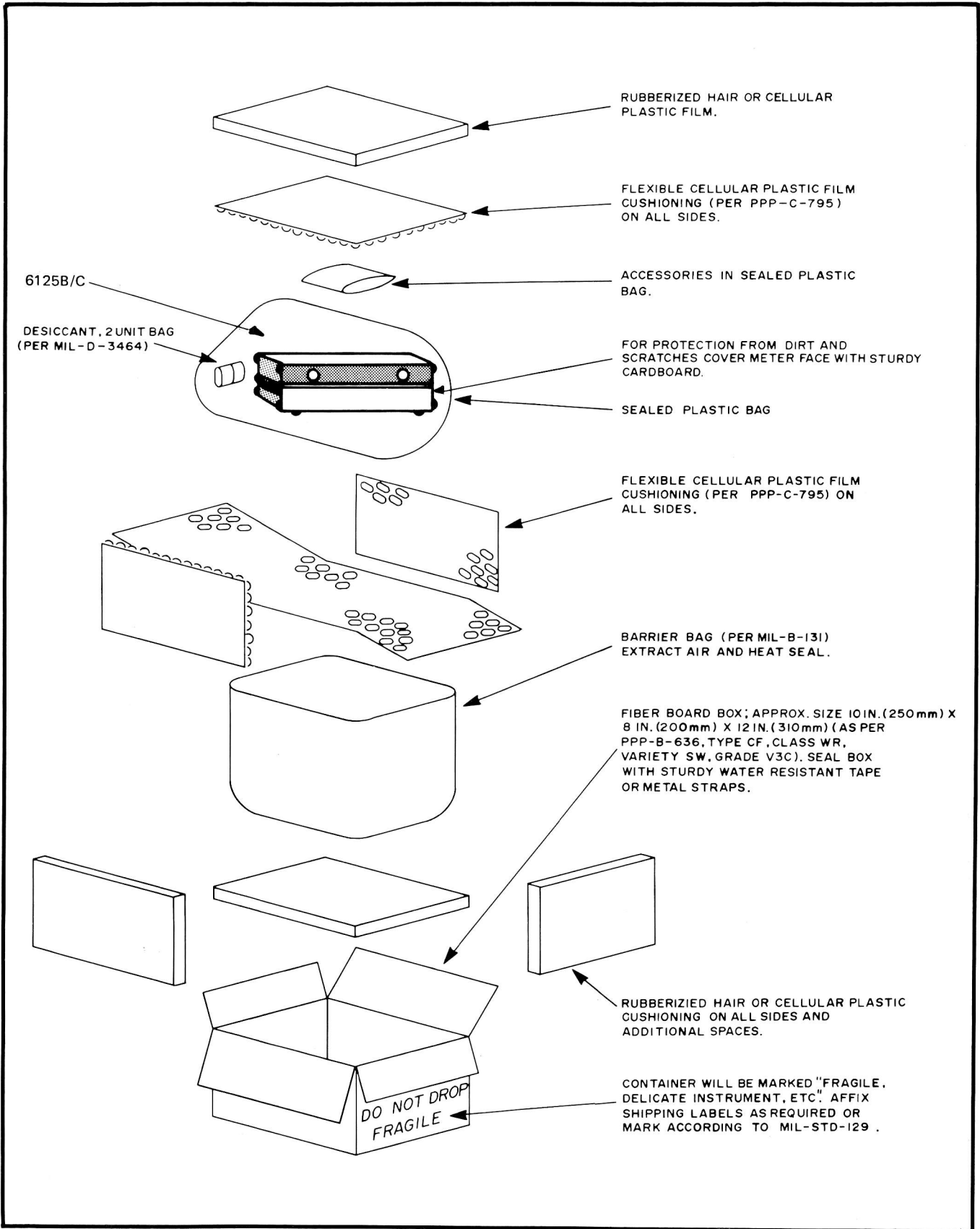
Figure 2-3. Model 6125B/C Time and Amplitude Test Set Packing Diagram.
