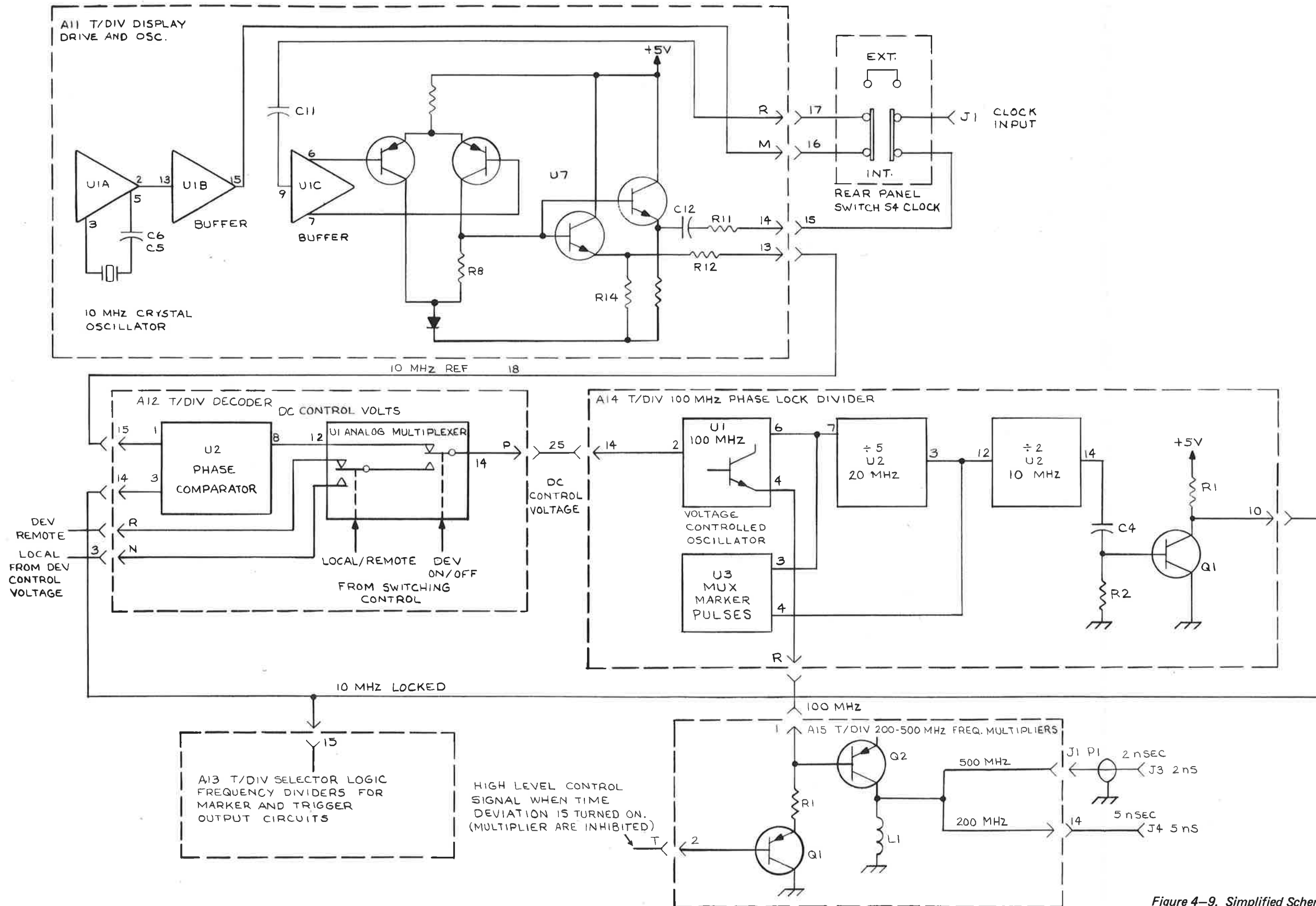
Figure 4-9. Simplified Schematic, Timing Source Circuits
