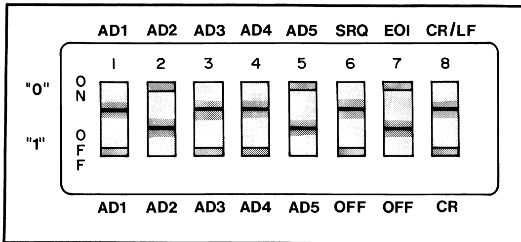
Figure 7-2. Address Switch
