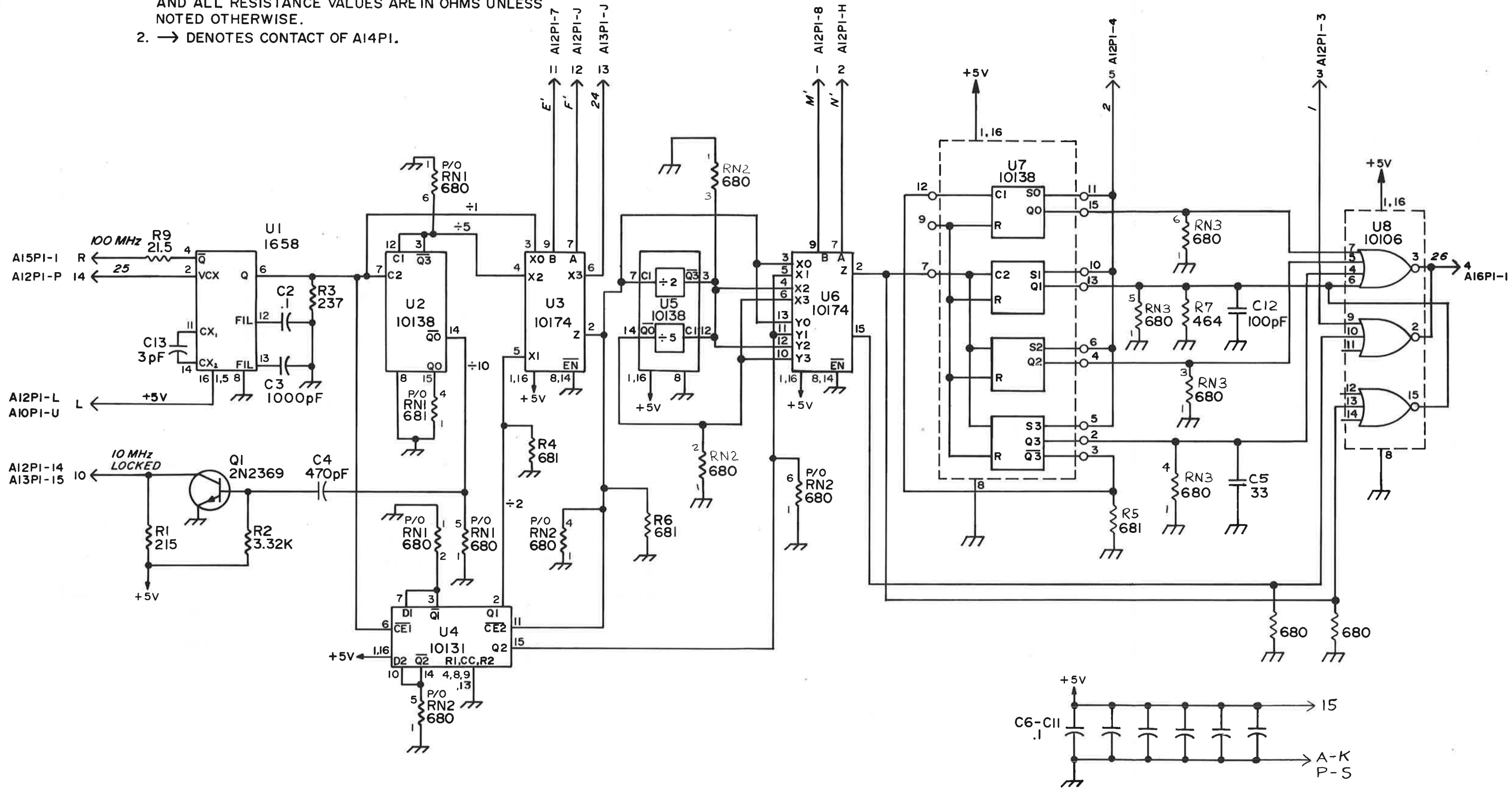
Figure 6-15. A14 6125B/C 100 MHz Phase Lock Divider
