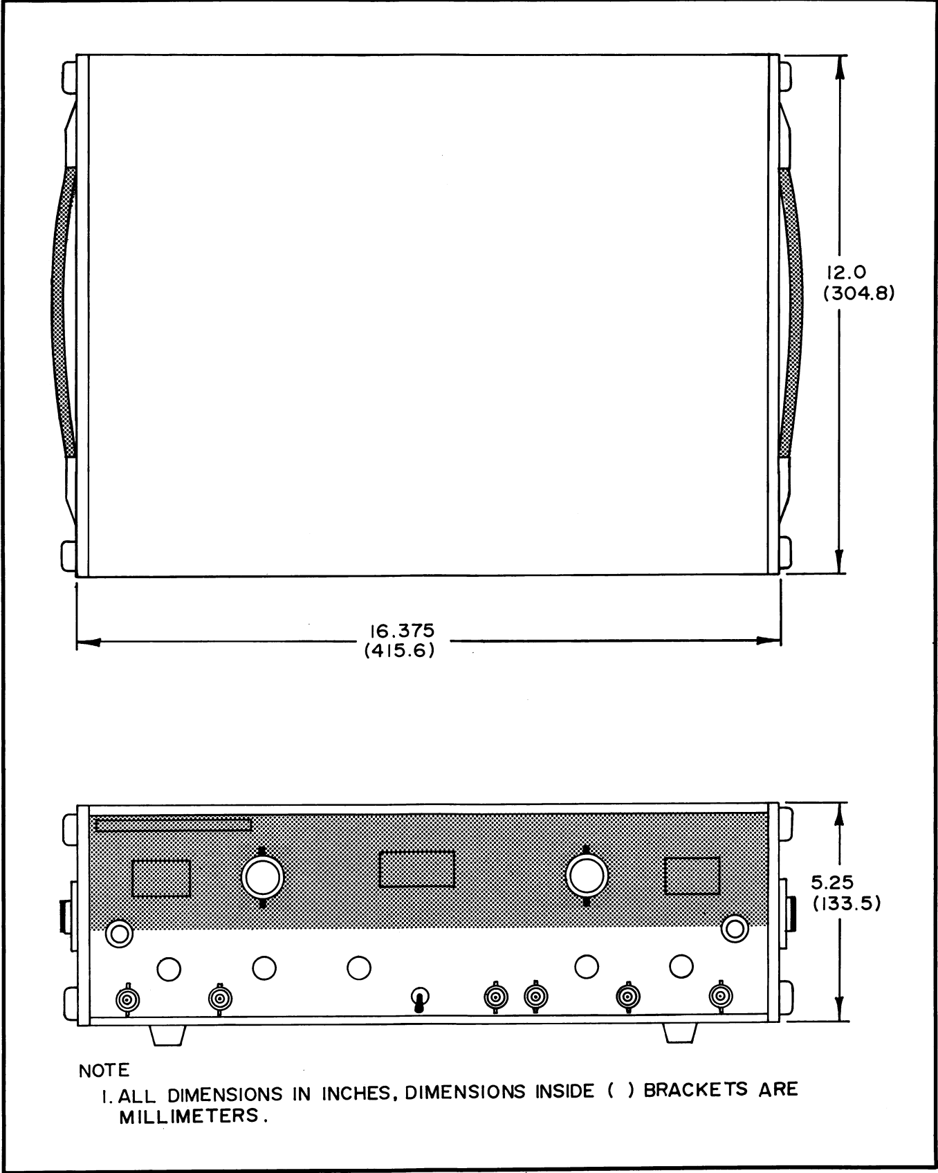
Figure 2-2. Model 6125B/C, Outline Drawing
