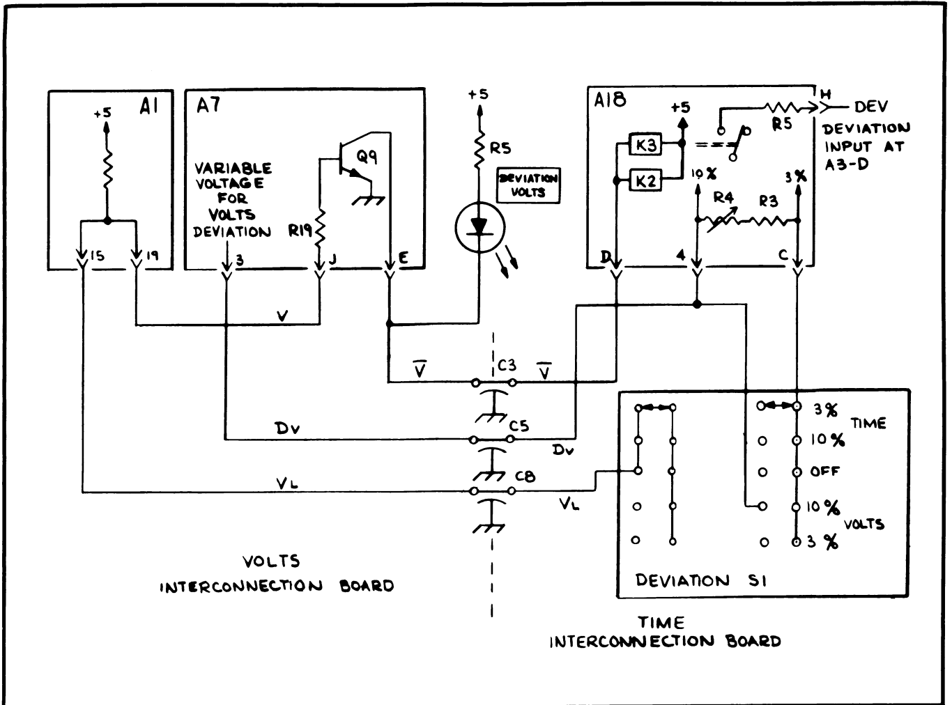
Figure 4-7B. Control Circuit, Volts Deviation
