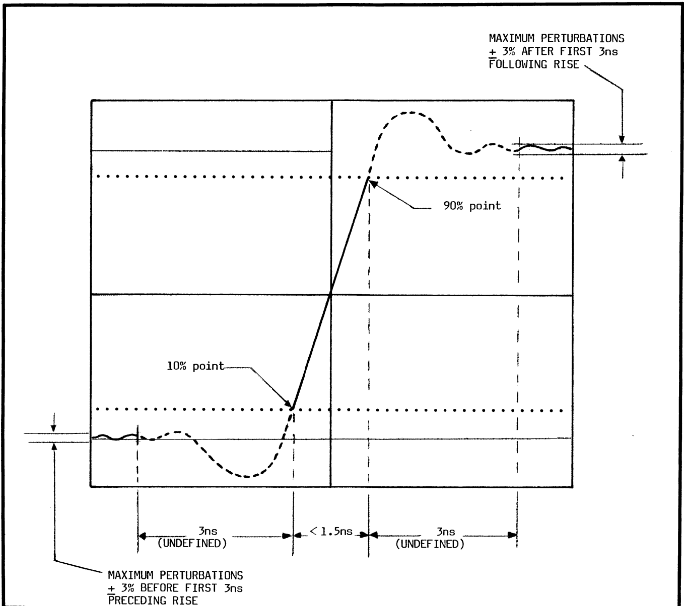
Figure 1-2. Determining Risetime
