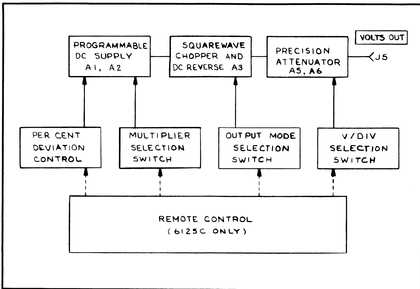
Figure 4-1. Functional Block Diagram, Volts Circuits.
