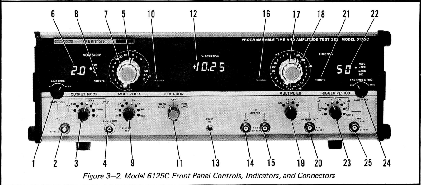
Figure 3-1. Model 6125B, Controls, Indicators, and Connectors
