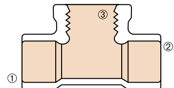
C x C x F Tee
