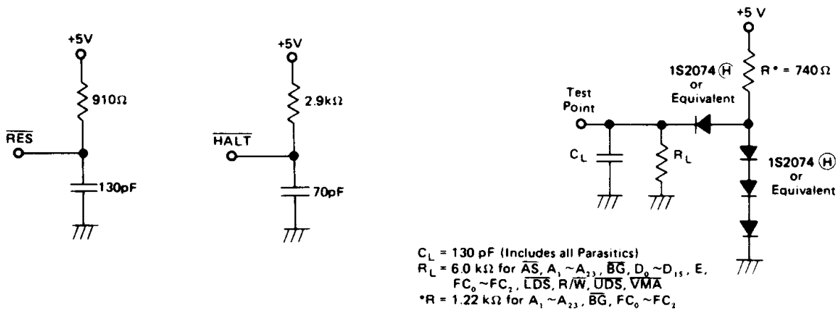
Figure 1 Test Loads
