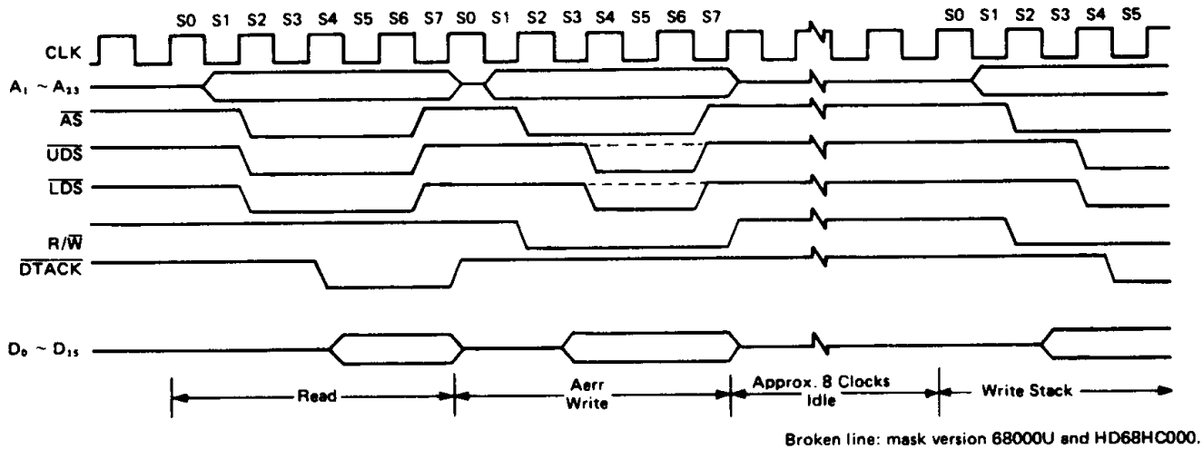
Figure 59 Address Error Timing
