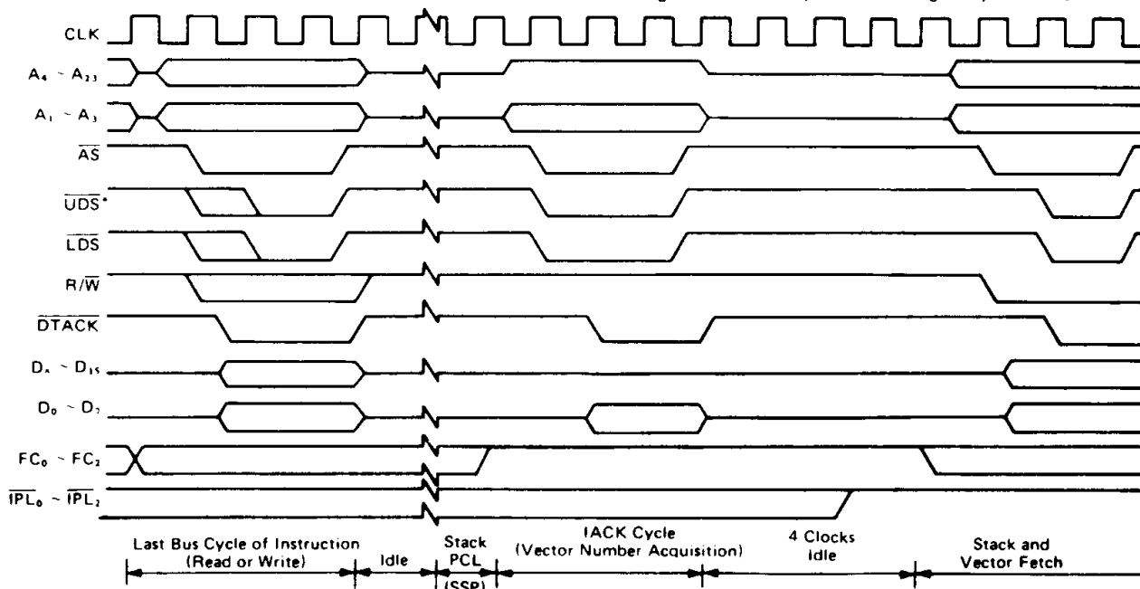
Figure 42 Interrupt Acknowledge Sequence Flow Chart
