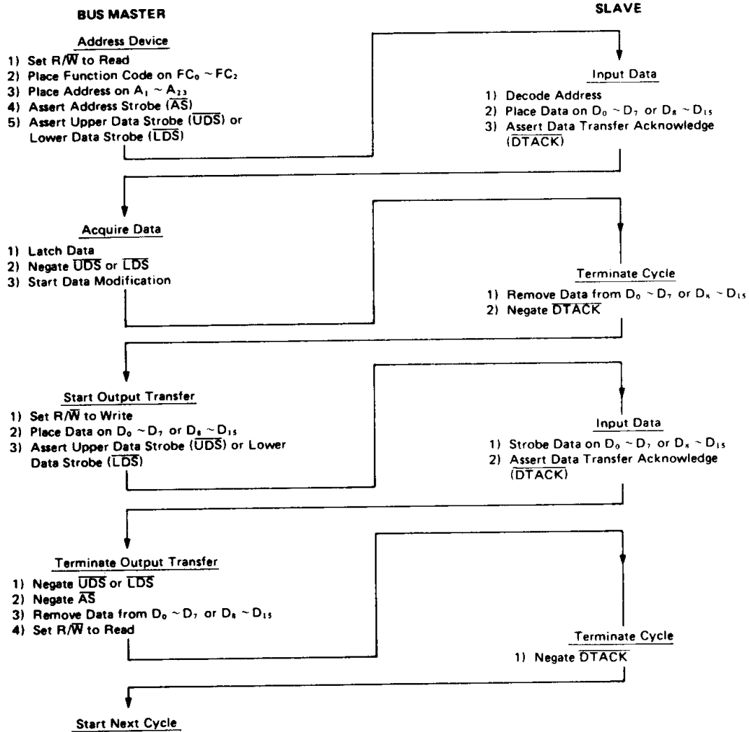
Figure 22 Read-Modify-Write Cycle Flow Chart
