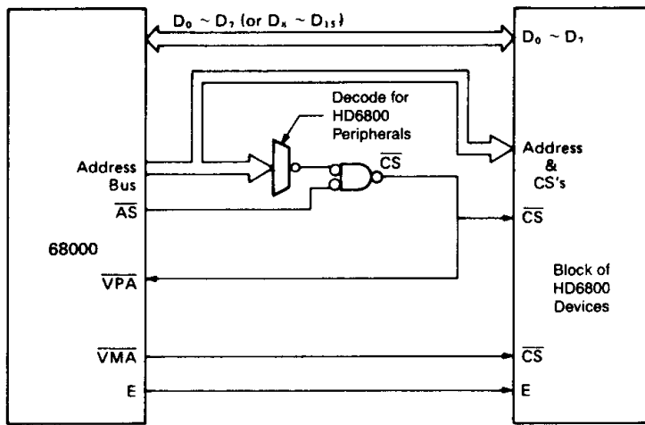
Figure 47 Connection of HD6800 Peripherals
