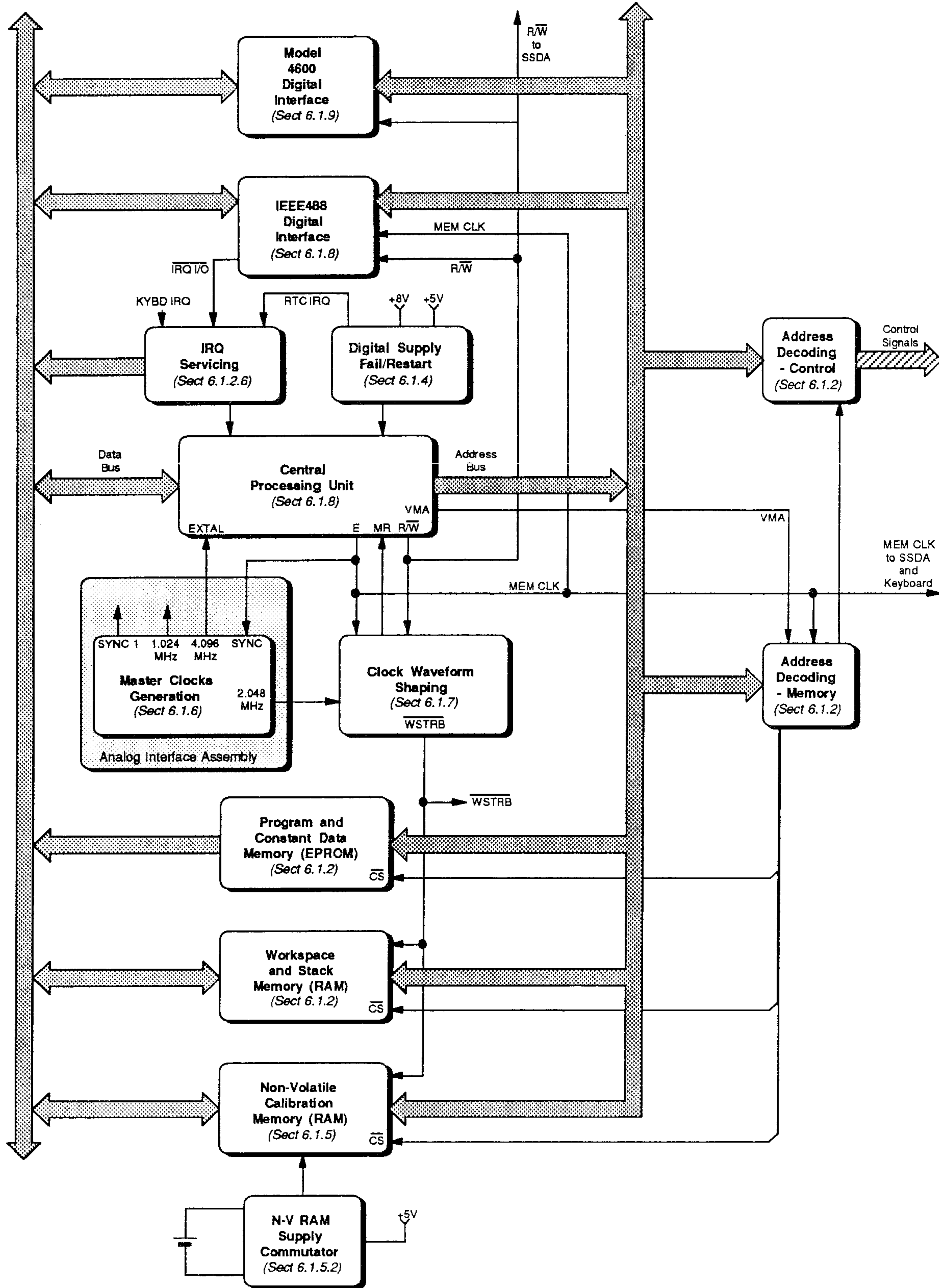
FIG. 6.1 DIGITAL FUNCTION BLOCK DIAGRAM
