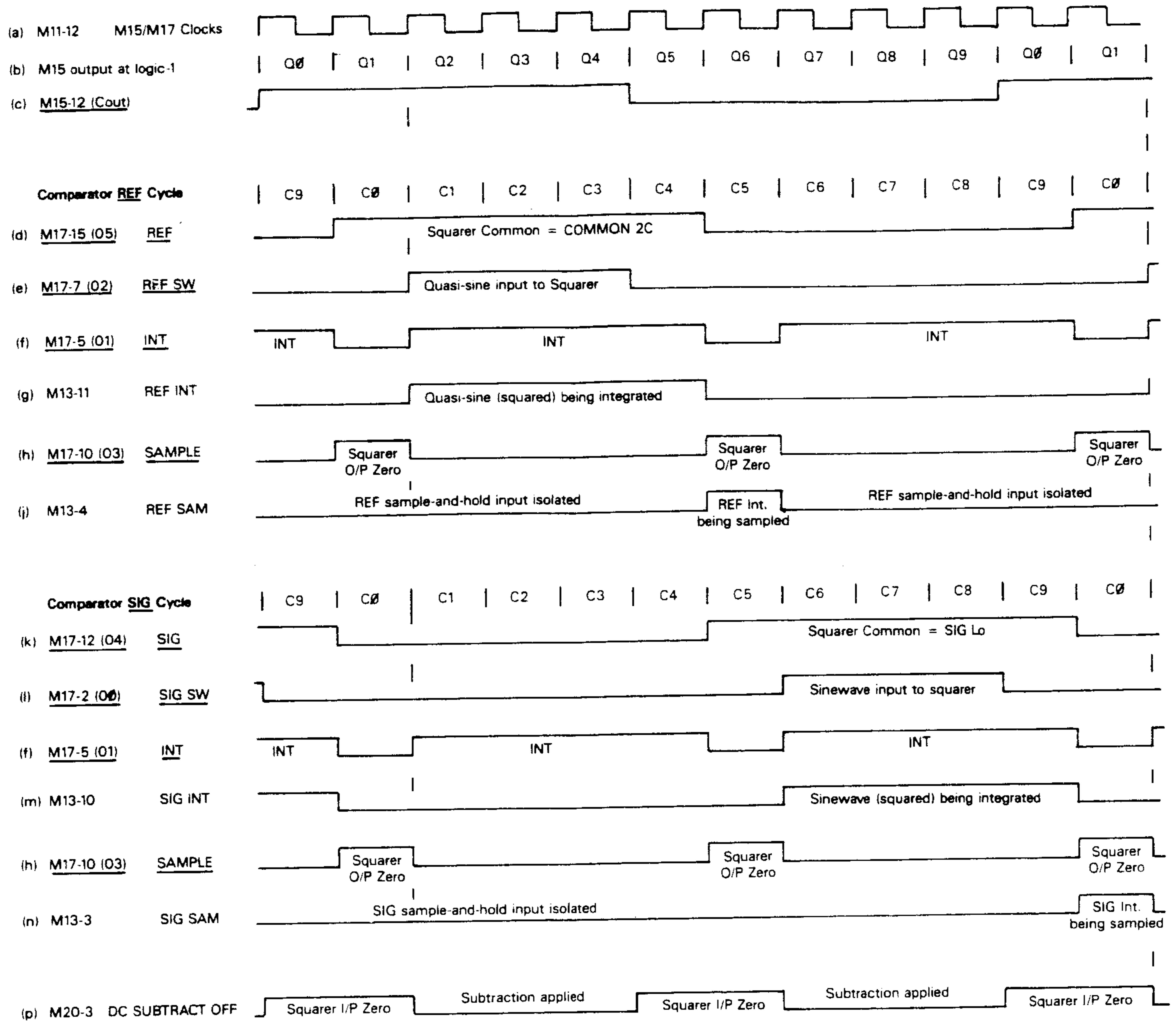
FIG. 9.13 COMPARATOR TIMING LOGIC
