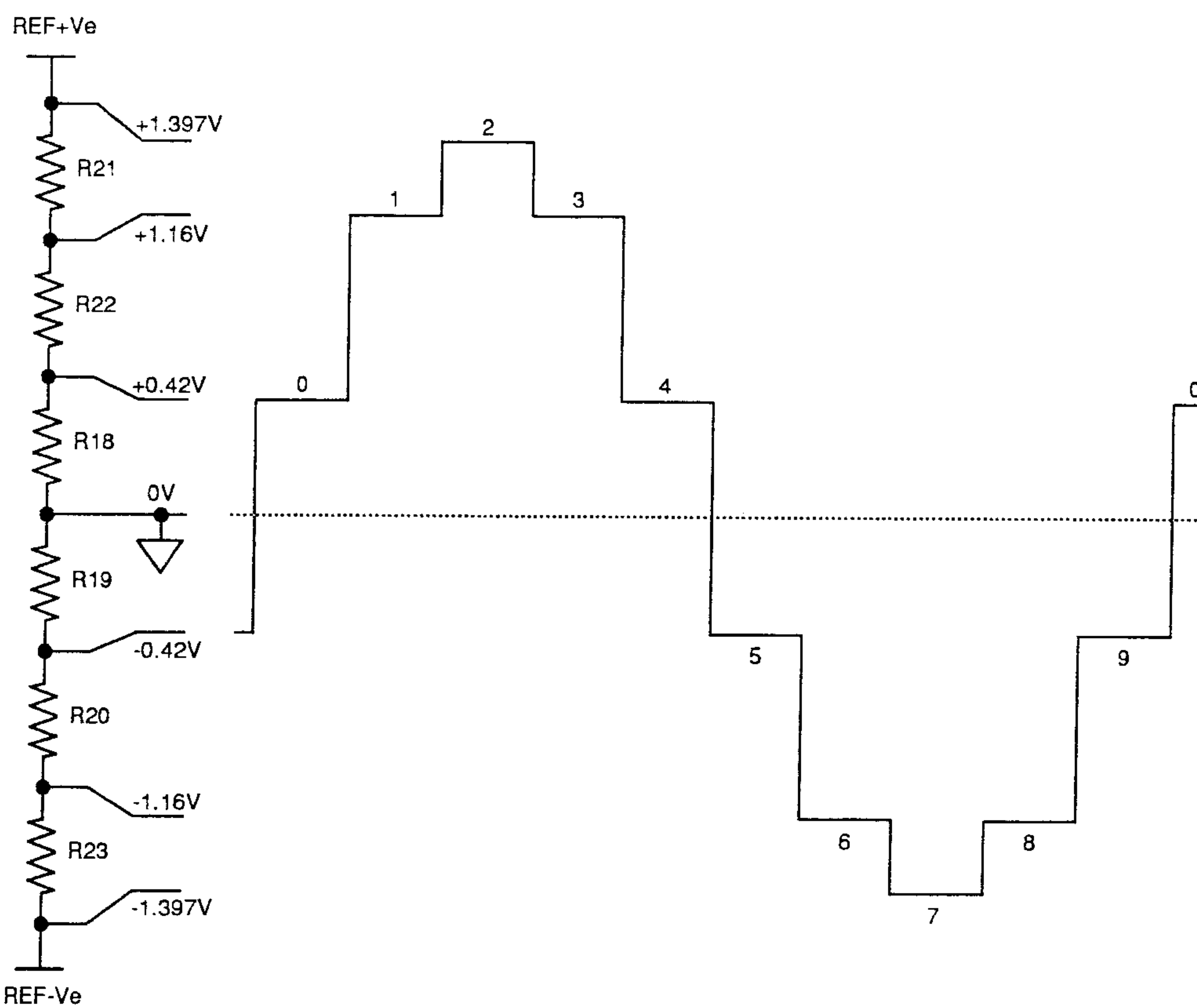
FIG. 6.28 QUASI-SINEWAVE GENERATION
