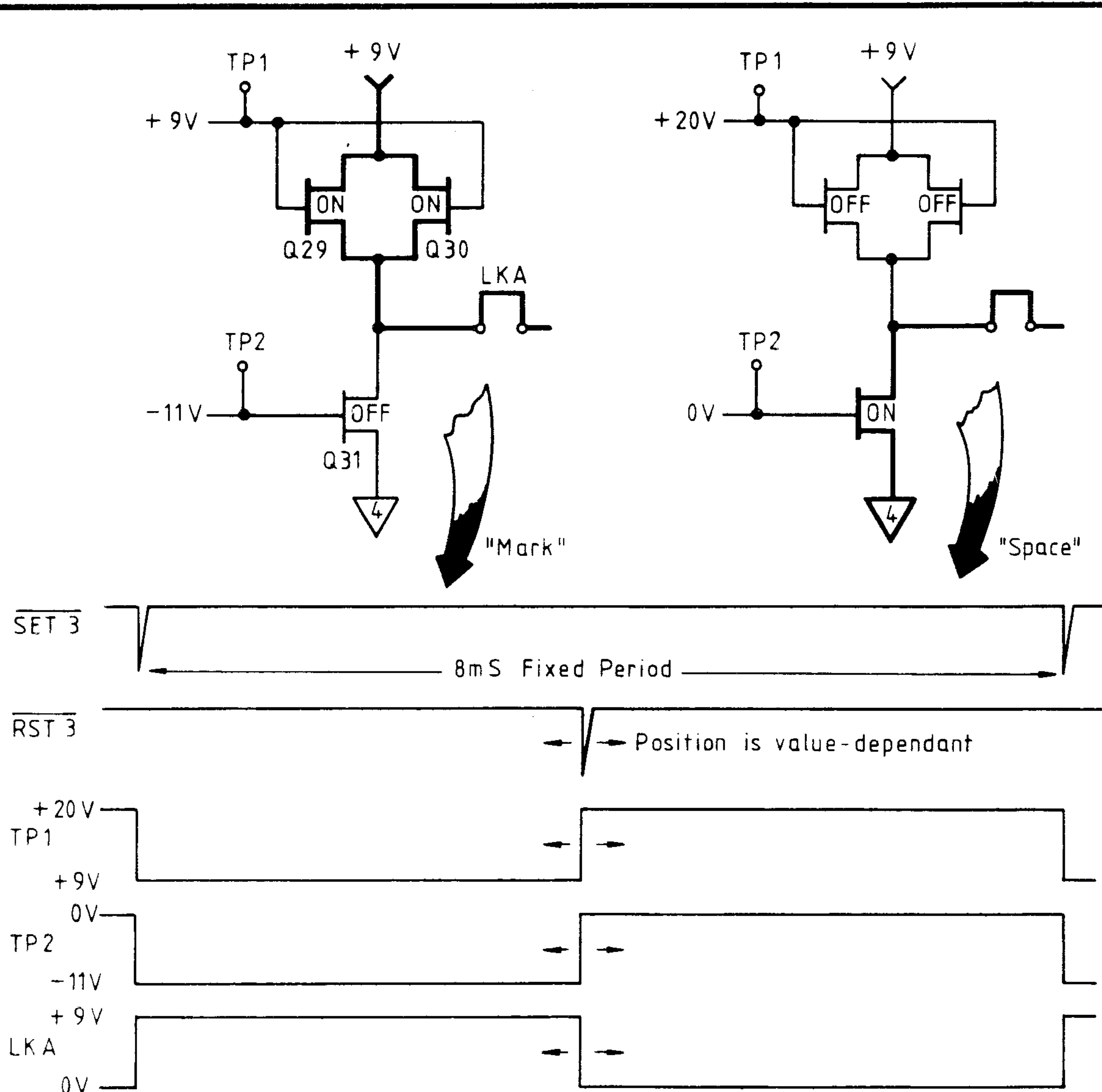
FIG. 6.26 ACTION OF LSD SWITCH
