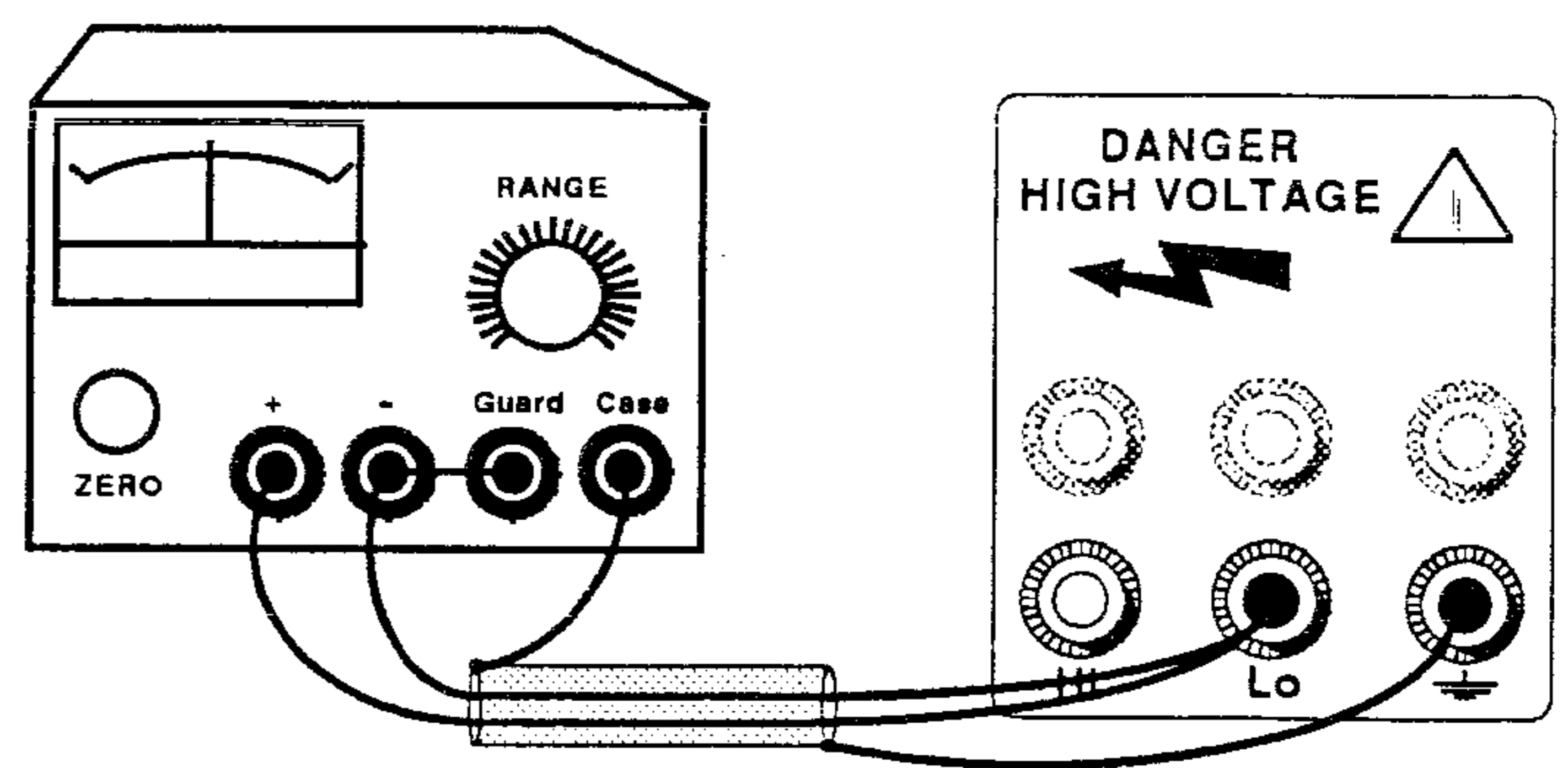
NULL DETECTOR SELF-ZERO
