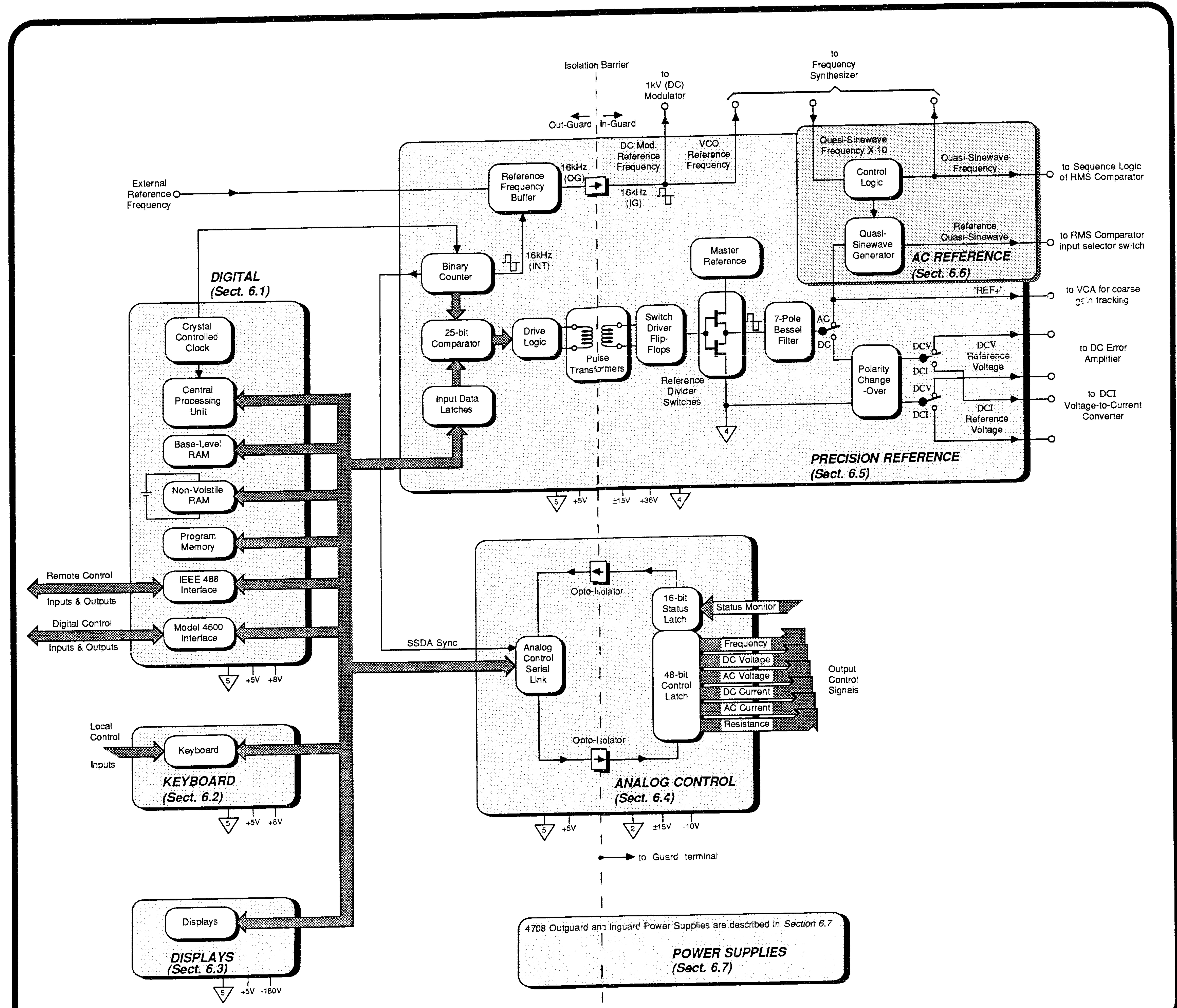
FIG. 5.2 4708 BLOCK DIAGRAM - DIGITAL, CONTROL AND REFERENCES
