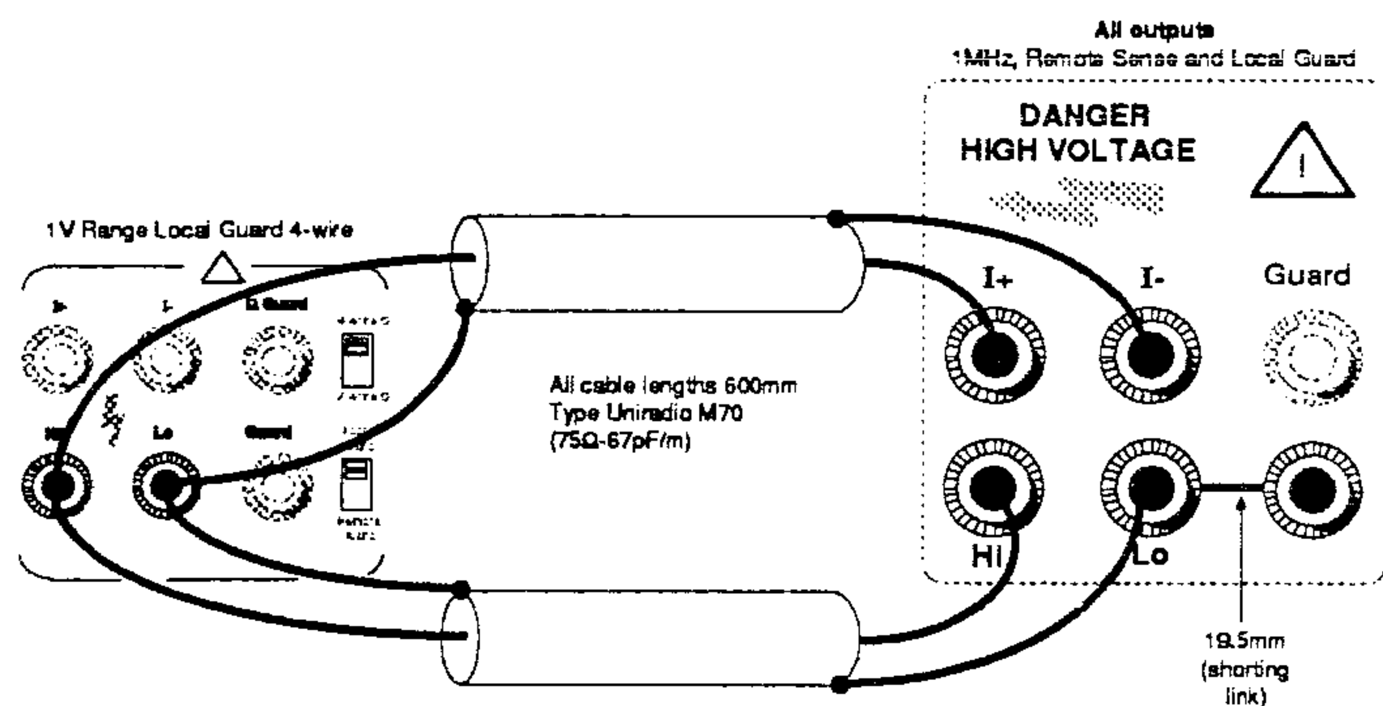
Fig. 1 AC DVM Standardization
