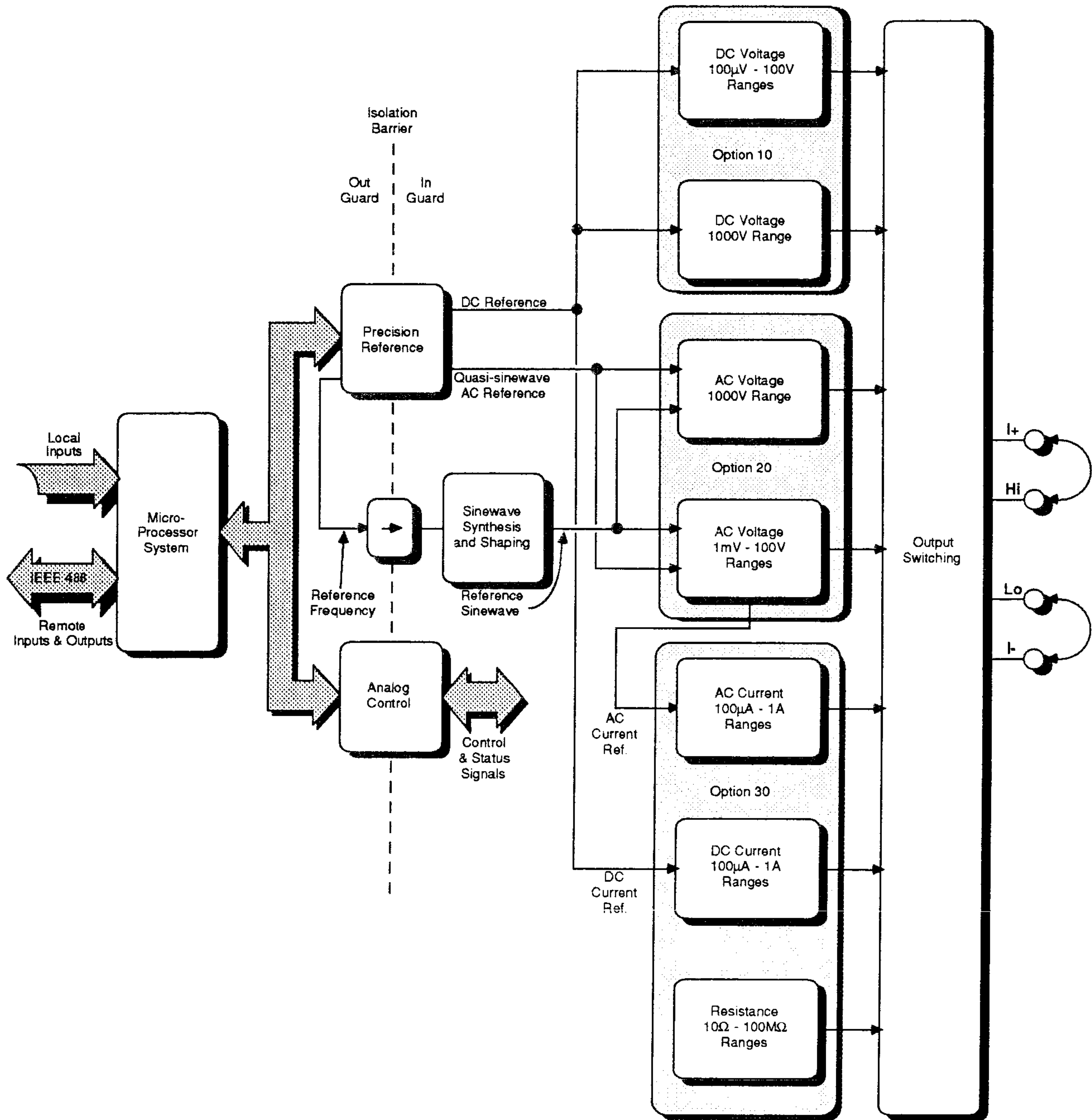
FIG. 5.1 4708 SIMPLIFIED BLOCK DIAGRAM
