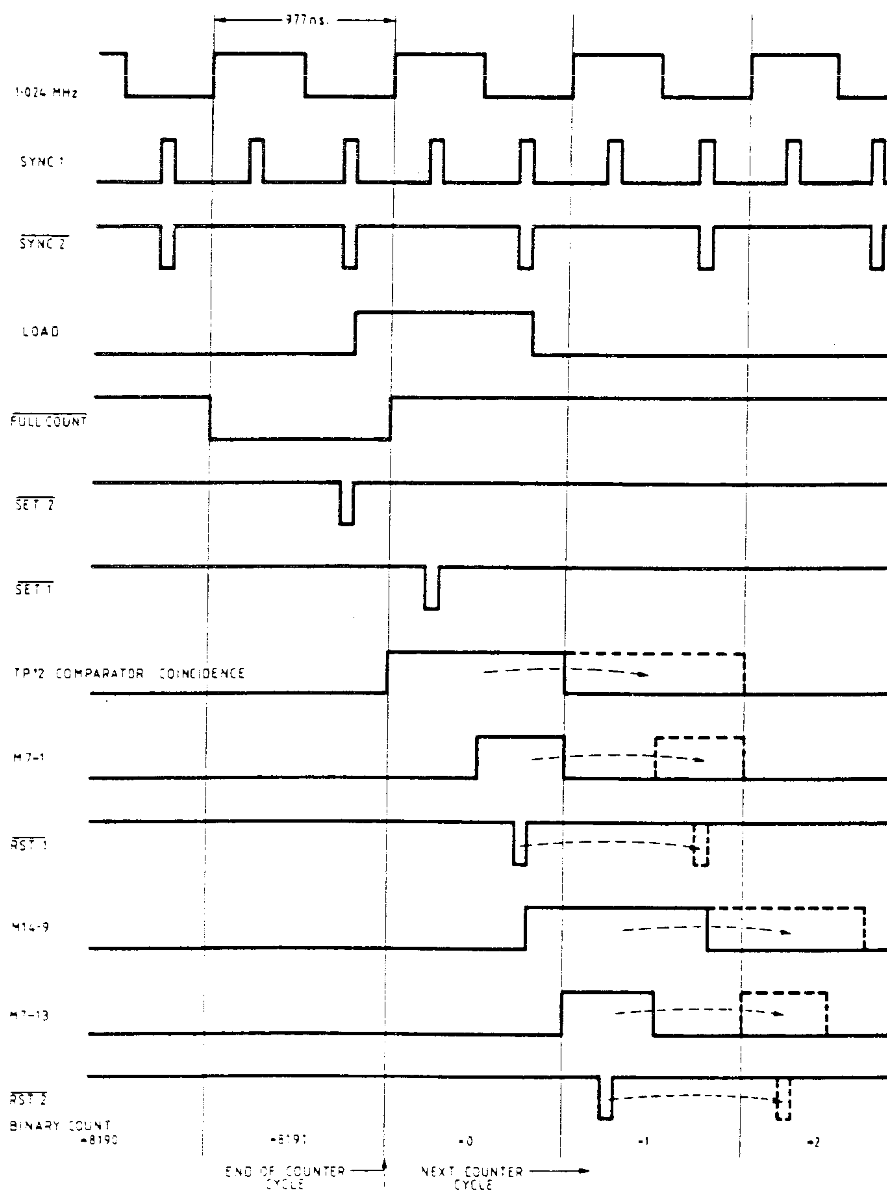
FIG. 6.23 MSB SET/RESET PULSE GENERATION
