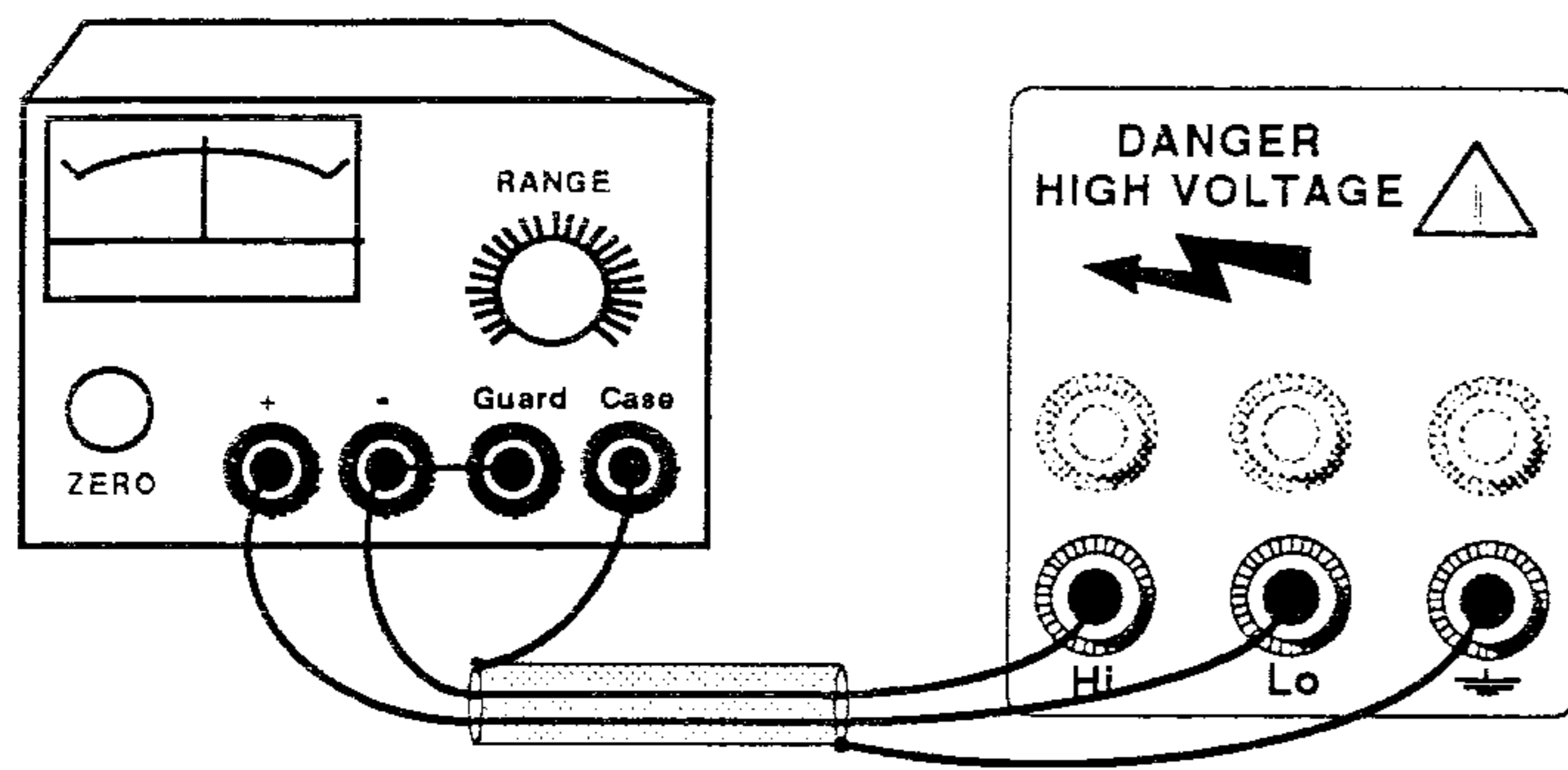
4708 ON+ & ON- ALIGNMENT
