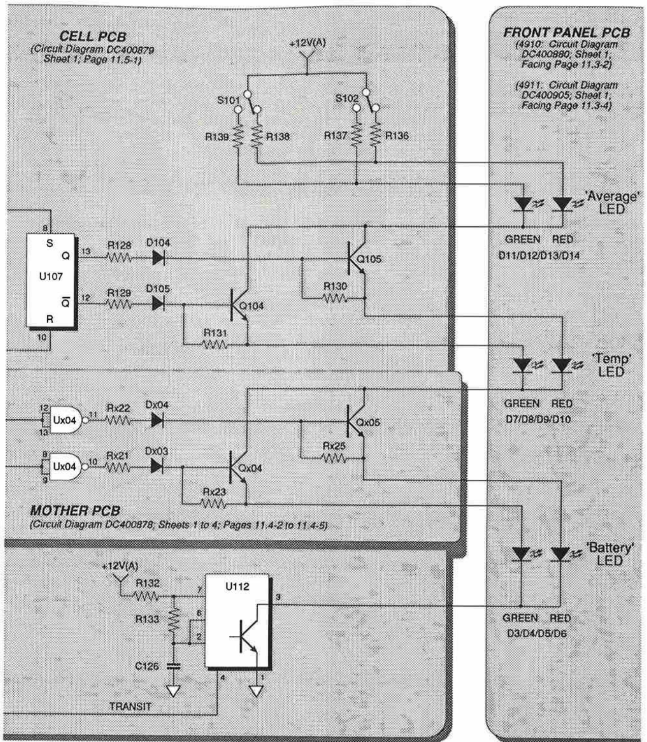
FIG. 4.2.9.1 FRONT PANEL LED SWITCHING
