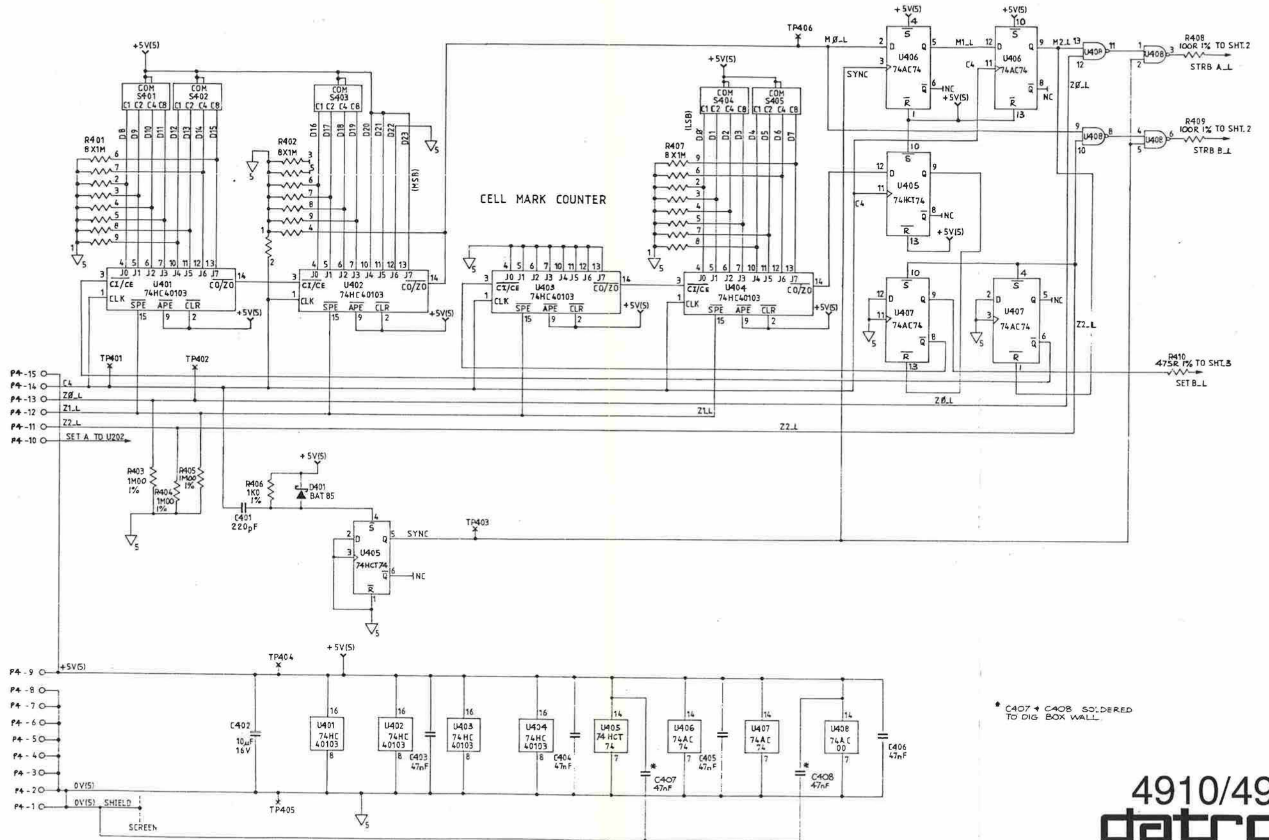
CELL PCB ASSEMBLY Drawing No. DC400879 Sheet 4
