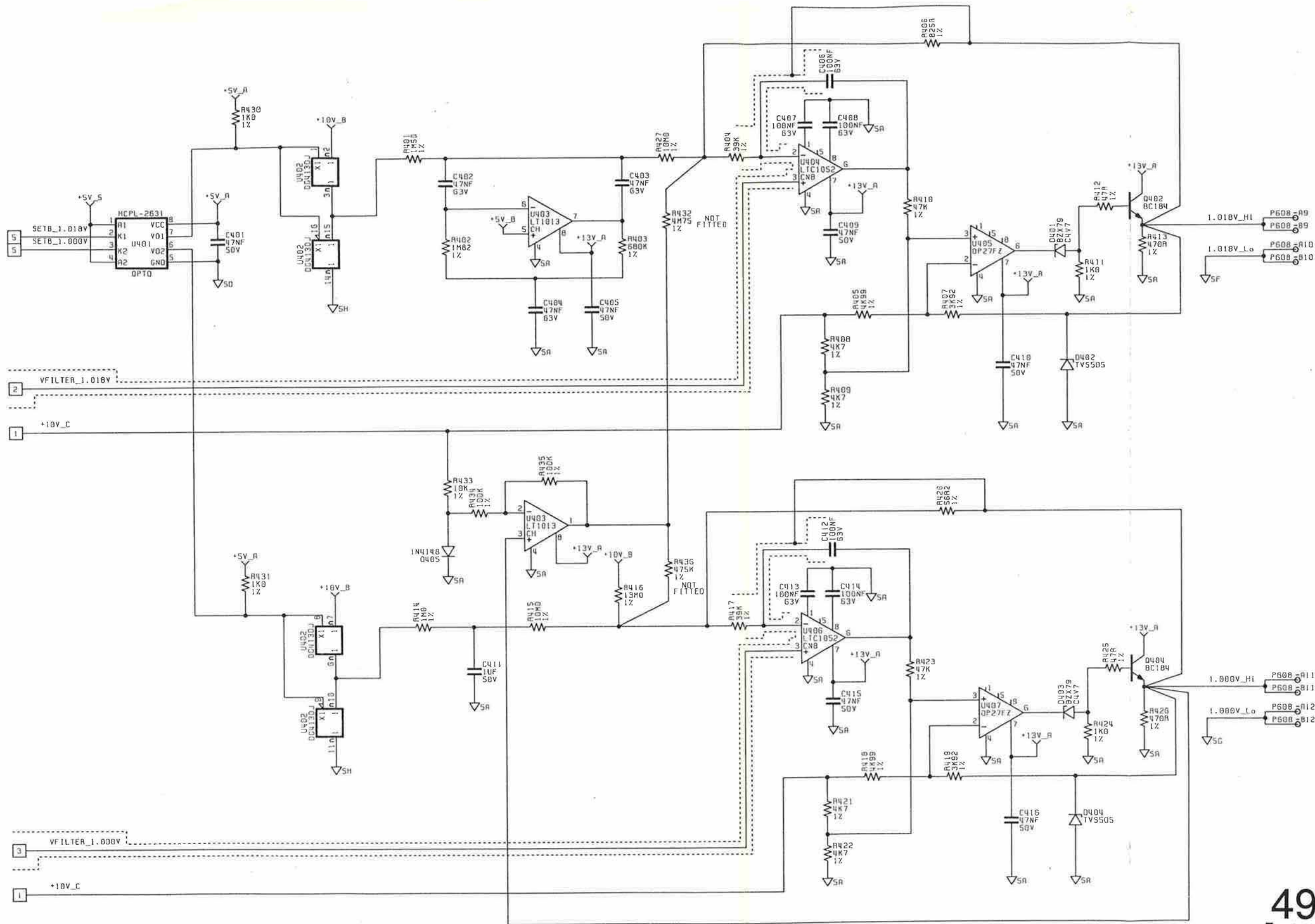
OUTPUT PCB ASSEMBLY Drawing No. DC400881 Sheet 4
