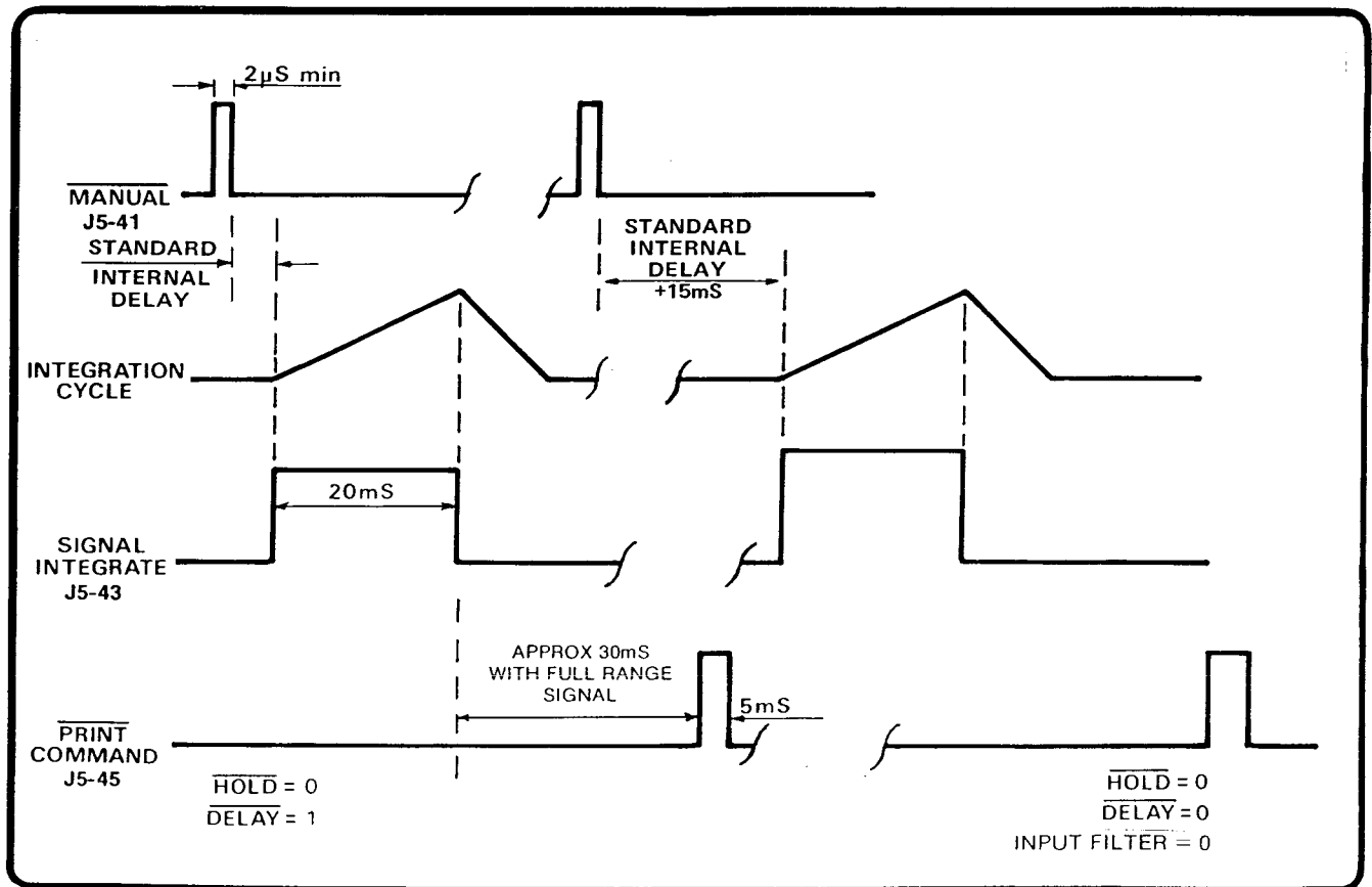
Fig. 5.1 Normal operation timing
