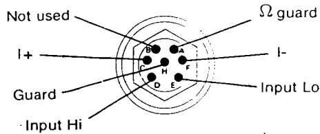
Fig. 2.2 Rear input 7 pin plug
