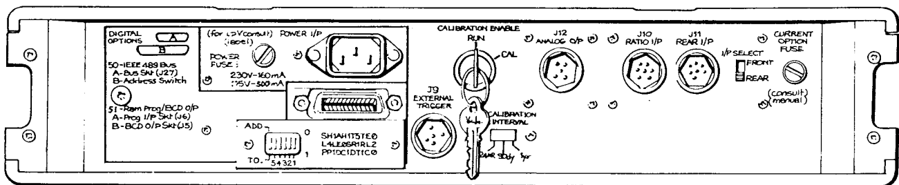
Fig 2.2 Rear panel
