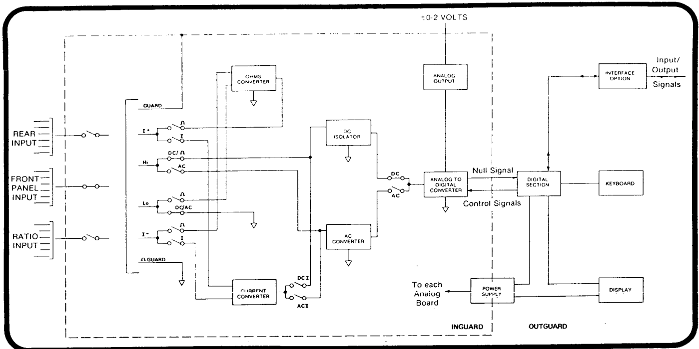
Fig 1.1 DVM simplified block diagram
