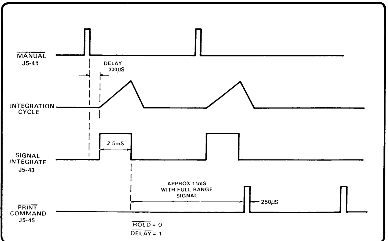
Fig. 5.3 Superfast timing (>100/sec)
