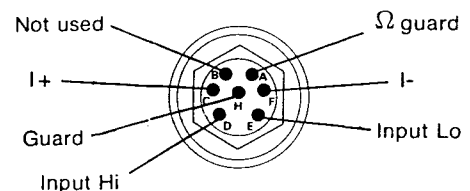
Fig 3.2 Rear and ratio inputs 7-pin plugs
