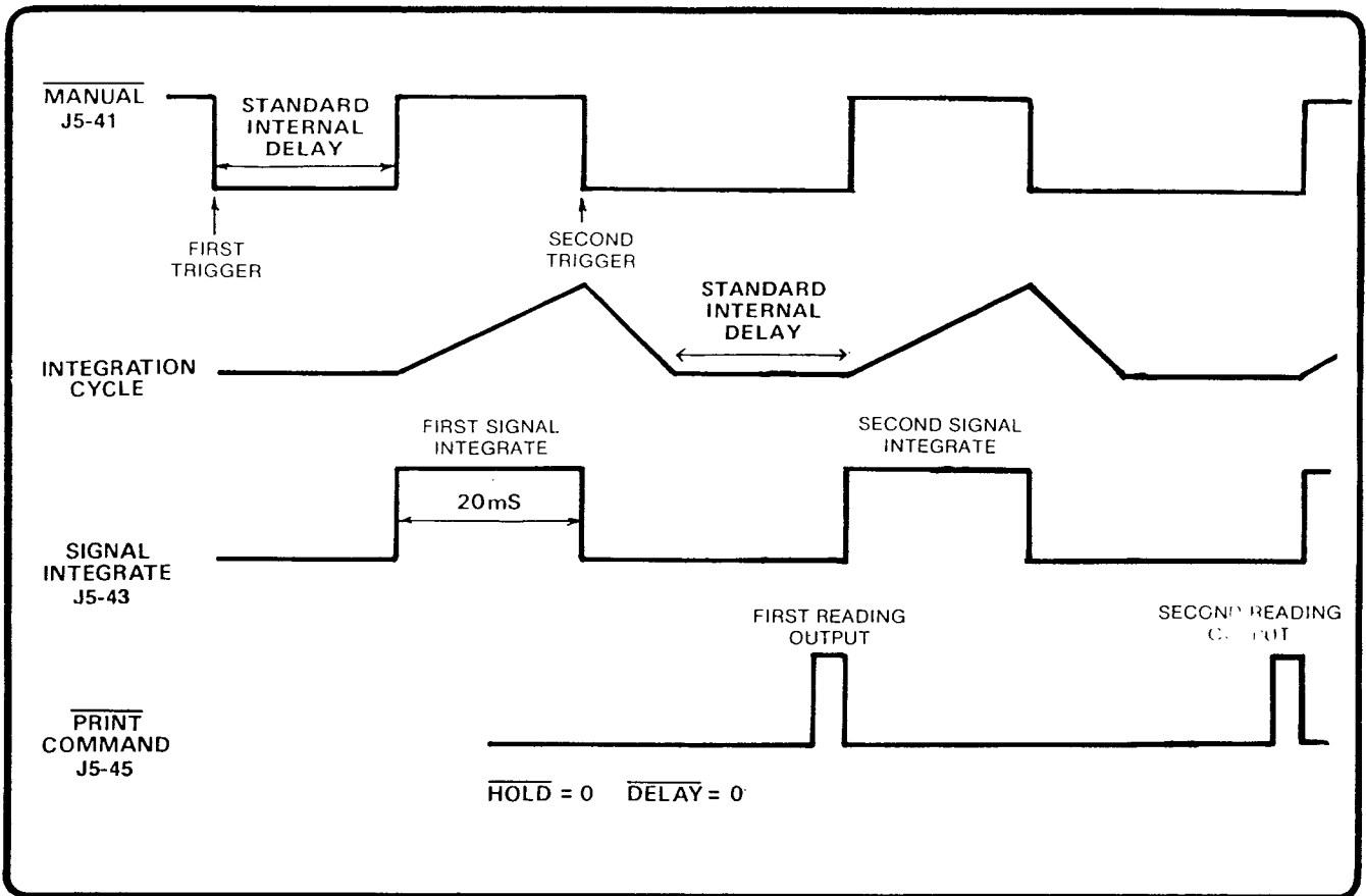
Fig. 5.2 Closed loop operation timing
