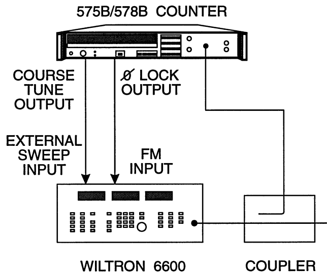
Figure 3-7. Source Locking Setup.
