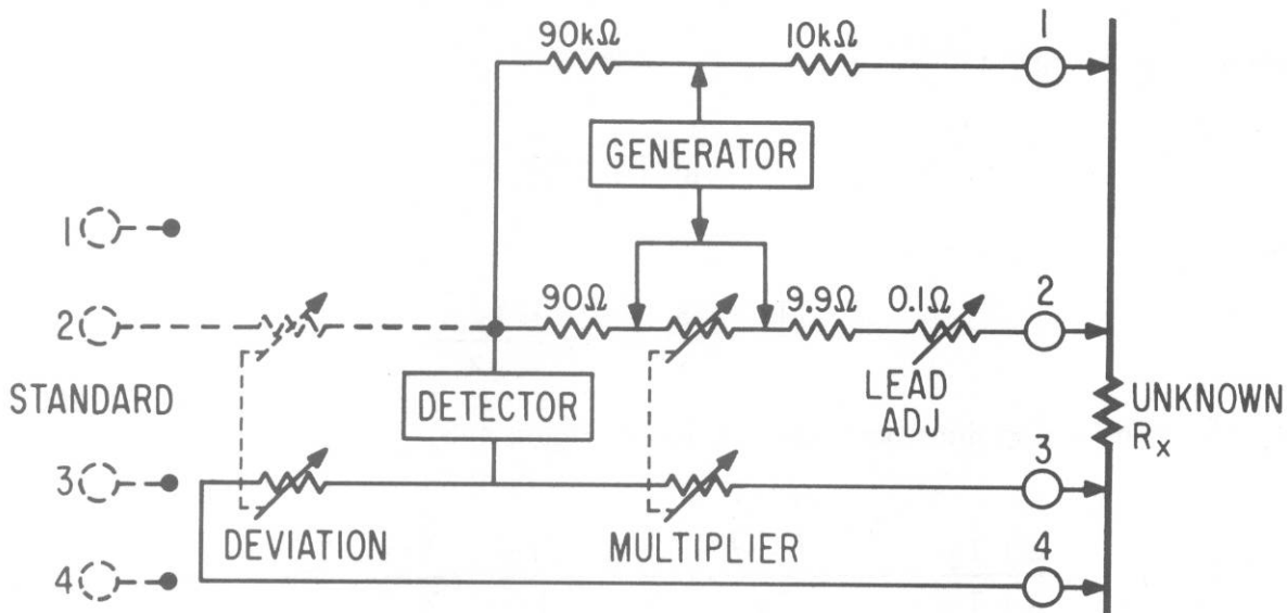
Figure 4-4. Lead Adjustment
