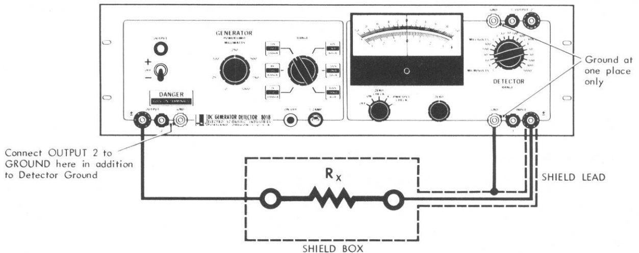
Figure 2-6. High-Resistance Measurement
