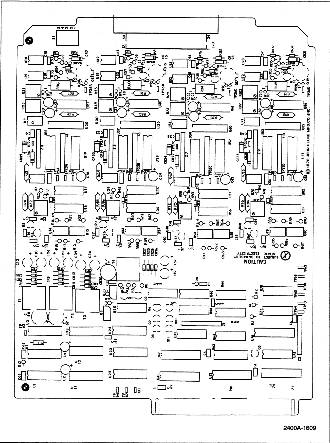
Figure 4-13. Option -011 Analog Output PCA
