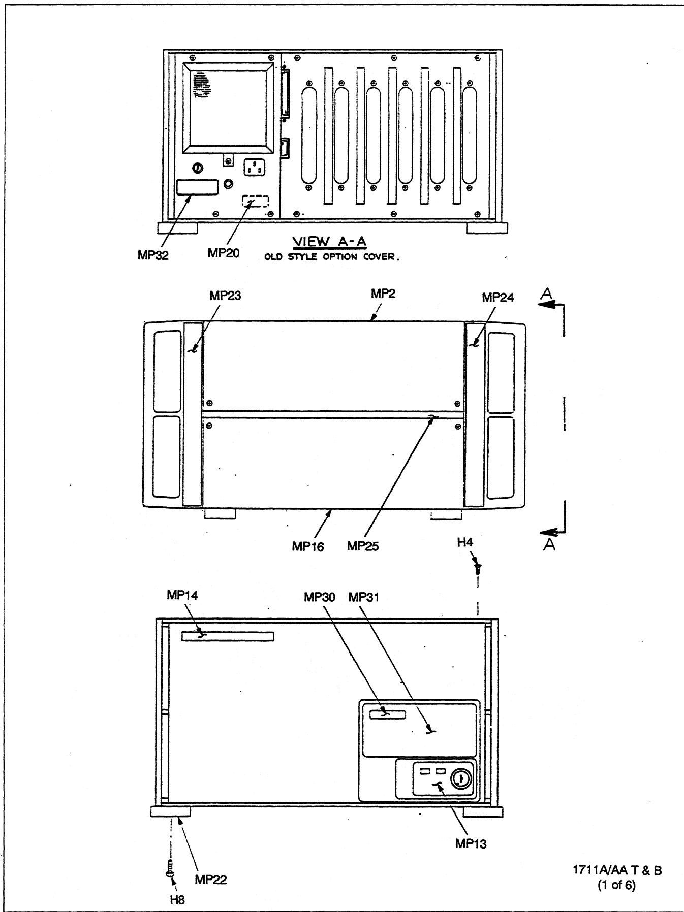
Figure 10-1. 1711A/AA Final Assembly
