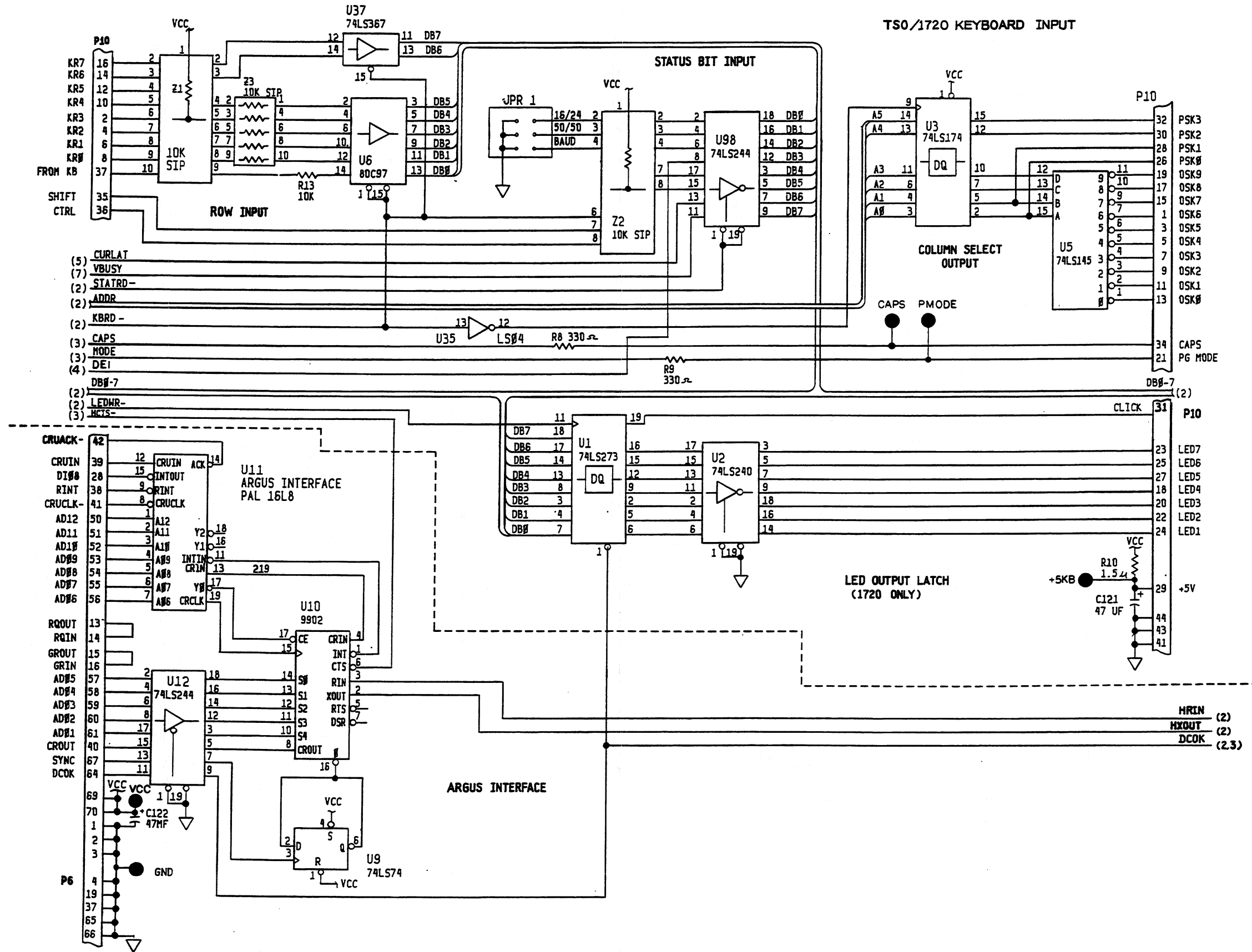
Figure 5-1. A1 Video/Graphics/Keyboard (VGK) Interface Module (cont)
