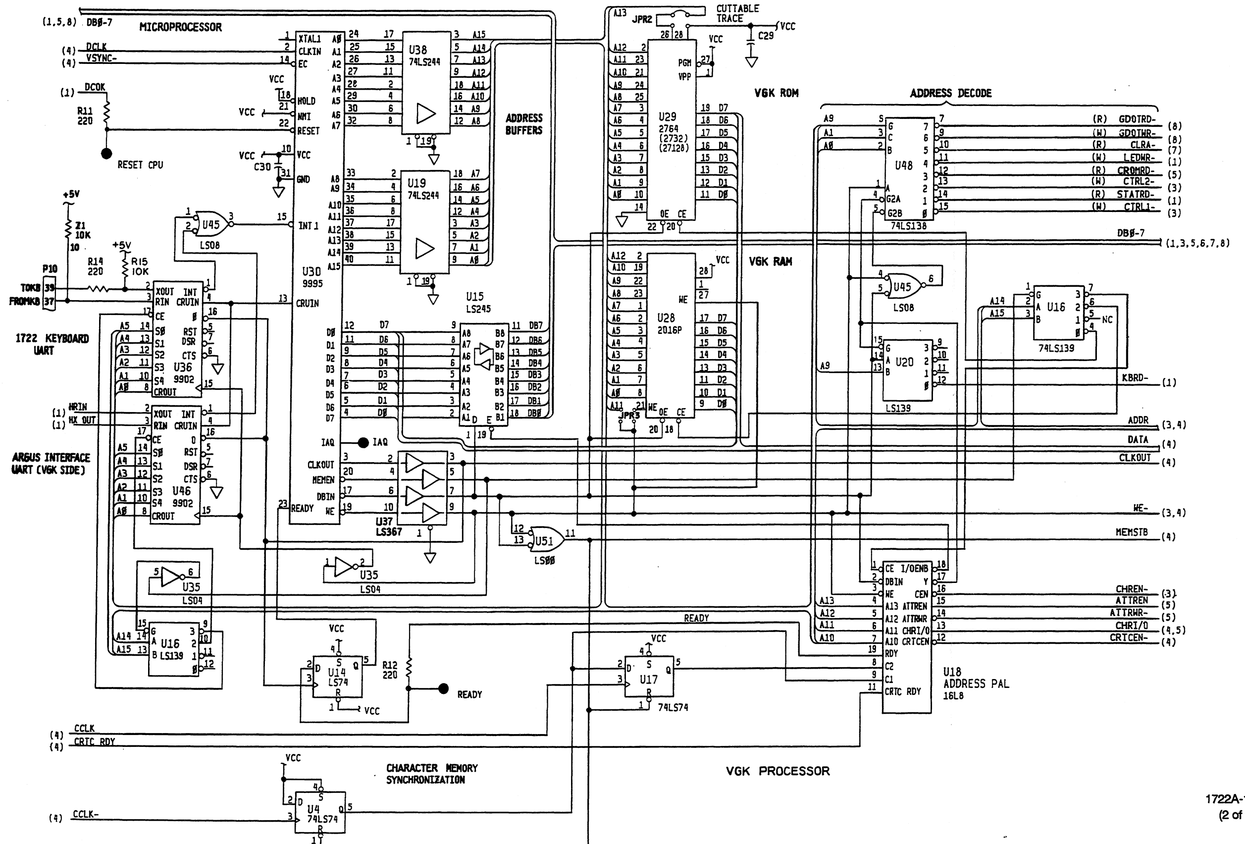
Figure 5-1. A1 Video/Graphics/Keyboard (VGK) Interface Module (cont)
