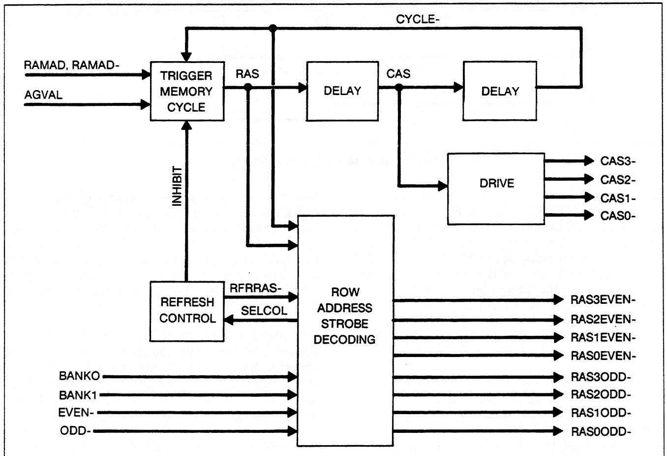
Figure 006-5. Memory Cycle Generation Circuitry
