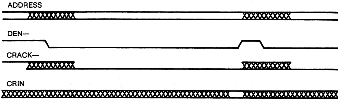
CRU READ CYCLE
