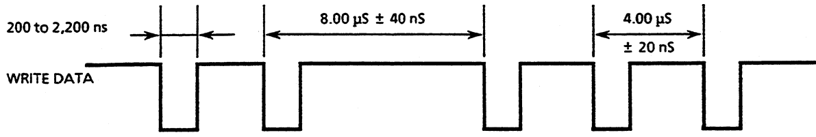
FIGURE 6-4 WRITE DATA TIMING
