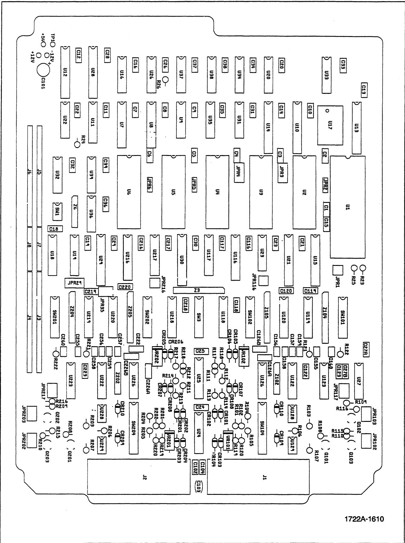
Figure 4-11. Option -009 Dual Serial Interface PCA
