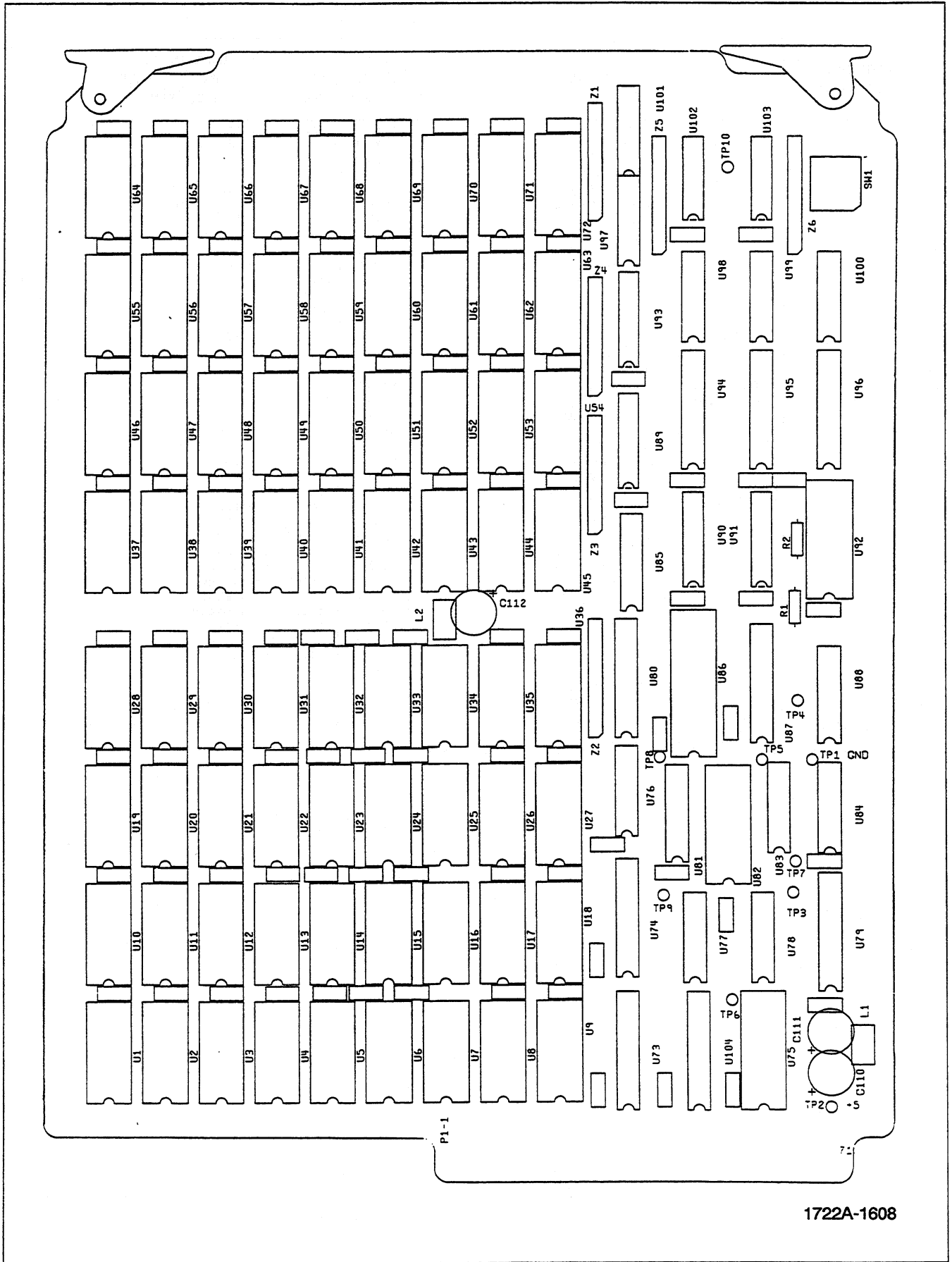
Figure 4-9. Option -006(256K) -007(512K) -016(1M) -017(2M) RAM Expansion PCA
