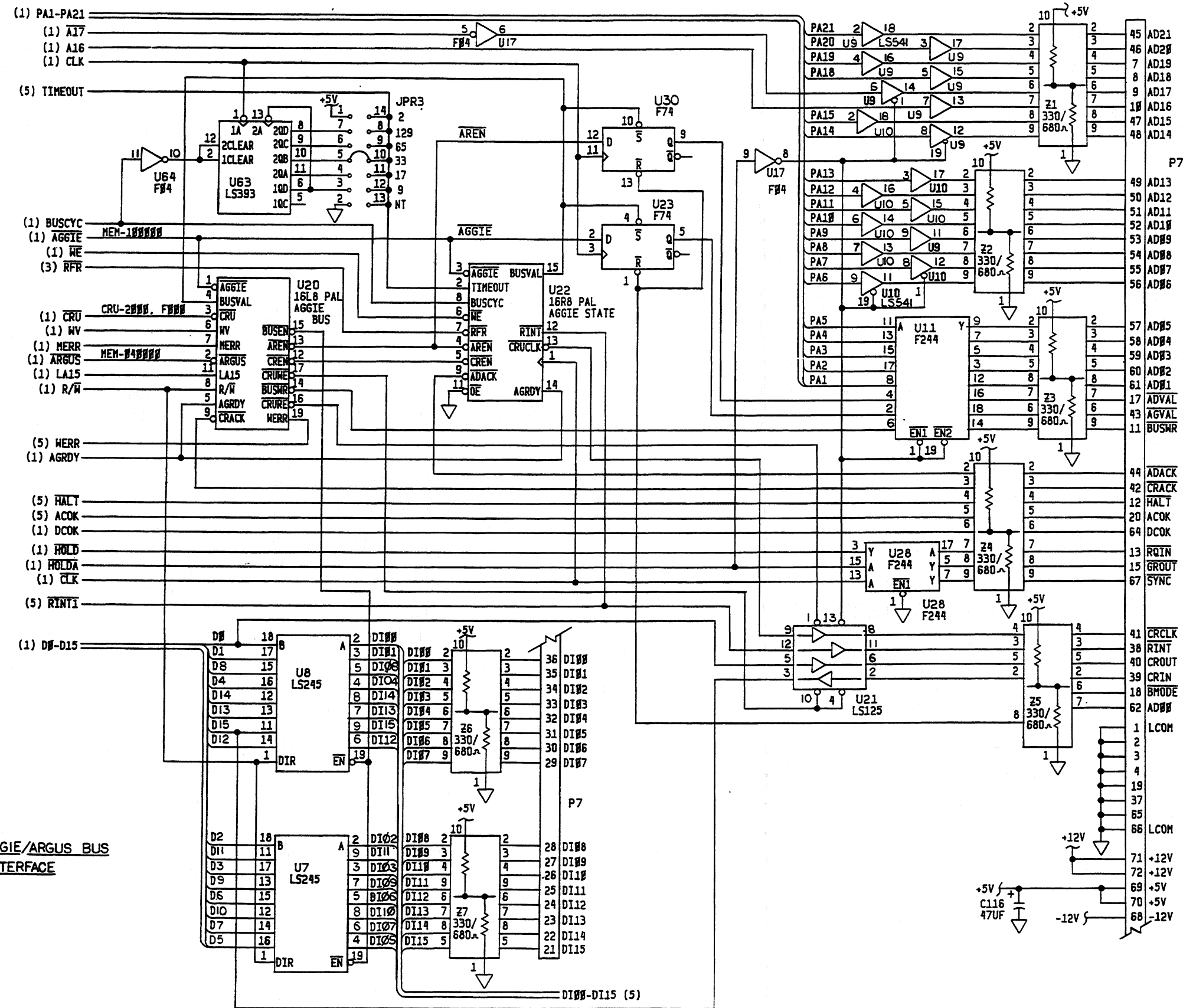
Figure 5-5. A4 Single-Board Computer (SBC) Module (Rev.K) (cont)
