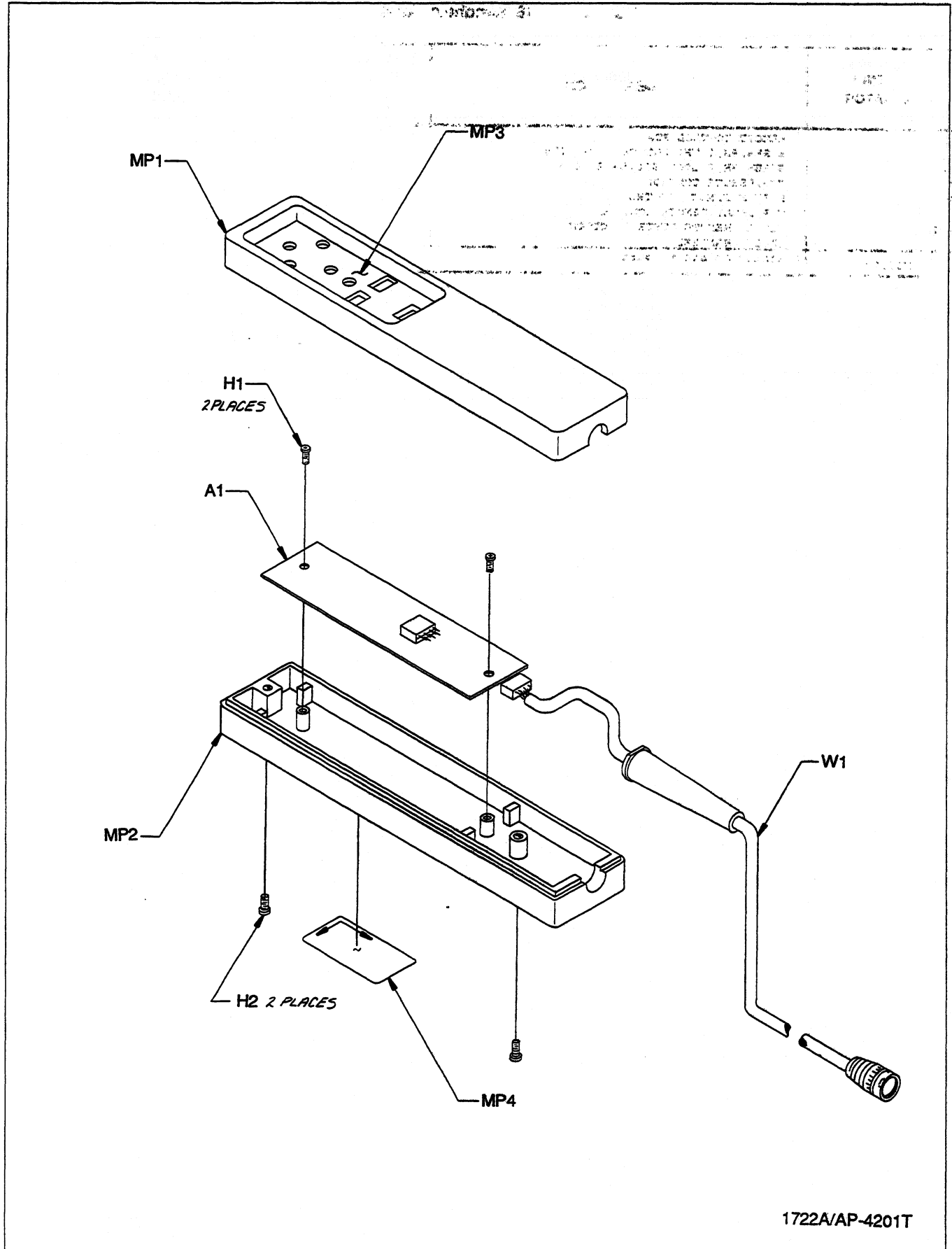
Figure 11-6. A16 Handheld Assembly
