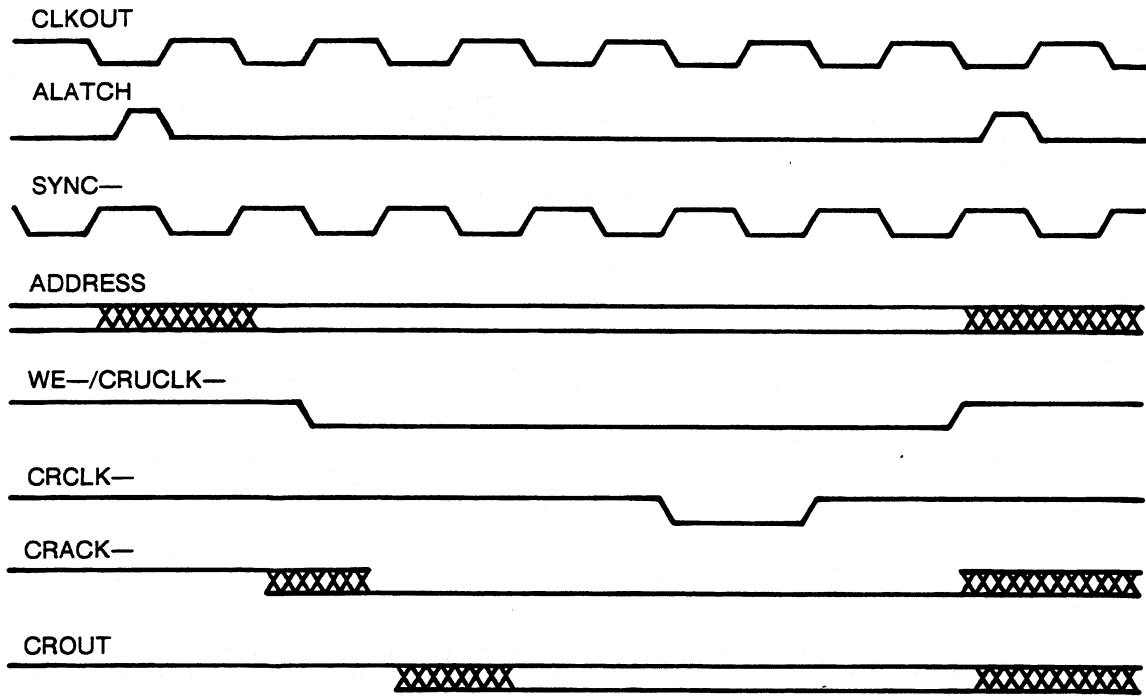
CRU WRITE CYCLE
