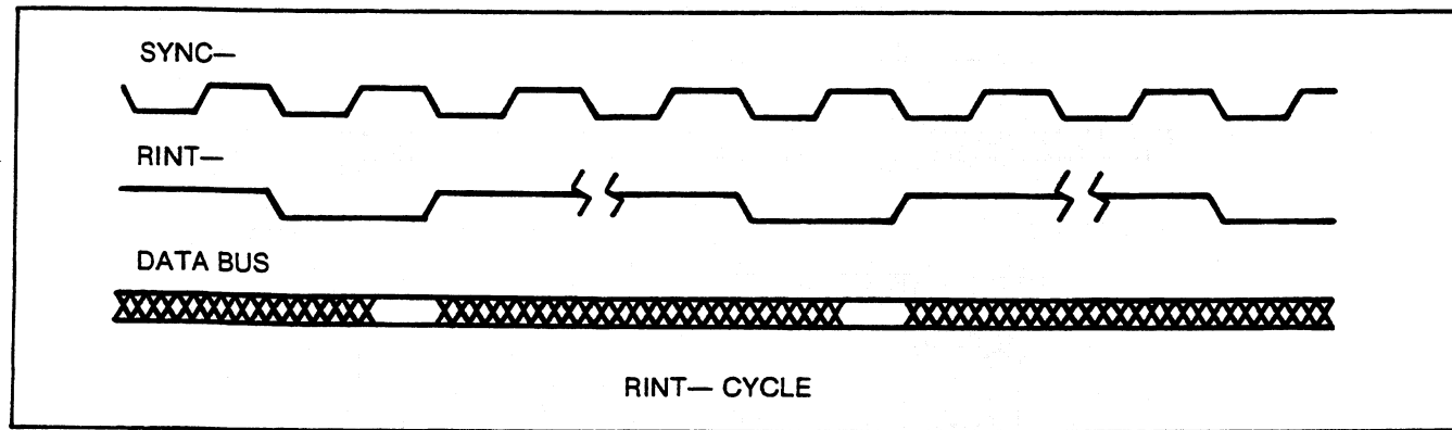
Figure 2-10. AGGIE Bus Interrupt Timing
