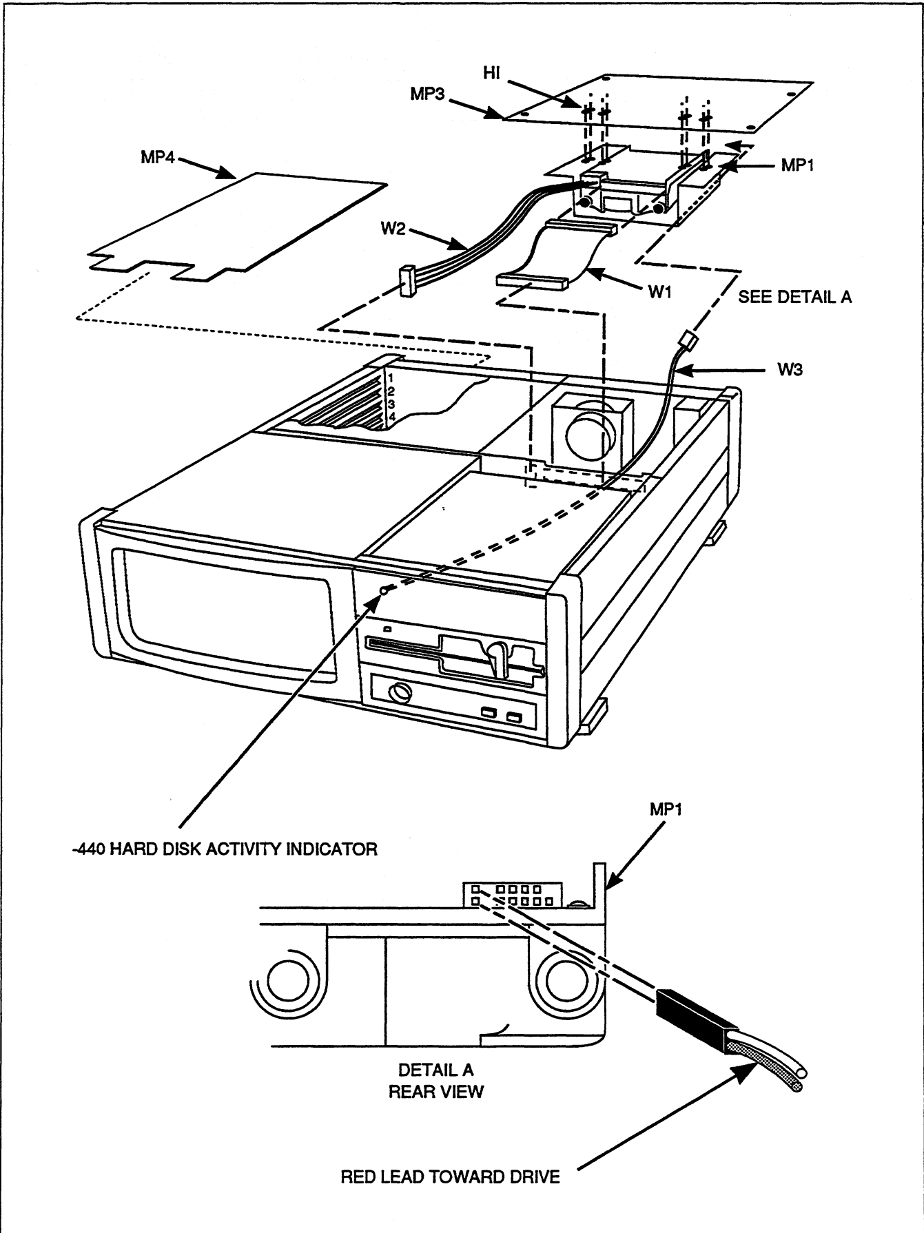
Figure 4-16. Option 1722A-440 Hard Disk, 40M
