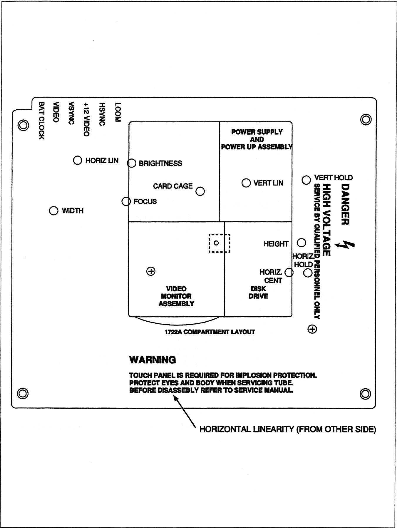
Figure 3-22. Video Adjustment Locations (Data Ray)
