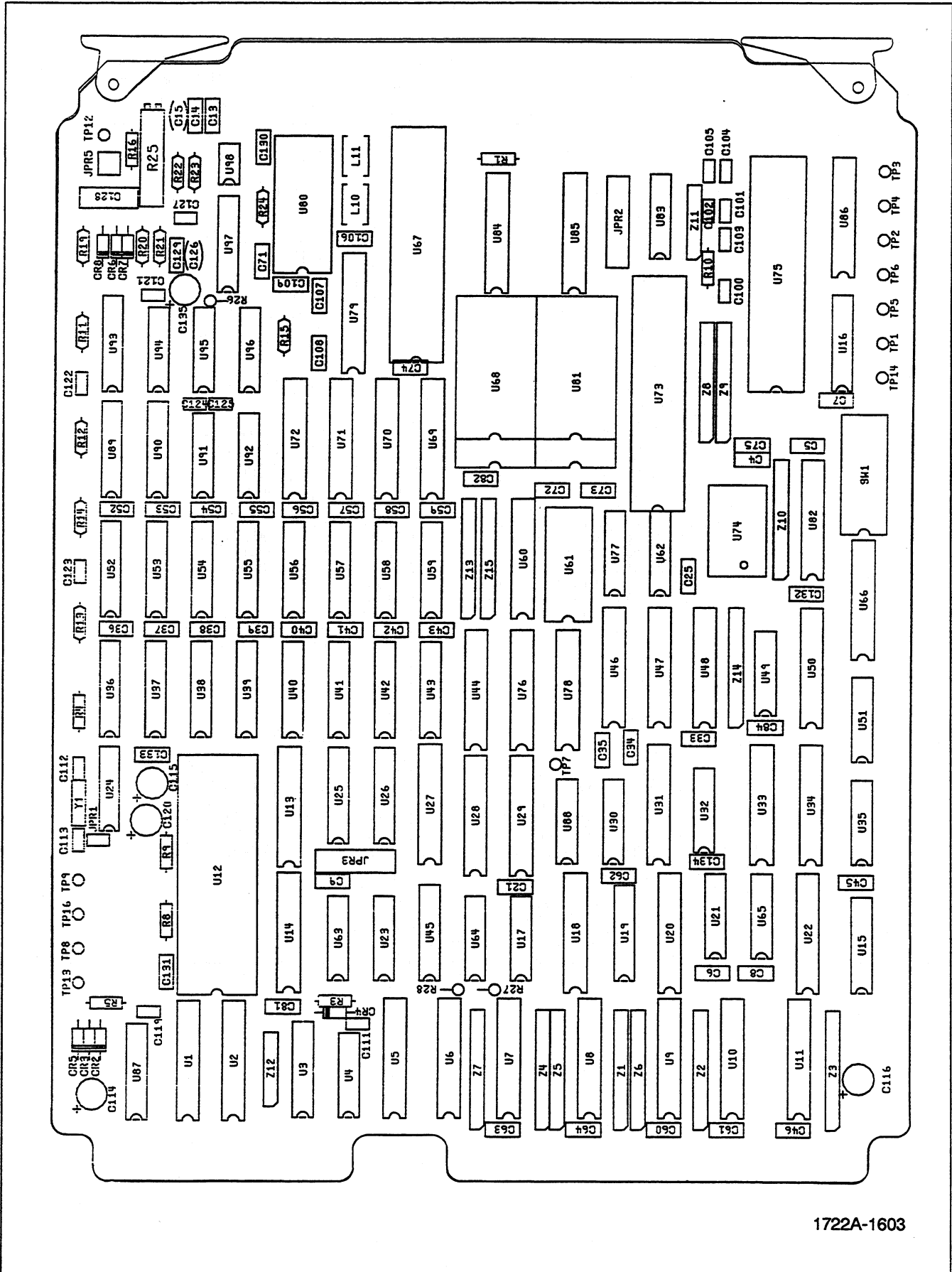
Figure 4-5. A4 Single-Board Computer (SBC) PCA
