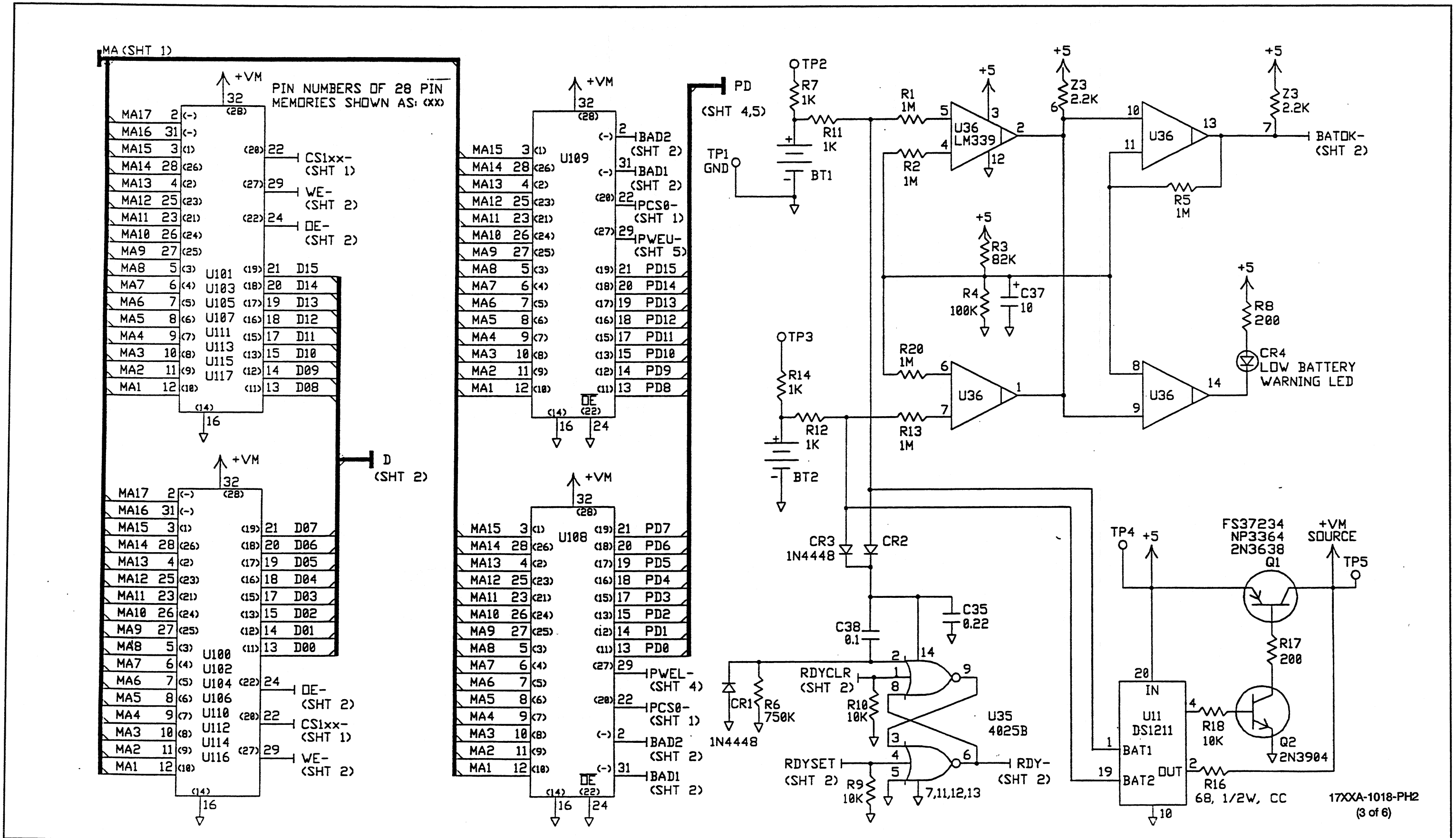
Figure 5-15. 018, 019, 020 PH2 NVRAM Modules (cont) (Rev. A)
