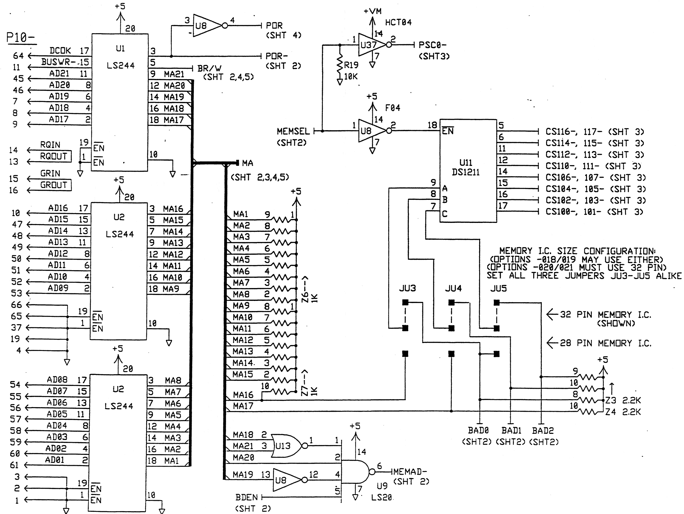
Figure 5-15. 018, 019, 020 PH2 NVRAM Modules (Rev. A) (cont)
