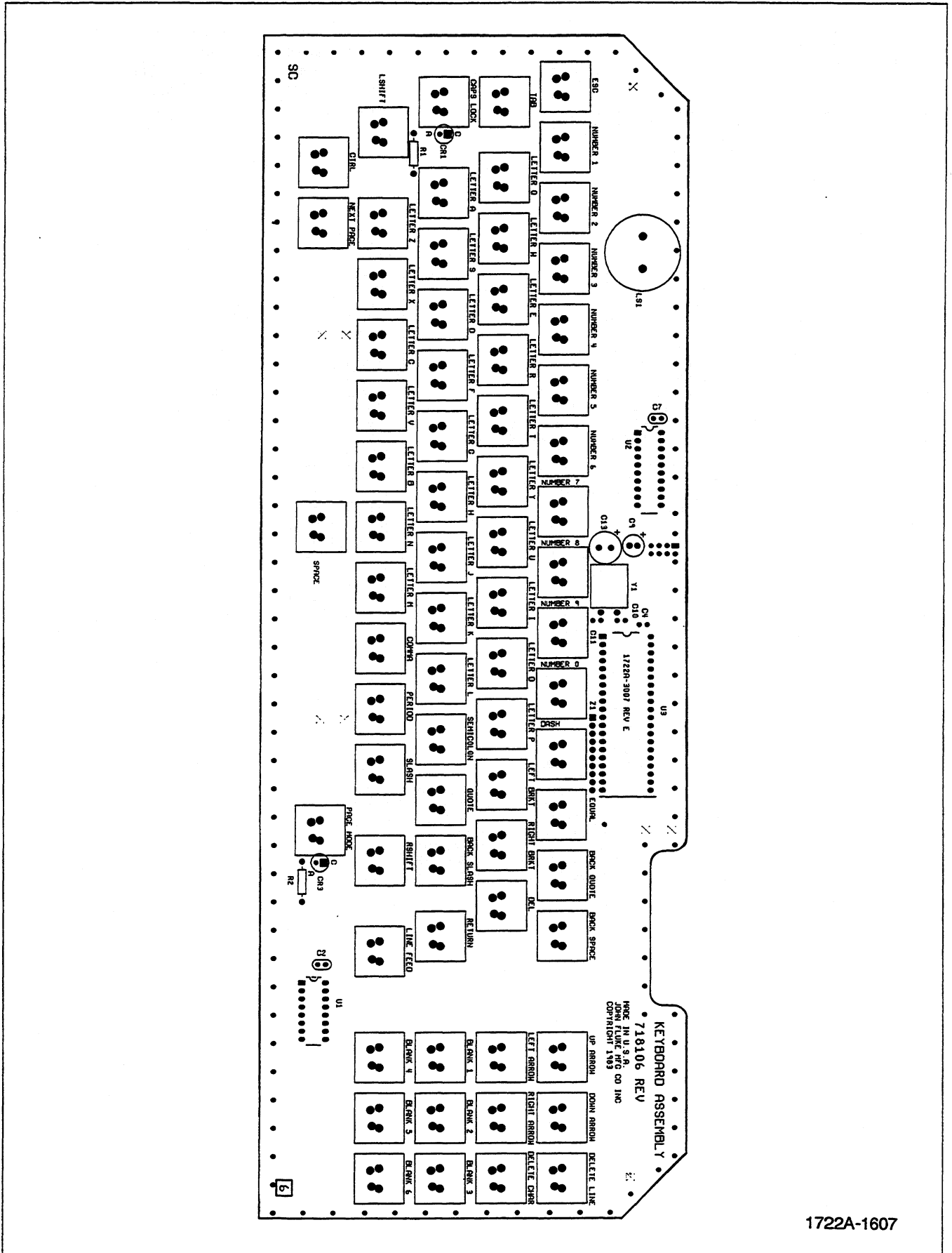
Figure 4-8. A6A1 Programmer's Keyboard PCA
