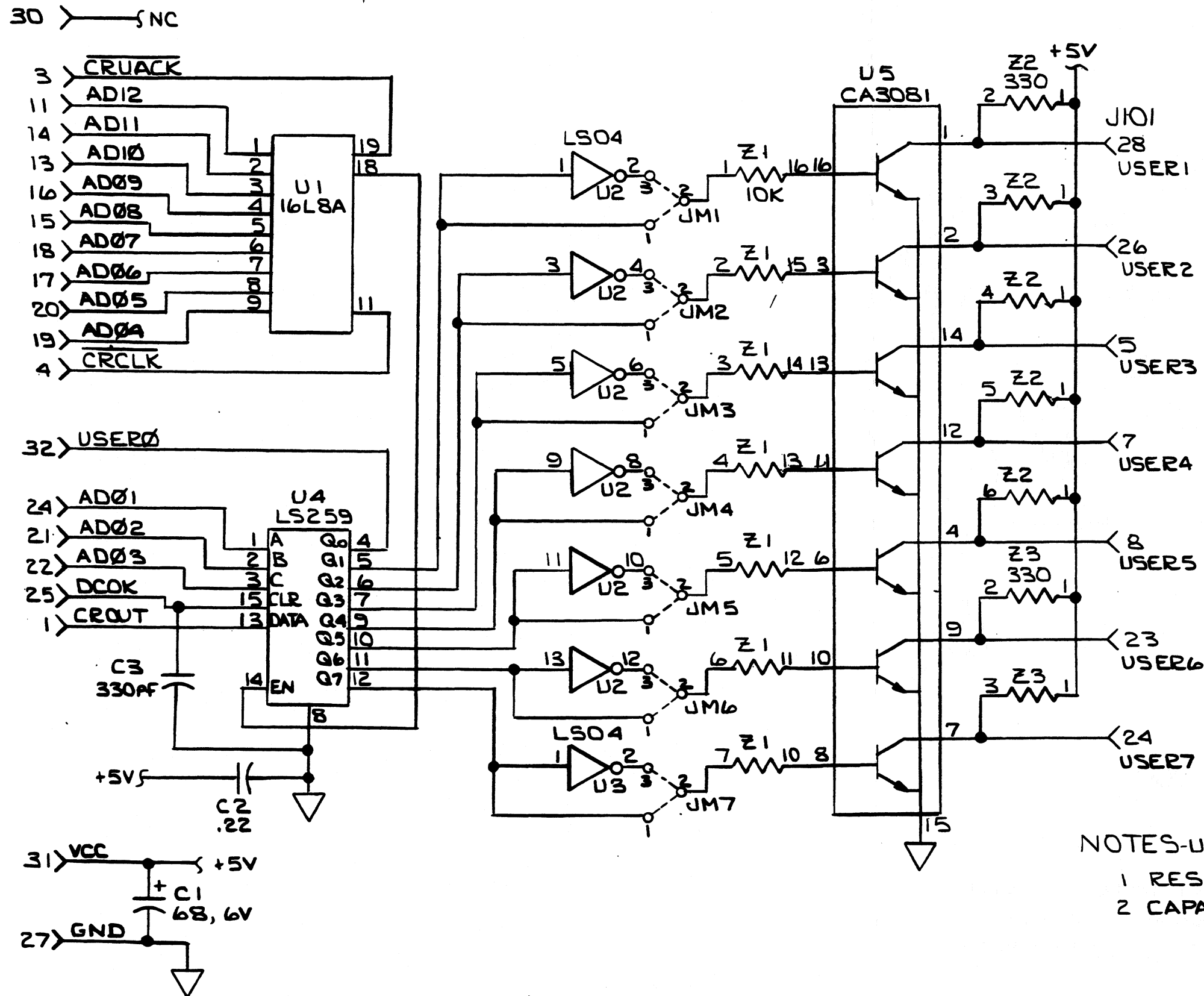
Figure 10-9. A19 User Defined Drive PCA
