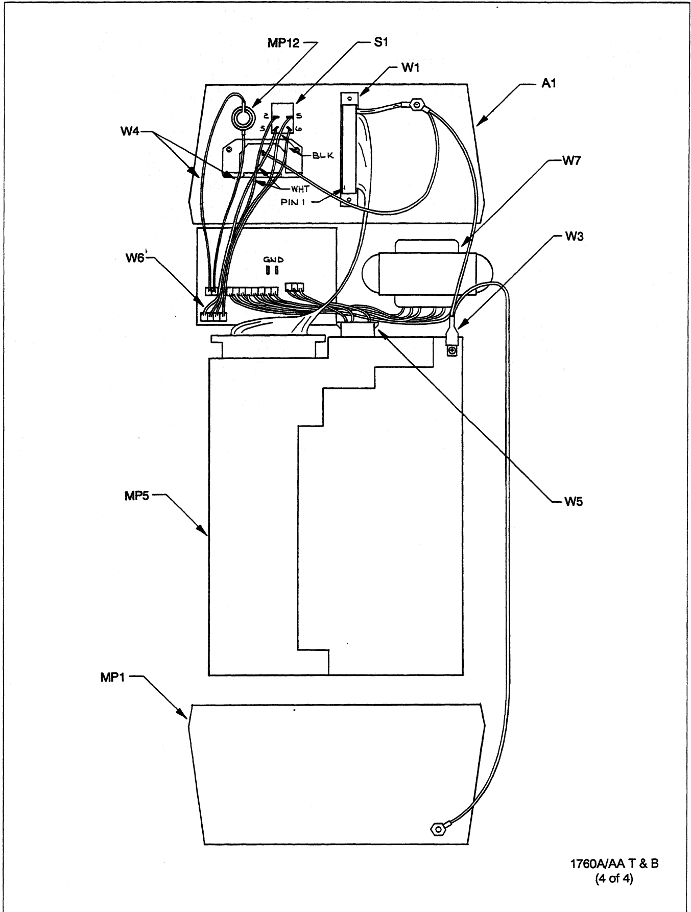
Figure 10-5. 1760/AA External Floppy Drive (cont)
