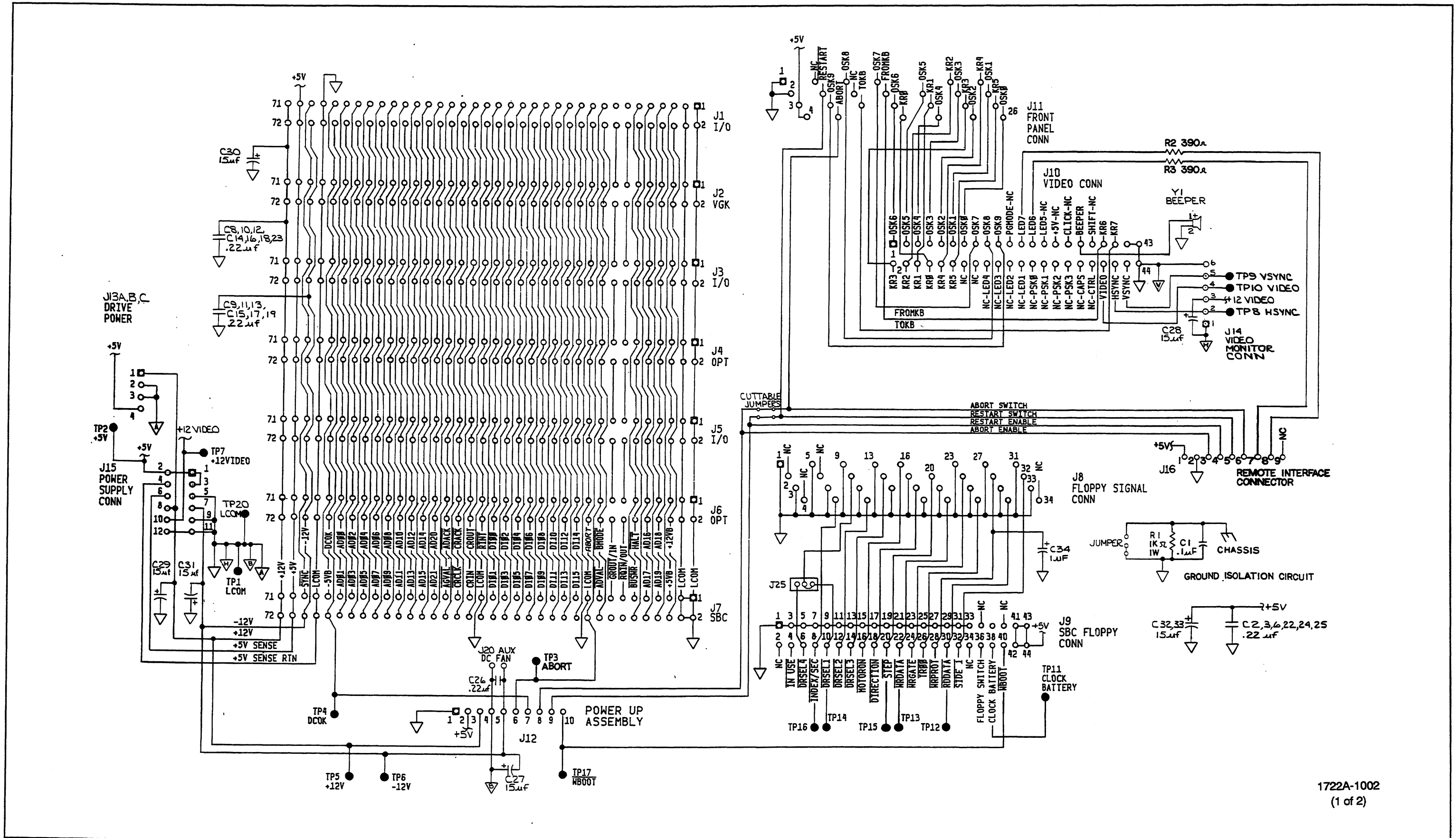
Figure 5-2. A2 Motherboard PCA (cont)
