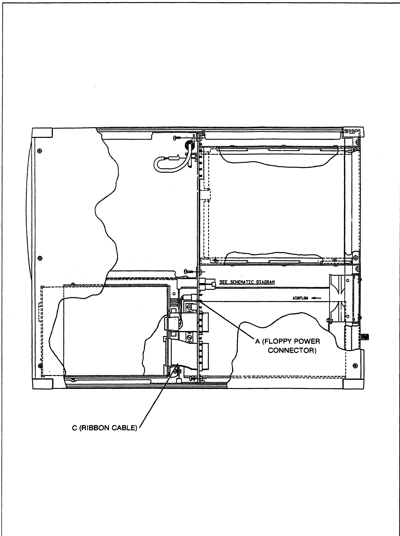
Figure 3-15. Top View of 1722A/1752A (New Chassis)
