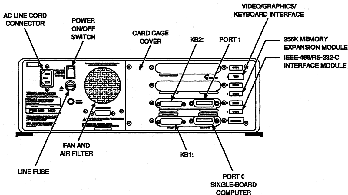
Figure 11-1. The 1722/AP Rear Panel
