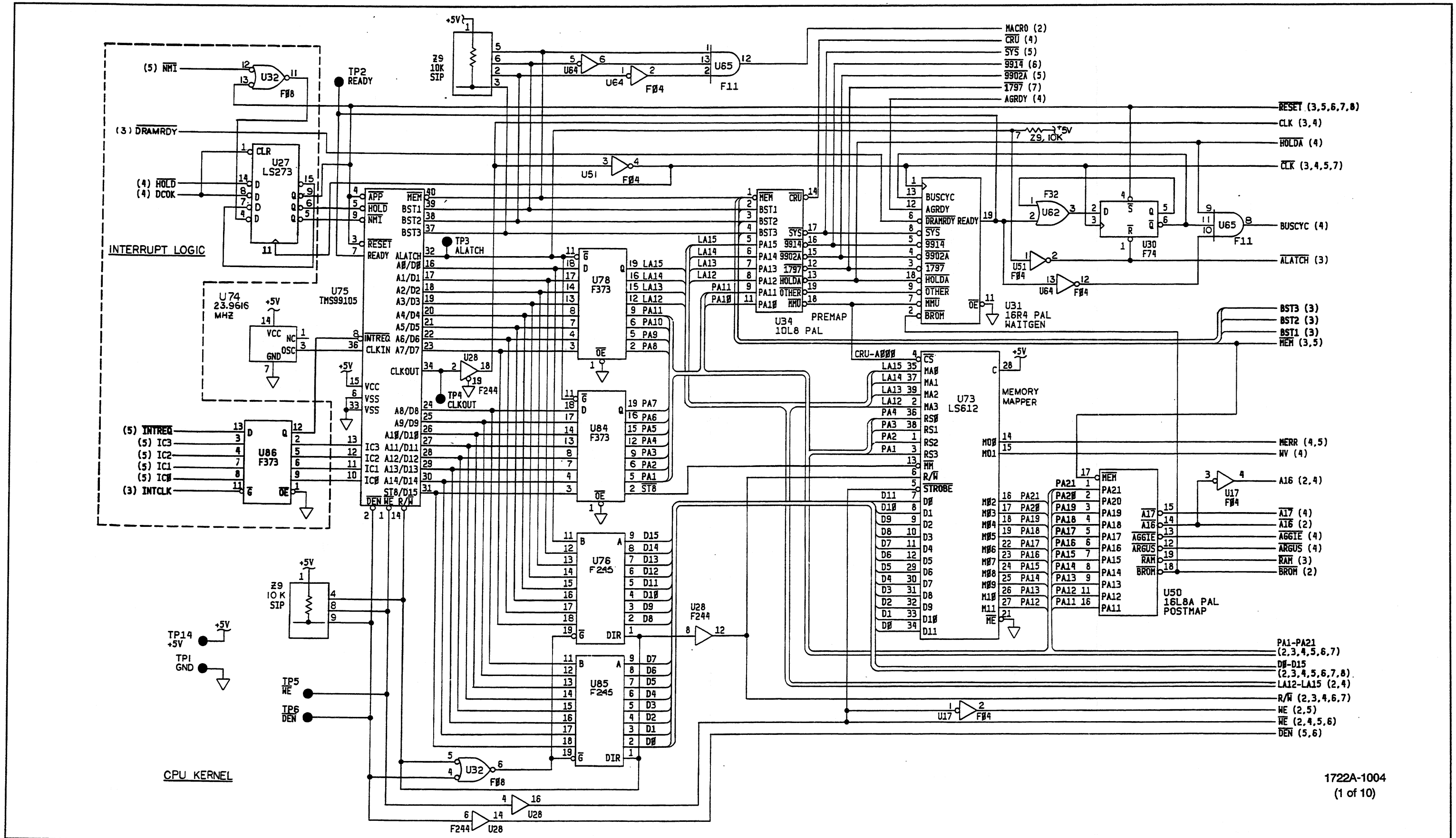
Figure 5-5. A4 Single-Board Computer (SBC) Module (Rev.K) (cont)
