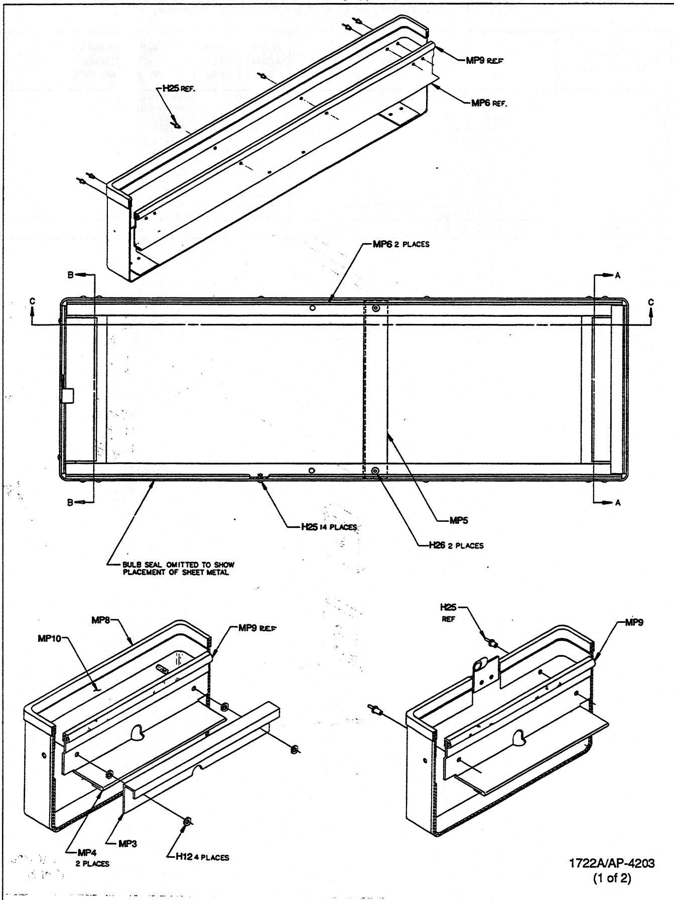
Figure 11-5. A15 Instrument Covers (Front & Back) Assembly
