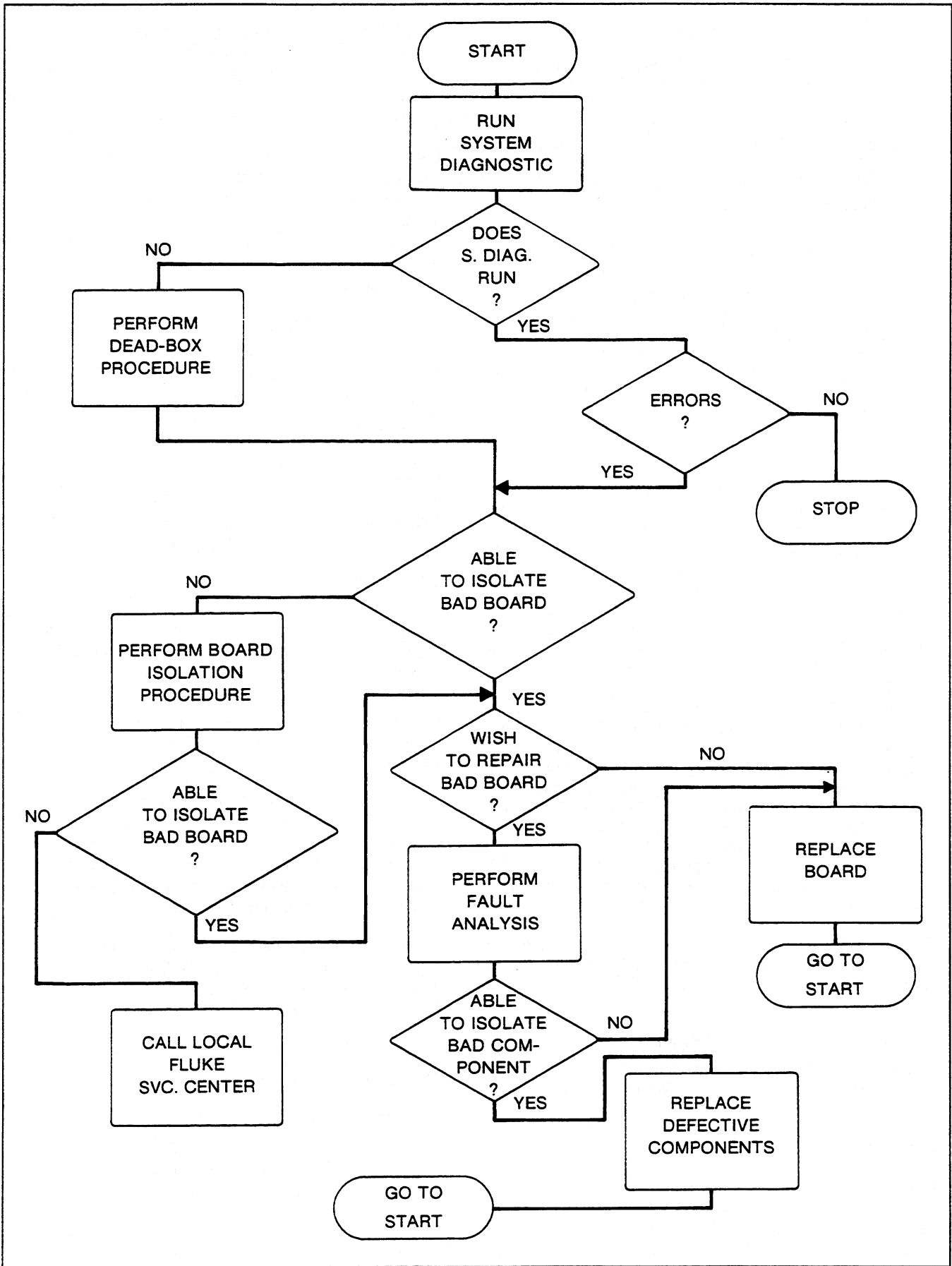
Figure 3-1. Overall Troubleshooting Flow Chart
