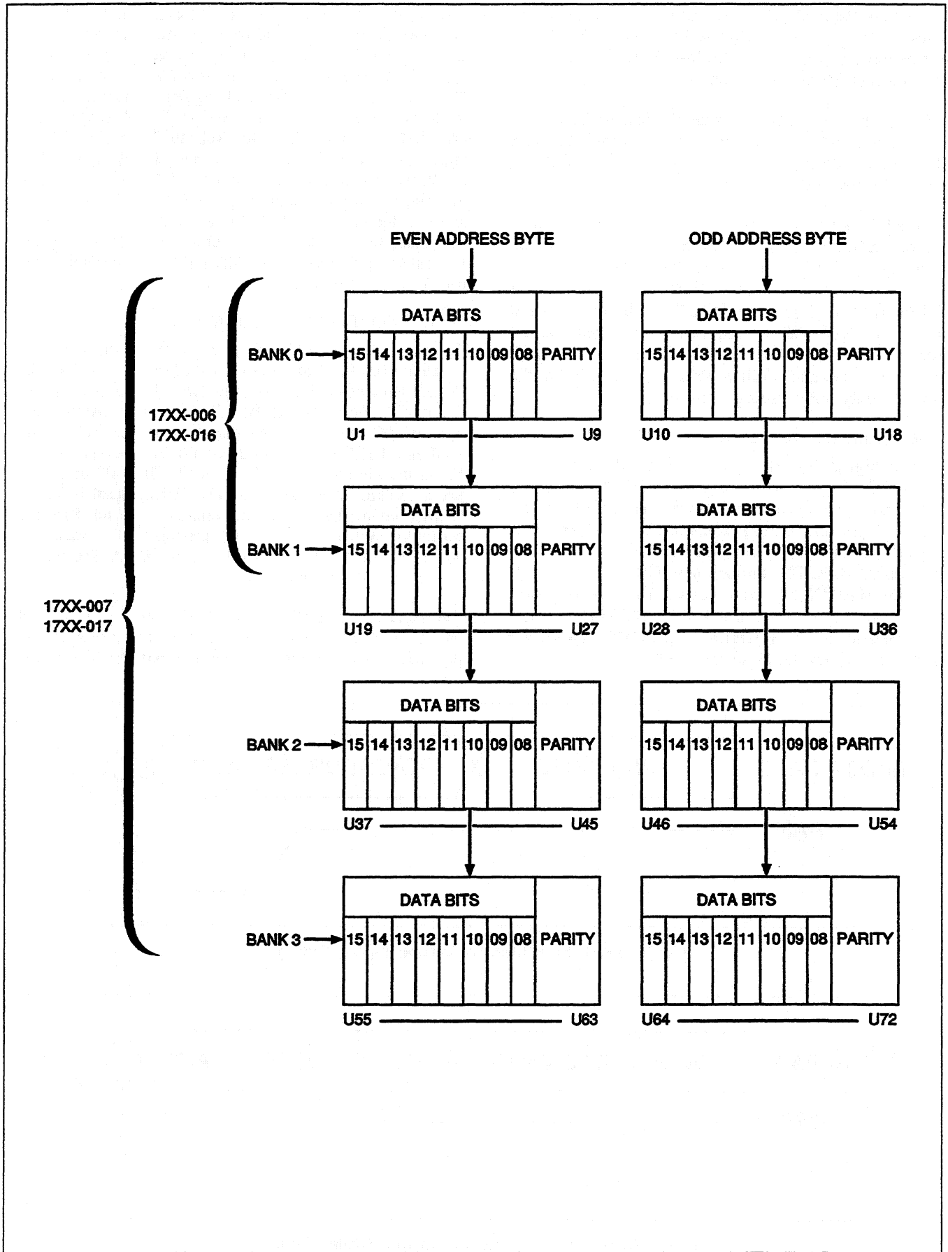
Figure 006-2. Memory Array Map
