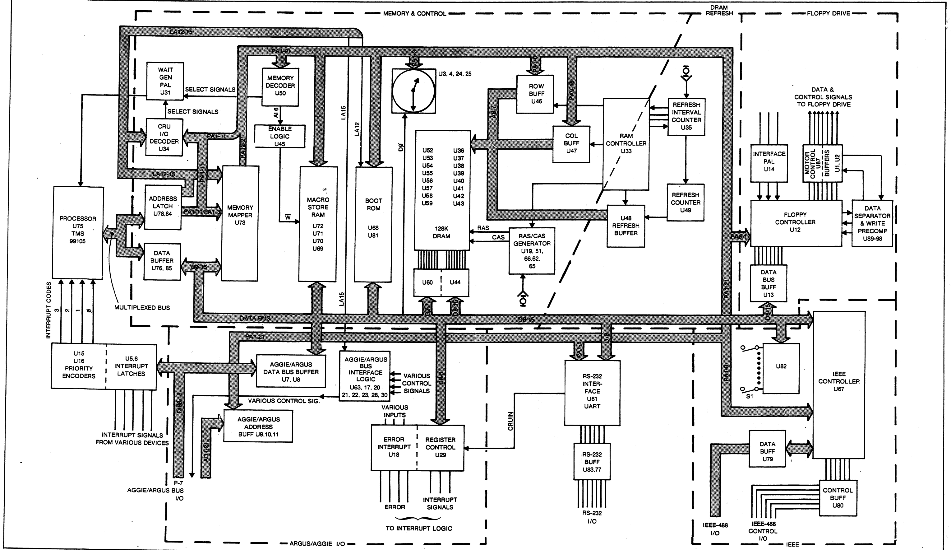
Figure 2-2. Detailed SBC Block Diagram
