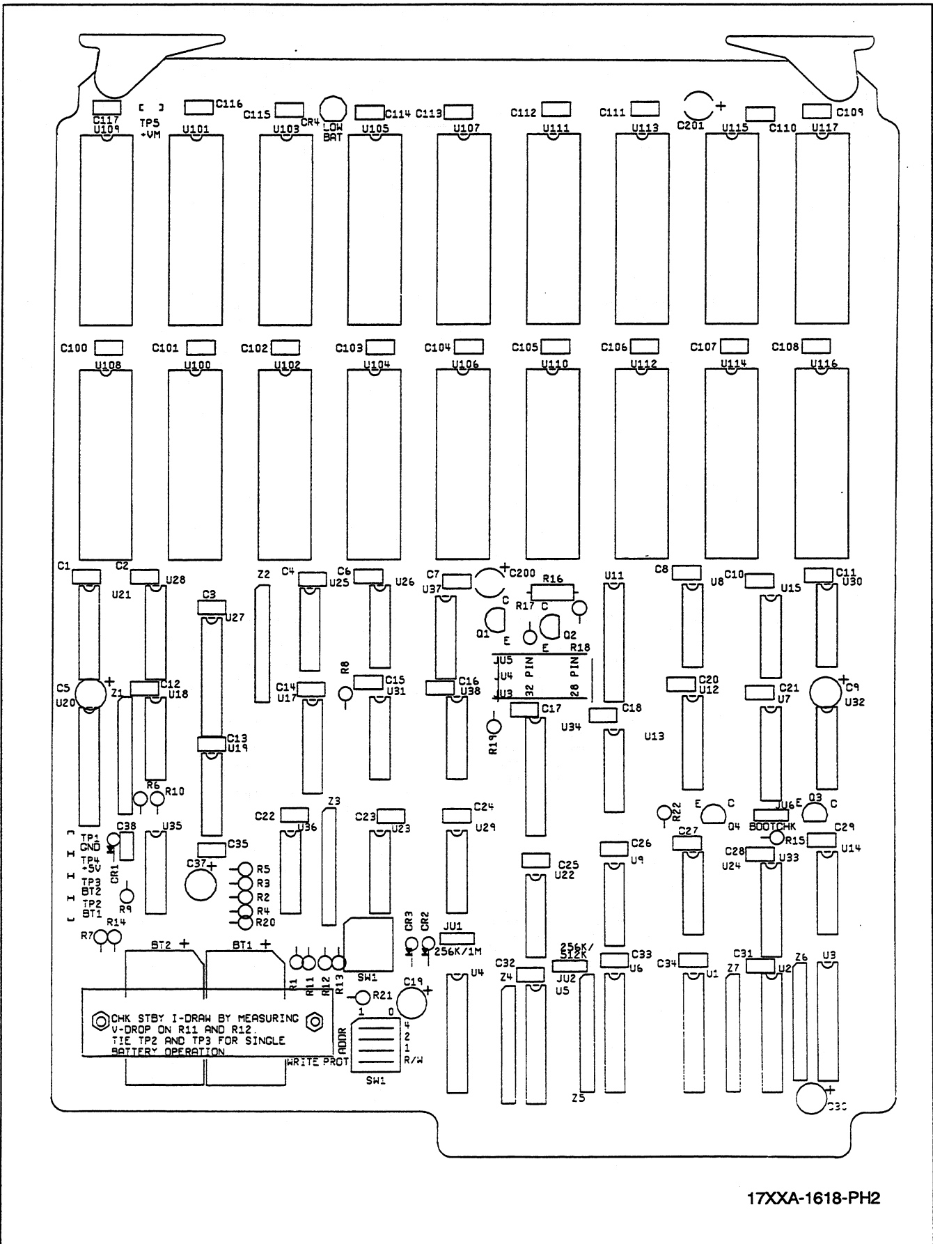
Figure 4-15. Option -018(256K) -019(512K) -020(1M) Non-Volatile RAM PCA (Rev. A)
