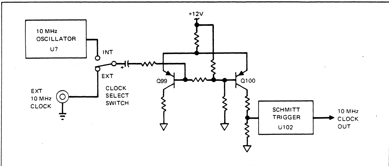
Figure 3-4. Reference Generator
