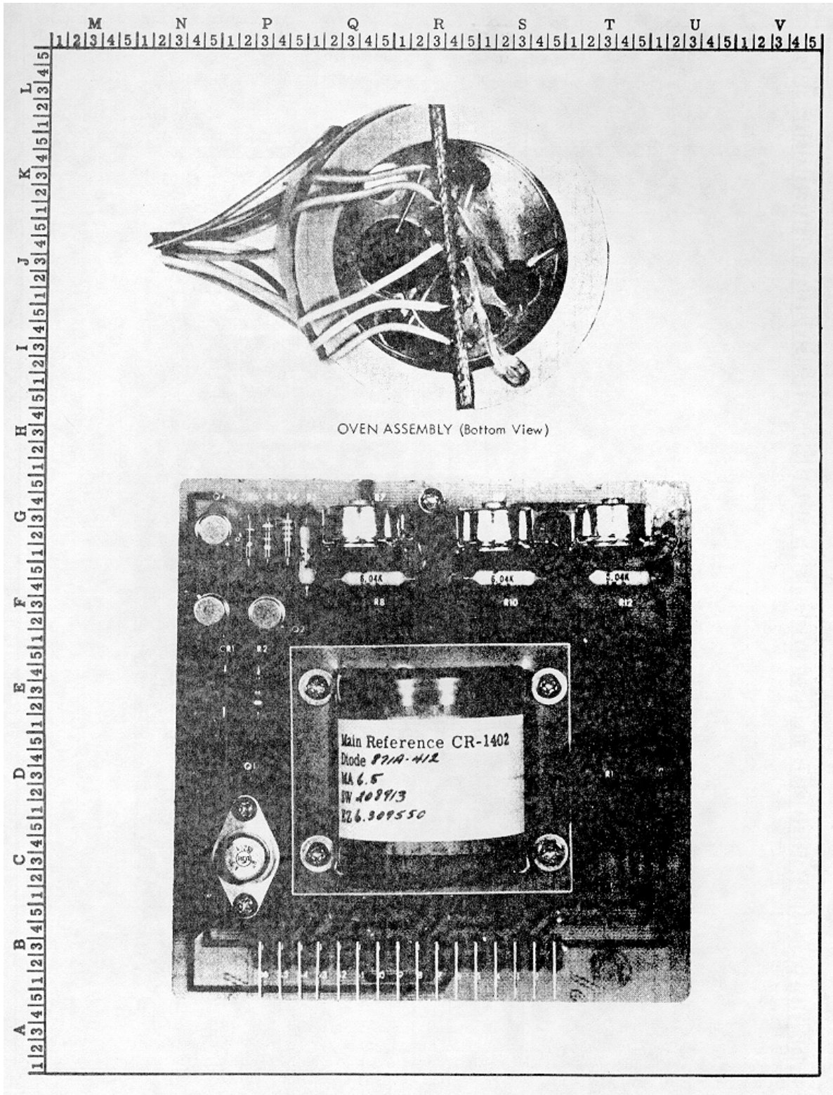
Figure 5-7. MASTER VOLTAGE REFERENCE P/C ASSEMBLY
