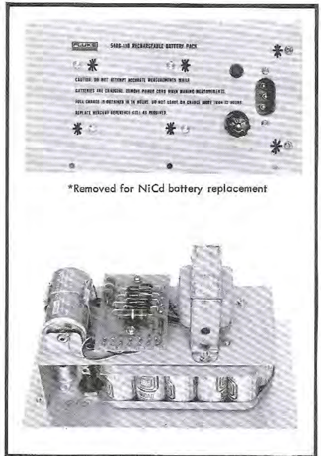
Figure 3-4. 540B RECHARGEABLE BATTERY PACK
