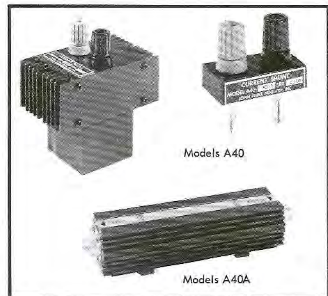
Figure 6-2. CURRENT SHUNTS
