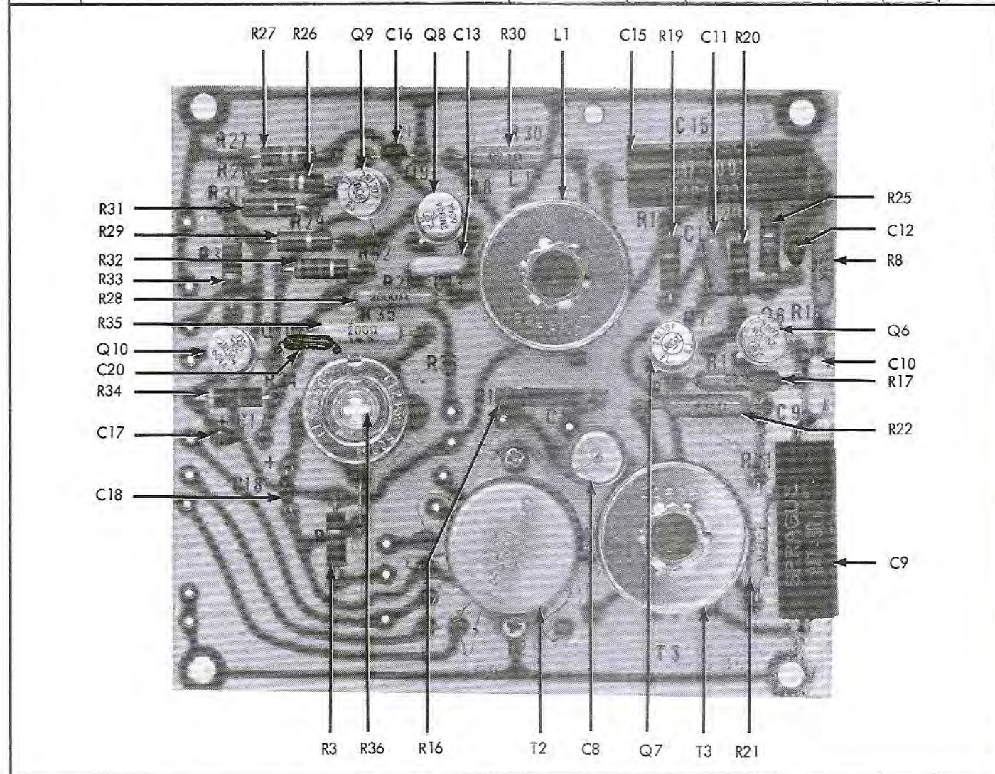
Figure 5-4. MAGNETIC MODULATOR/CARRIER AMPLIFIER ASSEMBLY
