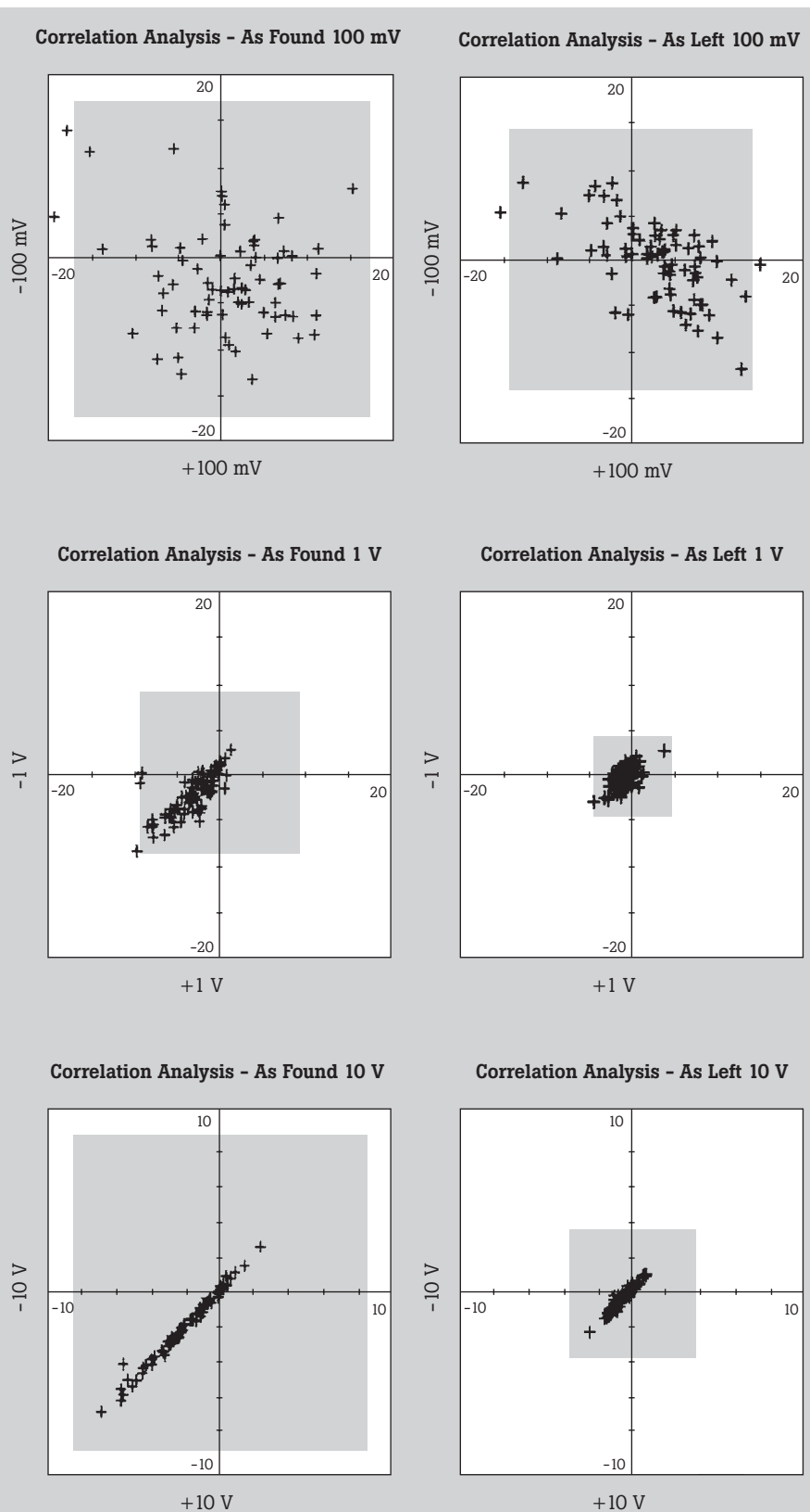
Figure 1. Scale values are ppm. Shaded boxes show one year specification, As Found , and 24 hour specification, As Left .
