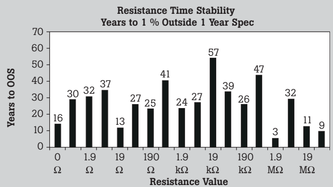
Figure 8. Resistance stability in years to 1 % out of tolerance.
