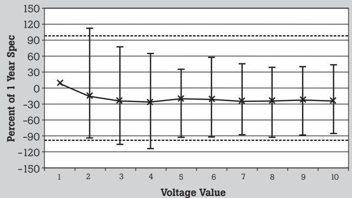
Figure 14. Deviations from nominal and 99 % limits, all verified direct voltages.
