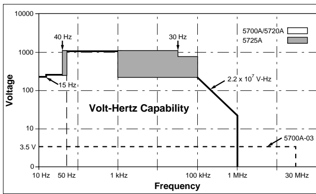
Figure 1-1. Volt-Hertz Capability
