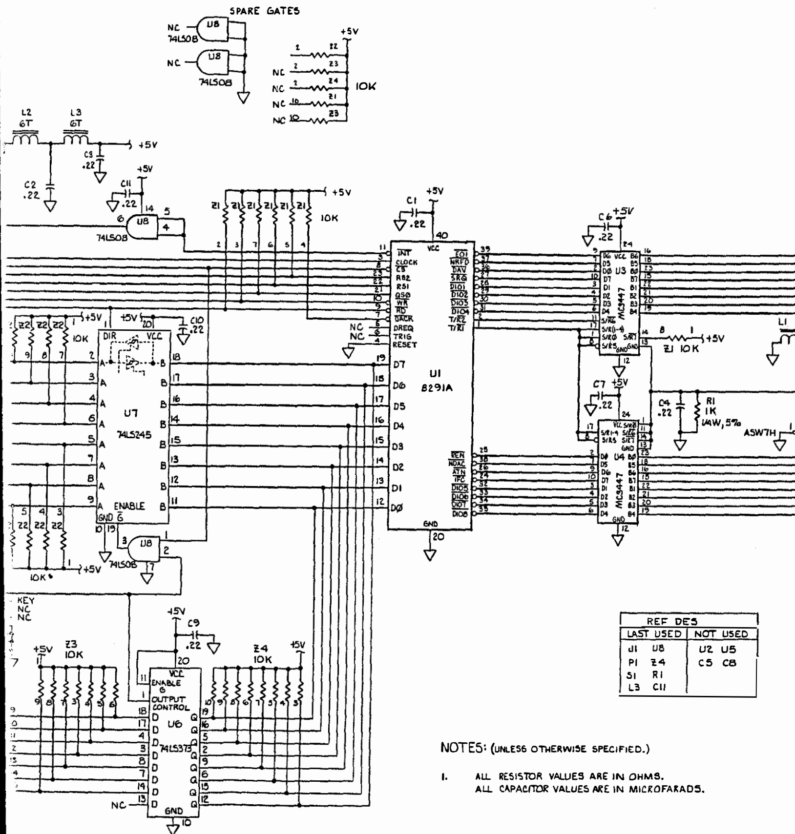
Figure 8-16. A3A3A1 I (Option -4)
