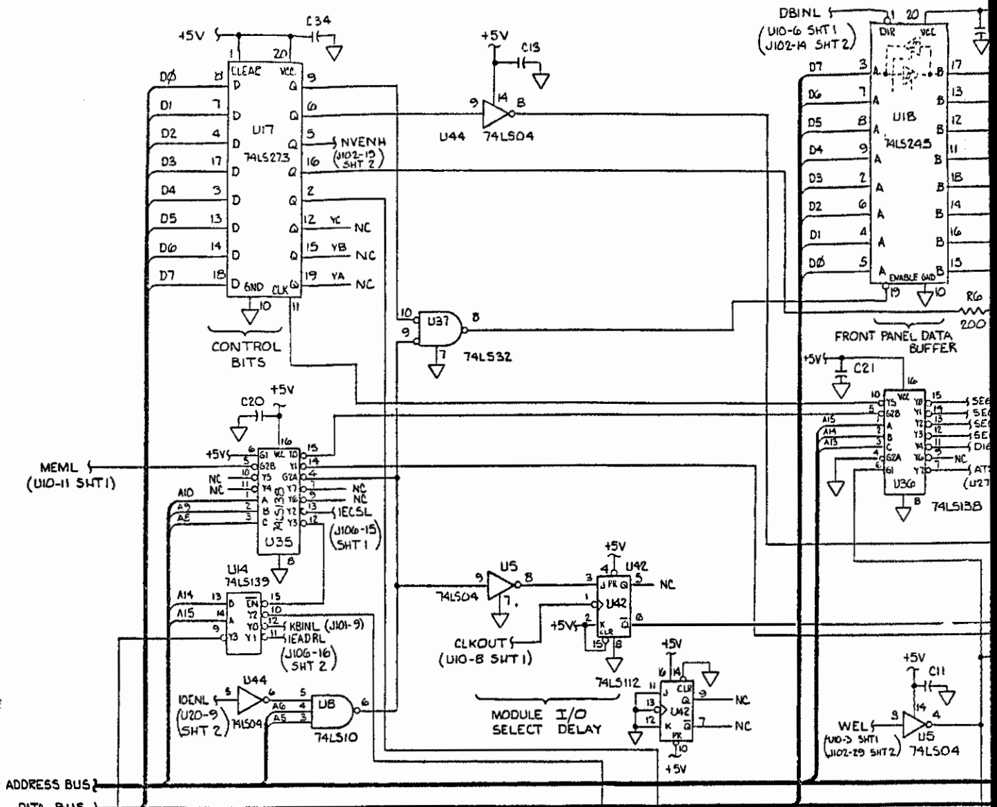
Fig 8-11 (3 of 3) Sht 1 of 2
