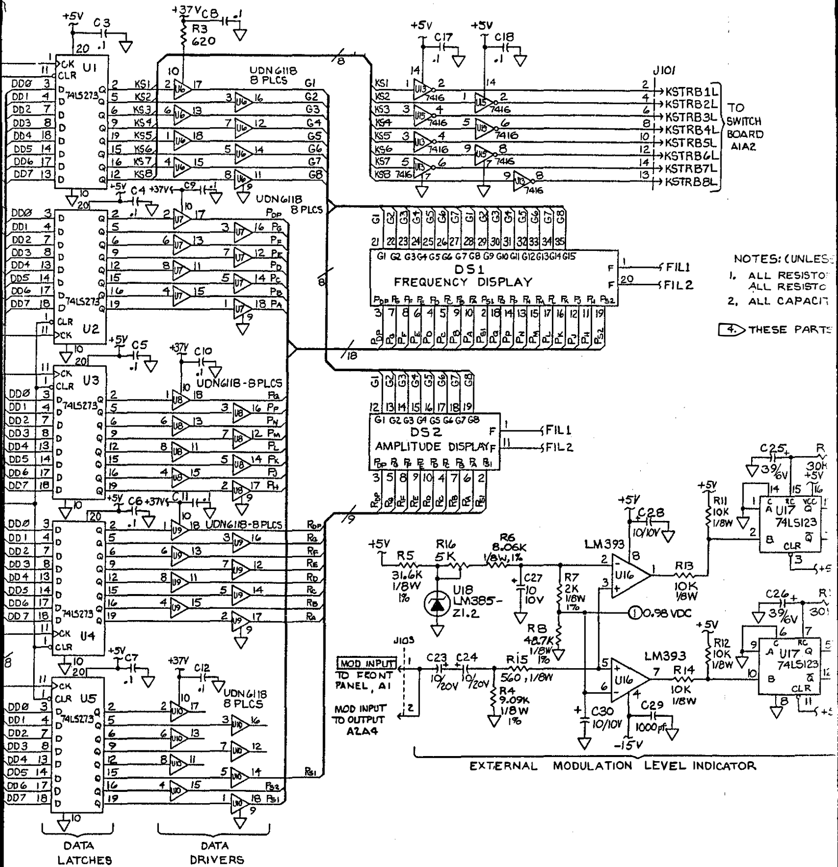
Fig 8-5 (Cont) Skt 2 of 3
