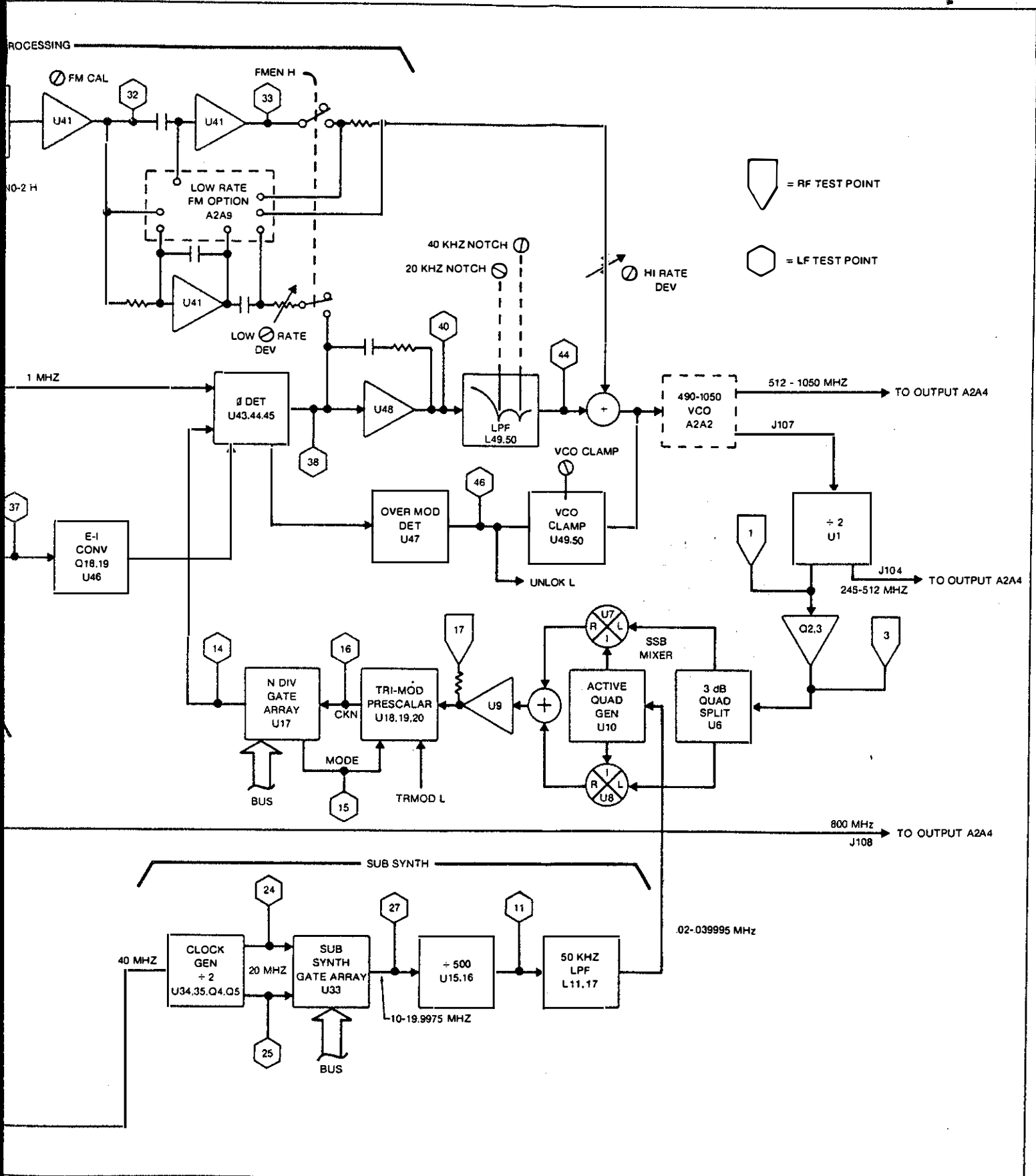
Figure 8-3. Synthesizer Block Diagram
