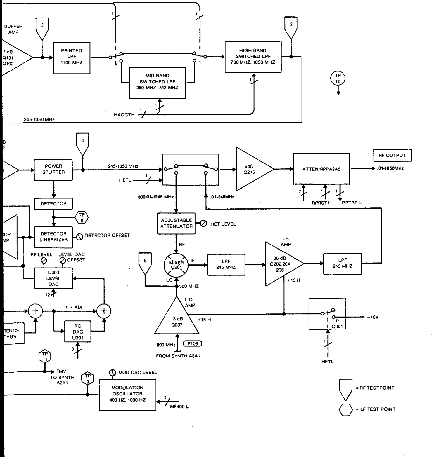
Figure 8-4. Output Block Diagram
