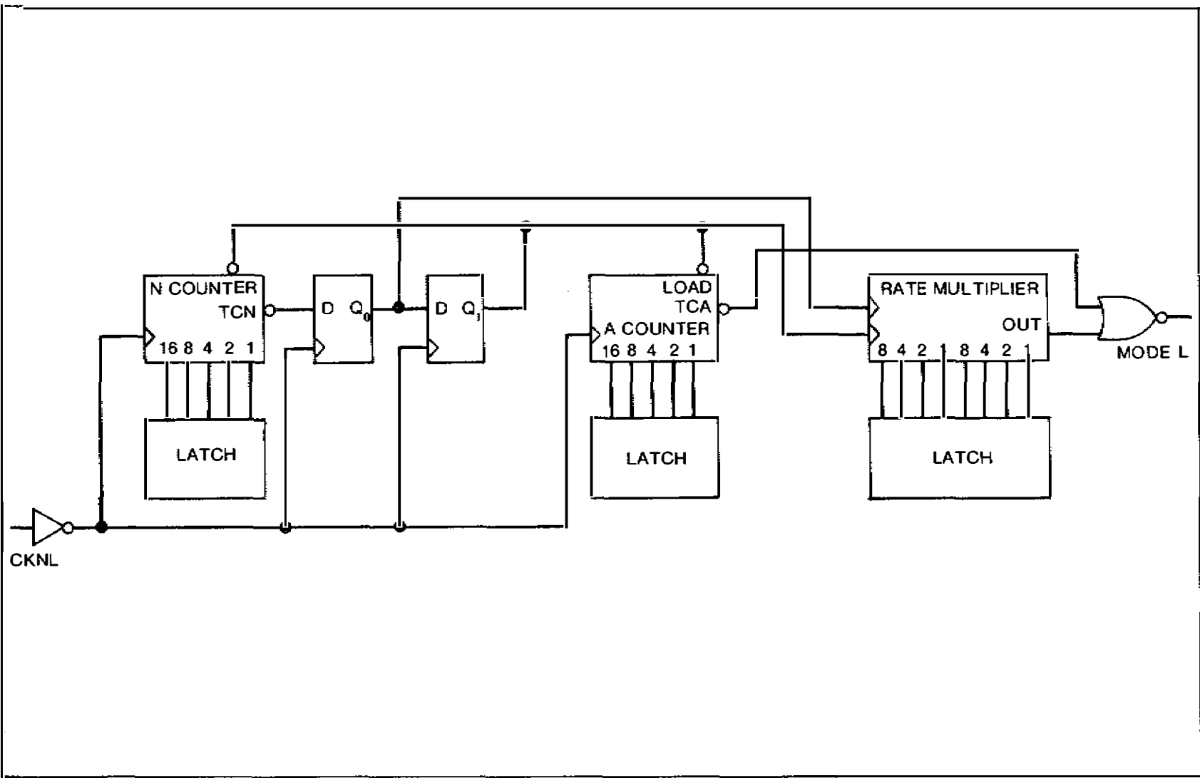
Figure 3-2. N-Divider Operation
