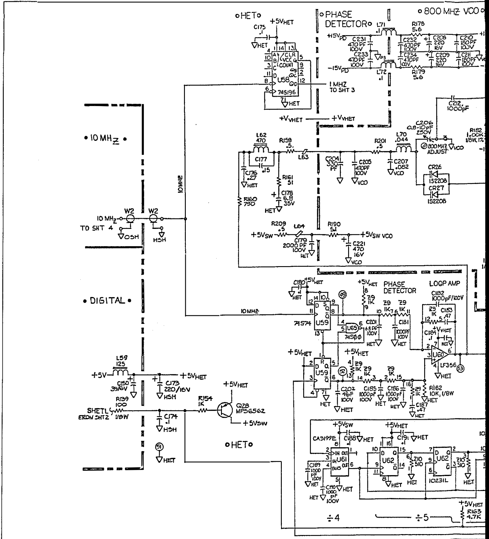
Fig 8-6 (5 of 5) Sht 1 of 2
