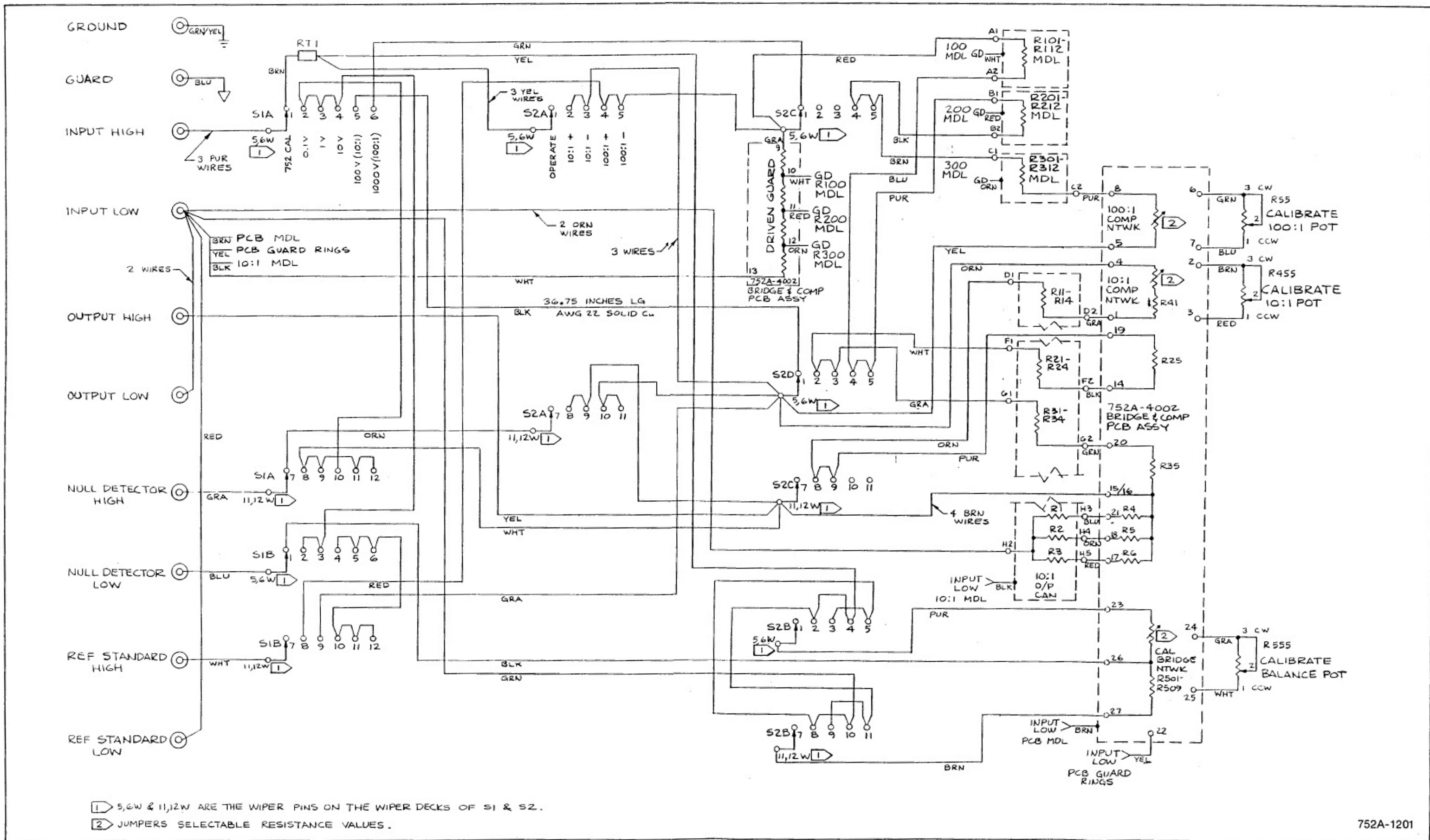
Figure 8-1. 752A Ref Divider Interconnect
